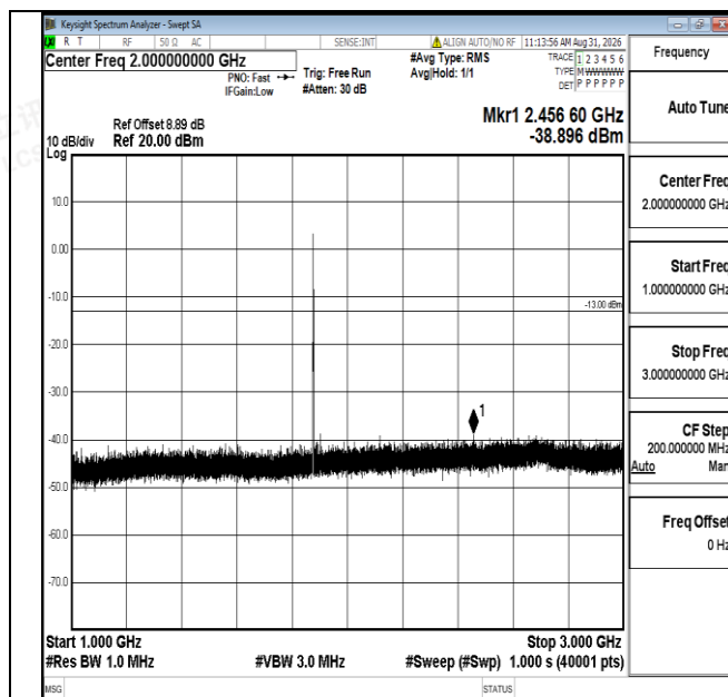
Band25-15MHz-16QAM-26365-1RB#0-1000~3000-PASS
