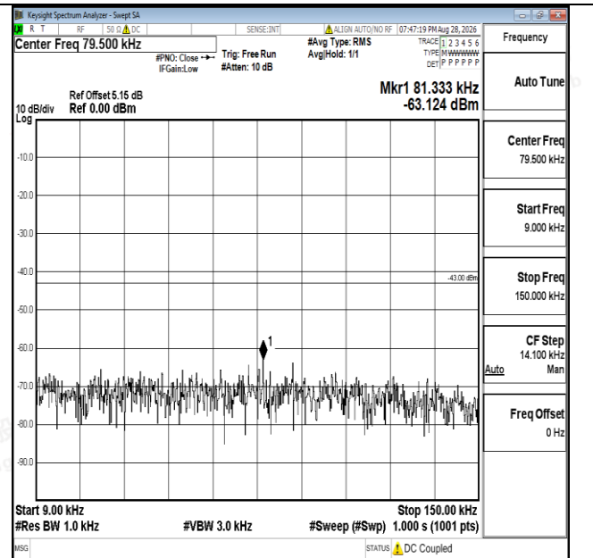
Band25-20MHz-16QAM-26140-1RB#0-0.009~0.15-PASS
