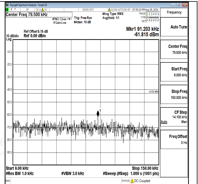
Band25-20MHz-16QAM-26590-1RB#0-0.009~0.15-PASS
