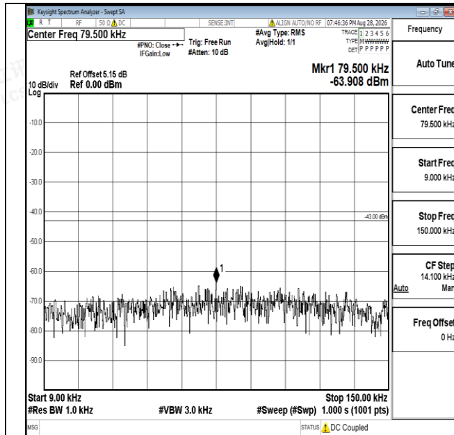
Band25-20MHz-QPSK-26140-1RB#0-0.009~0.15-PASS
