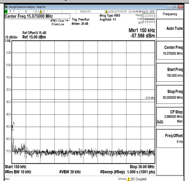
Band25-15MHz-QPSK-26615-1RB#0-0.15~30-PASS
