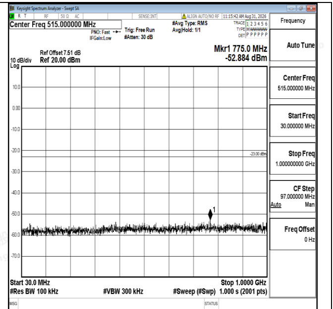
Band25-15MHz-16QAM-26615-1RB#0-30~1000-PASS
