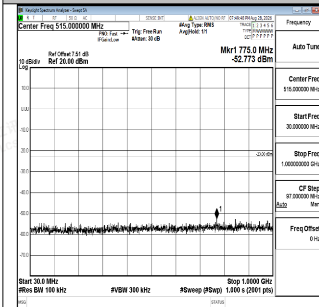
Band25-20MHz-QPSK-26590-1RB#0-30~1000-PASS
