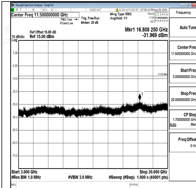
Band25-20MHz-QPSK-26590-1RB#0-3000~20000-PASS
