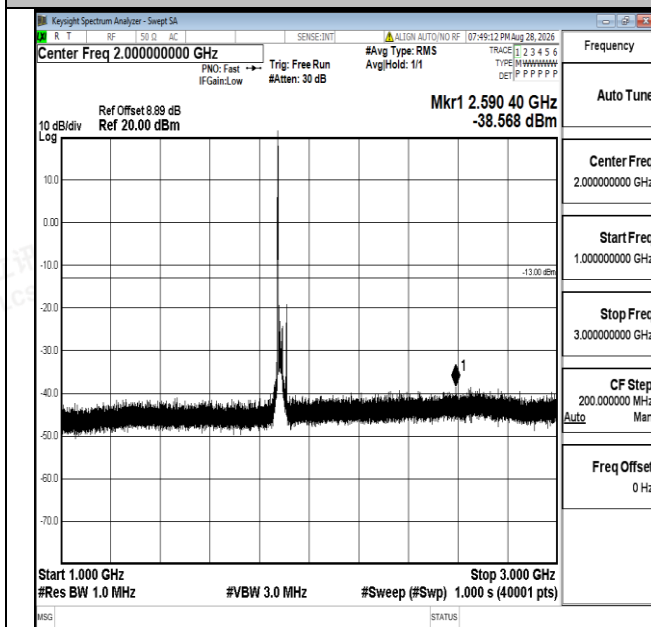
Band25-20MHz-16QAM-26365-1RB#0-1000~3000-PASS
