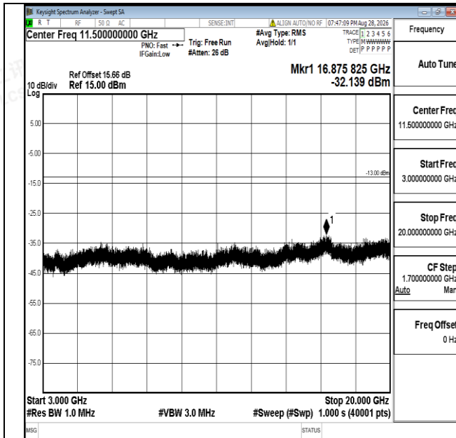
Band25-20MHz-QPSK-26140-1RB#0-3000~20000-PASS
