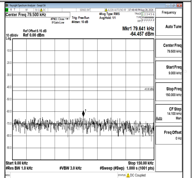
Band25-20MHz-16QAM-26365-1RB#0-0.009~0.15-PASS
