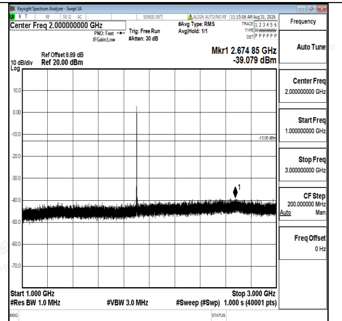
Band25-15MHz-QPSK-26615-1RB#0-1000~3000-PASS
