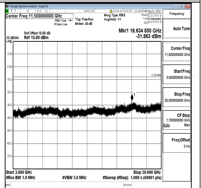
Band25-15MHz-16QAM-26615-1RB#0-3000~20000-PASS
