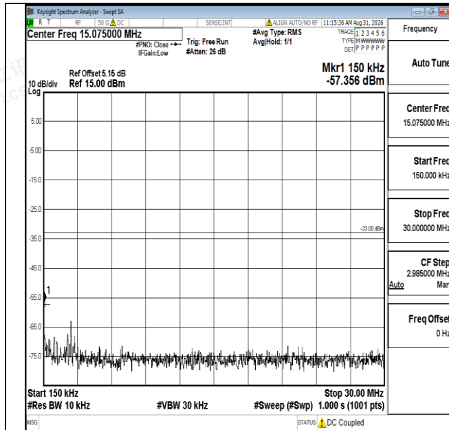
Band25-15MHz-16QAM-26615-1RB#0-0.15~30-PASS
