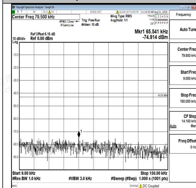
Band25-15MHz-QPSK-26615-1RB#0-0.009~0.15-PASS
