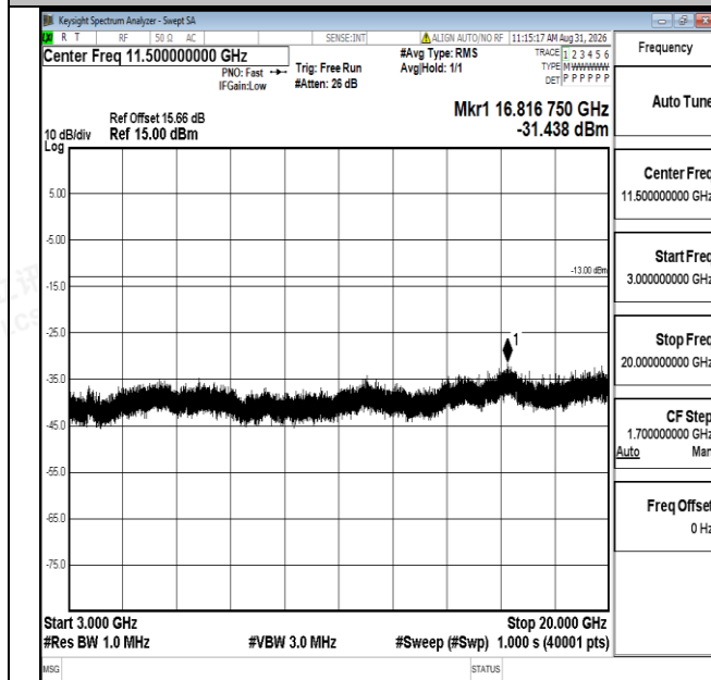
Band25-15MHz-QPSK-26615-1RB#0-3000~20000-PASS
