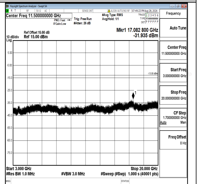
Band25-20MHz-16QAM-26365-1RB#0-3000~20000-PASS
