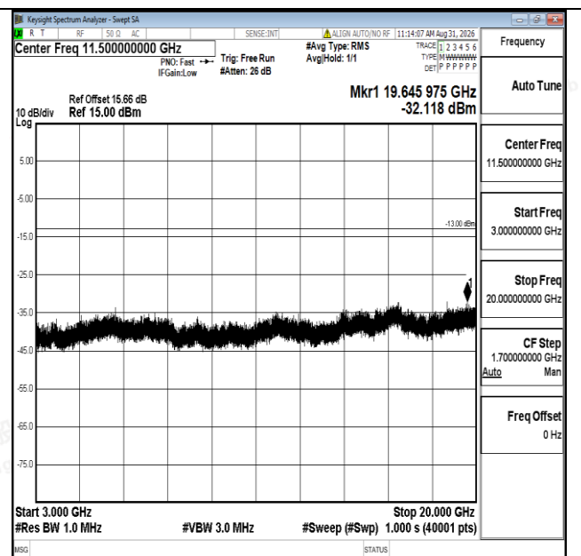
Band25-15MHz-16QAM-26365-1RB#0-3000~20000-PASS
