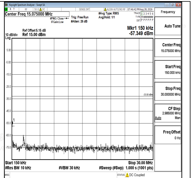
Band25-20MHz-QPSK-26140-1RB#0-0.15~30-PASS
