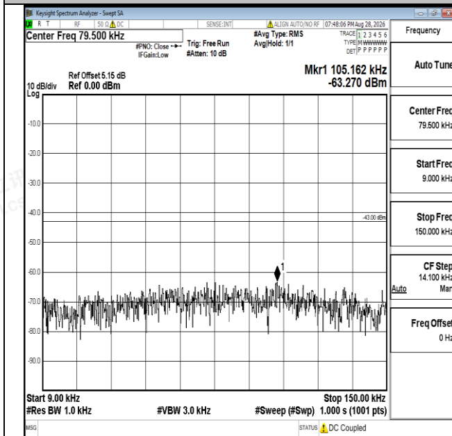
Band25-20MHz-QPSK-26365-1RB#0-0.009-0.15-PASS
