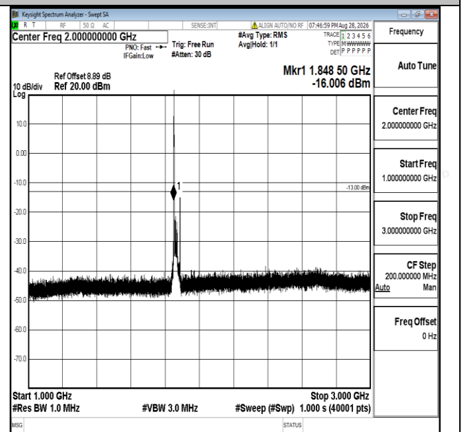
Band25-20MHz-QPSK-26140-1RB#0-1000~3000-PASS
