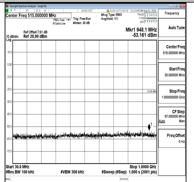
Band25-15MHz-16QAM-26365-1RB#0-30~1000-PASS
