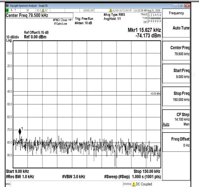
Band25-15MHz-16QAM-26615-1RB#0-0.009~0.15-PASS
