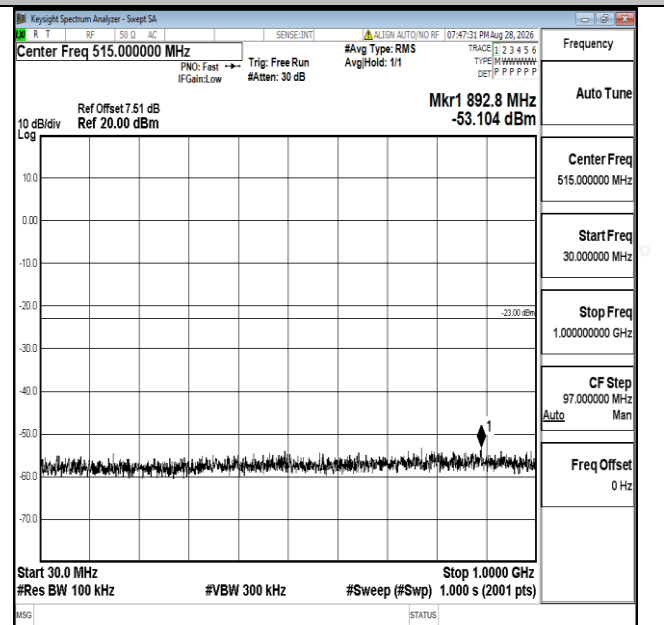
Band25-20MHz-16QAM-26140-1RB#0-30~1000-PASS
