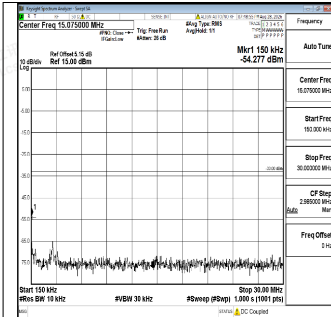
Band25-20MHz-16QAM-26365-1RB#0-0.15~30-PASS
