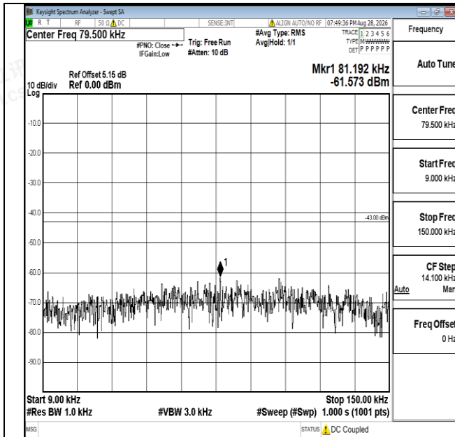
Band25-20MHz-QPSK-26590-1RB#0-0.009~0.15-PASS
