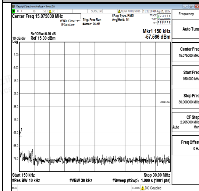
Band25-15MHz-16QAM-26365-1RB#0-0.15~30-PASS
