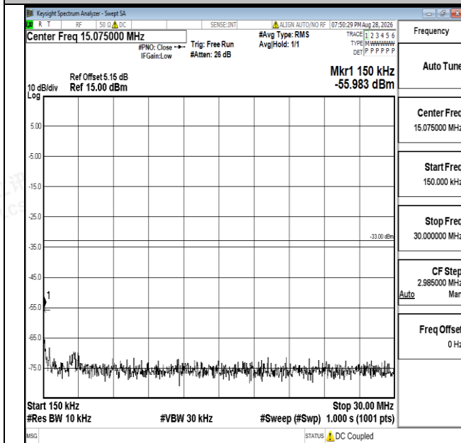
Band25-20MHz-16QAM-26590-1RB#0-0.15~30-PASS
