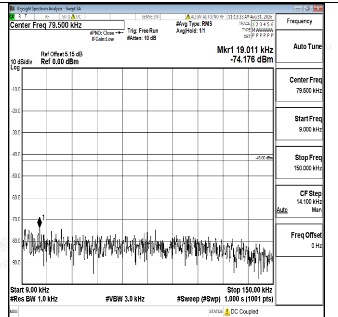
Band25-15MHz-16QAM-26365-1RB#0-0.009~0.15-PASS
