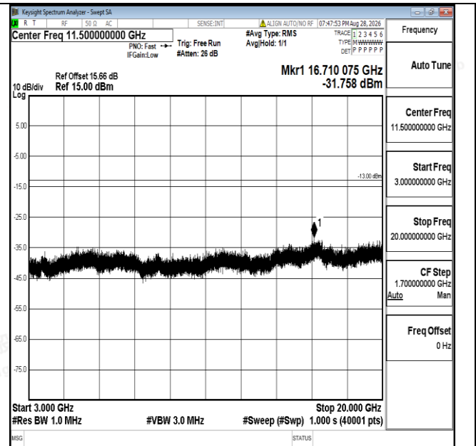
Band25-20MHz-16QAM-26140-1RB#0-3000-20000-PASS
