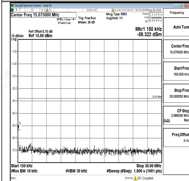
Band25-20MHz-16QAM-26140-1RB#0-0.15~30-PASS
