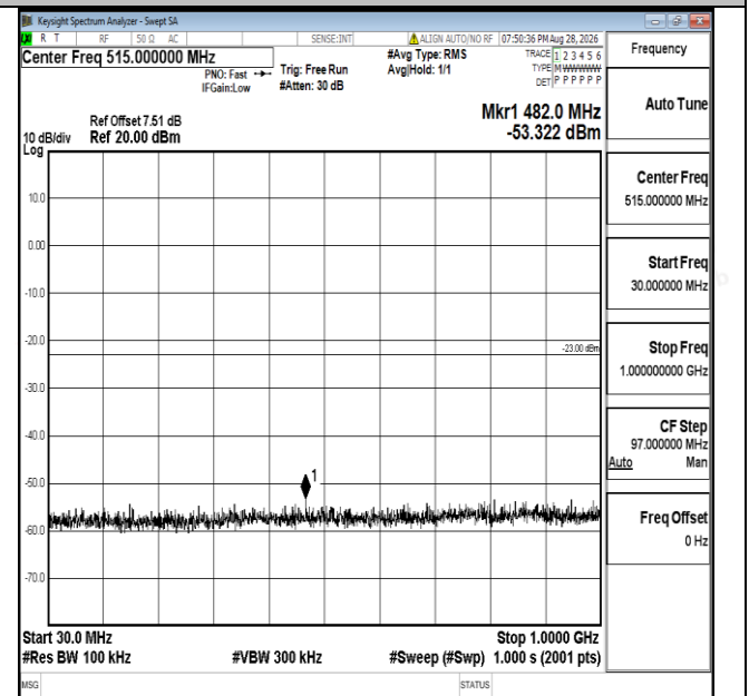
Band25-20MHz-16QAM-26590-1RB#0-30~1000-PASS
