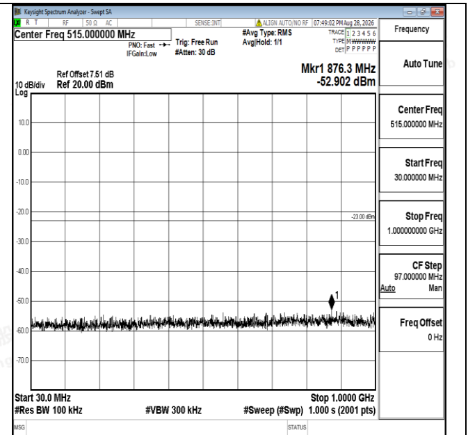
Band25-20MHz-16QAM-26365-1RB#0-30~1000-PASS
