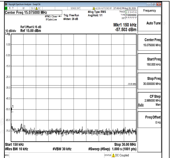
Band25-20MHz-QPSK-26590-1RB#0-0.15~30-PASS
