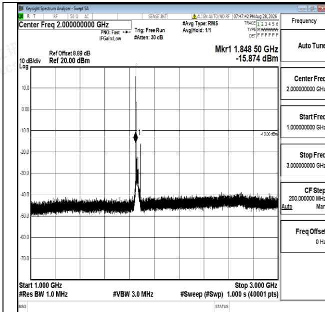
Band25-20MHz-16QAM-26140-1RB#0-1000-3000-PASS
