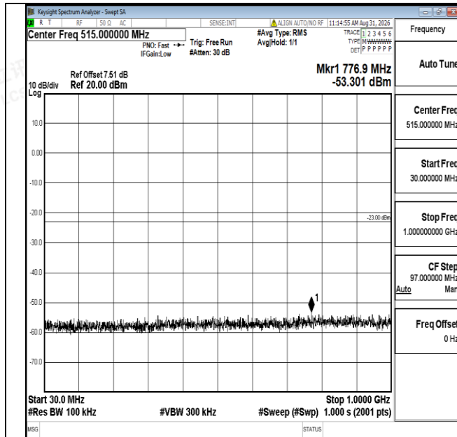
Band25-15MHz-QPSK-26615-1RB#0-30~1000-PASS
