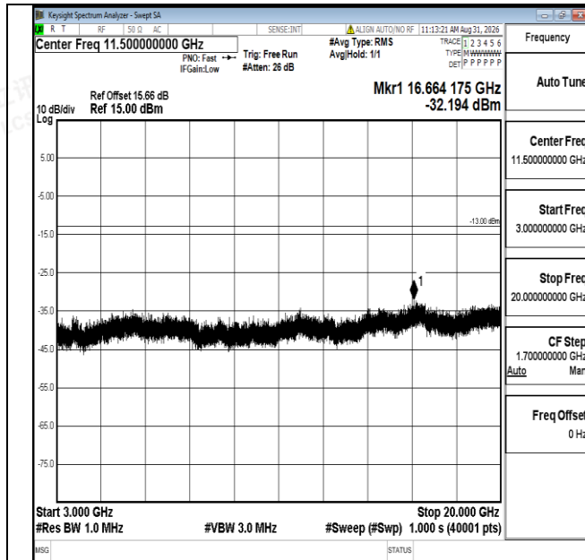
Band25-15MHz-QPSK-26365-1RB#0-3000~20000-PASS
