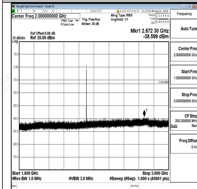
Band25-15MHz-16QAM-26615-1RB#0-1000~3000-PASS
