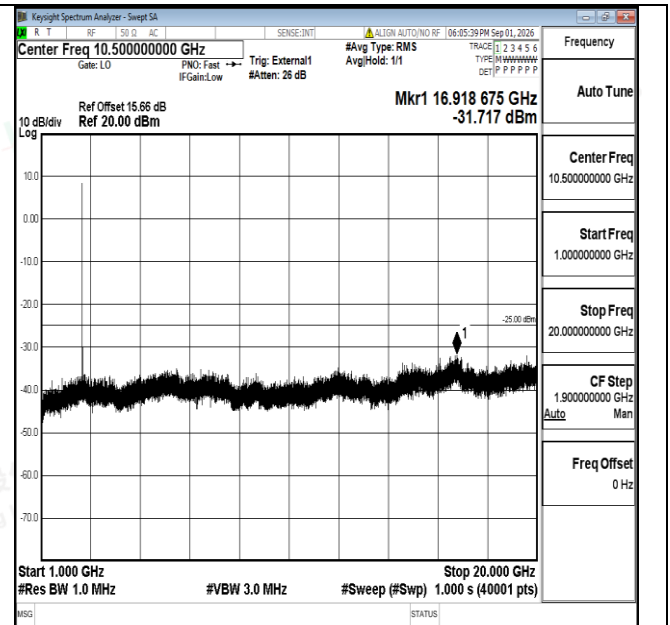
Band38-10MHz-QPSK-37800-1RB#0-1000~20000-PASS
