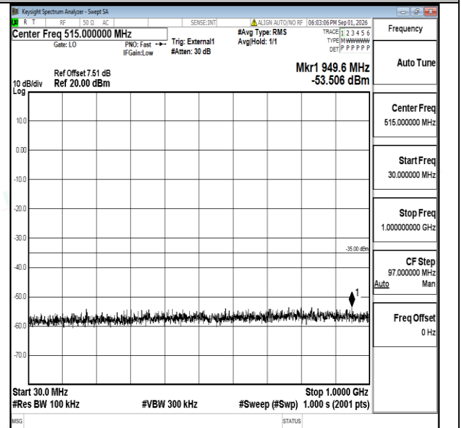
Band38-5MHz-16QAM-38225-1RB#0-30~1000-PASS
