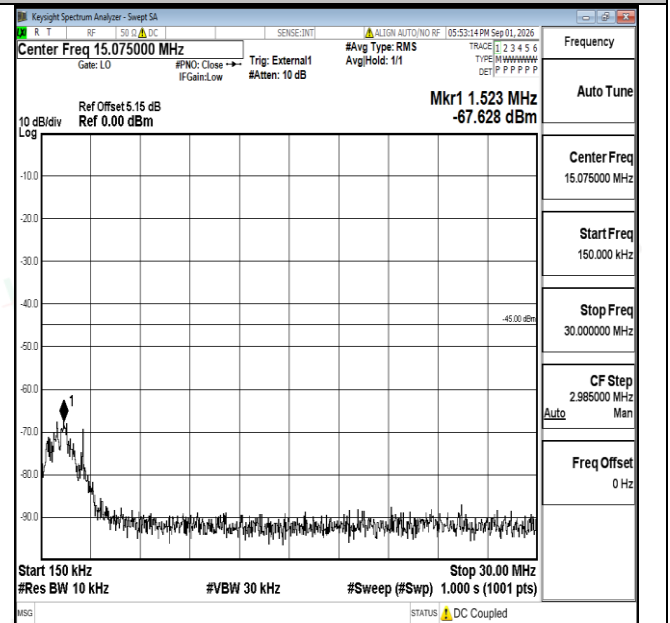
Band38-5MHz-QPSK-38000-1RB#0-0.15~30-PASS
