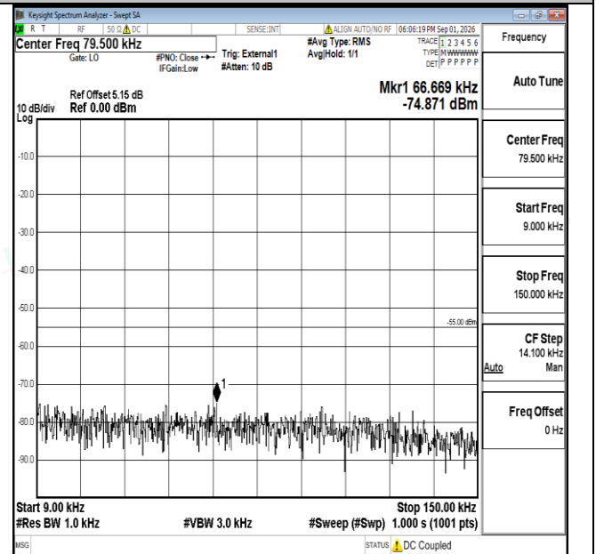
Band38-10MHz-16QAM-37800-1RB#0-0.009~0.15-PASS
