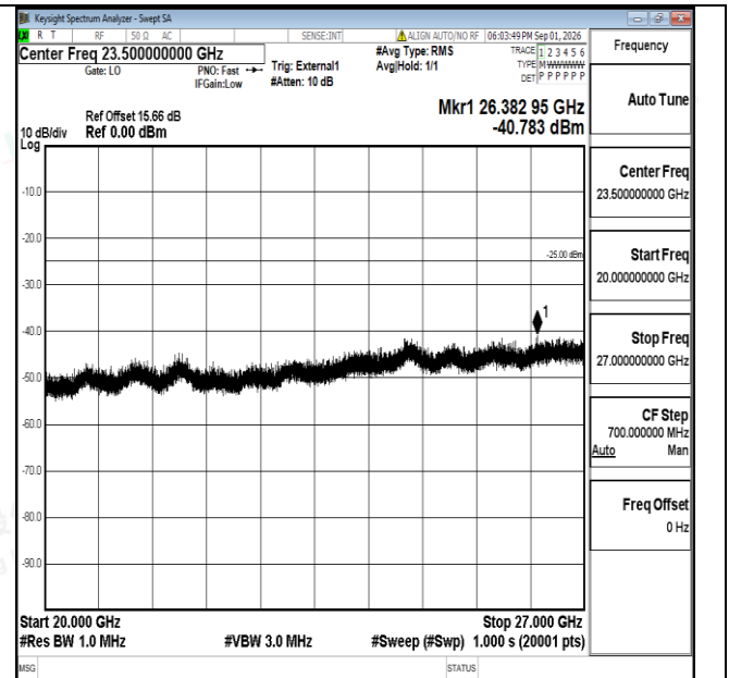
Band38-5MHz-16QAM-38225-1RB#0-20000~27000-PASS
