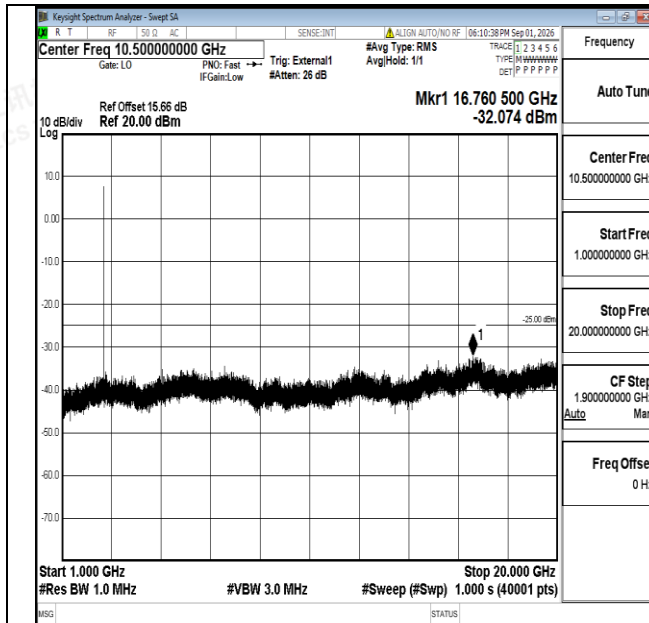
Band38-10MHz-16QAM-38000-1RB#0-1000~20000-PASS
