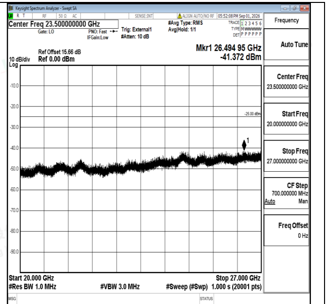
Band38-5MHz-16QAM-37775-1RB#0-20000~27000-PASS
