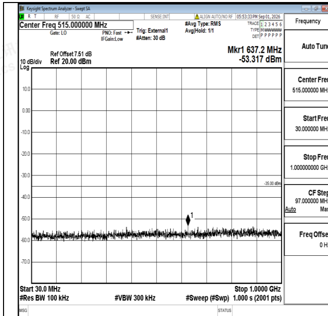
Band38-5MHz-QPSK-38000-1RB#0-30~1000-PASS
