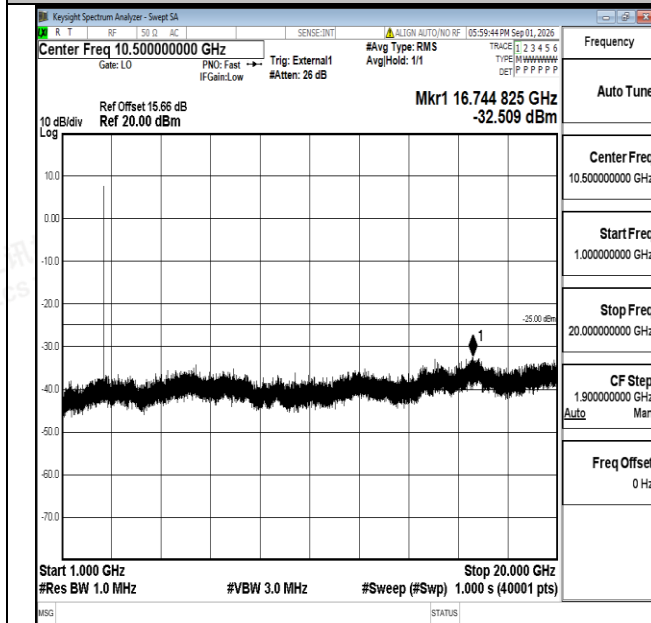
Band38-5MHz-16QAM-38000-1RB#0-1000~20000-PASS
