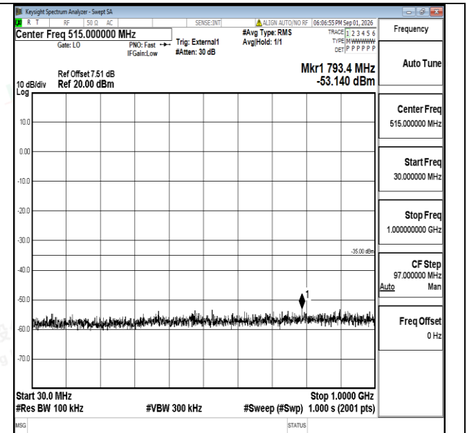
Band38-10MHz-16QAM-37800-1RB#0-30~1000-PASS
