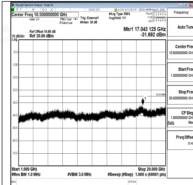
Band38-5MHz-16QAM-37775-1RB#0-1000~20000-PASS
