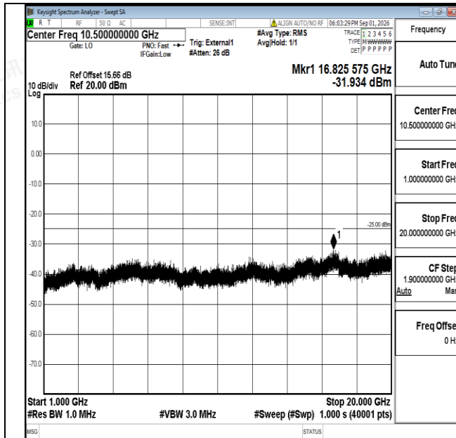
Band38-5MHz-16QAM-38225-1RB#0-1000~20000-PASS
