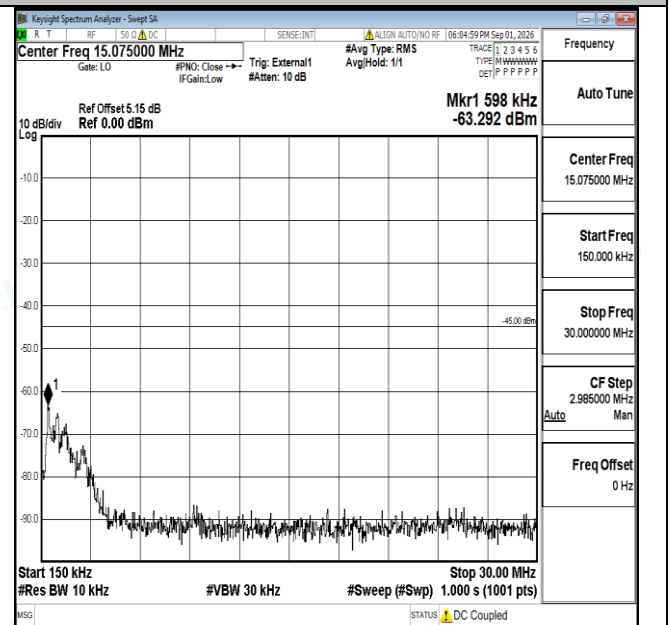
Band38-10MHz-QPSK-37800-1RB#0-0.15~30-PASS
