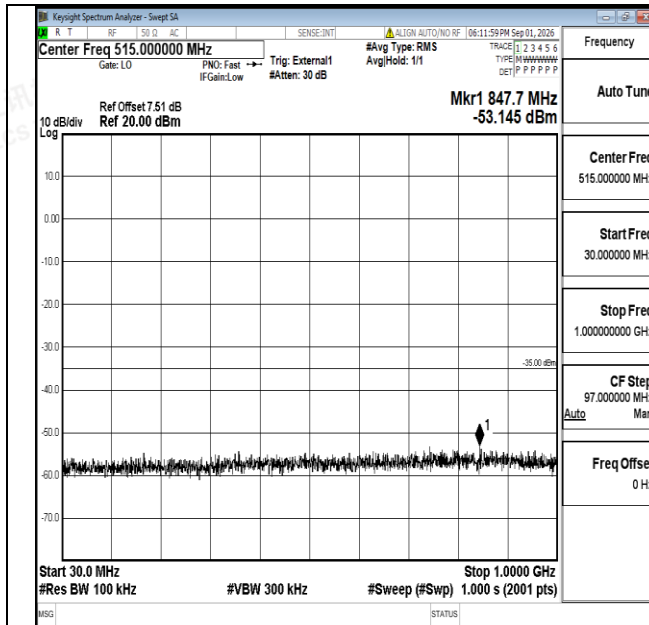
Band38-10MHz-QPSK-38200-1RB#0-30~1000-PASS
