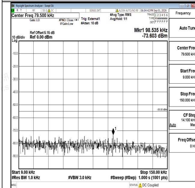
Band38-10MHz-QPSK-37800-1RB#0-0.009~0.15-PASS
