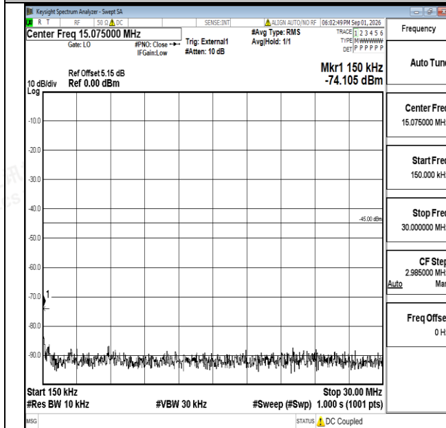
Band38-5MHz-16QAM-38225-1RB#0-0.15~30-PASS
