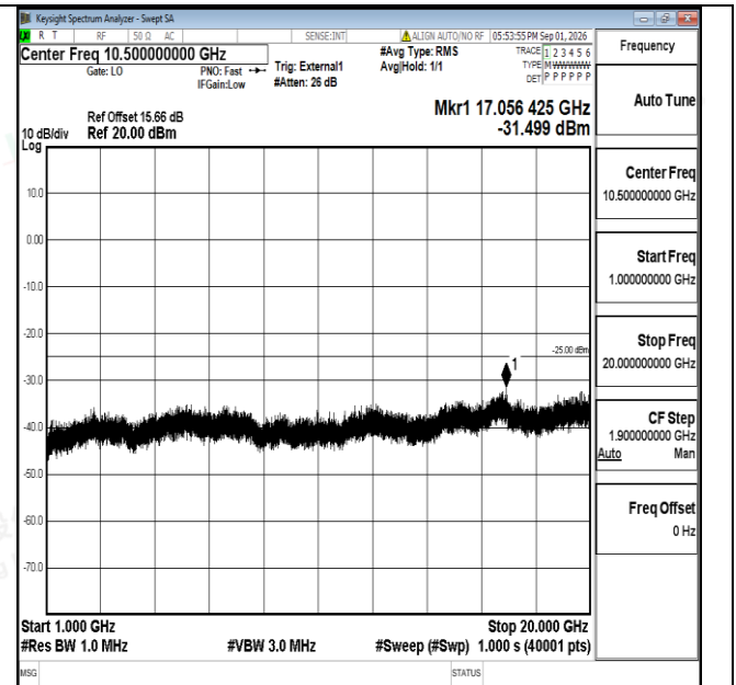
Band38-5MHz-QPSK-38000-1RB#0-1000~20000-PASS
