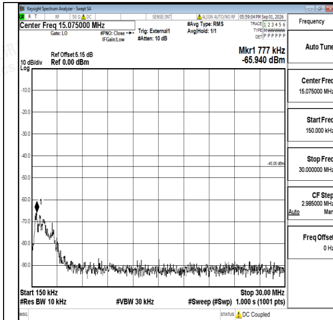
Band38-5MHz-16QAM-38000-1RB#0-0.15~30-PASS
