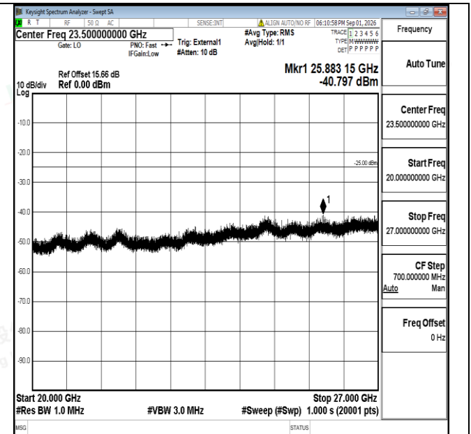
Band38-10MHz-16QAM-38000-1RB#0-20000~27000-PASS
