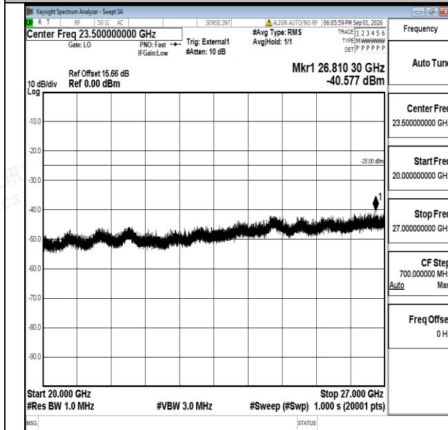
Band38-10MHz-QPSK-37800-1RB#0-20000~27000-PASS
