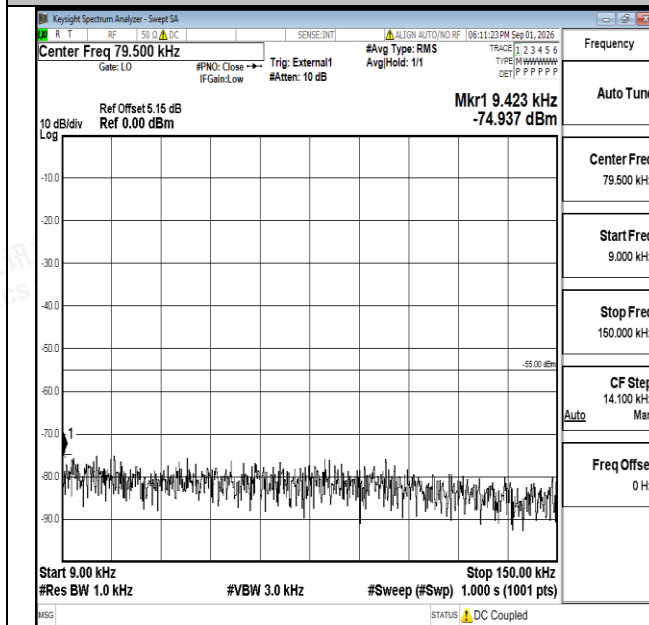
Band38-10MHz-QPSK-38200-1RB#0-0.009~0.15-PASS
