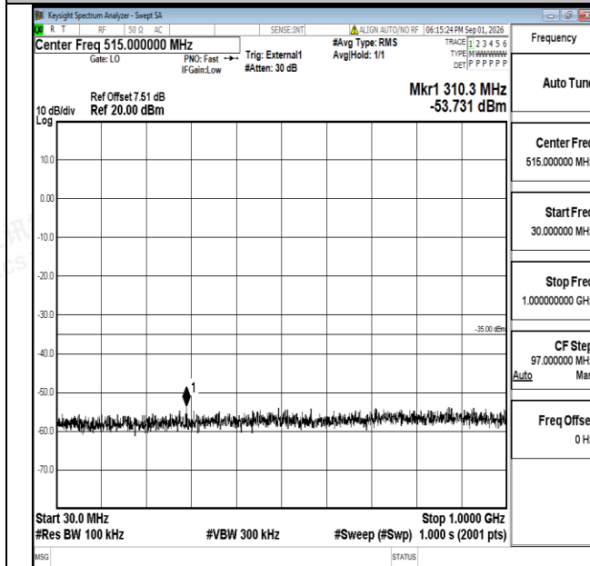
Band38-15MHz-QPSK-37825-1RB#0-30~1000-PASS
