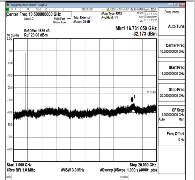
Band38-10MHz-QPSK-38000-1RB#0-1000~20000-PASS
