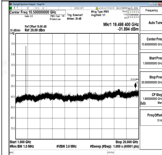
Band38-10MHz-16QAM-38200-1RB#0-1000~20000-PASS
