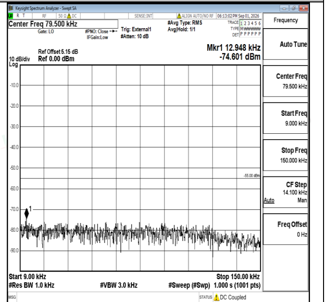
Band38-10MHz-16QAM-38200-1RB#0-0.009~0.15-PASS
