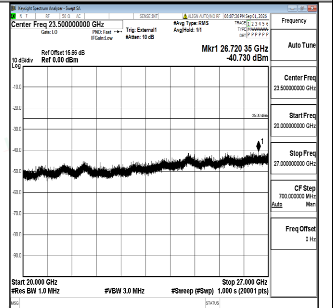
Band38-10MHz-16QAM-37800-1RB#0-20000~27000-PASS
