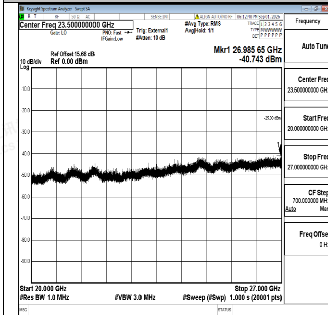
Band38-10MHz-QPSK-38200-1RB#0-20000~27000-PASS
