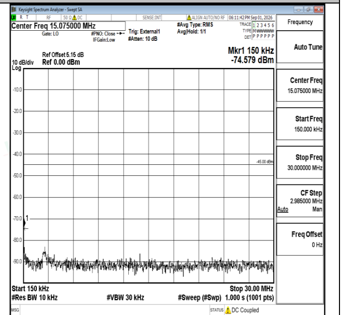
Band38-10MHz-QPSK-38200-1RB#0-0.15~30-PASS
