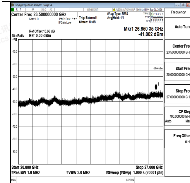
Band38-5MHz-QPSK-38225-1RB#0-20000~27000-PASS
