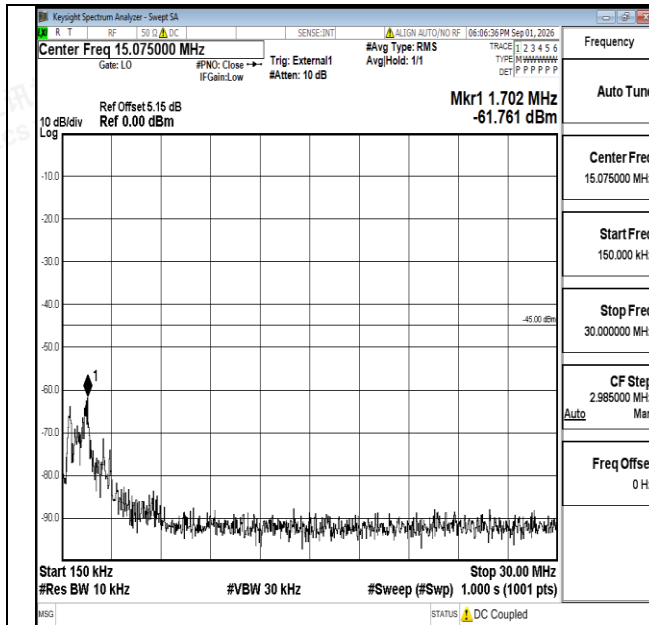
Band38-10MHz-16QAM-37800-1RB#0-0.15~30-PASS
