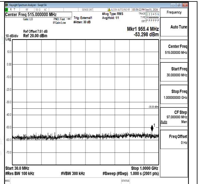
Band38-5MHz-16QAM-38000-1RB#0-30~1000-PASS
