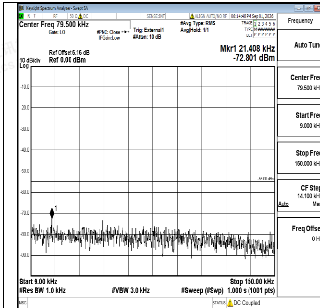
Band38-15MHz-QPSK-37825-1RB#0-0.009~0.15-PASS
