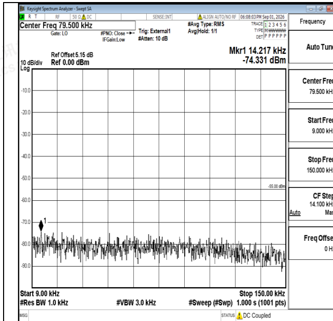
Band38-10MHz-QPSK-38000-1RB#0-0.009~0.15-PASS
