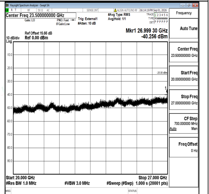
Band38-10MHz-16QAM-38200-1RB#0-20000~27000-PASS
