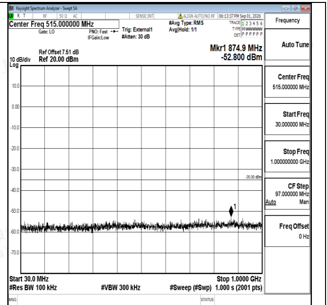
Band38-10MHz-16QAM-38200-1RB#0-30~1000-PASS
