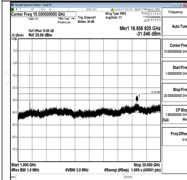
Band38-10MHz-16QAM-37800-1RB#0-1000~20000-PASS
