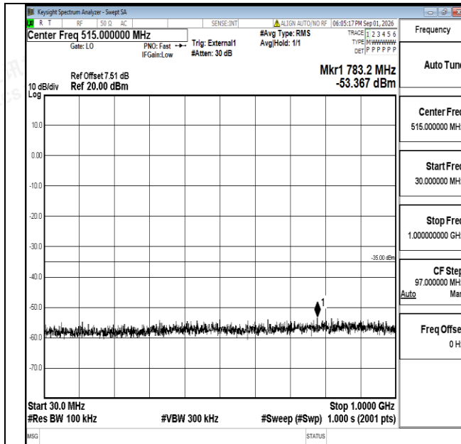
Band38-10MHz-QPSK-37800-1RB#0-30~1000-PASS
