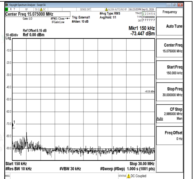
Band38-15MHz-QPSK-37825-1RB#0-0.15~30-PASS
