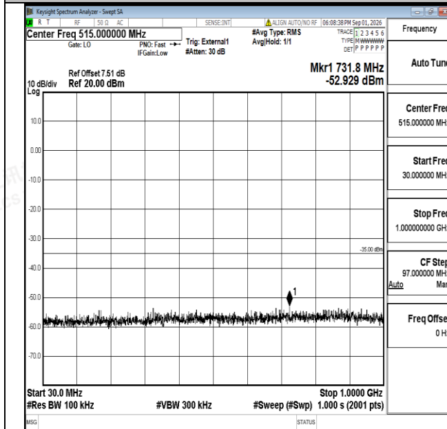
Band38-10MHz-QPSK-38000-1RB#0-30~1000-PASS
