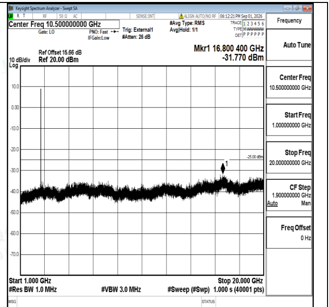
Band38-10MHz-QPSK-38200-1RB#0-1000~20000-PASS
