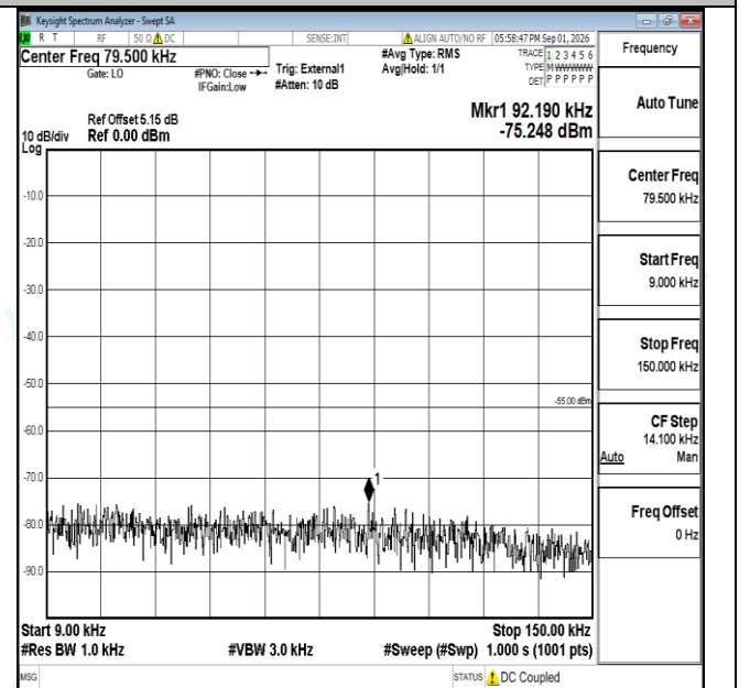
Band38-5MHz-16QAM-38000-1RB#0-0.009~0.15-PASS
