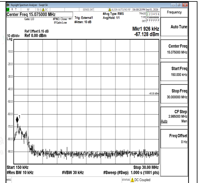
Band38-10MHz-QPSK-38000-1RB#0-0.15~30-PASS
