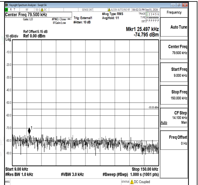
Band38-5MHz-16QAM-38225-1RB#0-0.009~0.15-PASS
