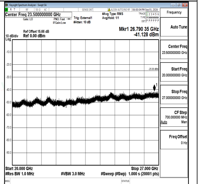
Band38-5MHz-16QAM-38000-1RB#0-20000~27000-PASS
