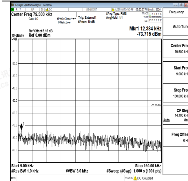
Band38-5MHz-QPSK-38000-1RB#0-0.009~0.15-PASS
