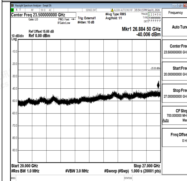
Band38-5MHz-QPSK-38000-1RB#0-20000~27000-PASS
