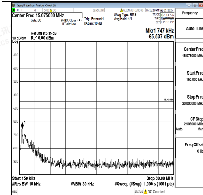
Band38-10MHz-16QAM-38200-1RB#0-0.15~30-PASS
