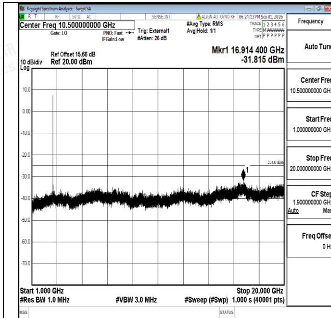
Band38-15MHz-16QAM-38175-1RB#0-1000~20000-PASS
