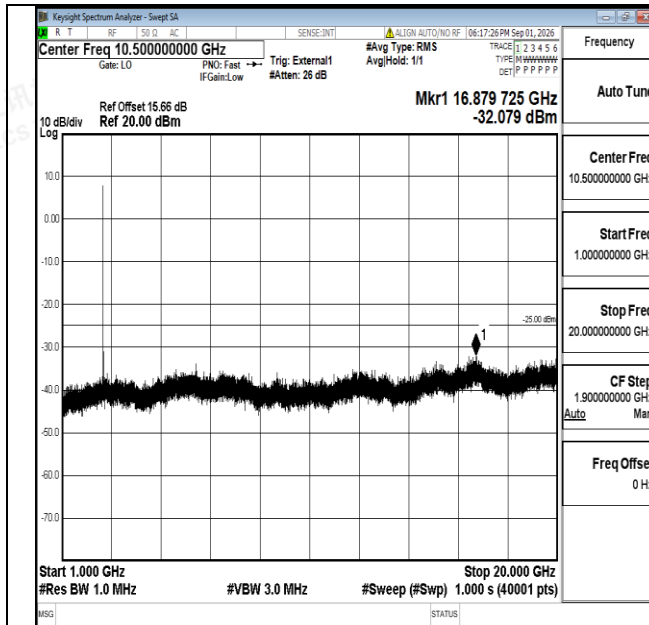
Band38-15MHz-16QAM-37825-1RB#0-1000~20000-PASS
