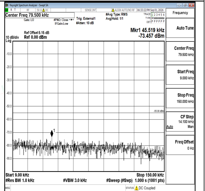
Band38-20MHz-16QAM-38150-1RB#0-0.009~0.15-PASS
