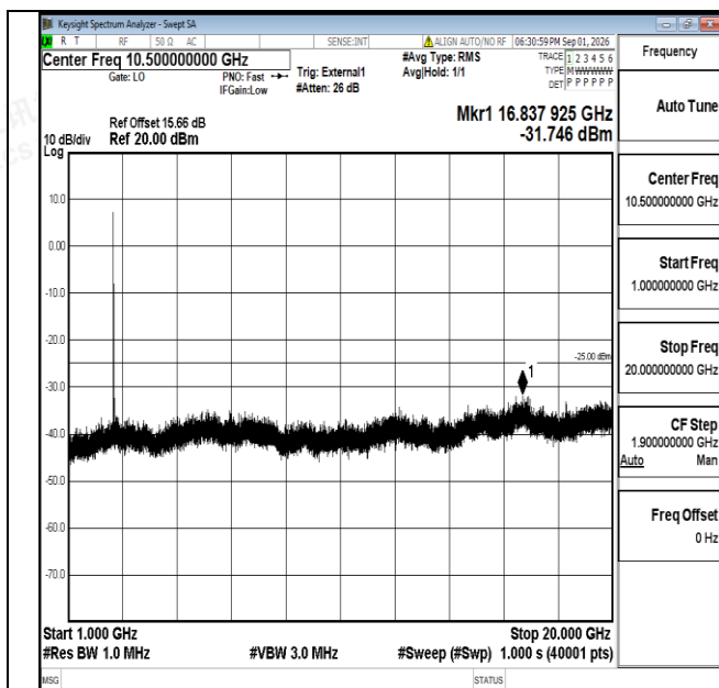
Band38-20MHz-16QAM-38000-1RB#0-1000~20000-PASS
