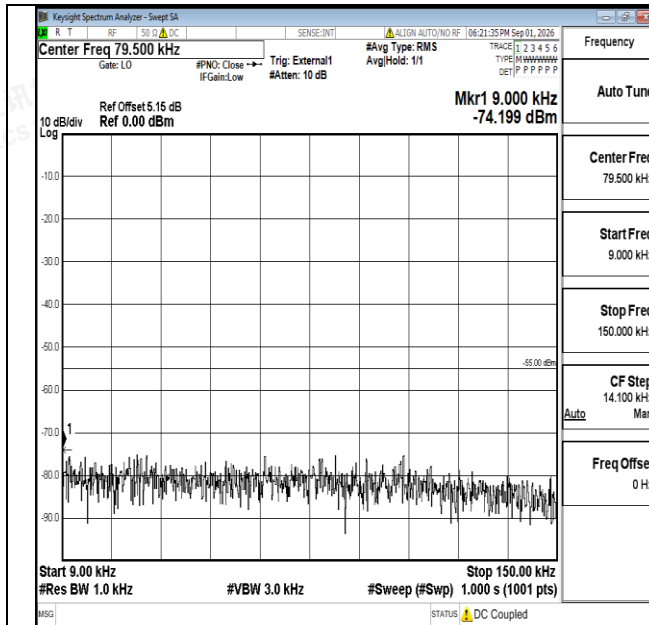
Band38-15MHz-QPSK-38175-1RB#0-0.009~0.15-PASS
