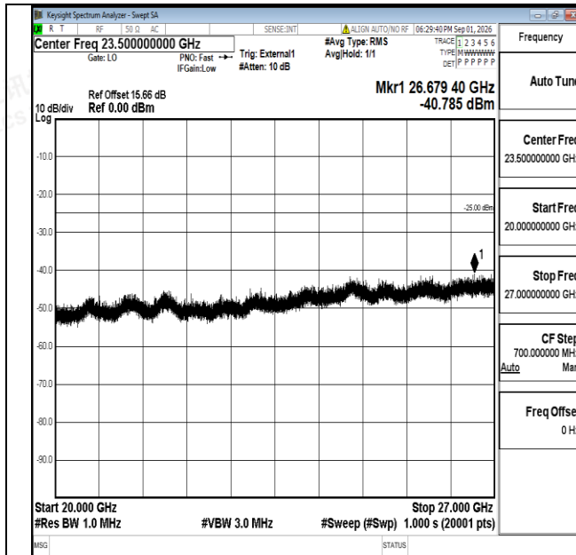
Band38-20MHz-QPSK-38000-1RB#0-20000~27000-PASS
