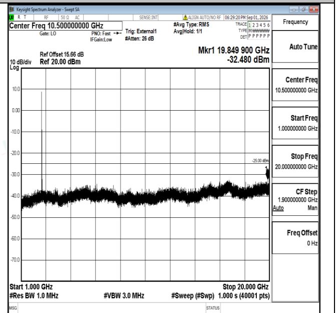
Band38-20MHz-QPSK-38000-1RB#0-1000~20000-PASS
