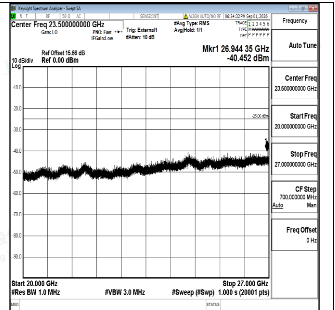
Band38-15MHz-16QAM-38175-1RB#0-20000~27000-PASS
