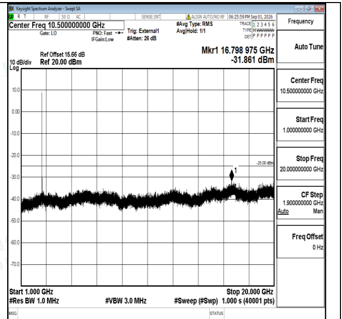
Band38-20MHz-QPSK-37850-1RB#0-1000~20000-PASS
