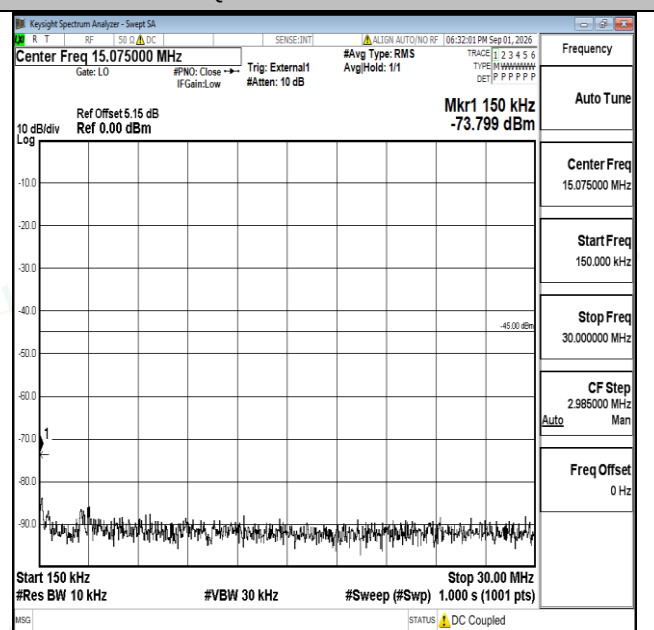
Band38-20MHz-QPSK-38150-1RB#0-0.15~30-PASS
