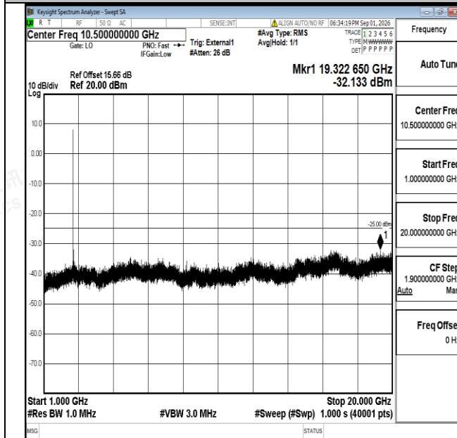
Band38-20MHz-16QAM-38150-1RB#0-1000~20000-PASS
