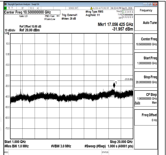
Band38-20MHz-QPSK-38150-1RB#0-1000~20000-PASS
