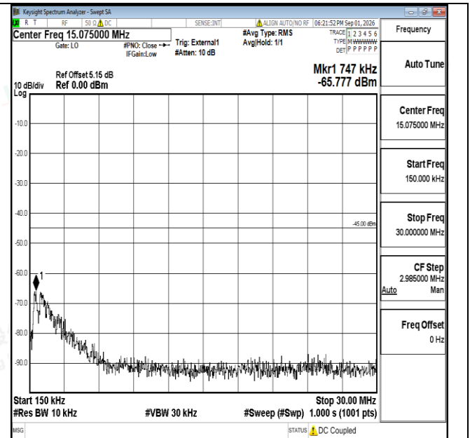
Band38-15MHz-QPSK-38175-1RB#0-0.15~30-PASS
