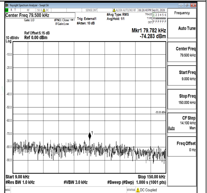
Band38-20MHz-16QAM-37850-1RB#0-0.009~0.15-PASS
