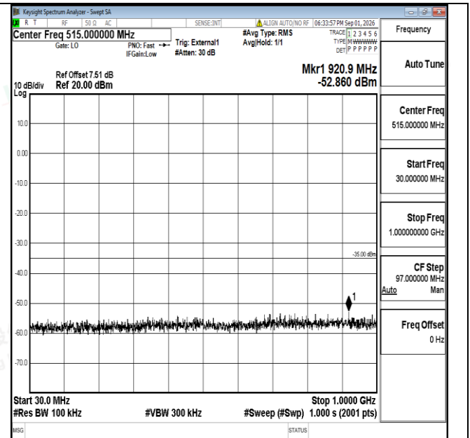
Band38-20MHz-16QAM-38150-1RB#0-30~1000-PASS
