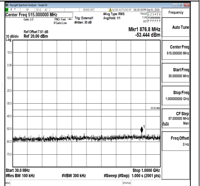
Band38-20MHz-16QAM-38000-1RB#0-30~1000-PASS
