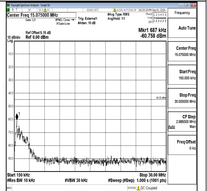
Band38-20MHz-QPSK-37850-1RB#0-0.15~30-PASS
