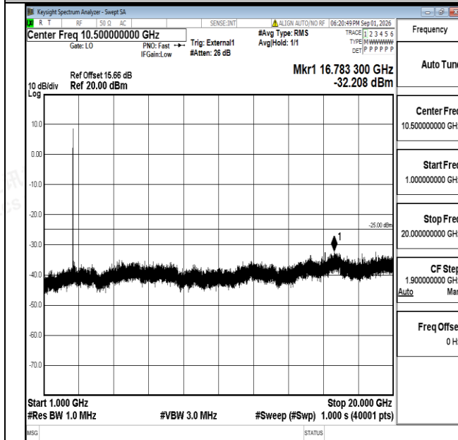
Band38-15MHz-16QAM-38000-1RB#0-1000~20000-PASS
