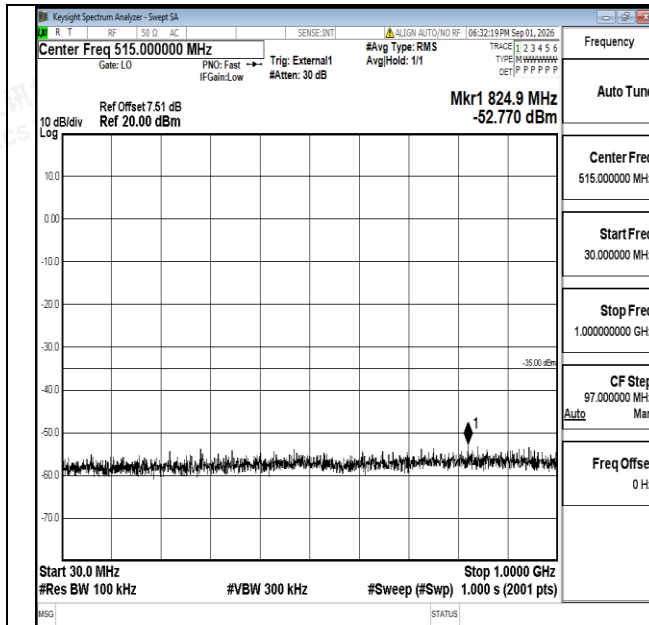
Band38-20MHz-QPSK-38150-1RB#0-30~1000-PASS
