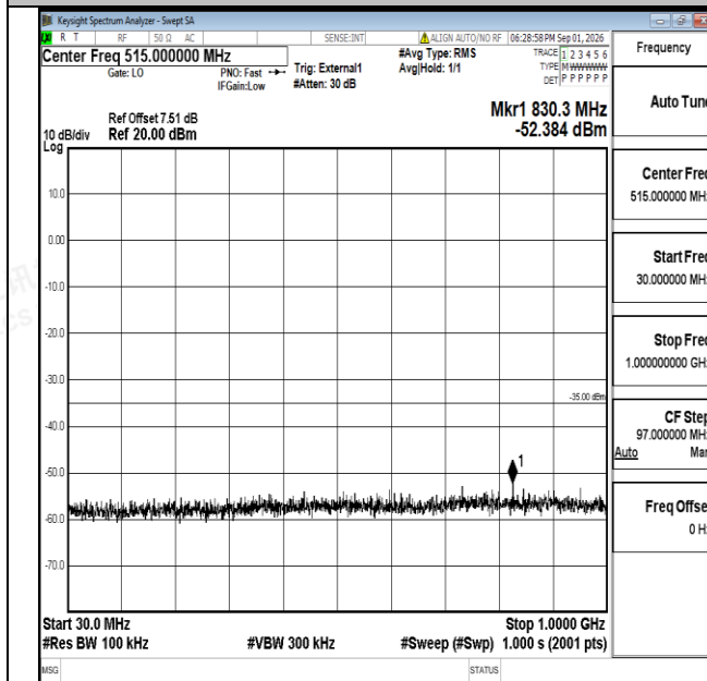
Band38-20MHz-QPSK-38000-1RB#0-30~1000-PASS
