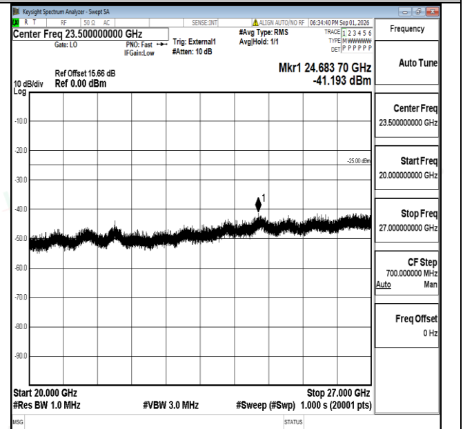
Band38-20MHz-16QAM-38150-1RB#0-20000~27000-PASS
