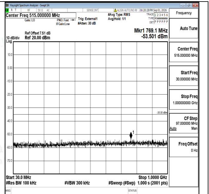
Band38-15MHz-16QAM-38000-1RB#0-30~1000-PASS
