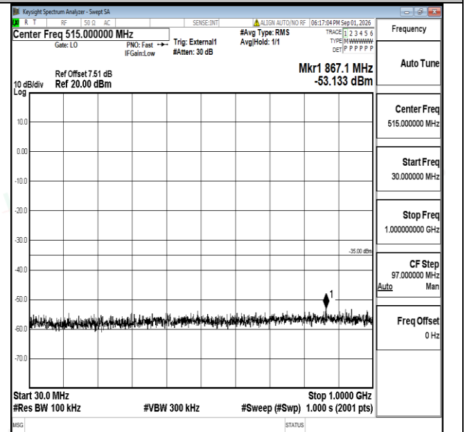
Band38-15MHz-16QAM-37825-1RB#0-30~1000-PASS
