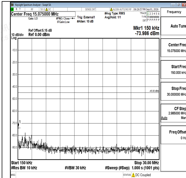
Band38-20MHz-16QAM-37850-1RB#0-0.15~30-PASS
