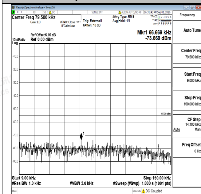
Band38-20MHz-QPSK-38150-1RB#0-0.009~0.15-PASS
