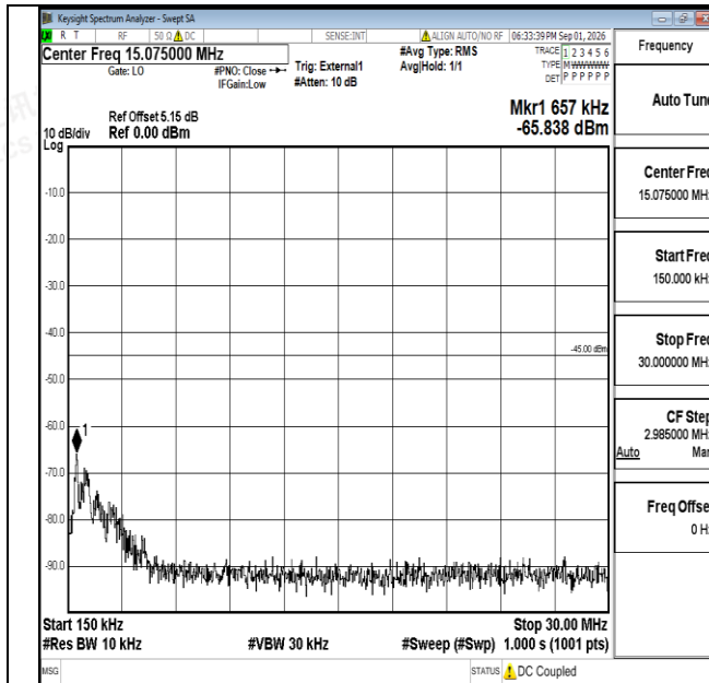
Band38-20MHz-16QAM-38150-1RB#0-0.15~30-PASS
