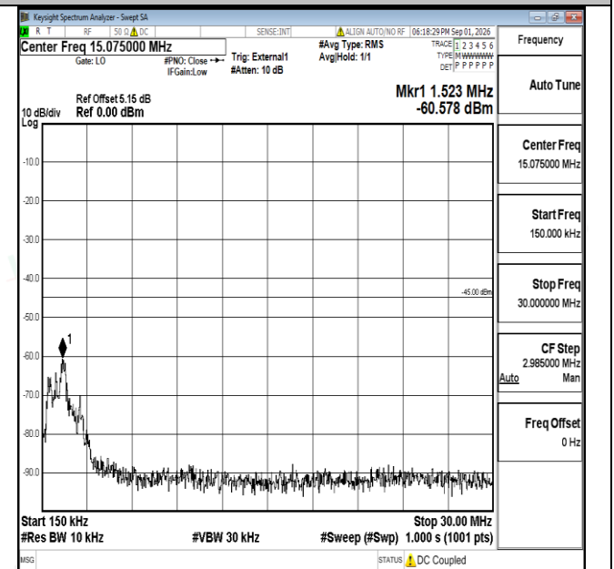
Band38-15MHz-QPSK-38000-1RB#0-0.15~30-PASS
