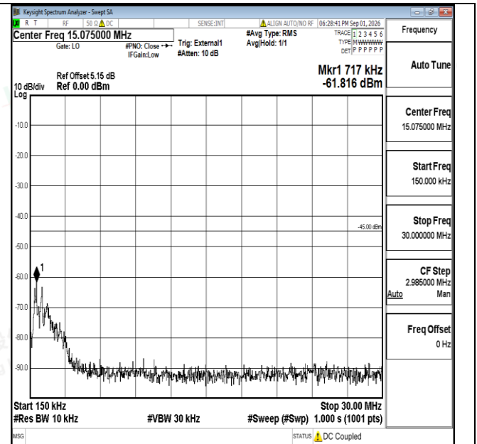
Band38-20MHz-QPSK-38000-1RB#0-0.15~30-PASS
