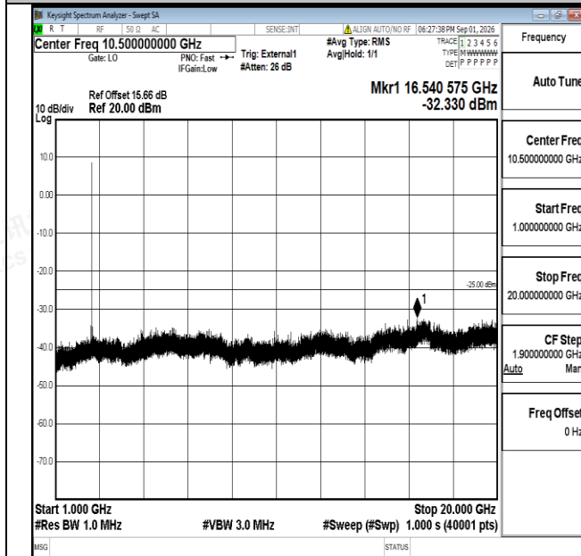
Band38-20MHz-16QAM-37850-1RB#0-1000~20000-PASS
