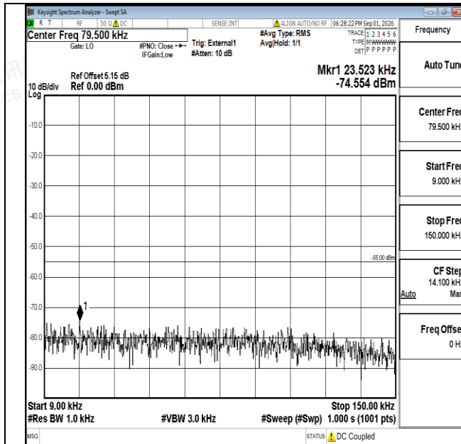
Band38-20MHz-QPSK-38000-1RB#0-0.009~0.15-PASS
