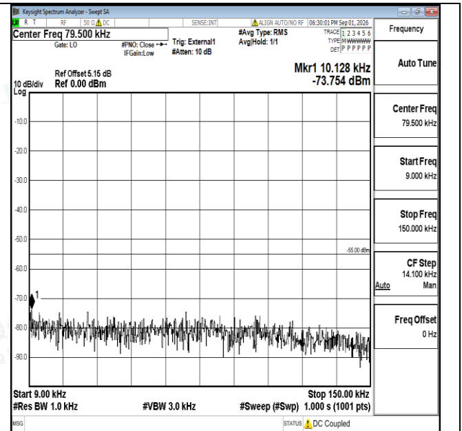
Band38-20MHz-16QAM-38000-1RB#0-0.009~0.15-PASS
