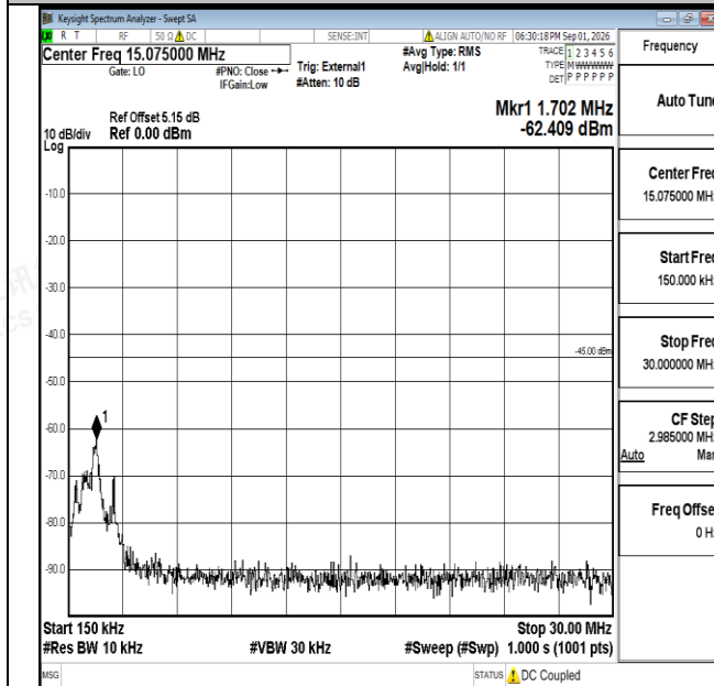
Band38-20MHz-16QAM-38000-1RB#0-0.15~30-PASS
