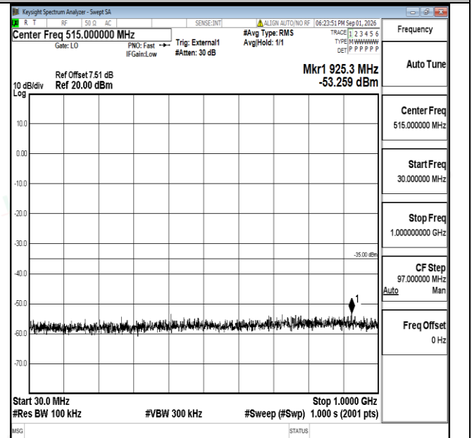
Band38-15MHz-16QAM-38175-1RB#0-30~1000-PASS
