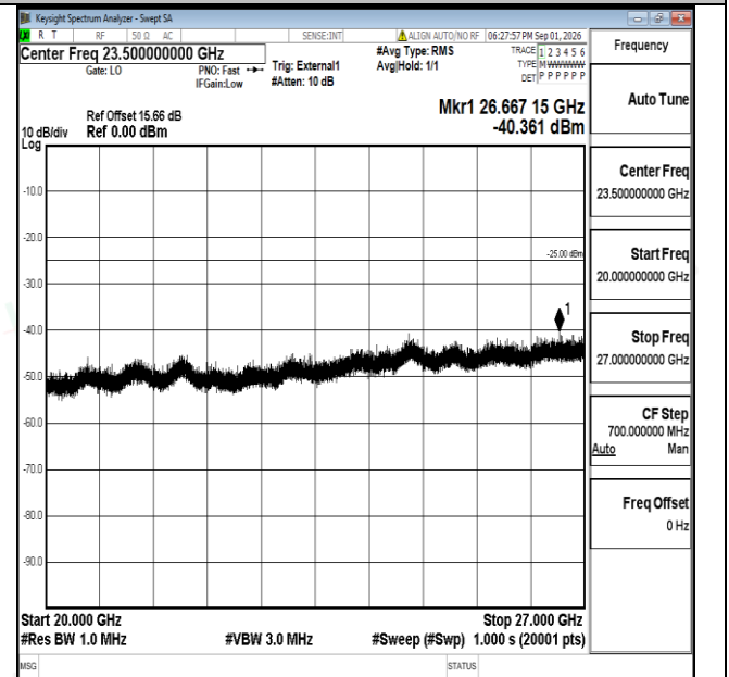
Band38-20MHz-16QAM-37850-1RB#0-20000~27000-PASS
