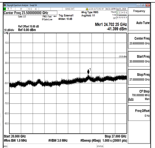
Band38-20MHz-16QAM-38000-1RB#0-20000~27000-PASS
