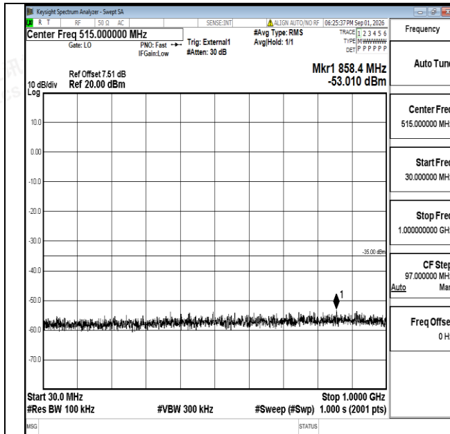
Band38-20MHz-QPSK-37850-1RB#0-30~1000-PASS
