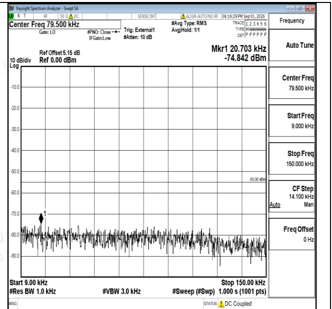
Band38-15MHz-16QAM-37825-1RB#0-0.009~0.15-PASS
