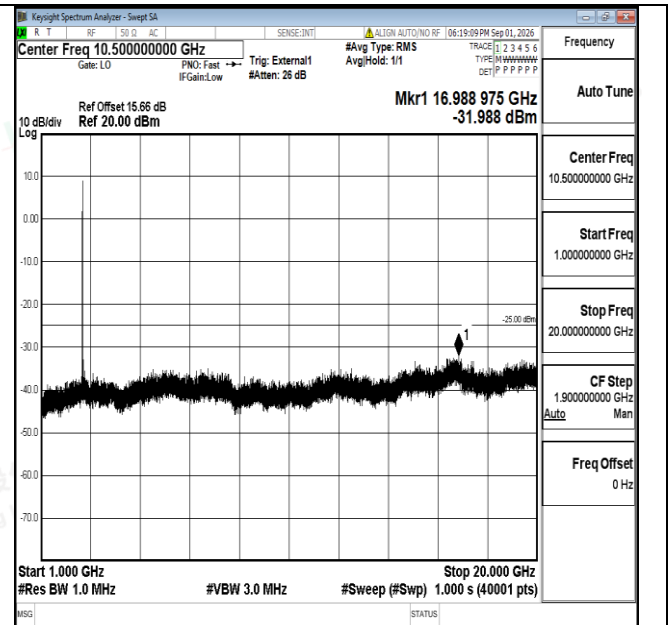
Band38-15MHz-QPSK-38000-1RB#0-1000~20000-PASS
