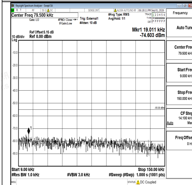
Band38-15MHz-QPSK-38000-1RB#0-0.009~0.15-PASS
