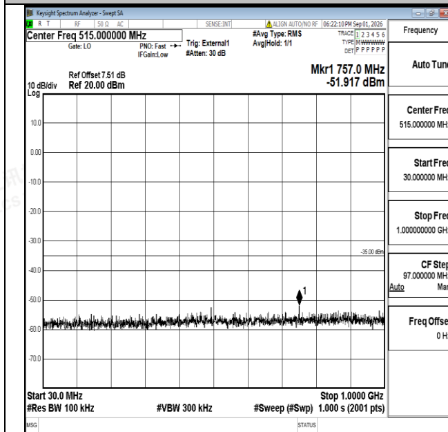
Band38-15MHz-QPSK-38175-1RB#0-30~1000-PASS
