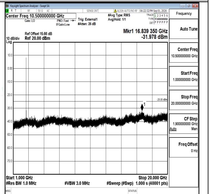
Band38-15MHz-QPSK-38175-1RB#0-1000~20000-PASS
