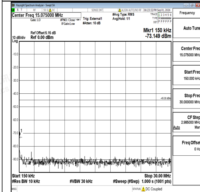
Band38-15MHz-16QAM-38175-1RB#0-0.15~30-PASS
