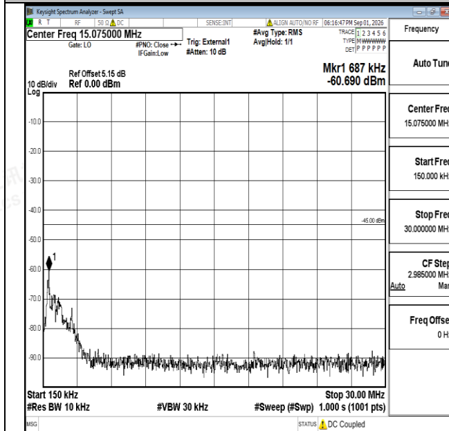
Band38-15MHz-16QAM-37825-1RB#0-0.15~30-PASS
