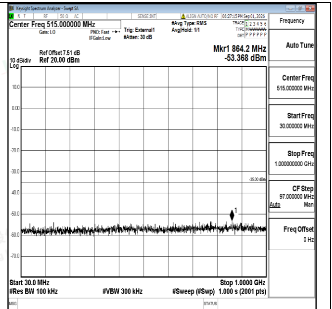
Band38-20MHz-16QAM-37850-1RB#0-30~1000-PASS
