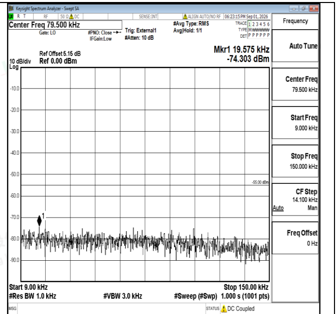
Band38-15MHz-16QAM-38175-1RB#0-0.009~0.15-PASS
