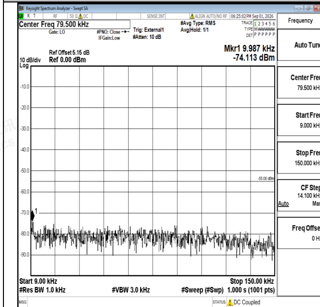
Band38-20MHz-QPSK-37850-1RB#0-0.009~0.15-PASS
