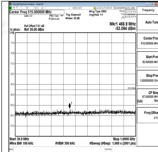
Band38-15MHz-QPSK-38000-1RB#0-30~1000-PASS
