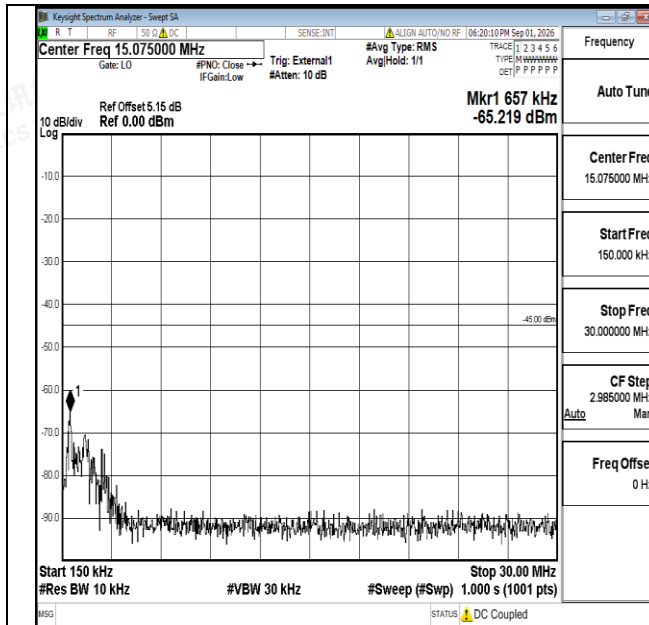
Band38-15MHz-16QAM-38000-1RB#0-0.15~30-PASS
