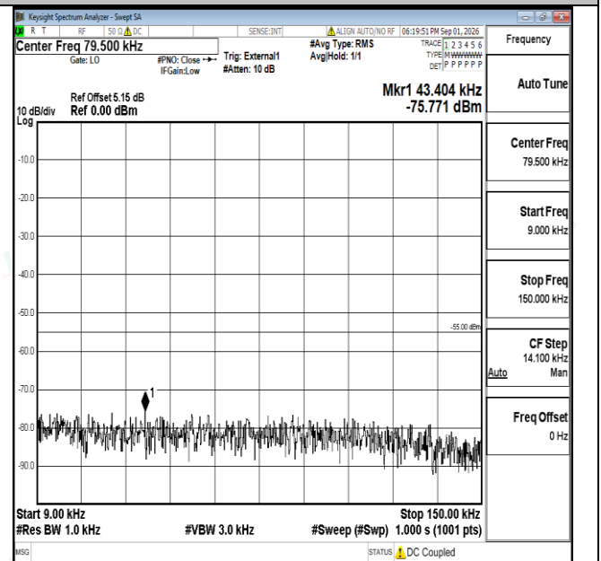
Band38-15MHz-16QAM-38000-1RB#0-0.009~0.15-PASS
