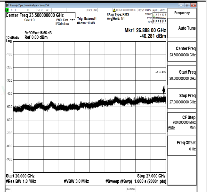
Band38-15MHz-16QAM-38000-1RB#0-20000~27000-PASS
