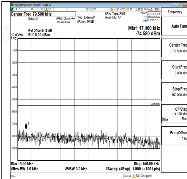
Band41-15MHz-QPSK-39725-1RB#0-0.009~0.15-PASS
