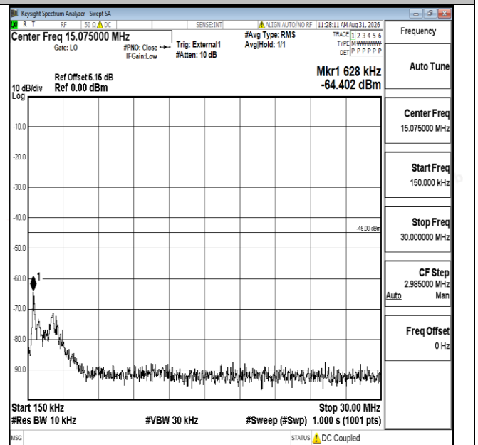
Band41-10MHz-QPSK-39700-1RB#0-0.15~30-PASS
