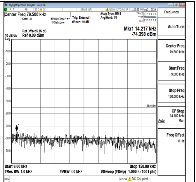
Band41-10MHz-16QAM-40620-1RB#0-0.009~0.15-PASS
