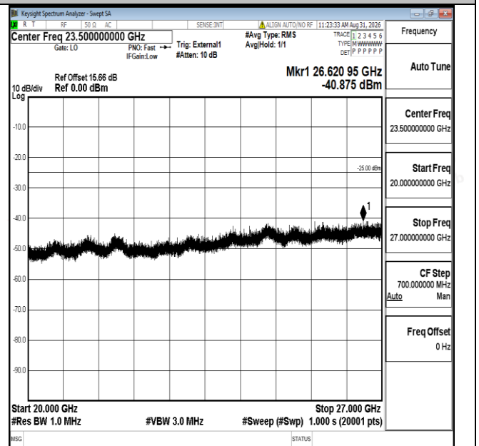
Band41-5MHz-16QAM-40620-1RB#0-20000~27000-PASS
