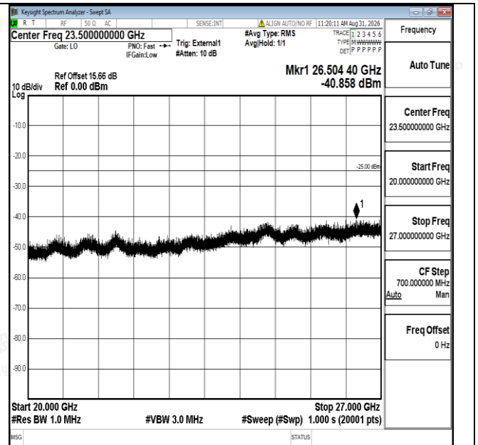
Band41-5MHz-16QAM-39675-1RB#0-20000~27000-PASS
