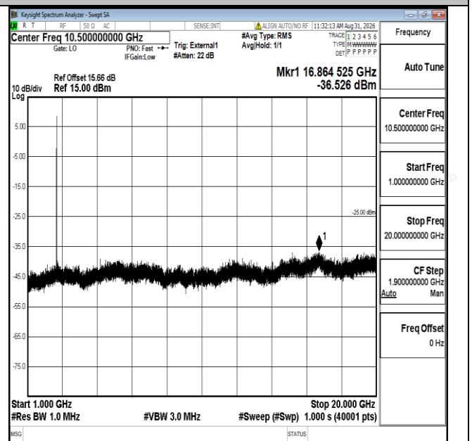
Band41-10MHz-QPSK-40620-1RB#0-1000~20000-PASS
