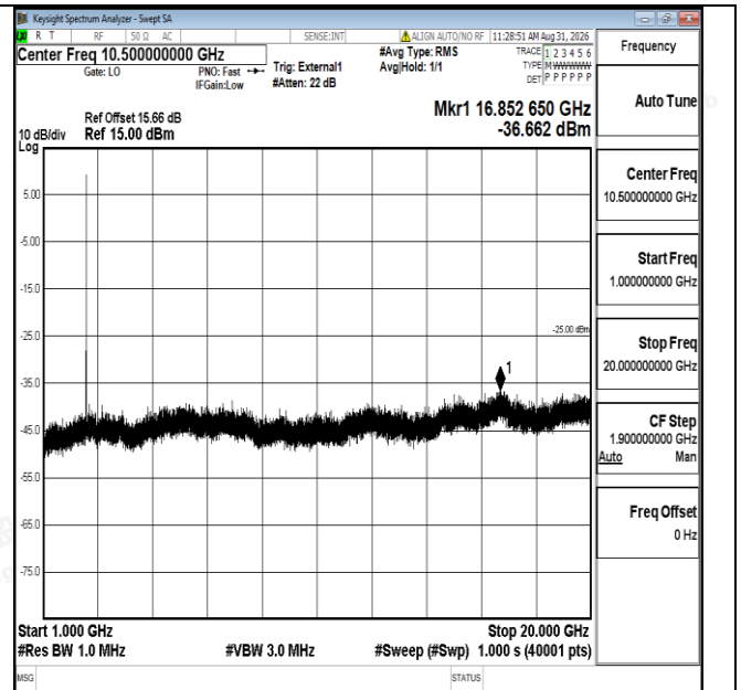
Band41-10MHz-QPSK-39700-1RB#0-1000~20000-PASS
