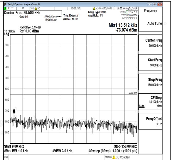
Band41-5MHz-16QAM-39675-1RB#0-0.009~0.15-PASS
