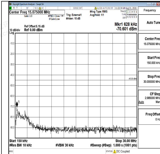
Band41-5MHz-16QAM-40620-1RB#0-0.15~30-PASS
