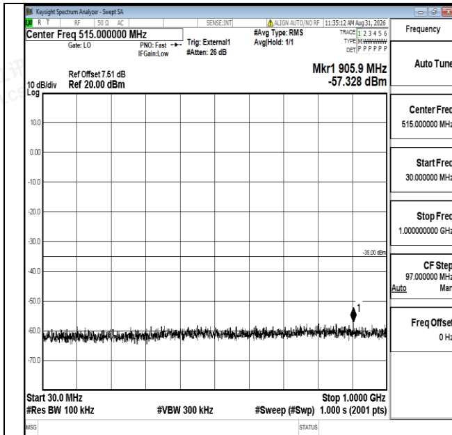
Band41-10MHz-QPSK-41540-1RB#0-30~1000-PASS
