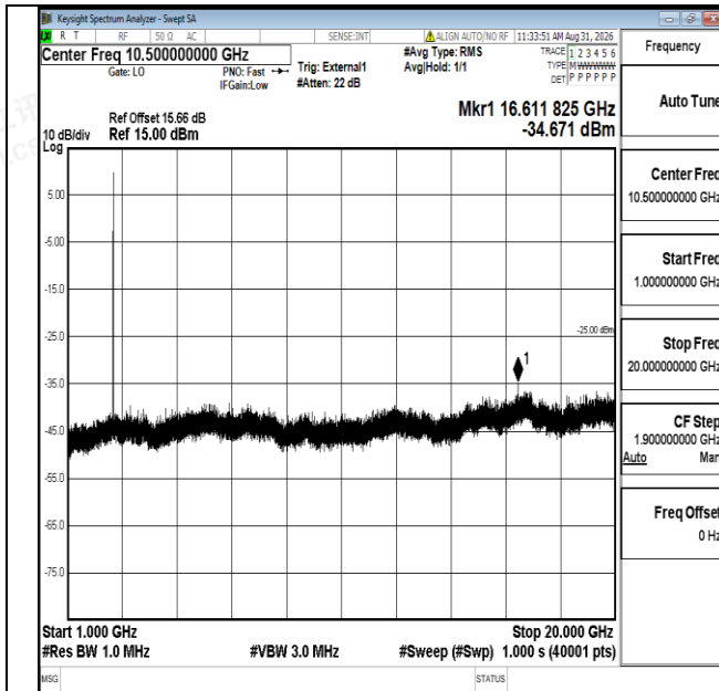
Band41-10MHz-16QAM-40620-1RB#0-1000~20000-PASS
