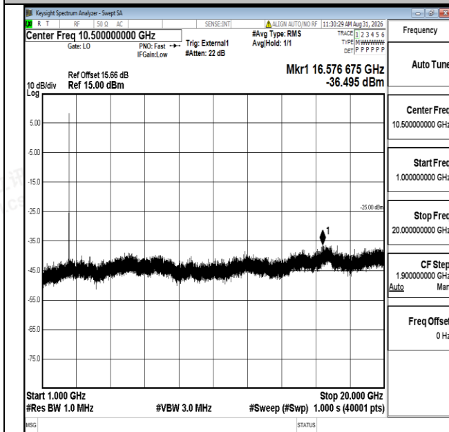
Band41-10MHz-16QAM-39700-1RB#0-1000~20000-PASS
