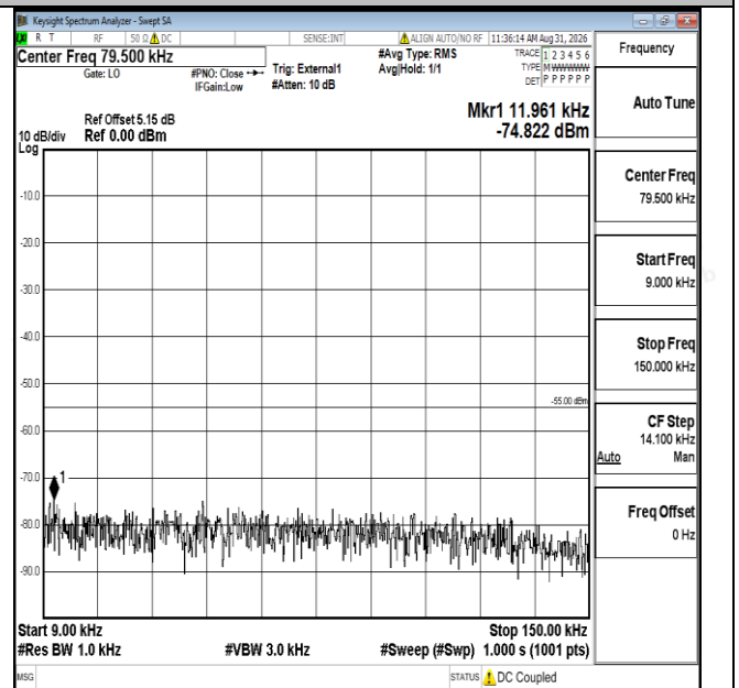
Band41-10MHz-16QAM-41540-1RB#0-0.009~0.15-PASS
