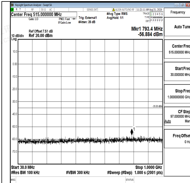
Band41-5MHz-QPSK-40620-1RB#0-30~1000-PASS
