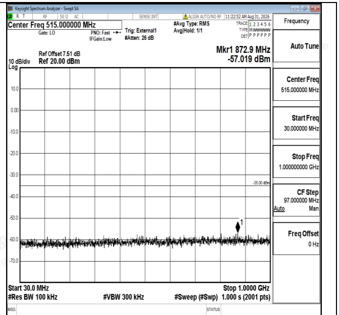
Band41-5MHz-16QAM-40620-1RB#0-30~1000-PASS
