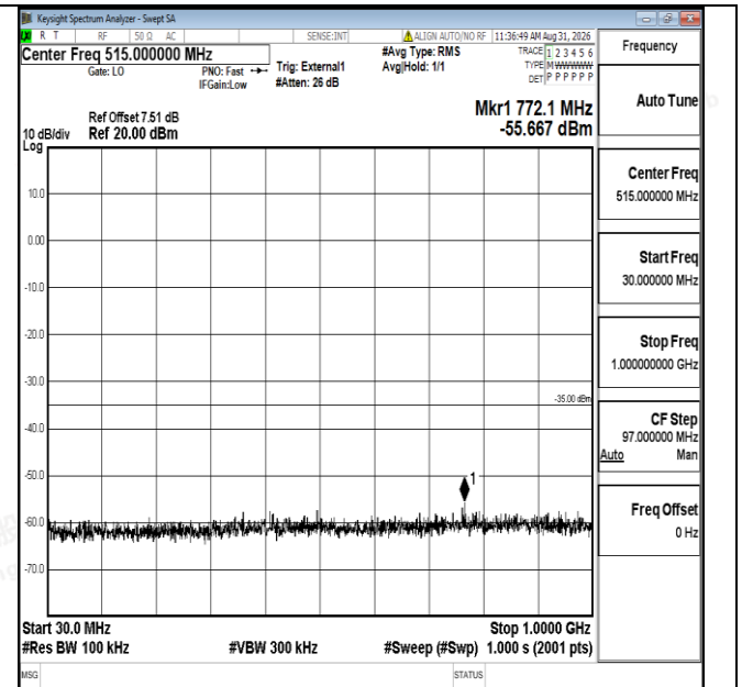
Band41-10MHz-16QAM-41540-1RB#0-30~1000-PASS
