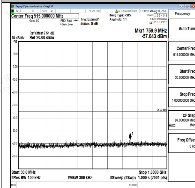
Band41-10MHz-QPSK-40620-1RB#0-30~1000-PASS
