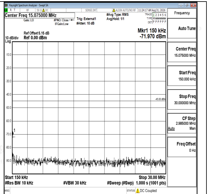
Band41-5MHz-QPSK-41565-1RB#0-0.15~30-PASS
