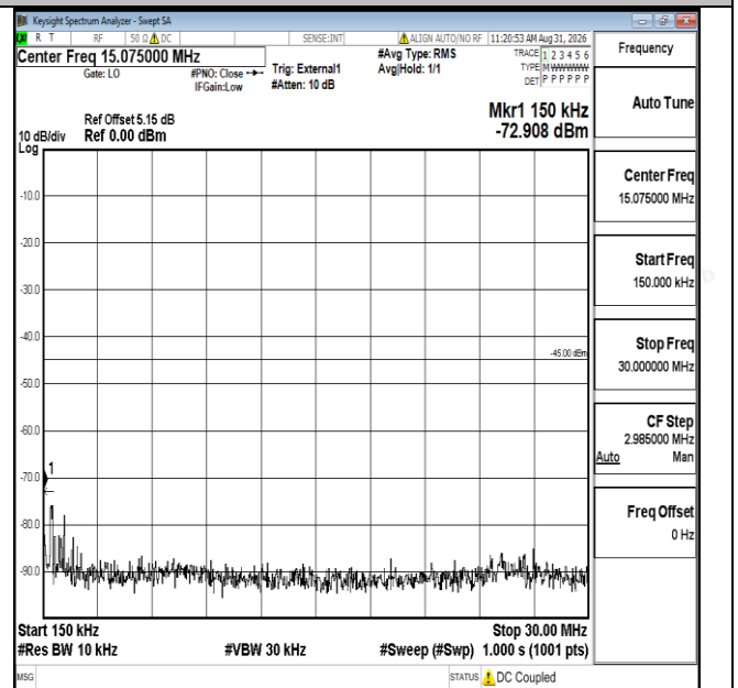
Band41-5MHz-QPSK-40620-1RB#0-0.15~30-PASS
