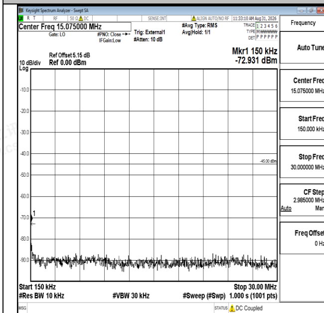
Band41-10MHz-16QAM-40620-1RB#0-0.15~30-PASS
