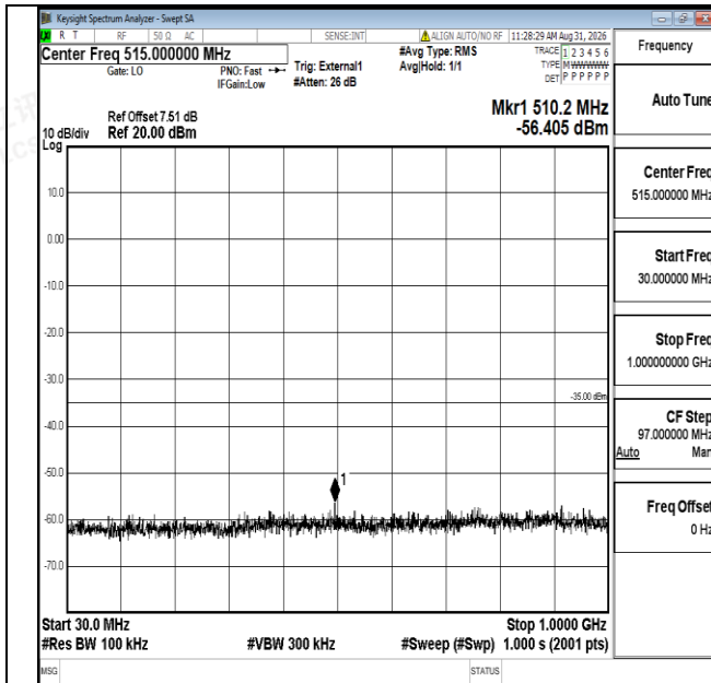
Band41-10MHz-QPSK-39700-1RB#0-30~1000-PASS
