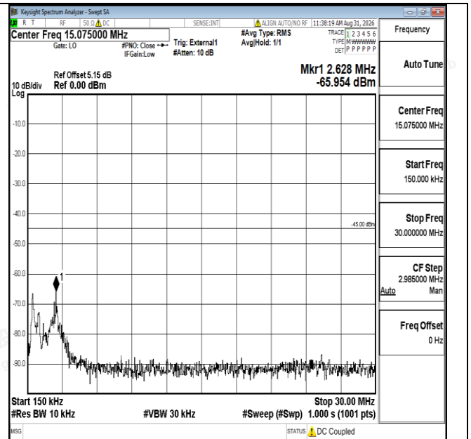
Band41-15MHz-QPSK-39725-1RB#0-0.15~30-PASS
