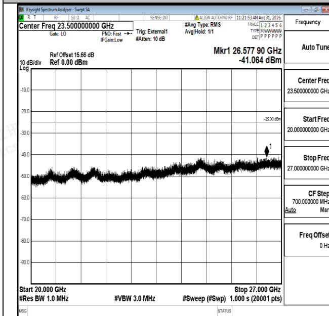
Band41-5MHz-QPSK-40620-1RB#0-20000~27000-PASS
