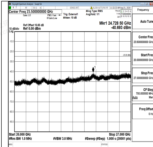
Band41-10MHz-QPSK-40620-1RB#0-20000~27000-PASS
