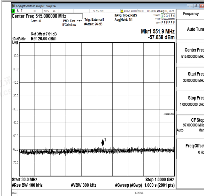
Band41-15MHz-QPSK-39725-1RB#0-30~1000-PASS
