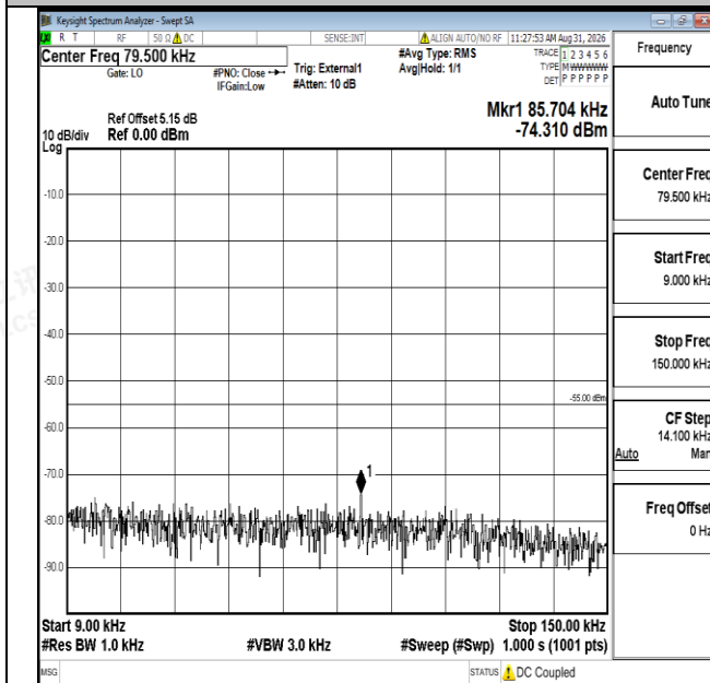
Band41-10MHz-QPSK-39700-1RB#0-0.009~0.15-PASS
