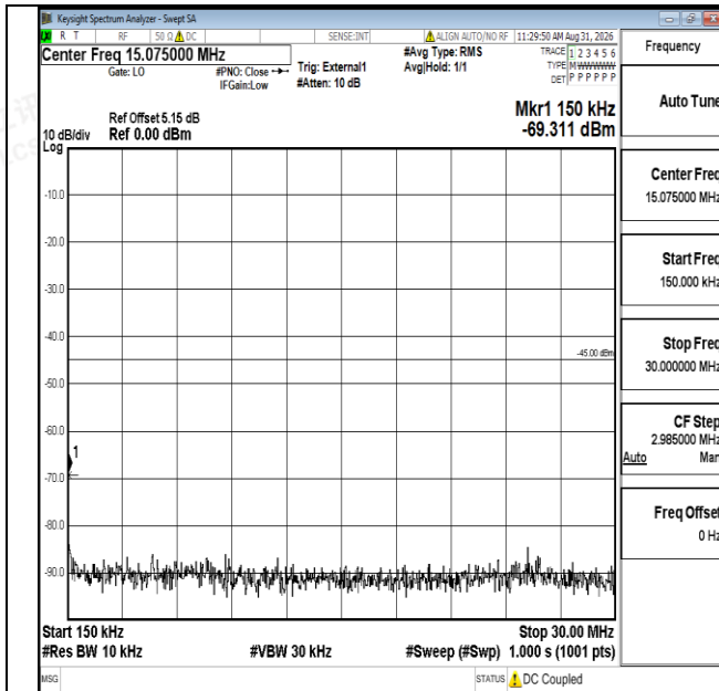
Band41-10MHz-16QAM-39700-1RB#0-0.15~30-PASS
