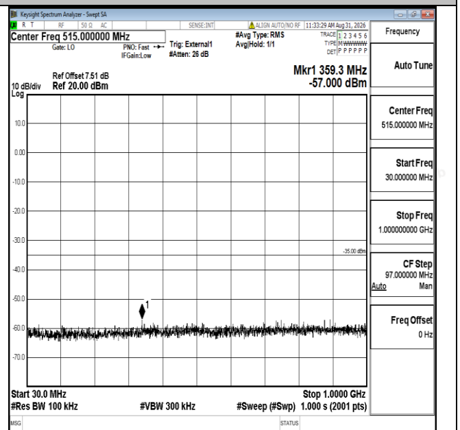
Band41-10MHz-16QAM-40620-1RB#0-30~1000-PASS
