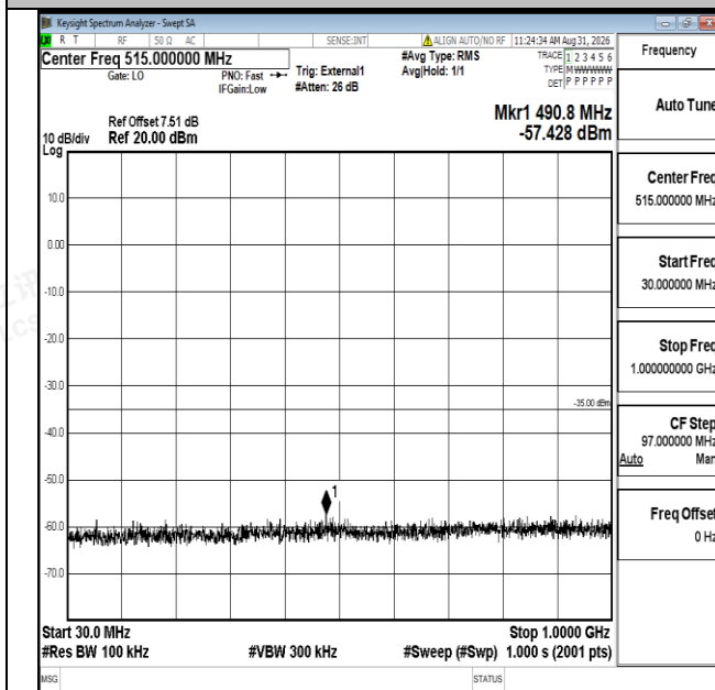
Band41-5MHz-QPSK-41565-1RB#0-30~1000-PASS
