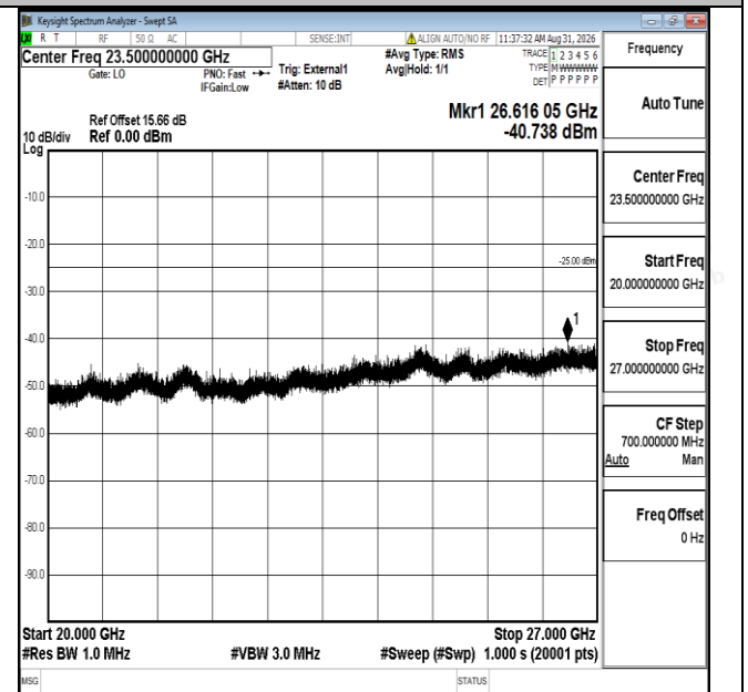
Band41-10MHz-16QAM-41540-1RB#0-20000~27000-PASS
