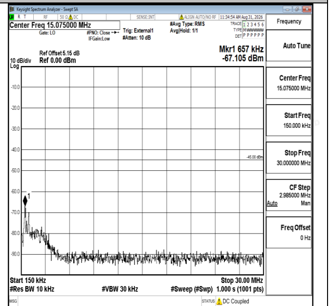
Band41-10MHz-QPSK-41540-1RB#0-0.15~30-PASS
