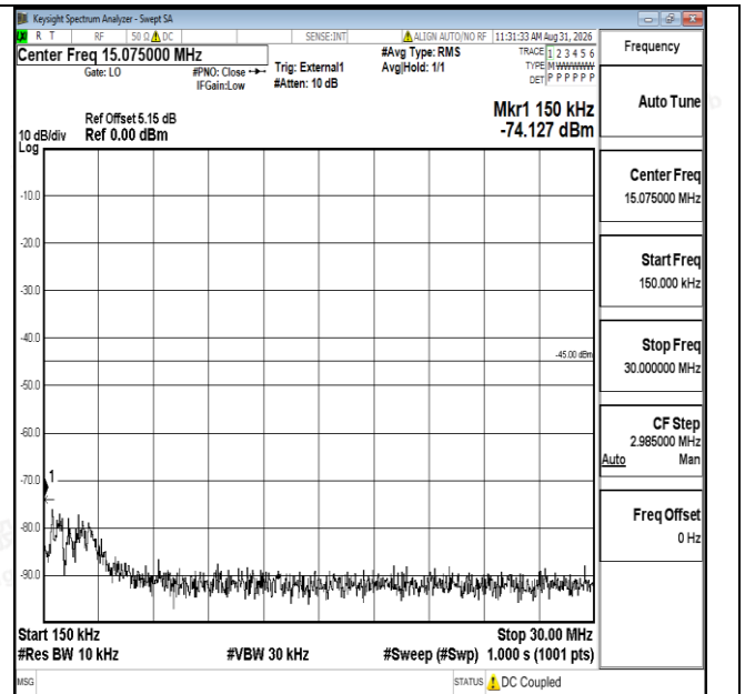
Band41-10MHz-QPSK-40620-1RB#0-0.15~30-PASS
