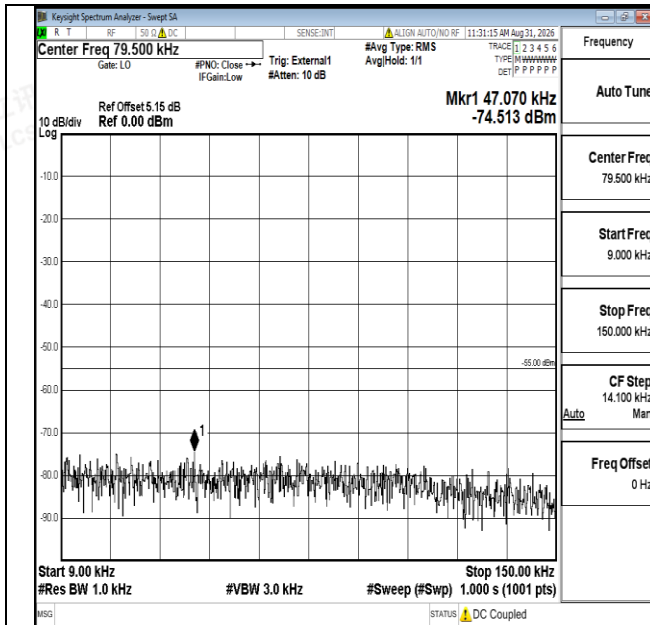
Band41-10MHz-QPSK-40620-1RB#0-0.009~0.15-PASS
