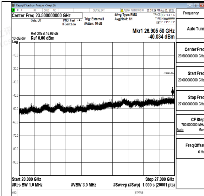
Band41-5MHz-QPSK-39675-1RB#0-20000~27000-PASS
