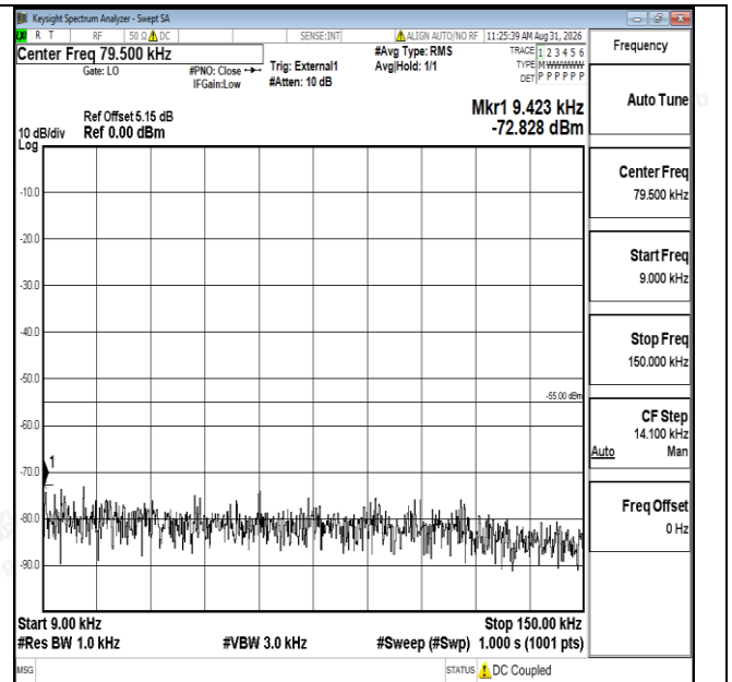
Band41-5MHz-16QAM-41565-1RB#0-0.009~0.15-PASS
