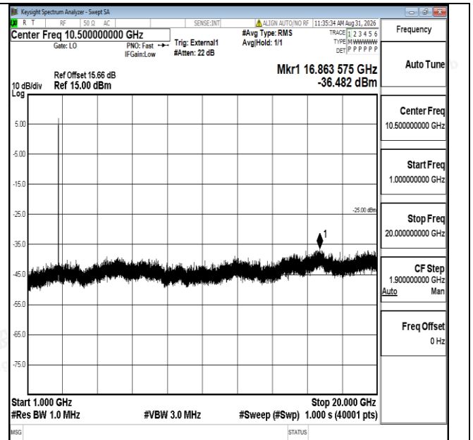
Band41-10MHz-QPSK-41540-1RB#0-1000~20000-PASS
