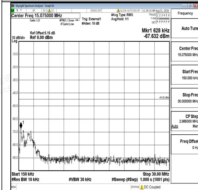
Band41-5MHz-16QAM-39675-1RB#0-0.15~30-PASS
