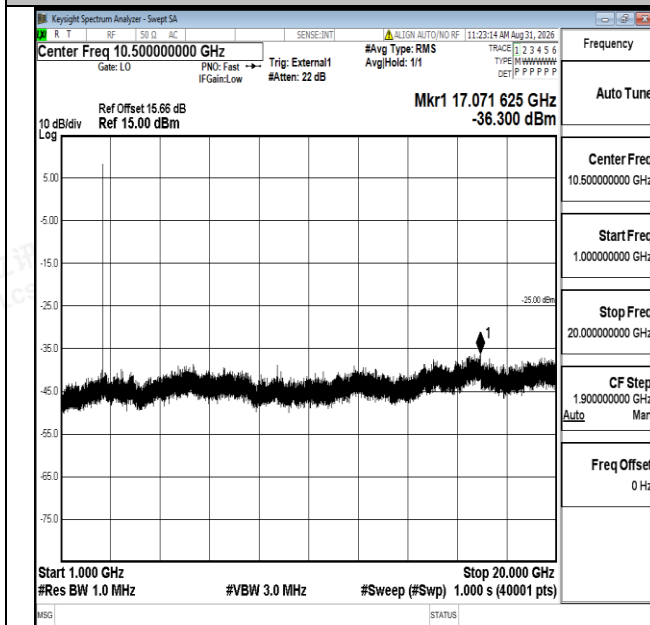
Band41-5MHz-16QAM-40620-1RB#0-1000~20000-PASS
