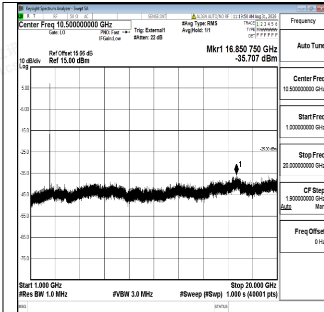
Band41-5MHz-16QAM-39675-1RB#0-1000~20000-PASS
