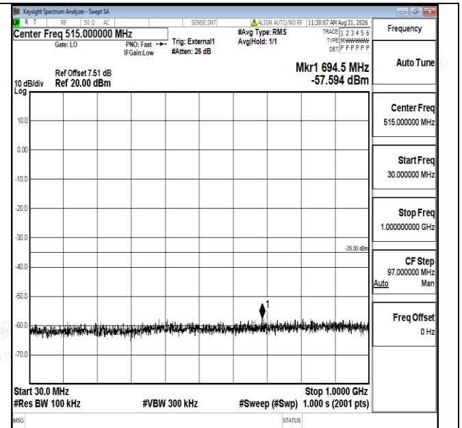
Band41-10MHz-16QAM-39700-1RB#0-30~1000-PASS
