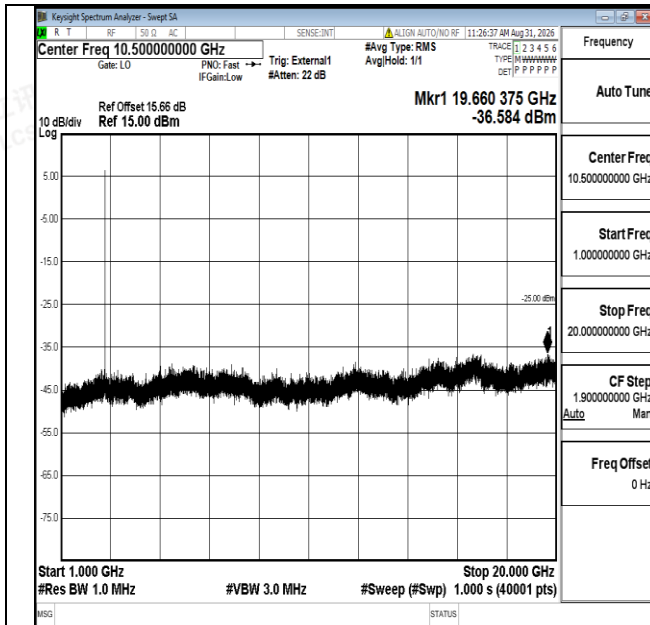
Band41-5MHz-16QAM-41565-1RB#0-1000~20000-PASS
