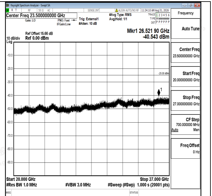
Band41-10MHz-16QAM-40620-1RB#0-20000~27000-PASS
