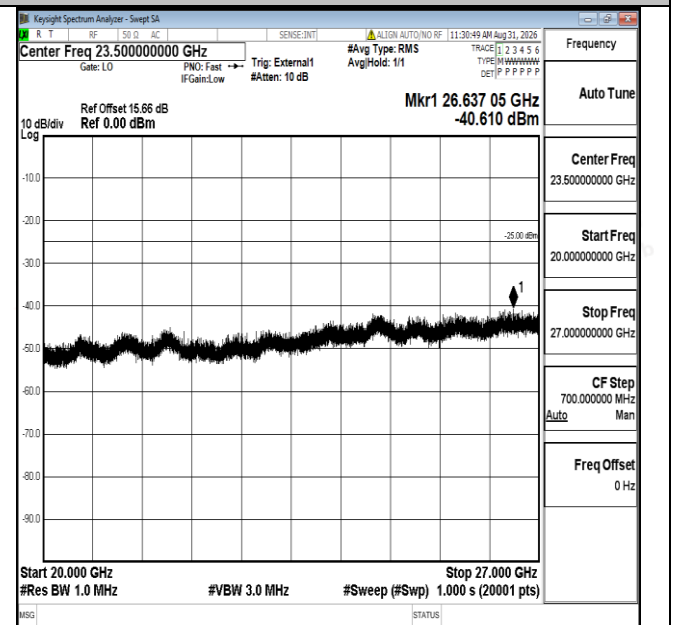
Band41-10MHz-16QAM-39700-1RB#0-20000~27000-PASS
