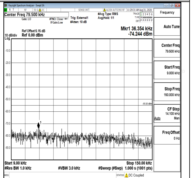
Band41-10MHz-16QAM-39700-1RB#0-0.009~0.15-PASS
