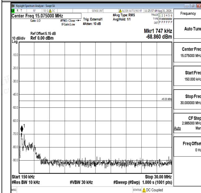
Band41-5MHz-16QAM-41565-1RB#0-0.15~30-PASS
