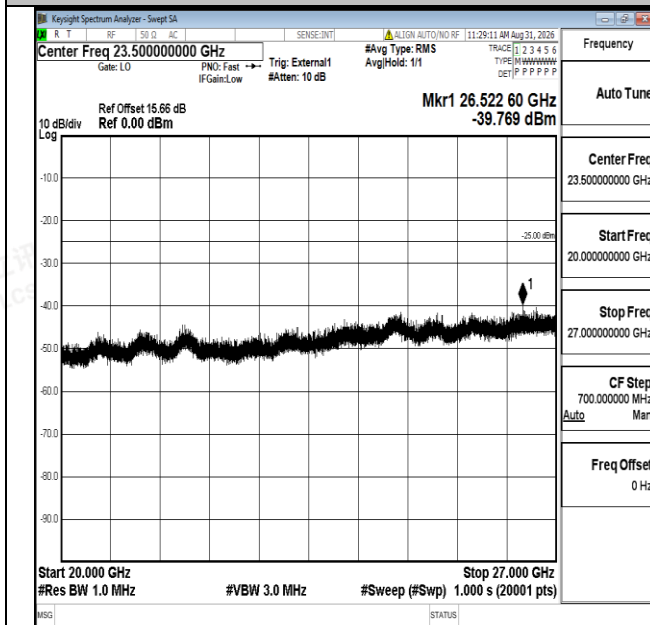
Band41-10MHz-QPSK-39700-1RB#0-20000~27000-PASS
