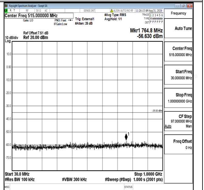
Band41-5MHz-16QAM-41565-1RB#0-30~1000-PASS
