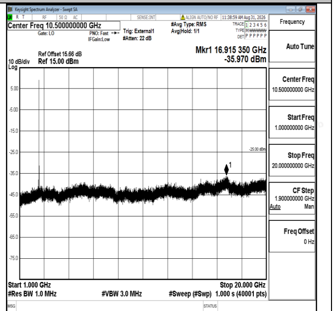
Band41-15MHz-QPSK-39725-1RB#0-1000~20000-PASS
