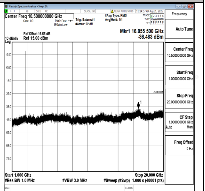
Band41-5MHz-QPSK-41565-1RB#0-1000~20000-PASS
