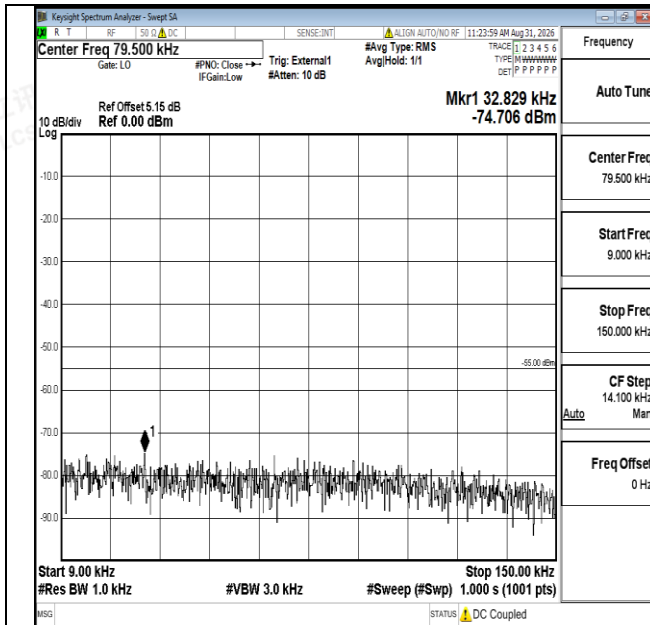
Band41-5MHz-QPSK-41565-1RB#0-0.009~0.15-PASS
