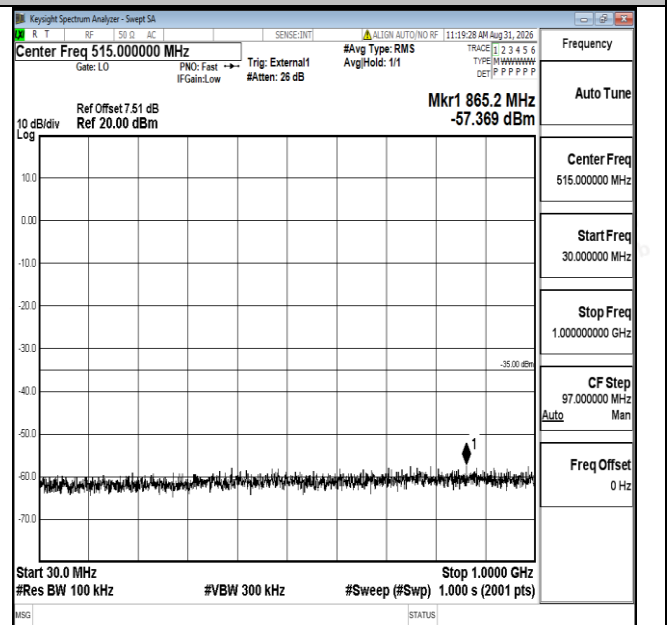
Band41-5MHz-16QAM-39675-1RB#0-30~1000-PASS
