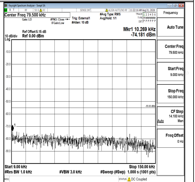
Band41-5MHz-16QAM-40620-1RB#0-0.009~0.15-PASS
