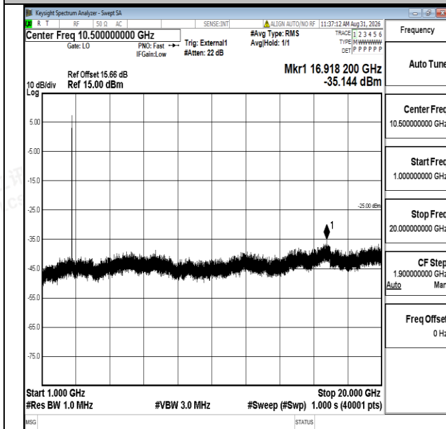
Band41-10MHz-16QAM-41540-1RB#0-1000~20000-PASS
