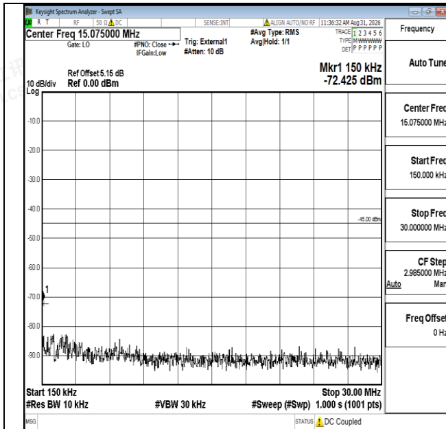
Band41-10MHz-16QAM-41540-1RB#0-0.15~30-PASS
