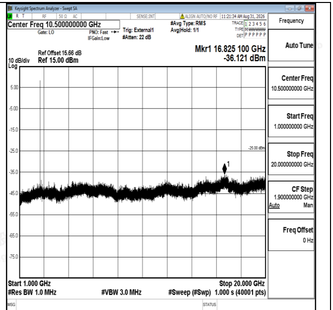
Band41-5MHz-QPSK-40620-1RB#0-1000~20000-PASS
