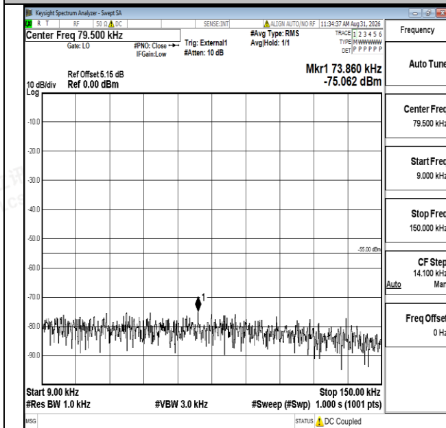
Band41-10MHz-QPSK-41540-1RB#0-0.009~0.15-PASS
