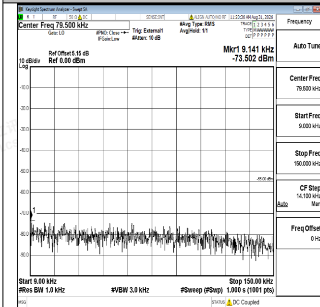
Band41-5MHz-QPSK-40620-1RB#0-0.009~0.15-PASS
