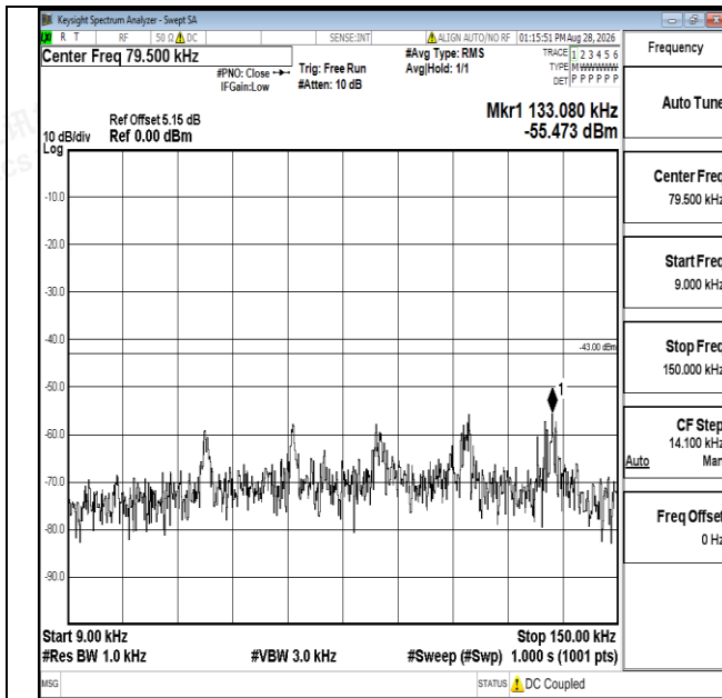
Band66-1.4MHz-QPSK-132322-1RB#0-0.009~0.15-PASS
