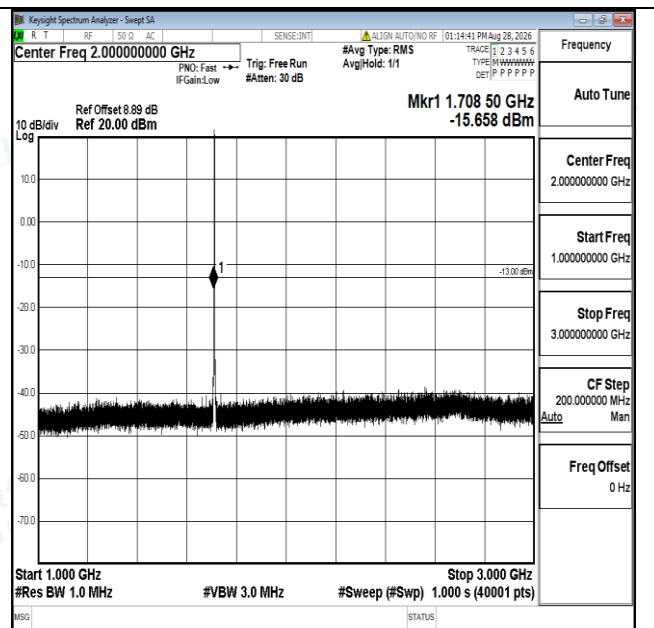
Band66-1.4MHz-QPSK-131979-1RB#0-1000~3000-PASS
