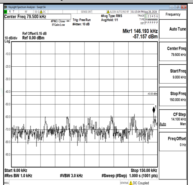
Band66-1.4MHz-16QAM-131979-1RB#0-0.009~0.15-PASS
