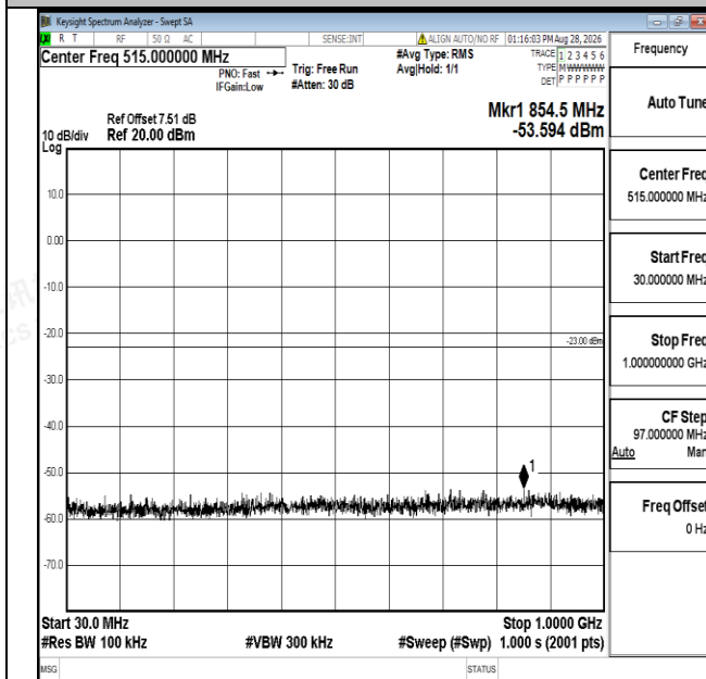
Band66-1.4MHz-QPSK-132322-1RB#0-30~1000-PASS
