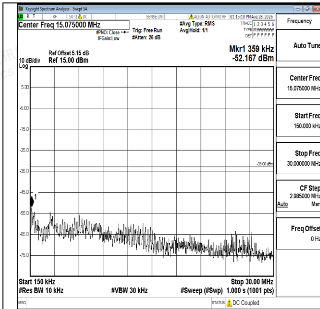
Band66-1.4MHz-16QAM-131979-1RB#0-0.15~30-PASS
