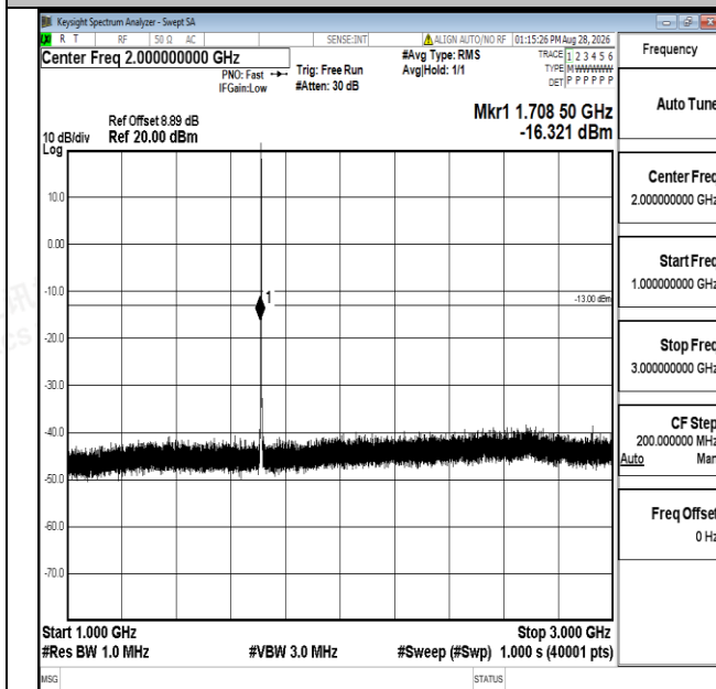
Band66-1.4MHz-16QAM-131979-1RB#0-1000~3000-PASS
