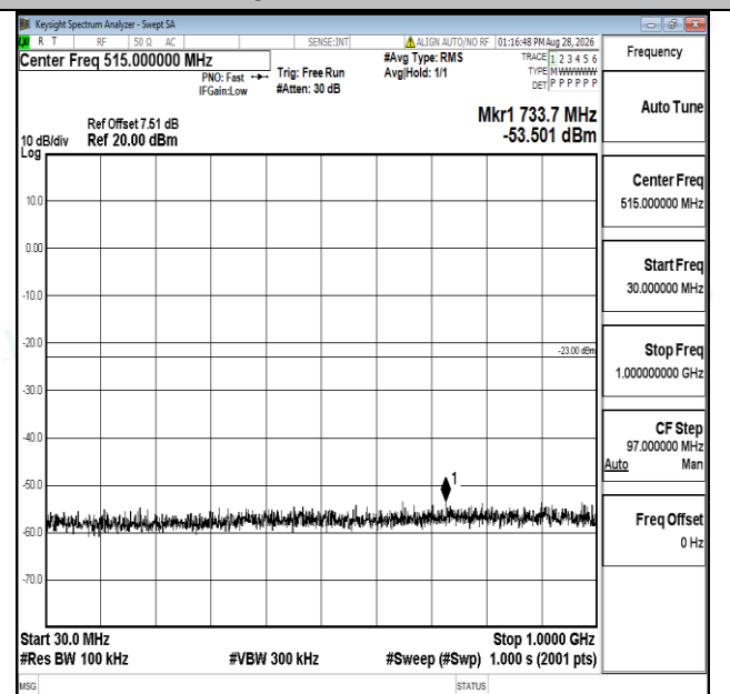
Band66-1.4MHz-16QAM-132322-1RB#0-30~1000-PASS
