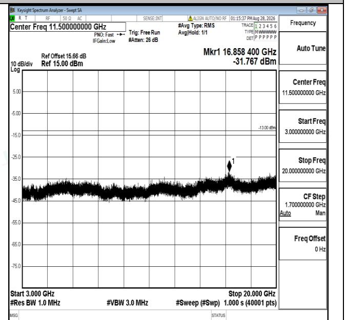
Band66-1.4MHz-16QAM-131979-1RB#0-3000~20000-PASS
