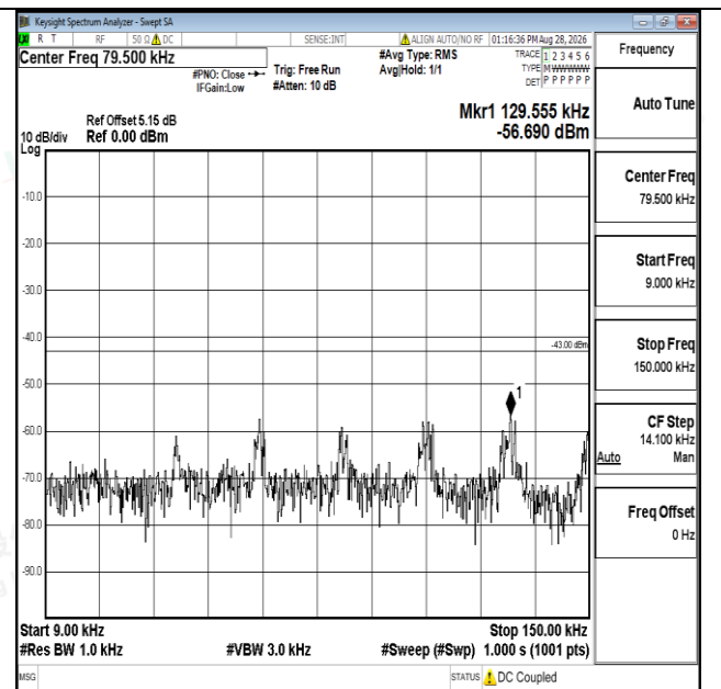
Band66-1.4MHz-16QAM-132322-1RB#0-0.009~0.15-PASS
