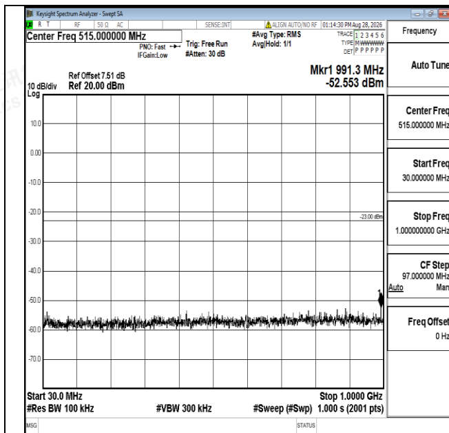
Band66-1.4MHz-QPSK-131979-1RB#0-30~1000-PASS
