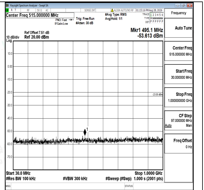
Band66-1.4MHz-16QAM-131979-1RB#0-30~1000-PASS
