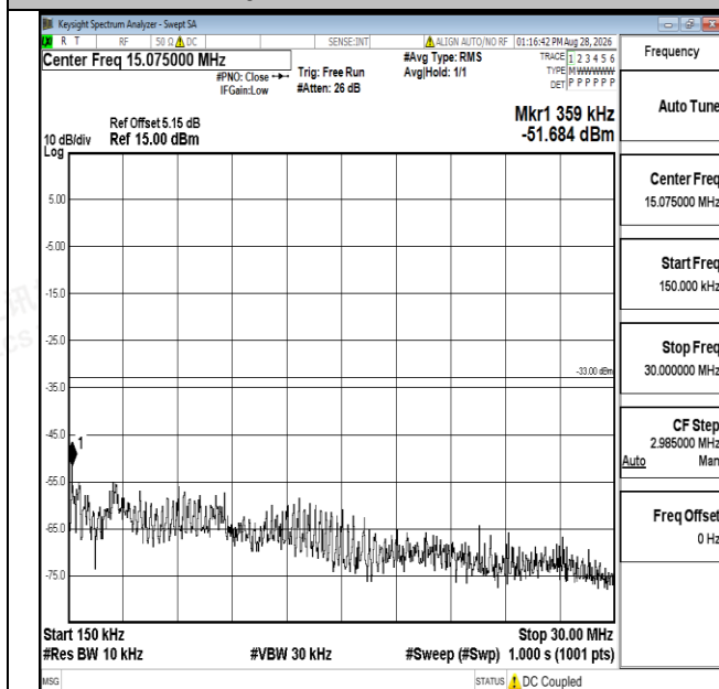
Band66-1.4MHz-16QAM-132322-1RB#0-0.15~30-PASS
