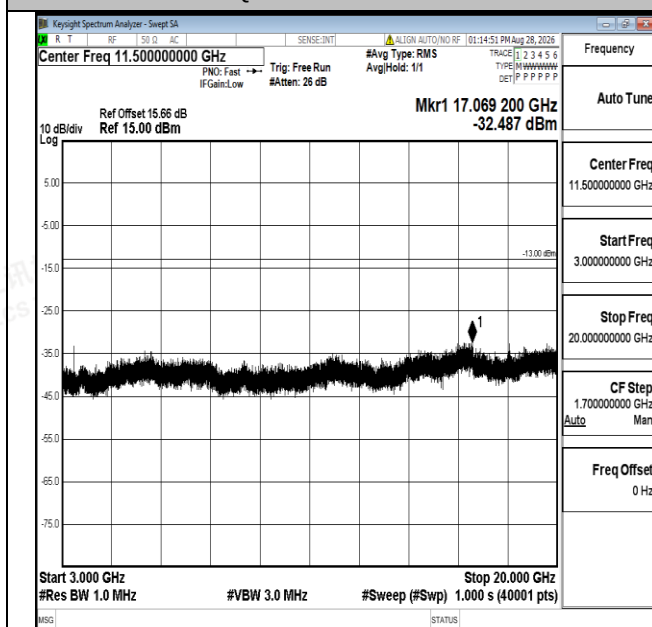
Band66-1.4MHz-QPSK-131979-1RB#0-3000~20000-PASS
