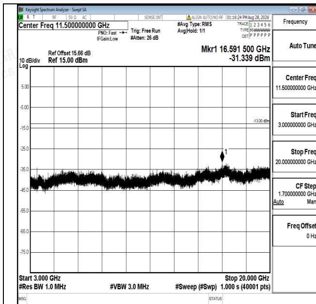
Band66-1.4MHz-QPSK-132322-1RB#0-3000~20000-PASS
