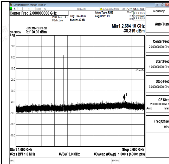
Band66-5MHz-16QAM-132322-1RB#0-1000~3000-PASS
