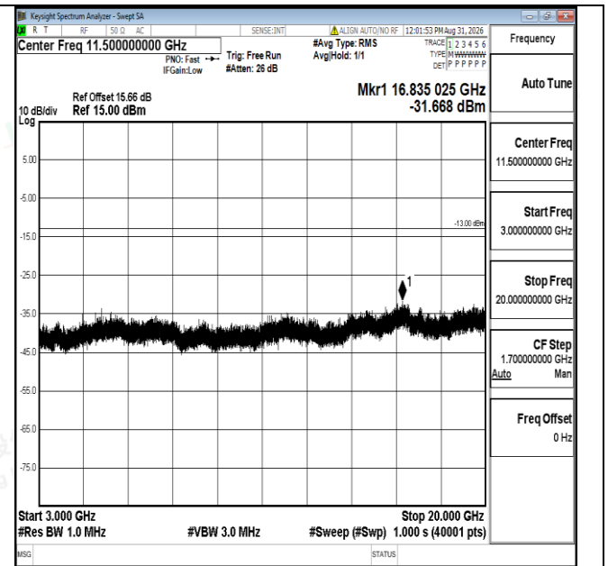
Band66-5MHz-16QAM-132322-1RB#0-3000~20000-PASS
