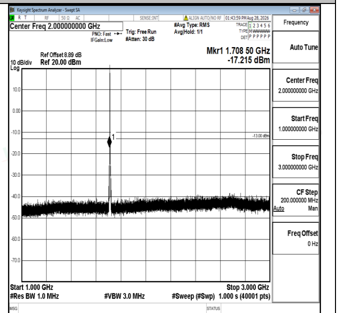
Band66-3MHz-QPSK-131987-1RB#0-1000~3000-PASS
