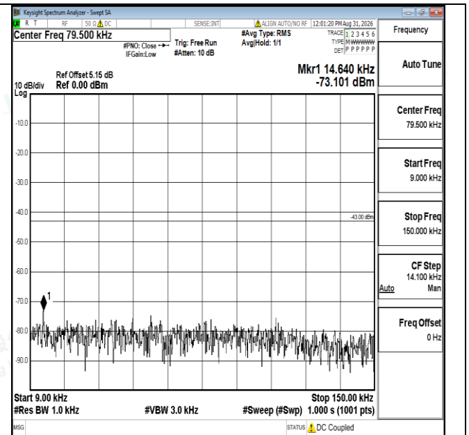
Band66-5MHz-16QAM-132322-1RB#0-0.009~0.15-PASS
