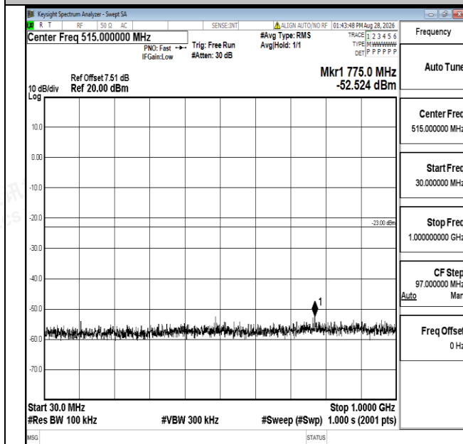
Band66-3MHz-QPSK-131987-1RB#0-30~1000-PASS
