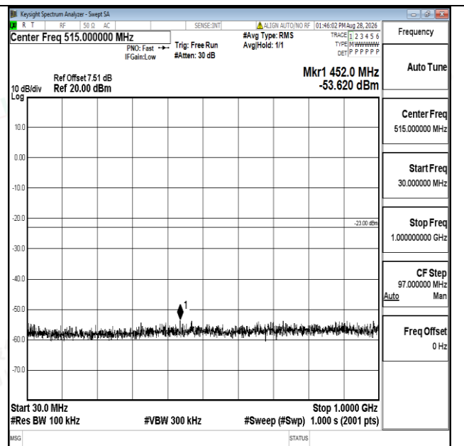
Band66-3MHz-16QAM-132322-1RB#0-30~1000-PASS
