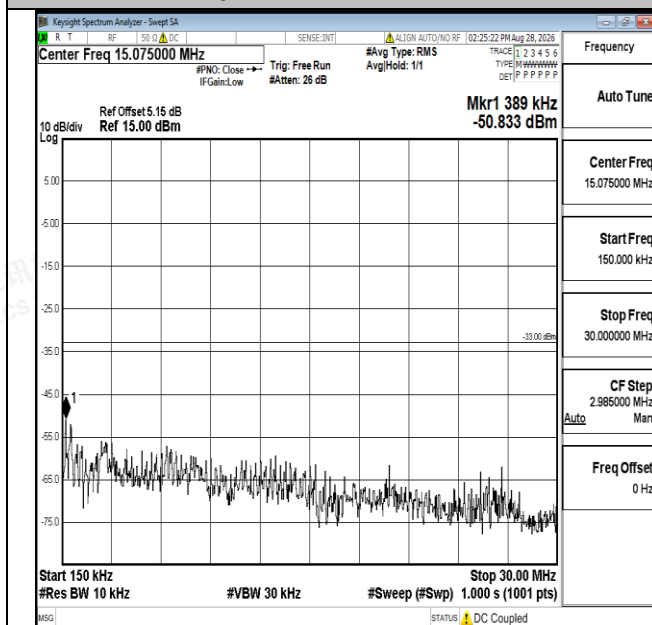
Band66-10MHz-16QAM-132022-1RB#0-0.15~30-PASS
