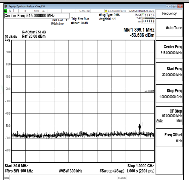
Band66-10MHz-16QAM-132022-1RB#0-30~1000-PASS
