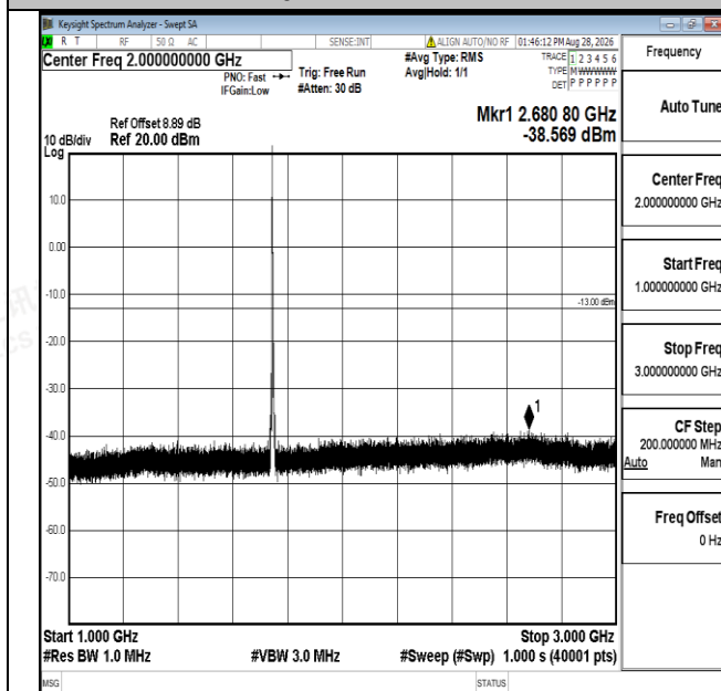
Band66-3MHz-16QAM-132322-1RB#0-1000~3000-PASS
