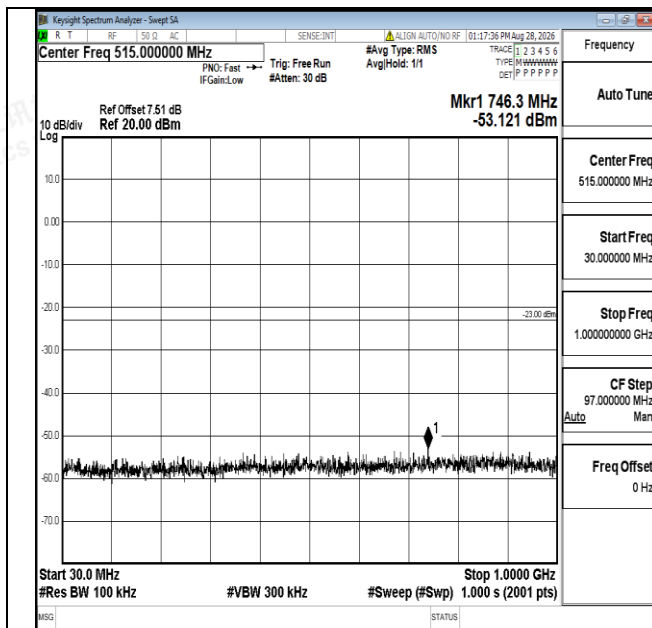
Band66-1.4MHz-QPSK-132665-1RB#0-30~1000-PASS
