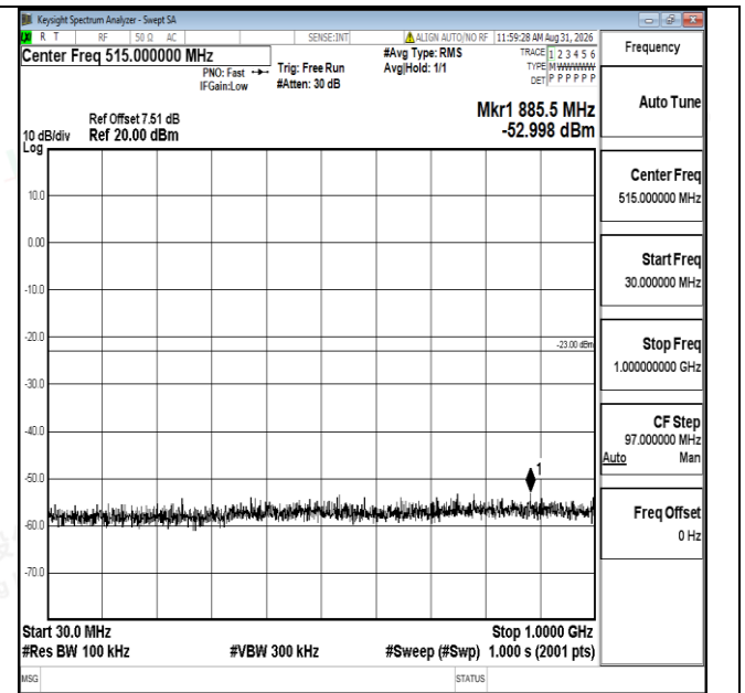
Band66-5MHz-16QAM-131997-1RB#0-30~1000-PASS
