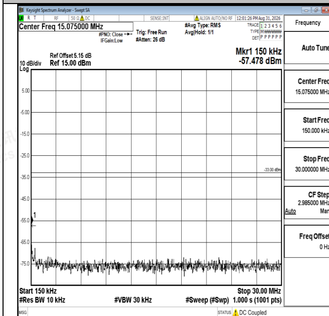
Band66-5MHz-16QAM-132322-1RB#0-0.15~30-PASS
