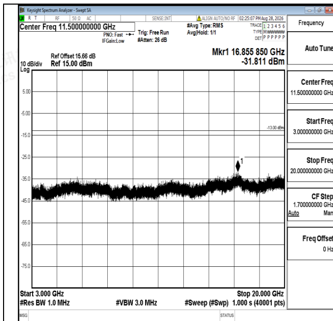
Band66-10MHz-QPSK-132022-1RB#0-3000~20000-PASS
