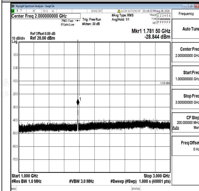
Band66-1.4MHz-16QAM-132665-1RB#0-1000~3000-PASS
