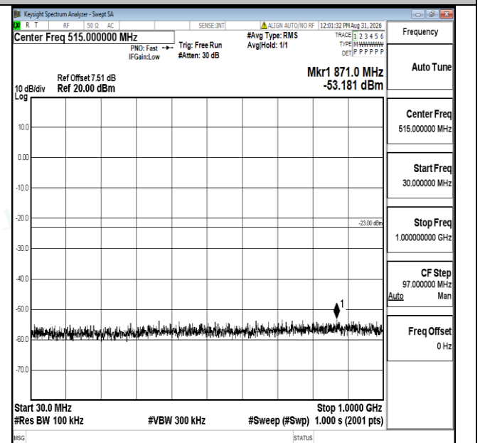
Band66-5MHz-16QAM-132322-1RB#0-30~1000-PASS
