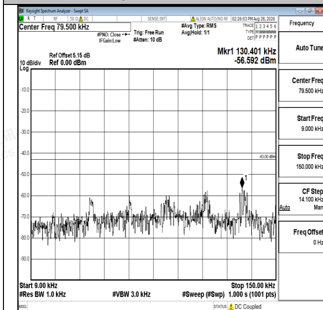
Band66-10MHz-QPSK-132322-1RB#0-0.009~0.15-PASS
