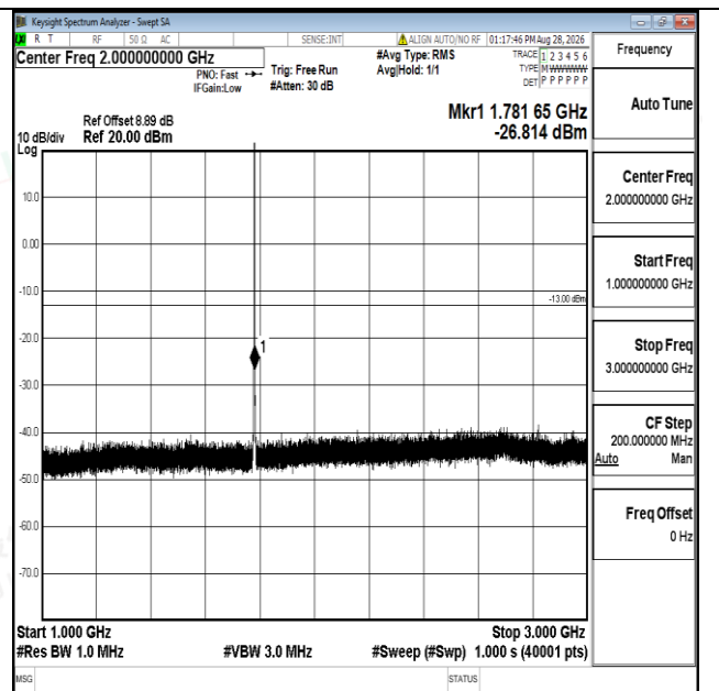
Band66-1.4MHz-QPSK-132665-1RB#0-1000~3000-PASS
