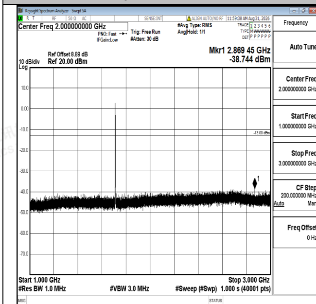
Band66-5MHz-16QAM-131997-1RB#0-1000~3000-PASS
