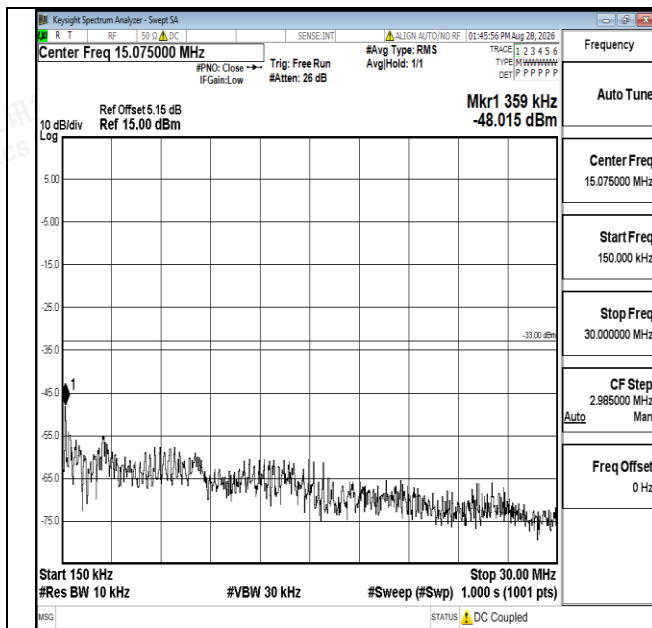
Band66-3MHz-16QAM-132322-1RB#0-0.15~30-PASS
