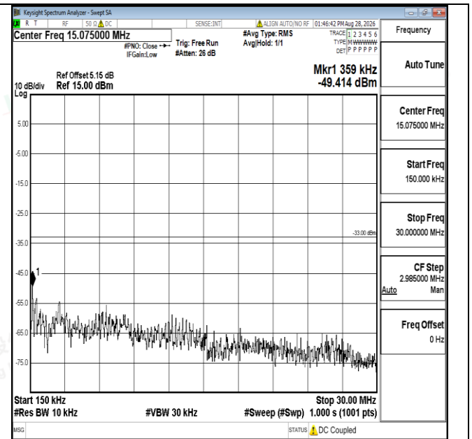
Band66-3MHz-QPSK-132657-1RB#0-0.15~30-PASS
