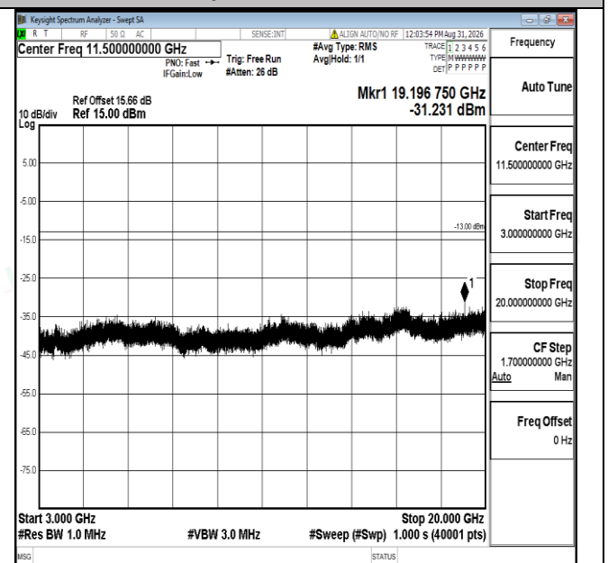
Band66-5MHz-16QAM-132647-1RB#0-3000~20000-PASS
