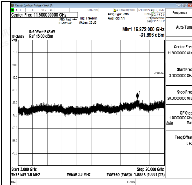
Band66-5MHz-QPSK-132322-1RB#0-3000~20000-PASS
