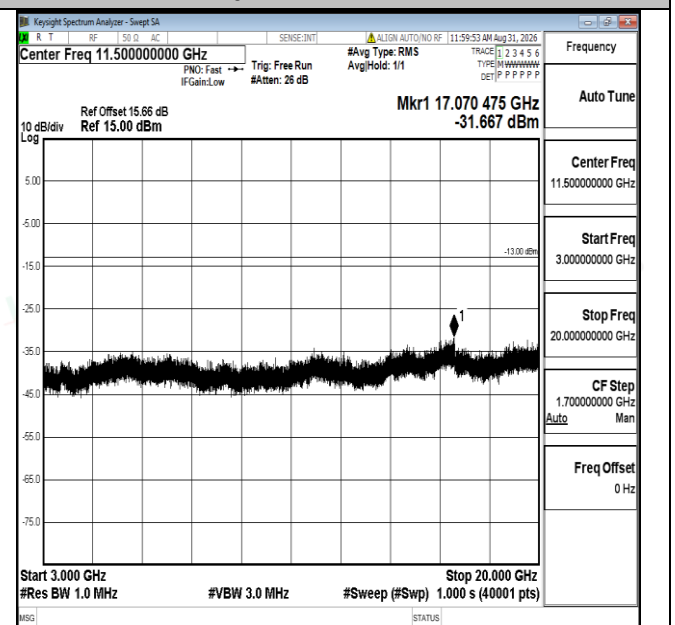
Band66-5MHz-16QAM-131997-1RB#0-3000~20000-PASS
