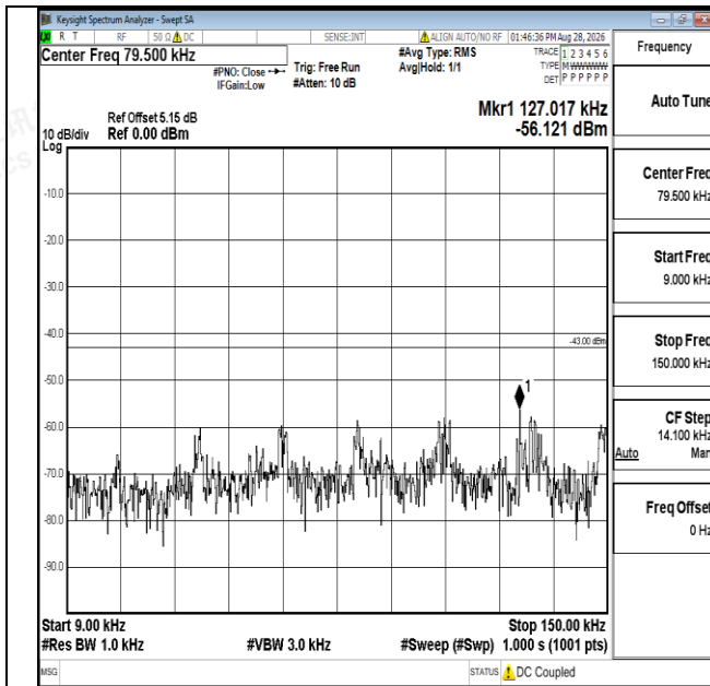
Band66-3MHz-QPSK-132657-1RB#0-0.009~0.15-PASS
