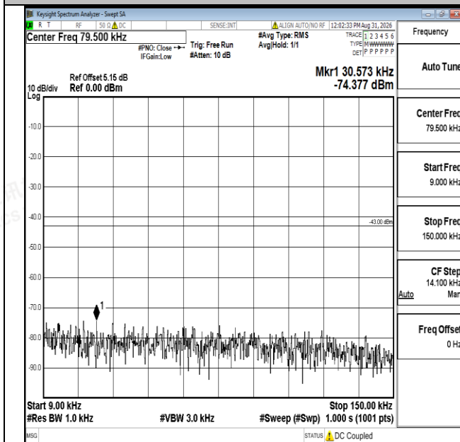
Band66-5MHz-QPSK-132647-1RB#0-0.009~0.15-PASS
