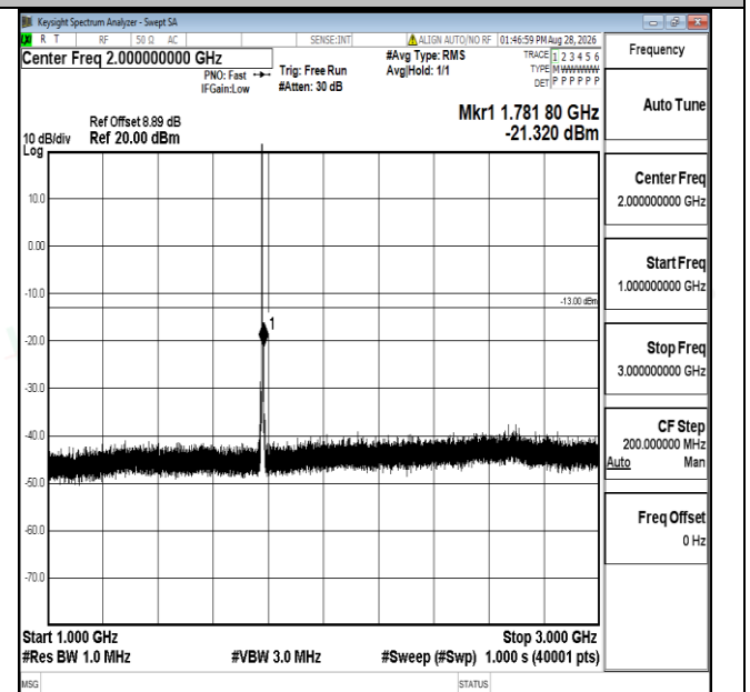
Band66-3MHz-QPSK-132657-1RB#0-1000~3000-PASS
