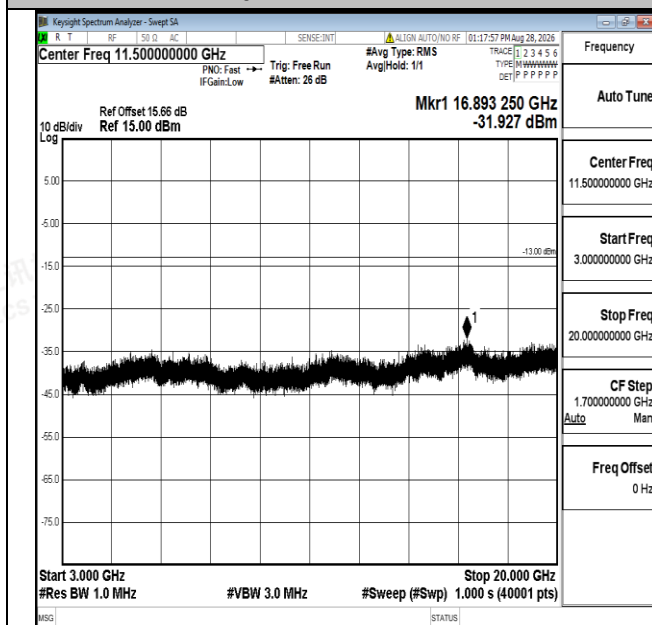
Band66-1.4MHz-QPSK-132665-1RB#0-3000~20000-PASS
