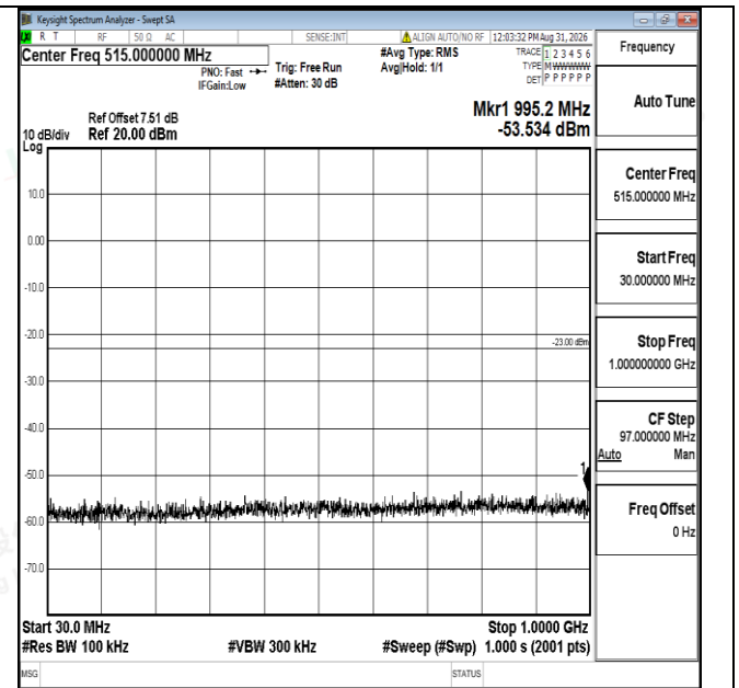
Band66-5MHz-16QAM-132647-1RB#0-30~1000-PASS
