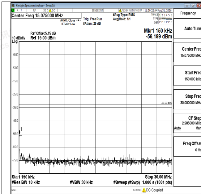
Band66-5MHz-16QAM-131997-1RB#0-0.15~30-PASS
