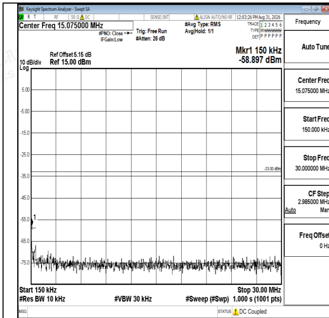
Band66-5MHz-16QAM-132647-1RB#0-0.15~30-PASS
