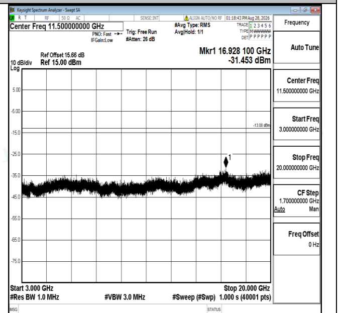
Band66-1.4MHz-16QAM-132665-1RB#0-3000~20000-PASS
