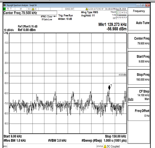
Band66-1.4MHz-16QAM-132665-1RB#0-0.009~0.15-PASS
