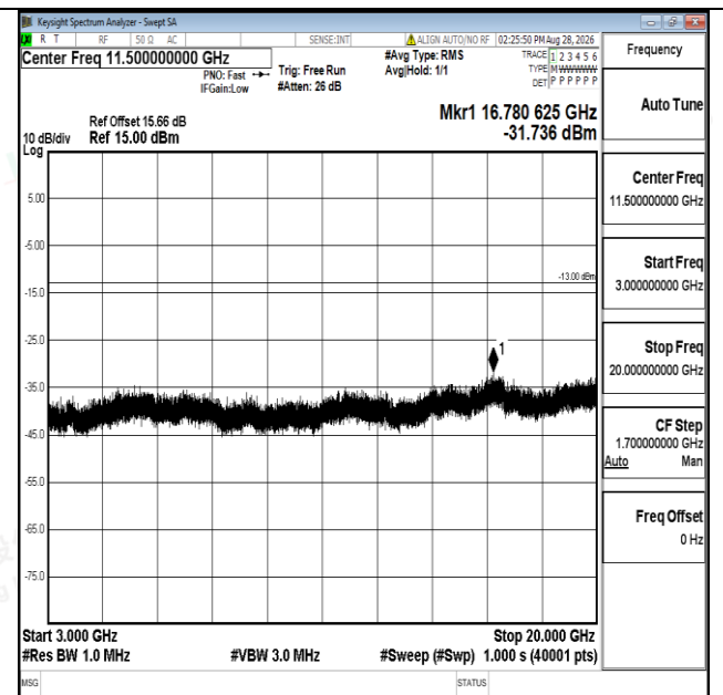
Band66-10MHz-16QAM-132022-1RB#0-3000~20000-PASS
