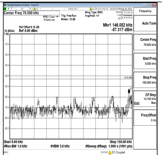
Band66-10MHz-16QAM-132022-1RB#0-0.009~0.15-PASS
