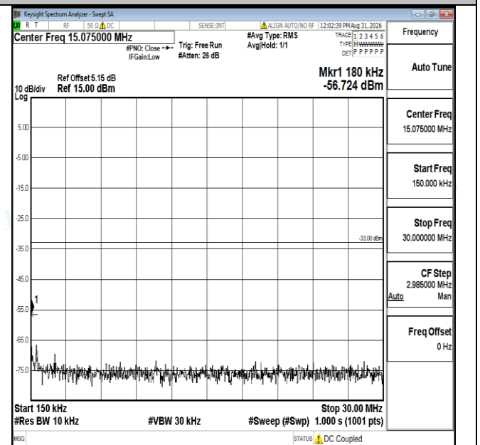
Band66-5MHz-QPSK-132647-1RB#0-0.15~30-PASS
