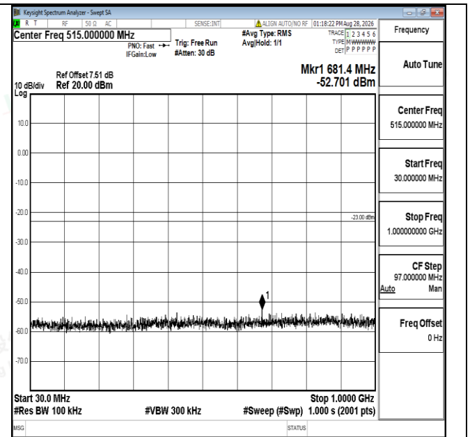
Band66-1.4MHz-16QAM-132665-1RB#0-30~1000-PASS
