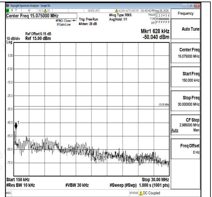
Band66-3MHz-QPSK-131987-1RB#0-0.15~30-PASS
