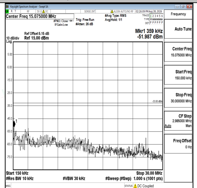
Band66-10MHz-QPSK-132322-1RB#0-0.15~30-PASS
