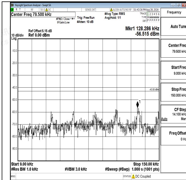
Band66-3MHz-QPSK-131987-1RB#0-0.009~0.15-PASS
