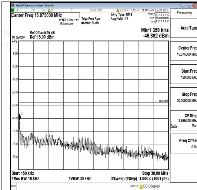
Band66-1.4MHz-16QAM-132665-1RB#0-0.15~30-PASS
