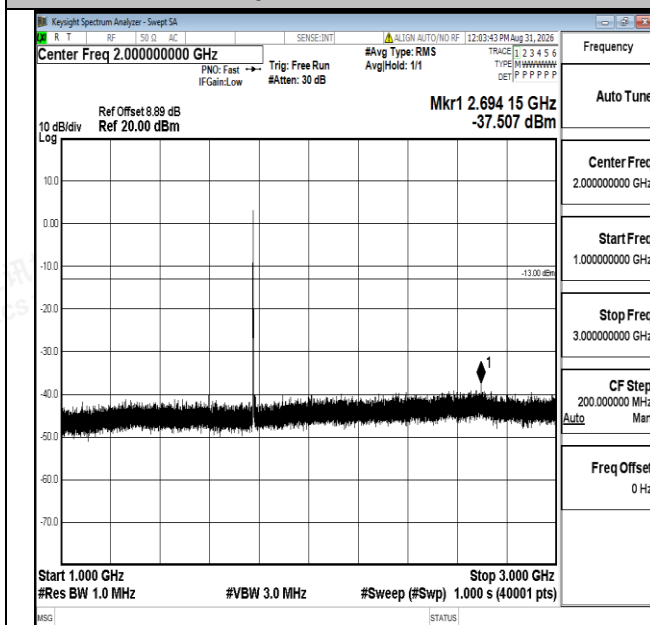
Band66-5MHz-16QAM-132647-1RB#0-1000~3000-PASS
