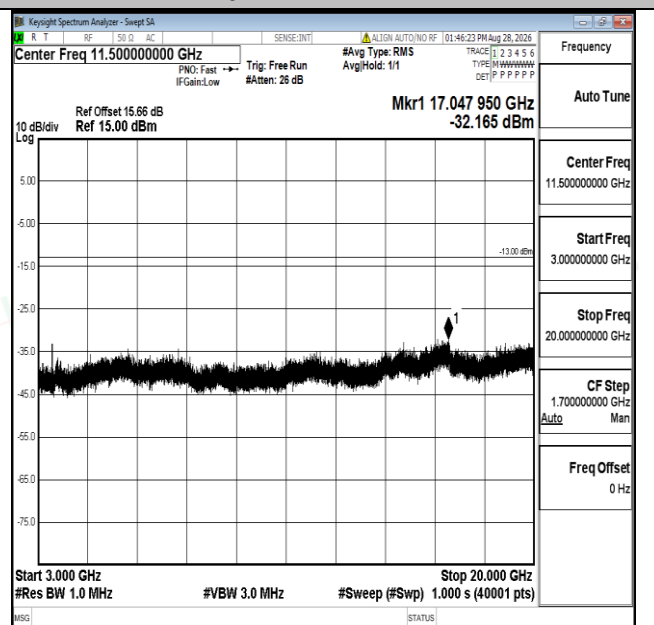
Band66-3MHz-16QAM-132322-1RB#0-3000~20000-PASS
