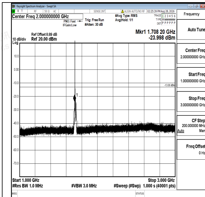
Band66-10MHz-16QAM-132022-1RB#0-1000~3000-PASS
