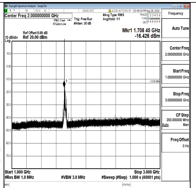
Band66-15MHz-QPSK-132047-1RB#0-1000~3000-PASS
