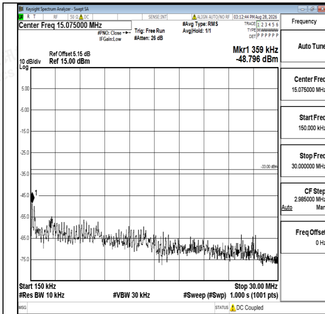
Band66-20MHz-16QAM-132322-1RB#0-0.15~30-PASS
