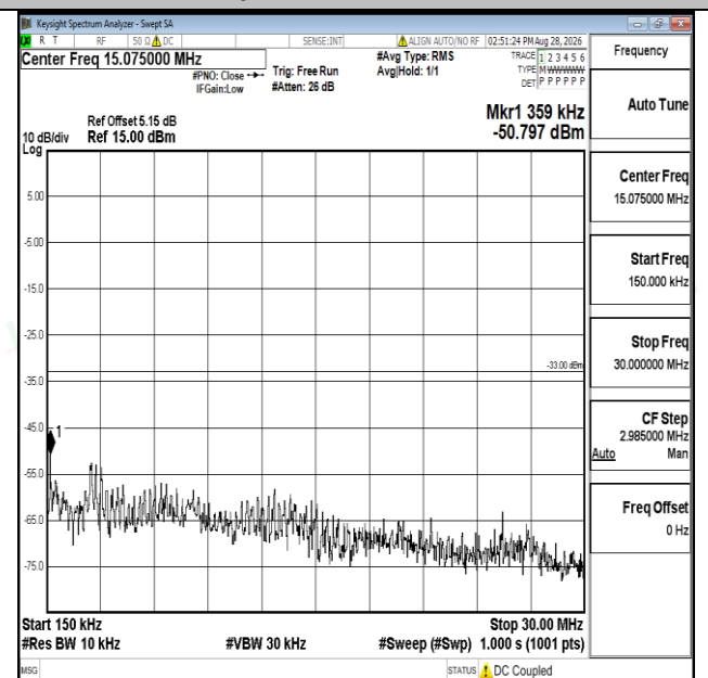
Band66-15MHz-QPSK-132597-1RB#0-0.15~30-PASS
