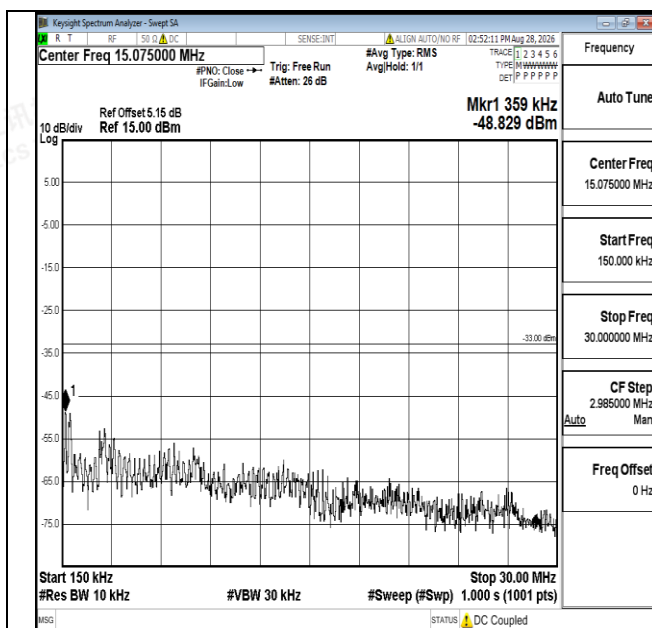
Band66-15MHz-16QAM-132597-1RB#0-0.15~30-PASS
