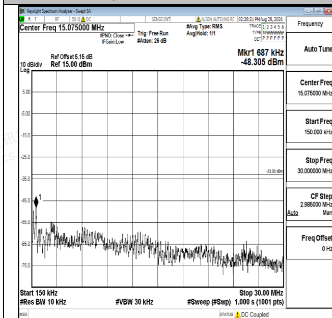
Band66-10MHz-16QAM-132622-1RB#0-0.15~30-PASS
