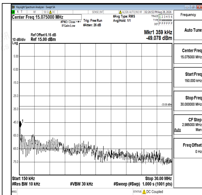
Band66-10MHz-16QAM-132322-1RB#0-0.15~30-PASS
