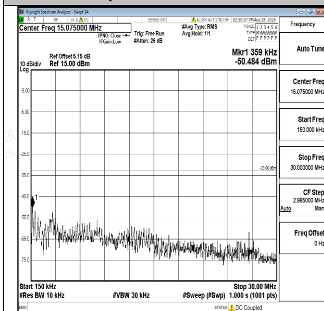
Band66-15MHz-16QAM-132322-1RB#0-0.15~30-PASS
