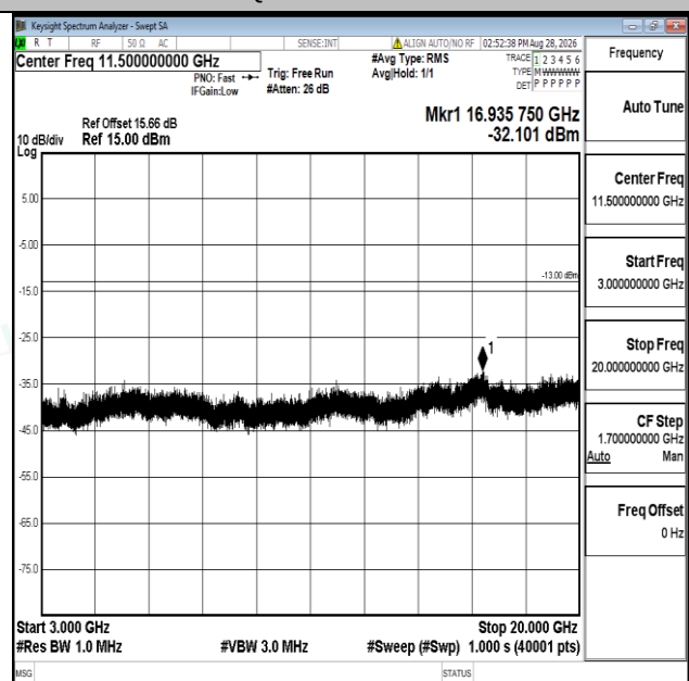
Band66-15MHz-16QAM-132597-1RB#0-3000~20000-PASS
