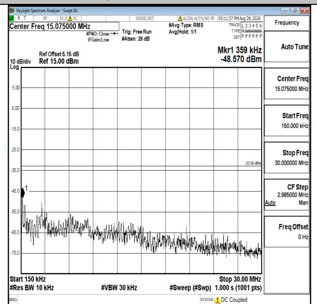
Band66-20MHz-QPSK-132322-1RB#0-0.15~30-PASS
