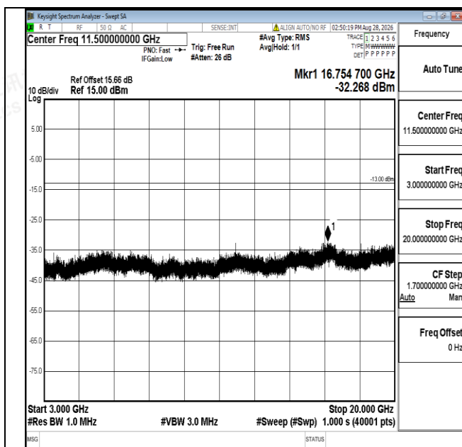
Band66-15MHz-QPSK-132322-1RB#0-3000~20000-PASS
