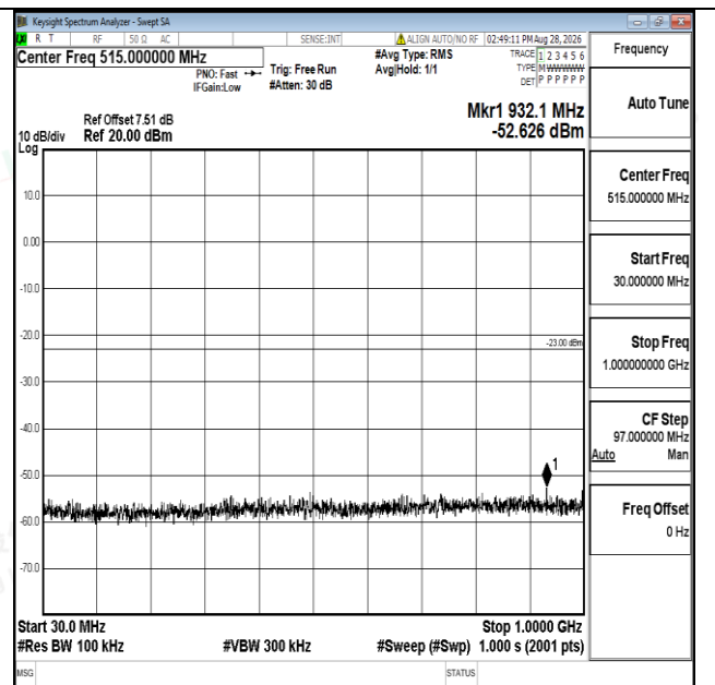
Band66-15MHz-16QAM-132047-1RB#0-30~1000-PASS
