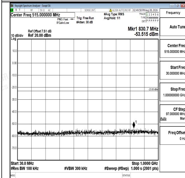
Band66-15MHz-QPSK-132322-1RB#0-30~1000-PASS
