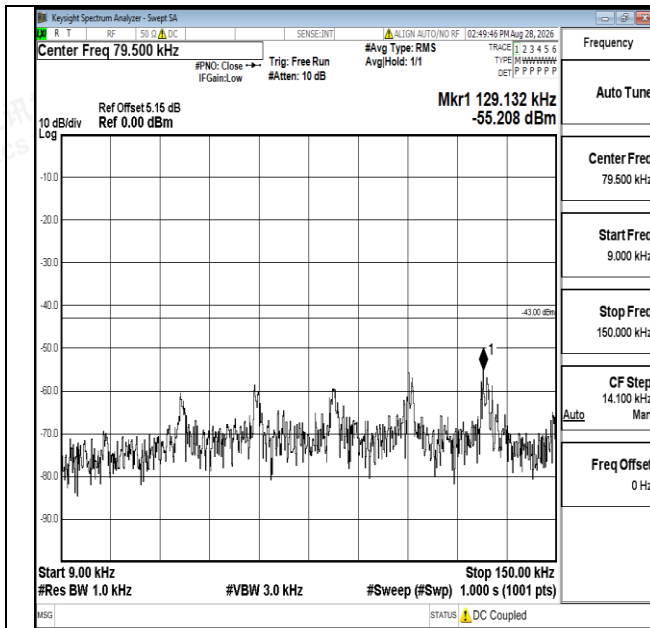
Band66-15MHz-QPSK-132322-1RB#0-0.009~0.15-PASS
