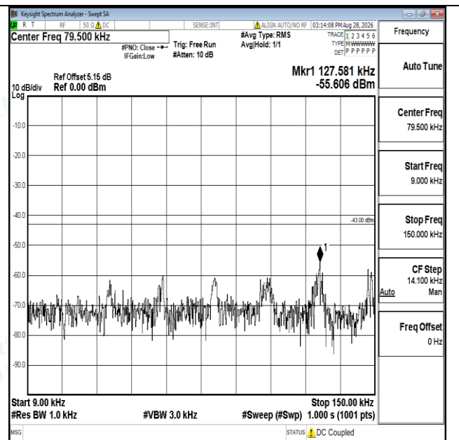
Band66-20MHz-16QAM-132572-1RB#0-0.009~0.15-PASS
