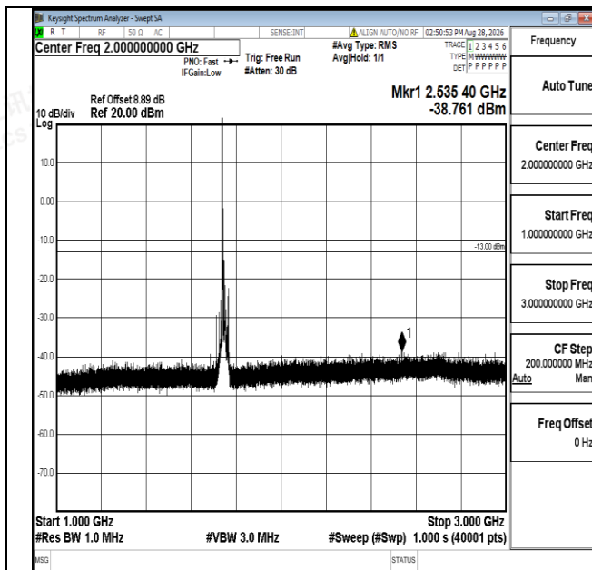
Band66-15MHz-16QAM-132322-1RB#0-1000~3000-PASS
