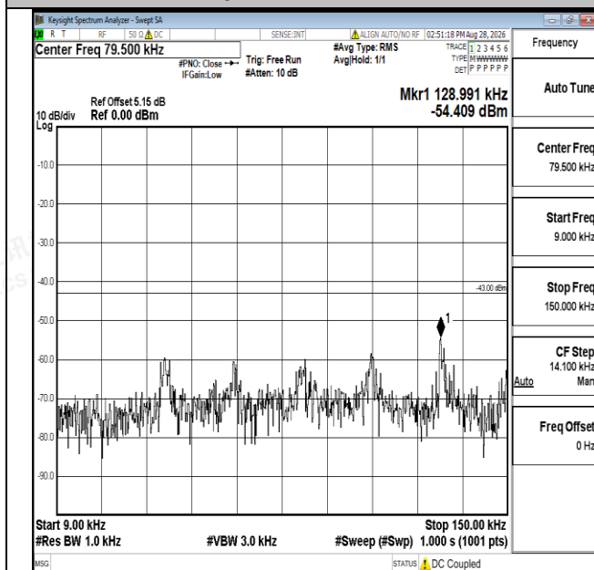
Band66-15MHz-QPSK-132597-1RB#0-0.009~0.15-PASS
