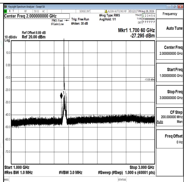
Band66-20MHz-QPSK-132322-1RB#0-1000~3000-PASS
