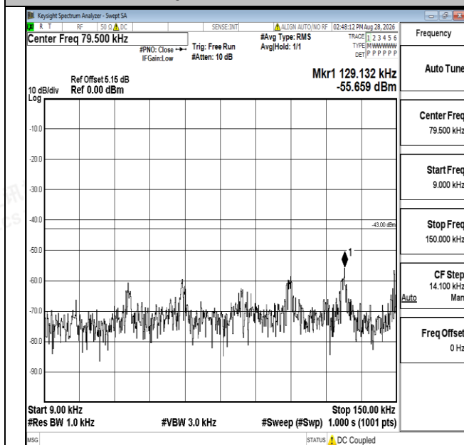
Band66-15MHz-QPSK-132047-1RB#0-0.009~0.15-PASS
