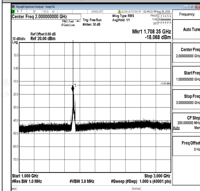
Band66-15MHz-16QAM-132047-1RB#0-1000~3000-PASS
