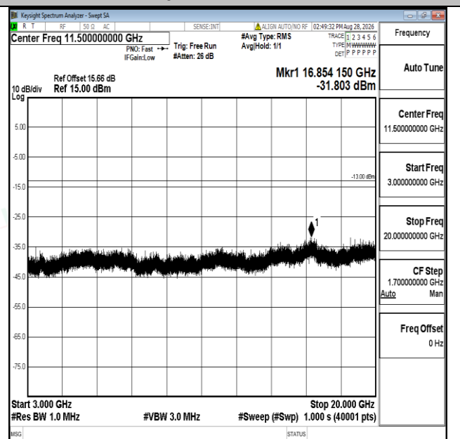
Band66-15MHz-16QAM-132047-1RB#0-3000~20000-PASS
