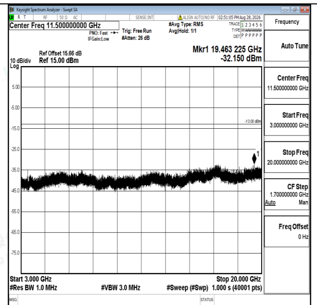
Band66-15MHz-16QAM-132322-1RB#0-3000~20000-PASS
