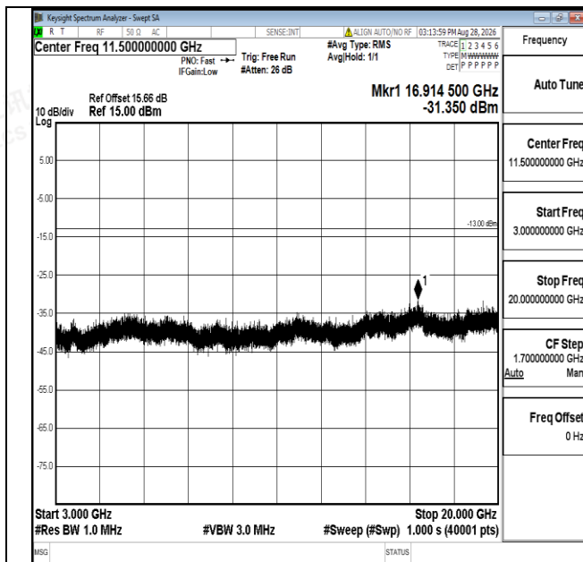
Band66-20MHz-QPSK-132572-1RB#0-3000~20000-PASS
