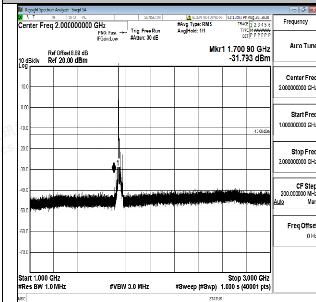
Band66-20MHz-16QAM-132322-1RB#0-1000~3000-PASS
