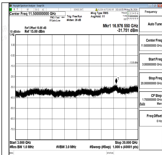
Band66-20MHz-QPSK-132072-1RB#0-3000~20000-PASS
