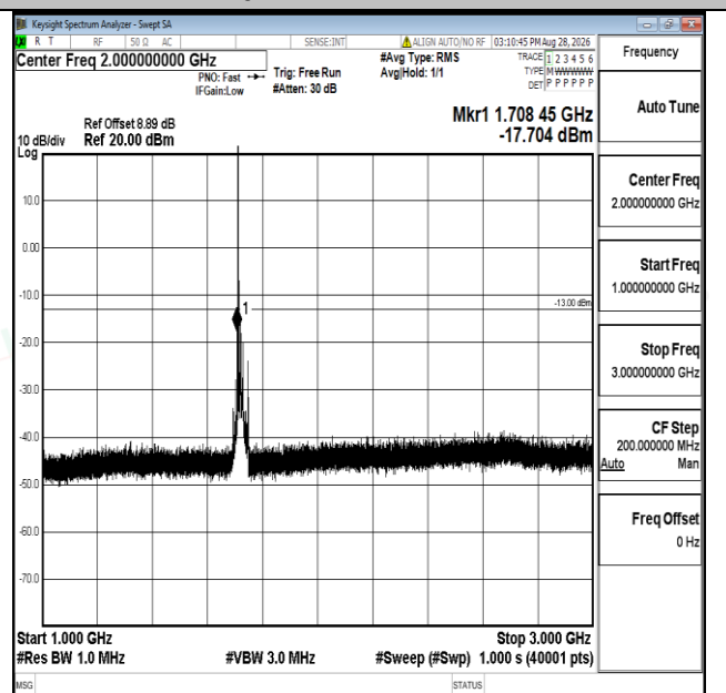
Band66-20MHz-QPSK-132072-1RB#0-1000~3000-PASS
