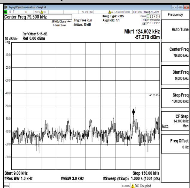
Band66-20MHz-16QAM-132322-1RB#0-0.009~0.15-PASS
