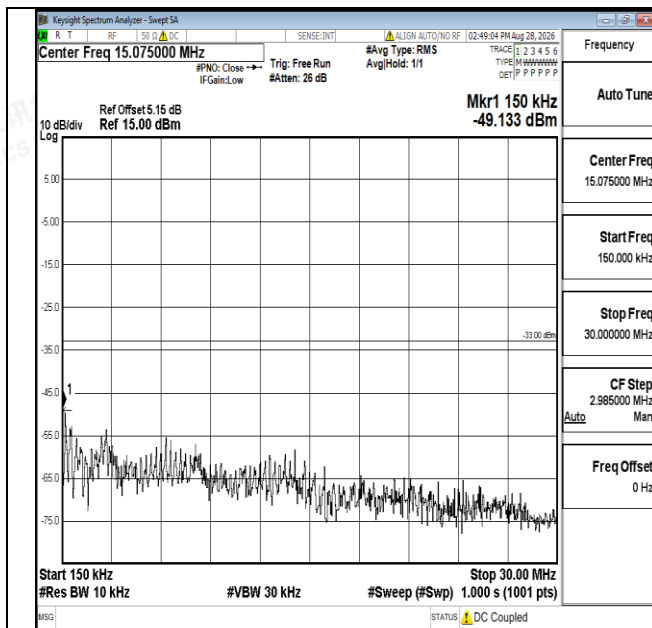
Band66-15MHz-16QAM-132047-1RB#0-0.15~30-PASS
