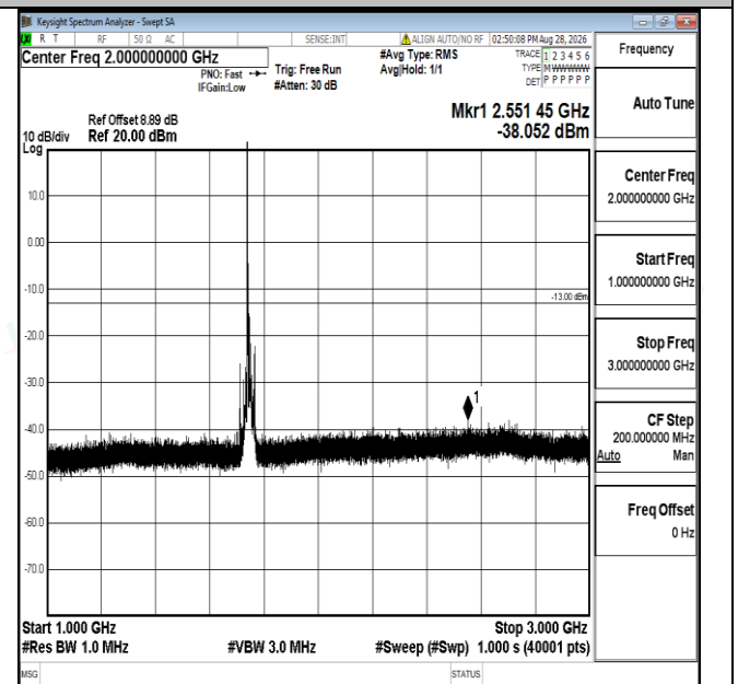
Band66-15MHz-QPSK-132322-1RB#0-1000~3000-PASS
