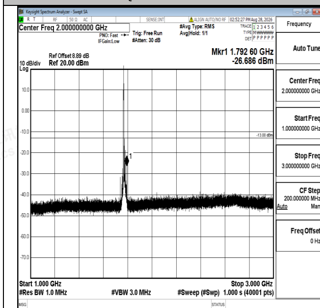
Band66-15MHz-16QAM-132597-1RB#0-1000~3000-PASS
