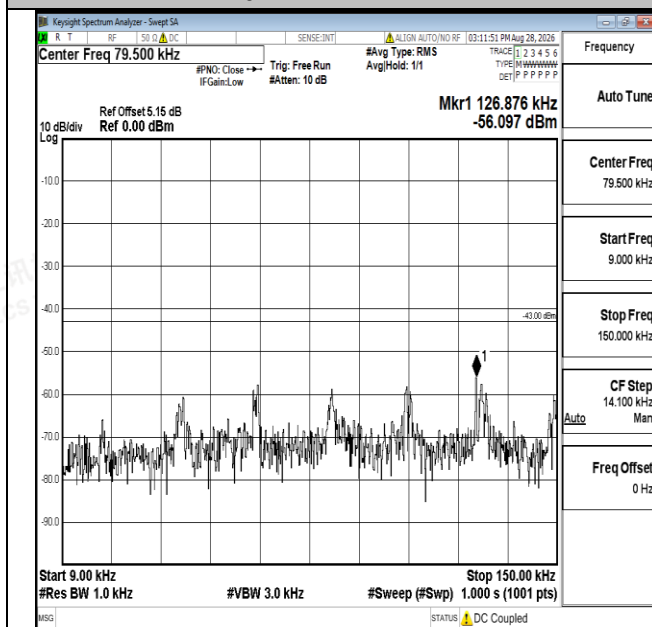
Band66-20MHz-QPSK-132322-1RB#0-0.009~0.15-PASS
