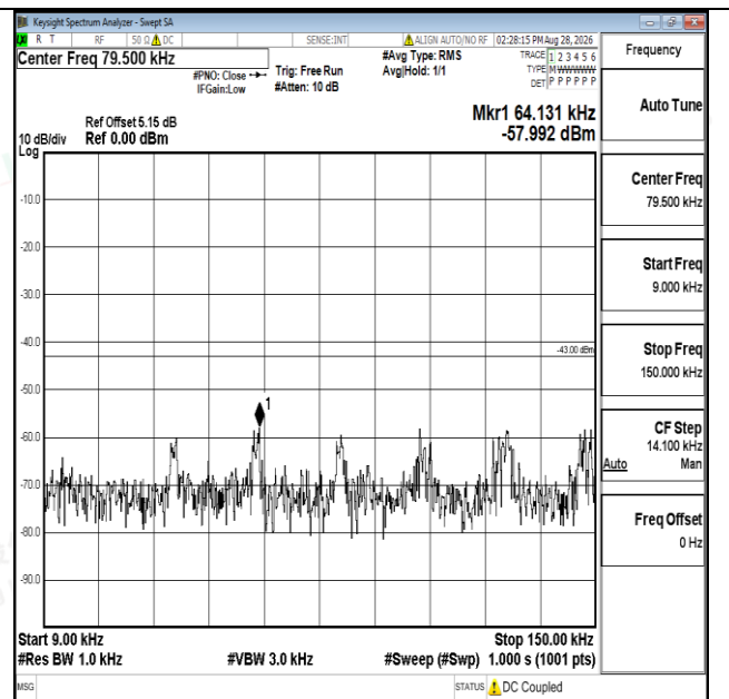
Band66-10MHz-16QAM-132622-1RB#0-0.009~0.15-PASS
