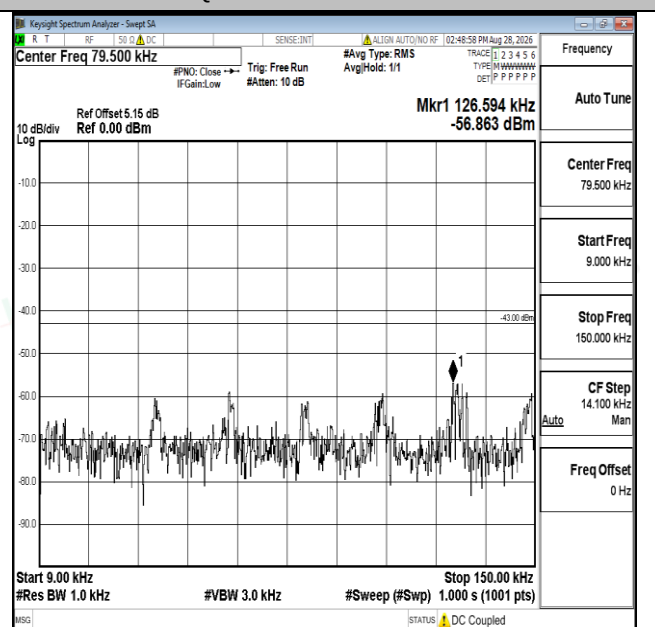
Band66-15MHz-16QAM-132047-1RB#0-0.009~0.15-PASS
