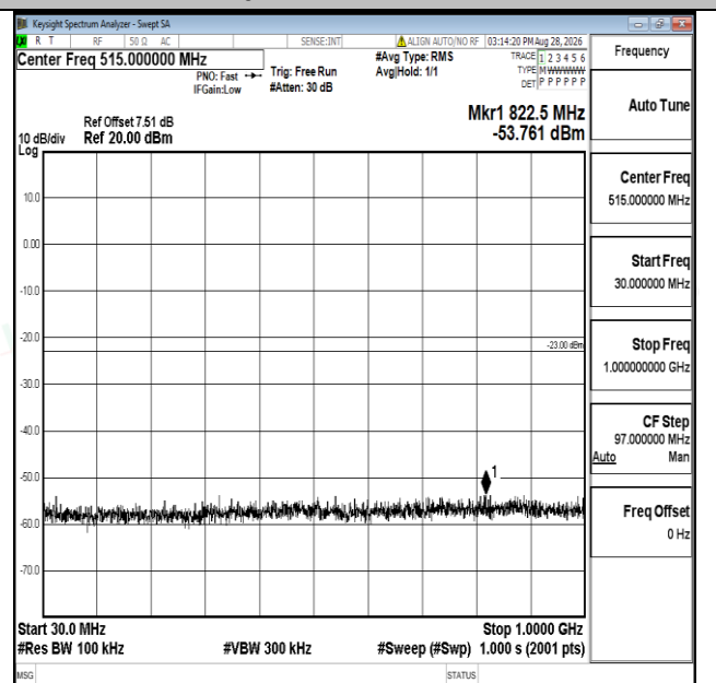
Band66-20MHz-16QAM-132572-1RB#0-30~1000-PASS
