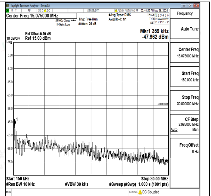
Band66-15MHz-QPSK-132322-1RB#0-0.15~30-PASS
