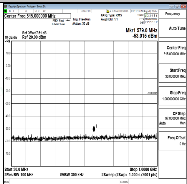
Band66-20MHz-16QAM-132072-1RB#0-30~1000-PASS
