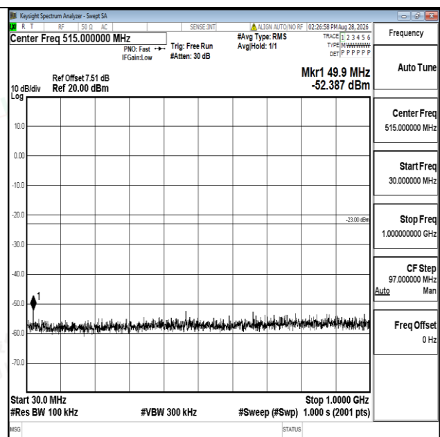
Band66-10MHz-16QAM-132322-1RB#0-30~1000-PASS
