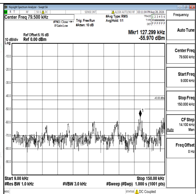
Band66-20MHz-16QAM-132072-1RB#0-0.009~0.15-PASS
