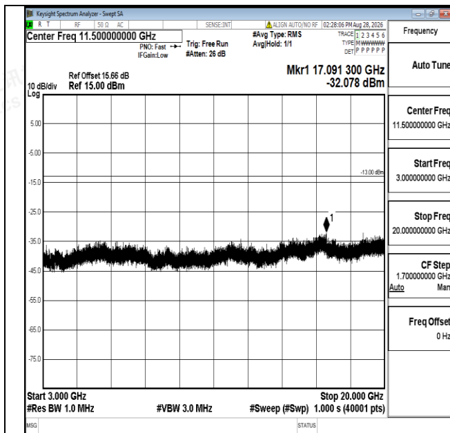
Band66-10MHz-QPSK-132622-1RB#0-3000~20000-PASS
