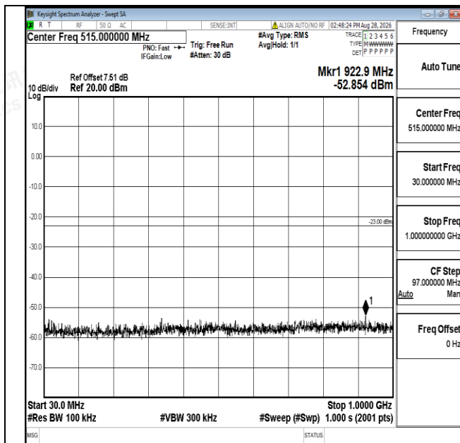
Band66-15MHz-QPSK-132047-1RB#0-30~1000-PASS
