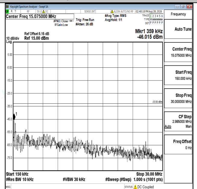
Band66-15MHz-QPSK-132047-1RB#0-0.15~30-PASS
