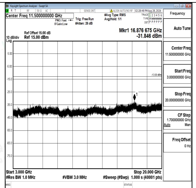
Band66-10MHz-16QAM-132622-1RB#0-3000~20000-PASS
