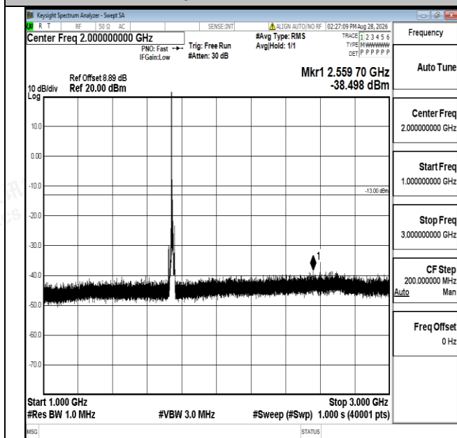
Band66-10MHz-16QAM-132322-1RB#0-1000~3000-PASS
