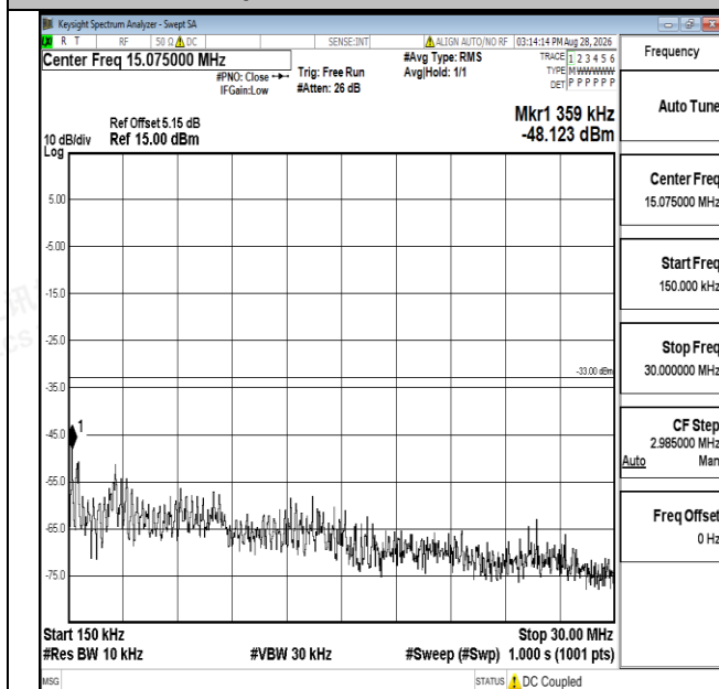
Band66-20MHz-16QAM-132572-1RB#0-0.15~30-PASS
