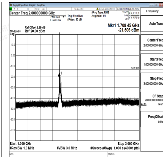
Band66-20MHz-16QAM-132072-1RB#0-1000~3000-PASS
