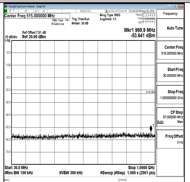
Band66-10MHz-16QAM-132622-1RB#0-30~1000-PASS
