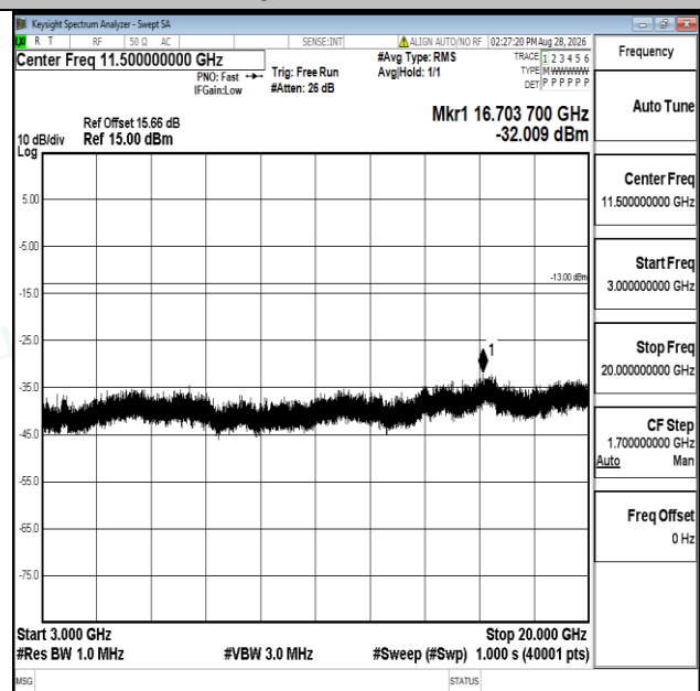
Band66-10MHz-16QAM-132322-1RB#0-3000~20000-PASS
