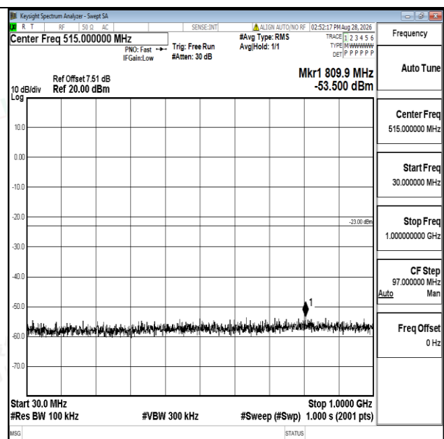
Band66-15MHz-16QAM-132597-1RB#0-30~1000-PASS
