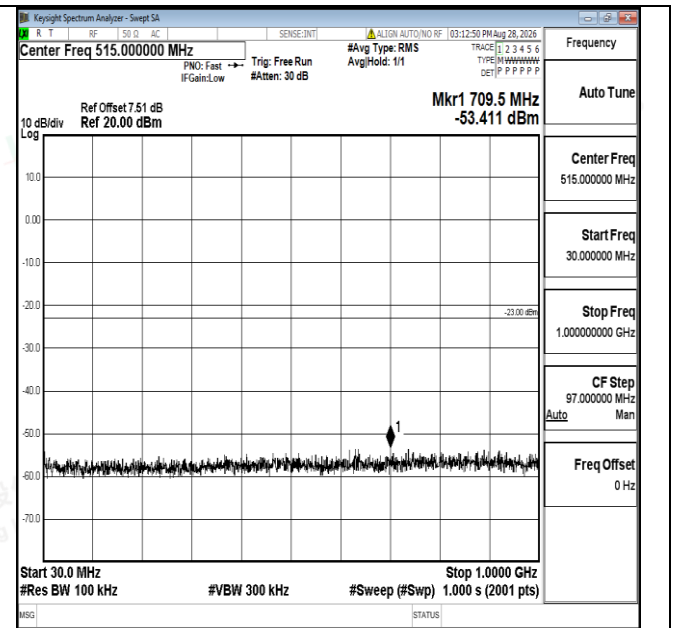
Band66-20MHz-16QAM-132322-1RB#0-30~1000-PASS
