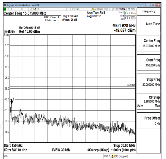
Band66-20MHz-QPSK-132072-1RB#0-0.15~30-PASS
