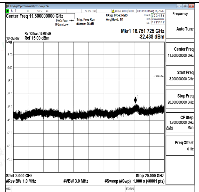
Band66-20MHz-16QAM-132072-1RB#0-3000~20000-PASS
