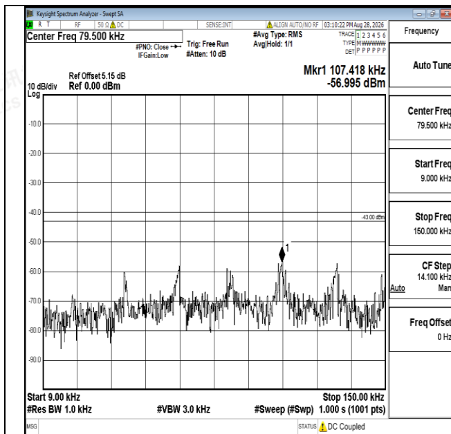
Band66-20MHz-QPSK-132072-1RB#0-0.009~0.15-PASS
