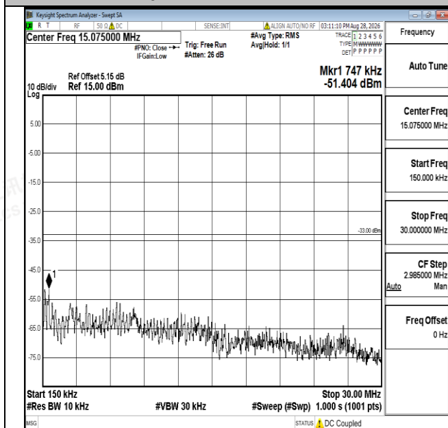
Band66-20MHz-16QAM-132072-1RB#0-0.15~30-PASS
