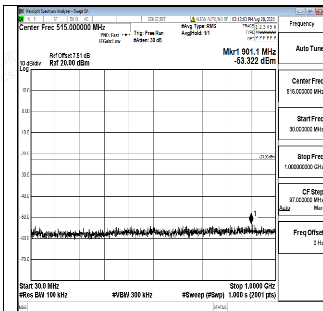
Band66-20MHz-QPSK-132322-1RB#0-30~1000-PASS
