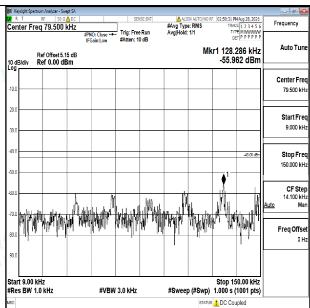
Band66-15MHz-16QAM-132322-1RB#0-0.009~0.15-PASS
