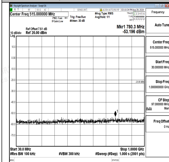
Band66-20MHz-QPSK-132072-1RB#0-30~1000-PASS
