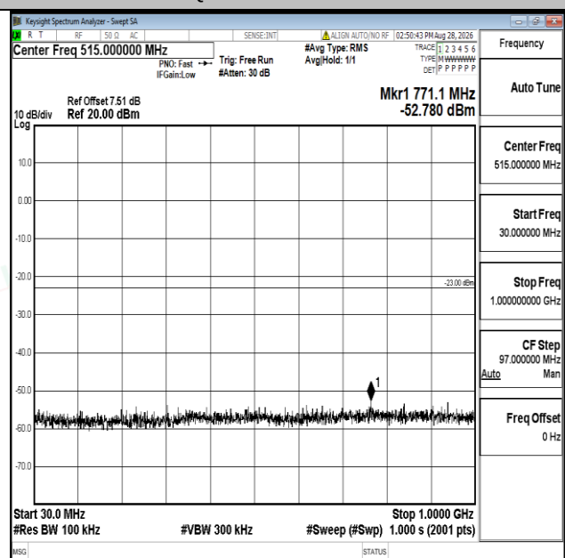
Band66-15MHz-16QAM-132322-1RB#0-30~1000-PASS
