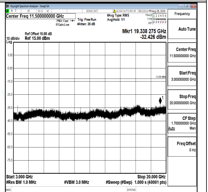
Band66-20MHz-16QAM-132322-1RB#0-3000~20000-PASS
