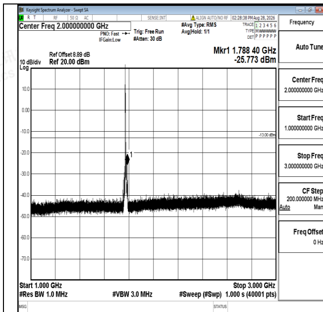
Band66-10MHz-16QAM-132622-1RB#0-1000~3000-PASS
