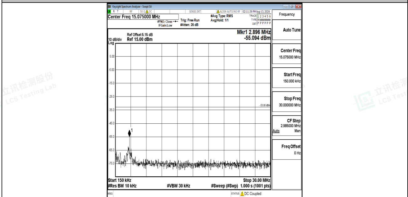
Band2-1.4MHz-QPSK-19193-1RB#0-0.15~30-PASS
