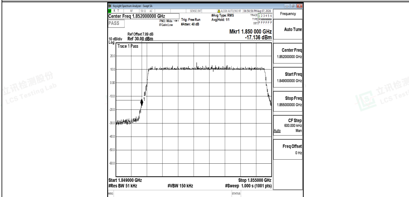
Band2-5MHz-16QAM-18625-25RB#0-PASS
