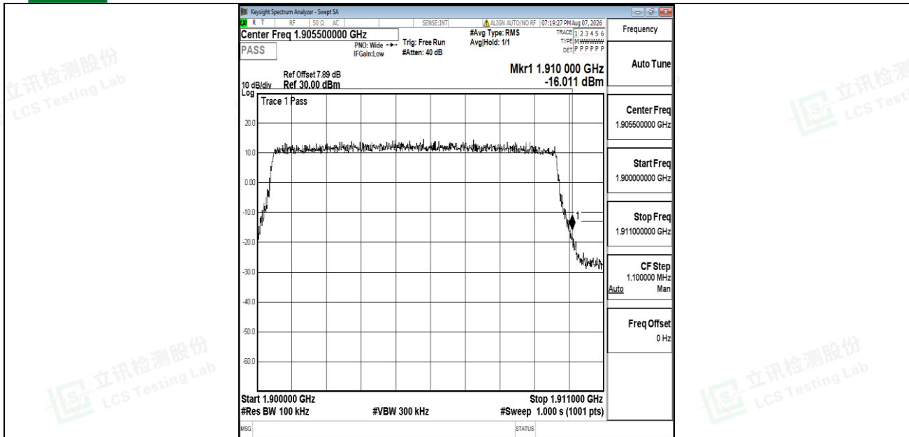
Band2-10MHz-QPSK-19150-50RB#0-PASS
