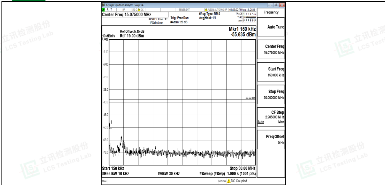
Band2-1.4MHz-16QAM-18900-1RB#0-0.15~30-PASS
