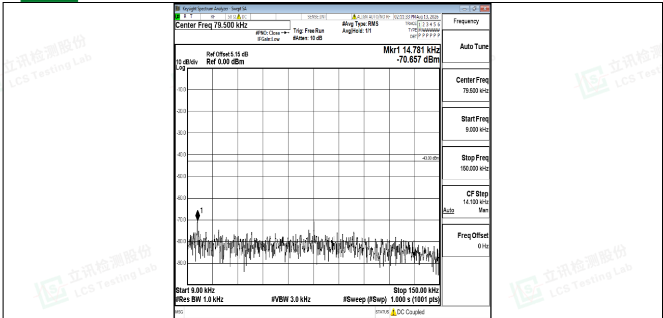
Band2-1.4MHz-QPSK-19193-1RB#0-0.009~0.15-PASS
