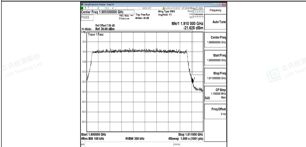
Band2-10MHz-16QAM-19150-50RB#0-PASS
