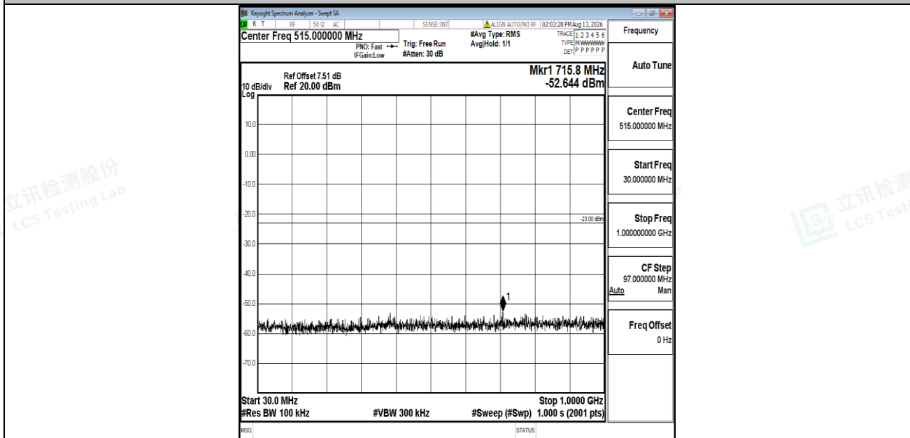
Band2-1.4MHz-16QAM-18900-1RB#0-30~1000-PASS
