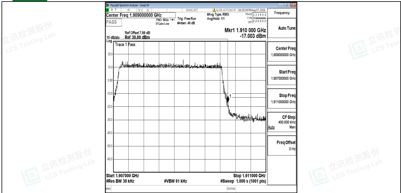
Band2-3MHz-QPSK-19185-15RB#0-PASS
