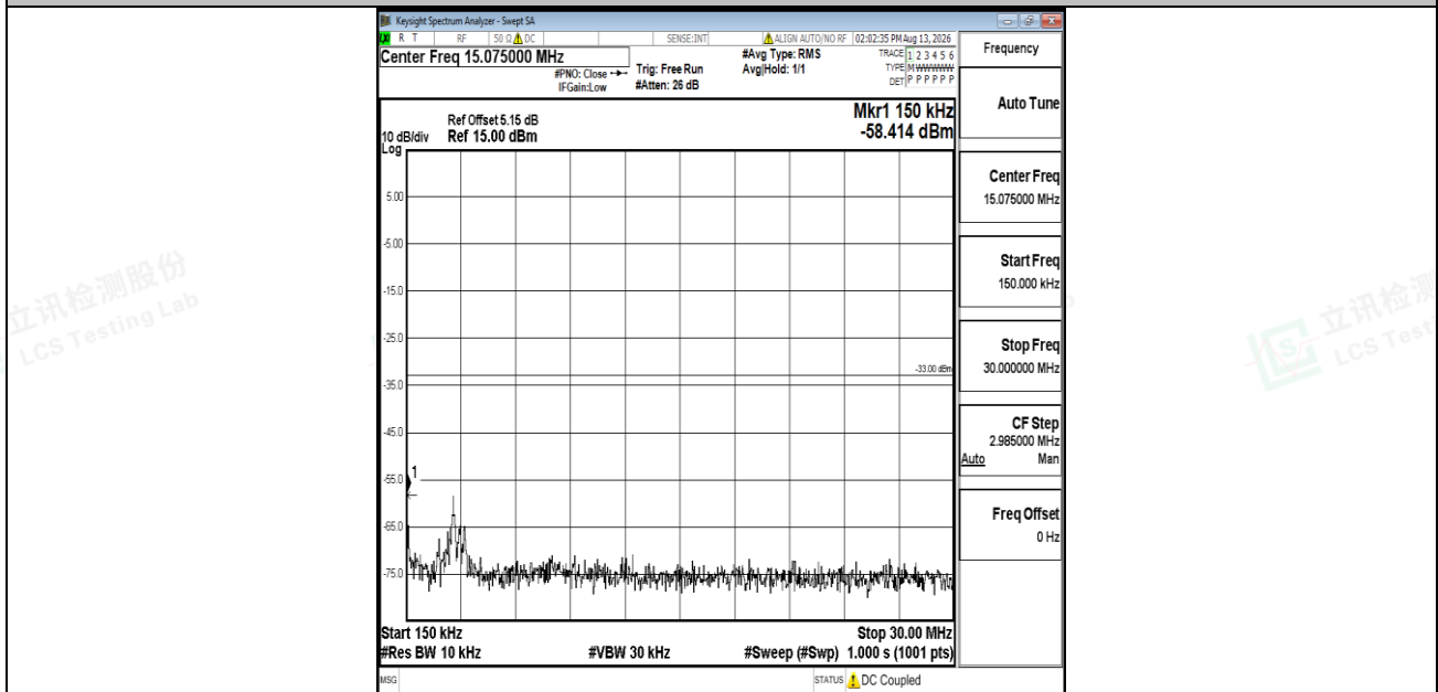
Band2-1.4MHz-QPSK-18900-1RB#0-0.15~30-PASS
