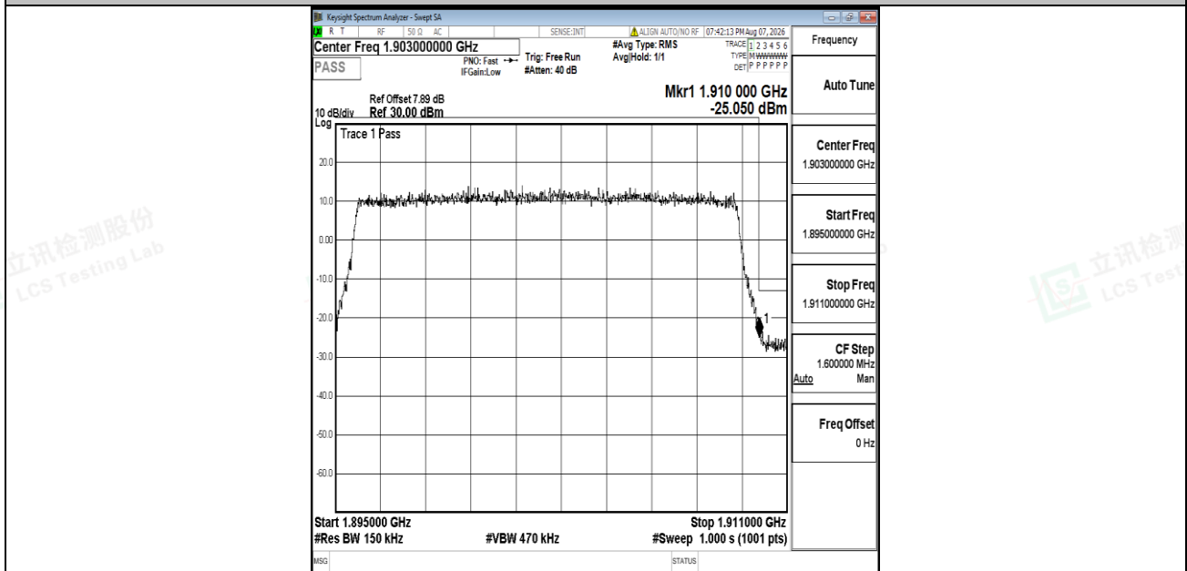
Band2-15MHz-16QAM-19125-75RB#0-PASS
