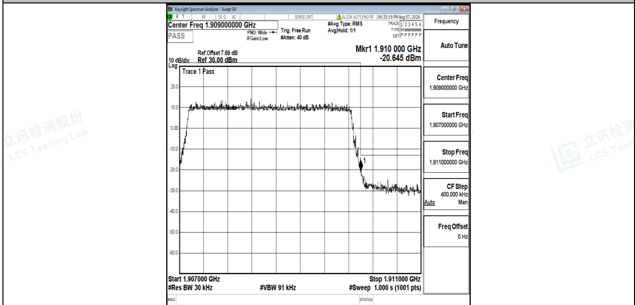
Band2-3MHz-16QAM-19185-15RB#0-PASS
