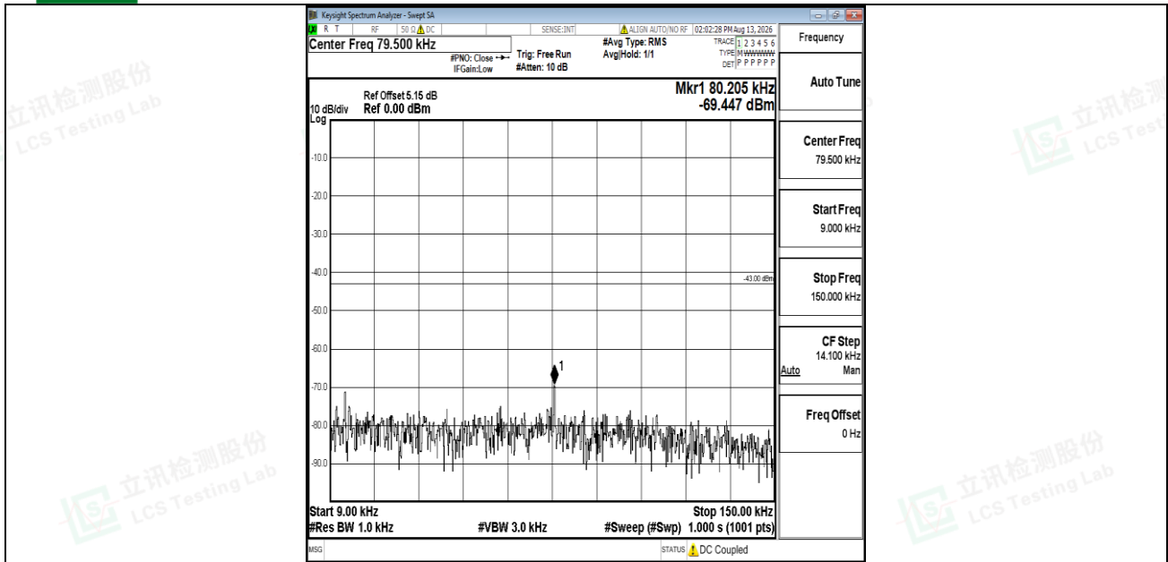
Band2-1.4MHz-QPSK-18900-1RB#0-0.009~0.15-PASS
