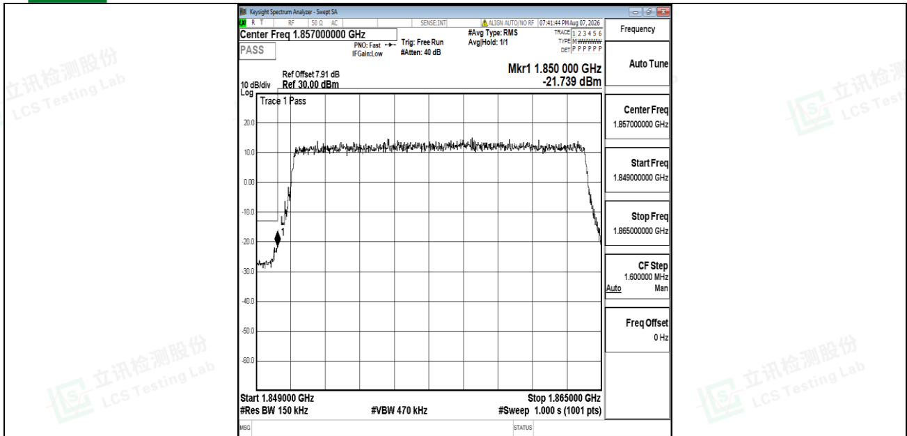
Band2-15MHz-QPSK-18675-75RB#0-PASS
