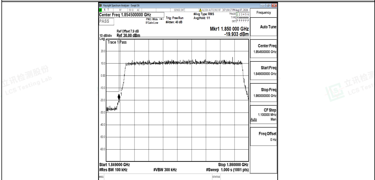
Band2-10MHz-16QAM-18650-50RB#0-PASS
