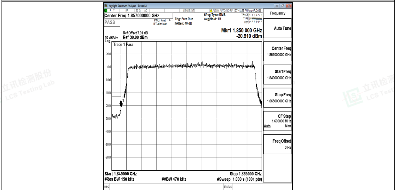
Band2-15MHz-16QAM-18675-75RB#0-PASS
