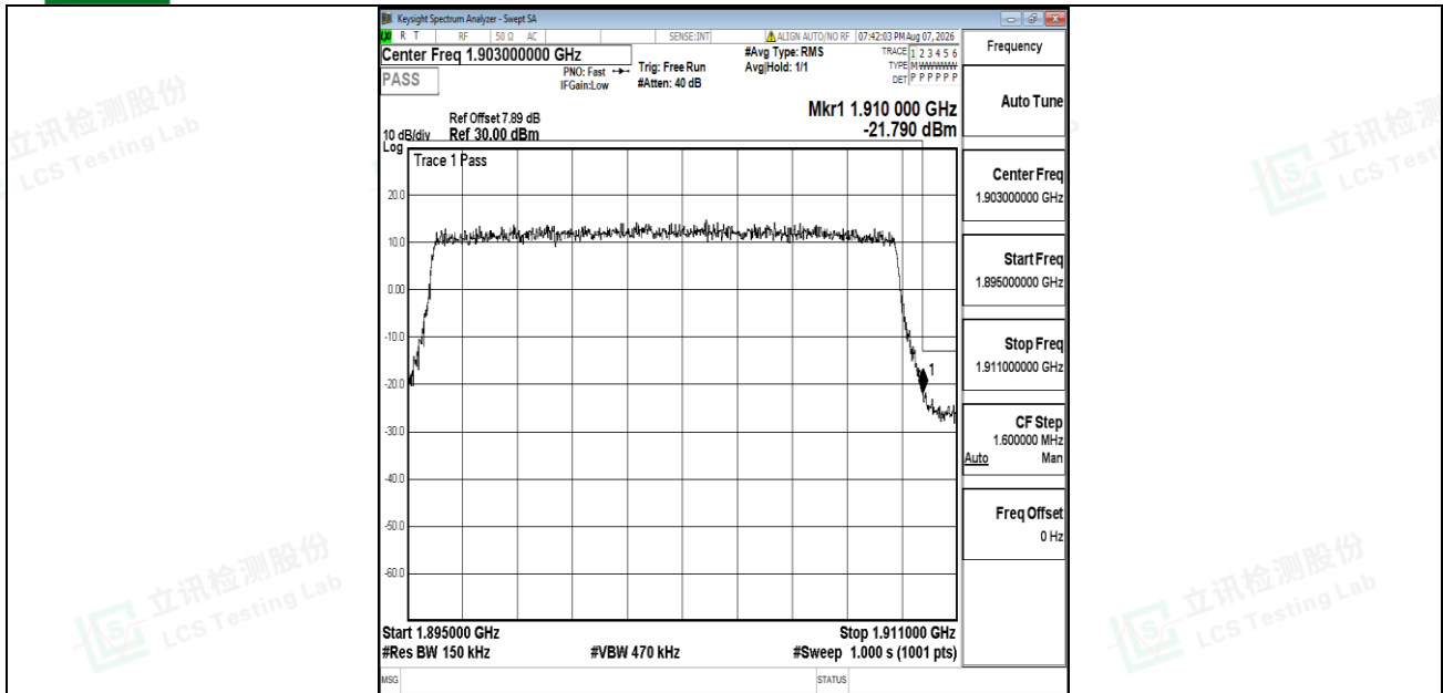
Band2-15MHz-QPSK-19125-75RB#0-PASS
