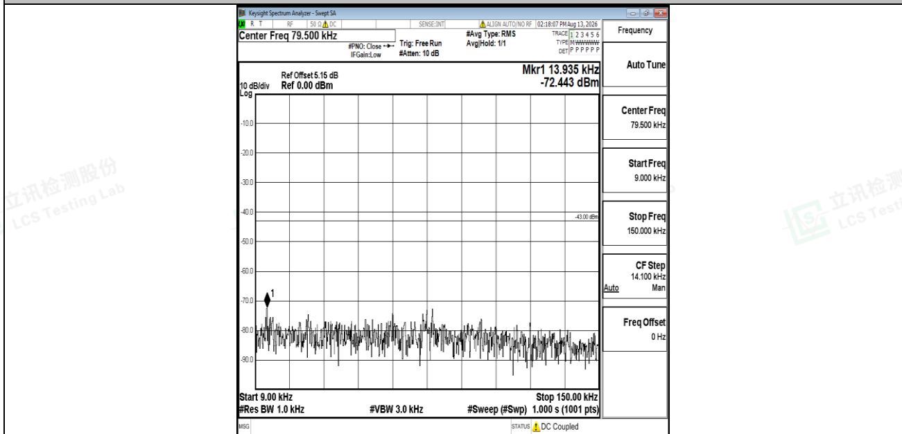
Band2-3MHz-16QAM-19185-1RB#0-0.009~0.15-PASS
