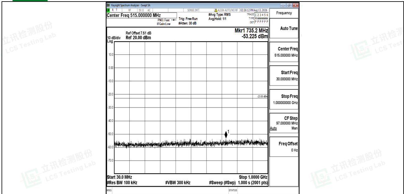
Band2-10MHz-QPSK-18650-1RB#0-30~1000-PASS
