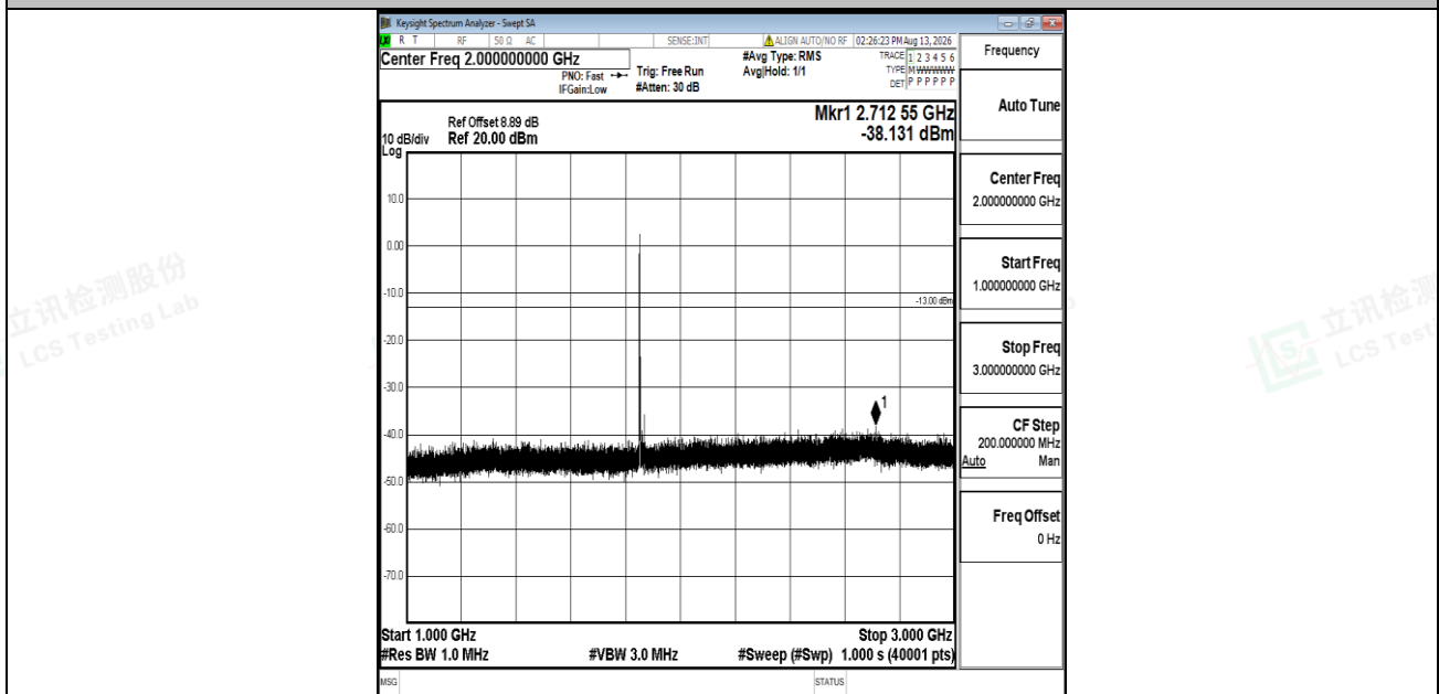
Band2-10MHz-QPSK-18650-1RB#0-1000~3000-PASS
