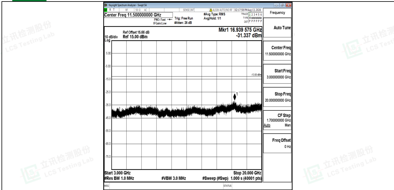
Band2-3MHz-QPSK-19185-1RB#0-3000~20000-PASS
