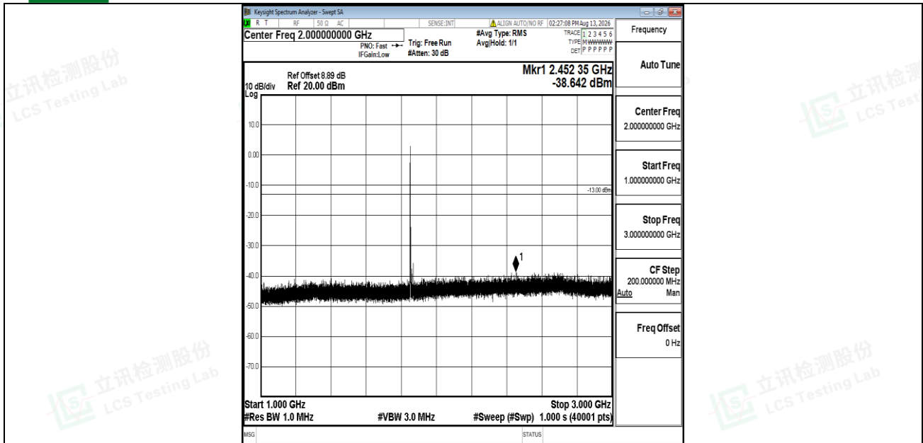
Band2-10MHz-16QAM-18650-1RB#0-1000~3000-PASS
