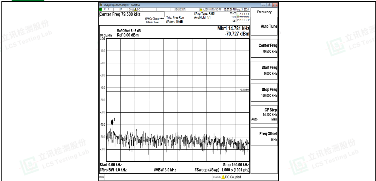
Band2-20MHz-QPSK-18900-1RB#0-0.009~0.15-PASS
