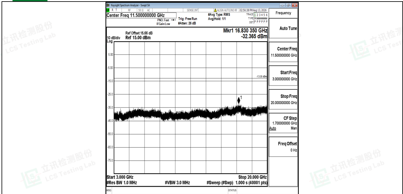
Band2-20MHz-QPSK-18700-1RB#0-3000~20000-PASS
