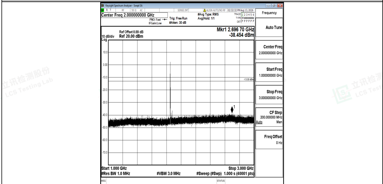
Band2-15MHz-QPSK-18675-1RB#0-1000~3000-PASS
