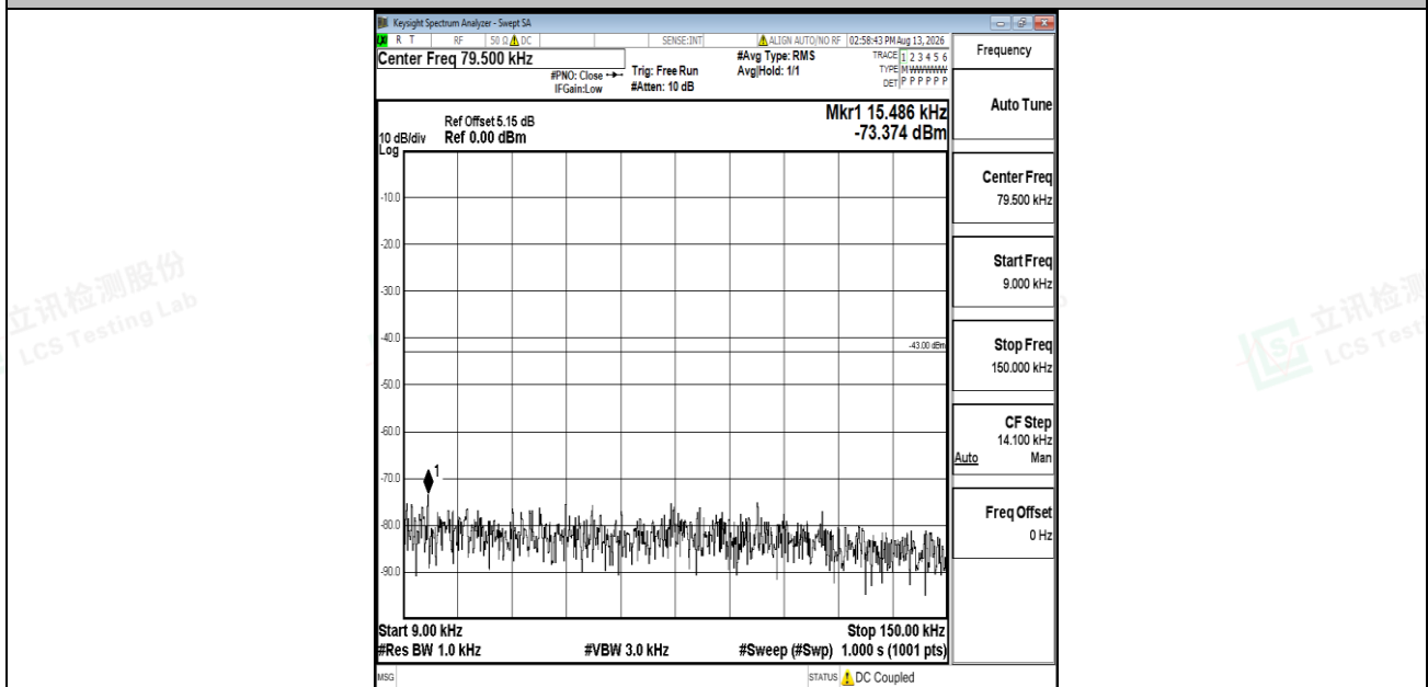
Band2-20MHz-16QAM-18900-1RB#0-0.009~0.15-PASS
