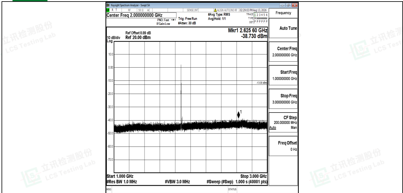
Band2-10MHz-16QAM-18900-1RB#0-1000~3000-PASS
