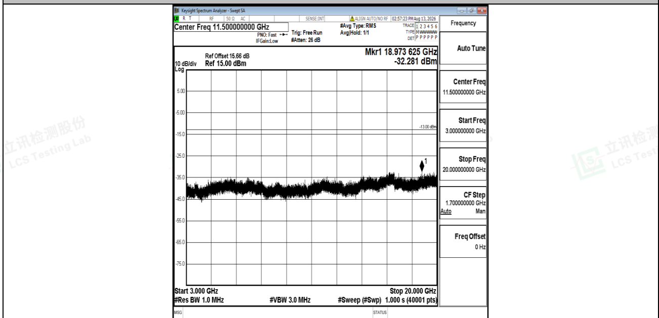
Band2-20MHz-16QAM-18700-1RB#0-3000~20000-PASS
