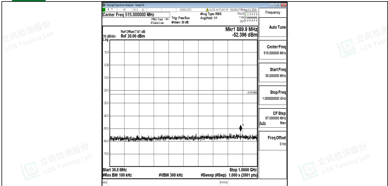
Band2-15MHz-QPSK-19125-1RB#0-30~1000-PASS
