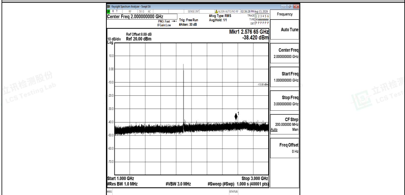
Band2-15MHz-QPSK-19125-1RB#0-1000~3000-PASS
