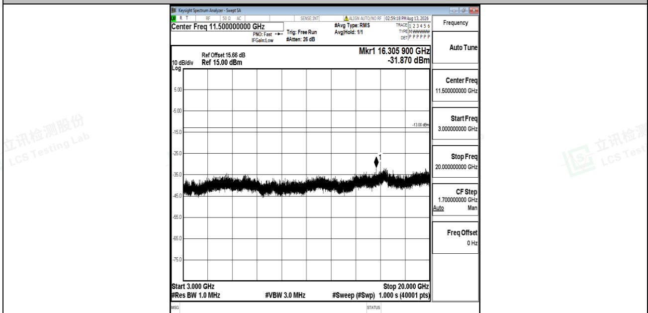
Band2-20MHz-16QAM-18900-1RB#0-3000~20000-PASS
