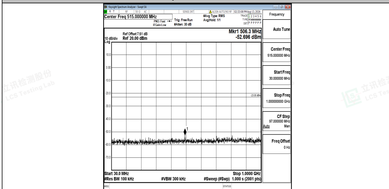
Band2-15MHz-16OAM-18675-1RB#0-30~1000-PASS
