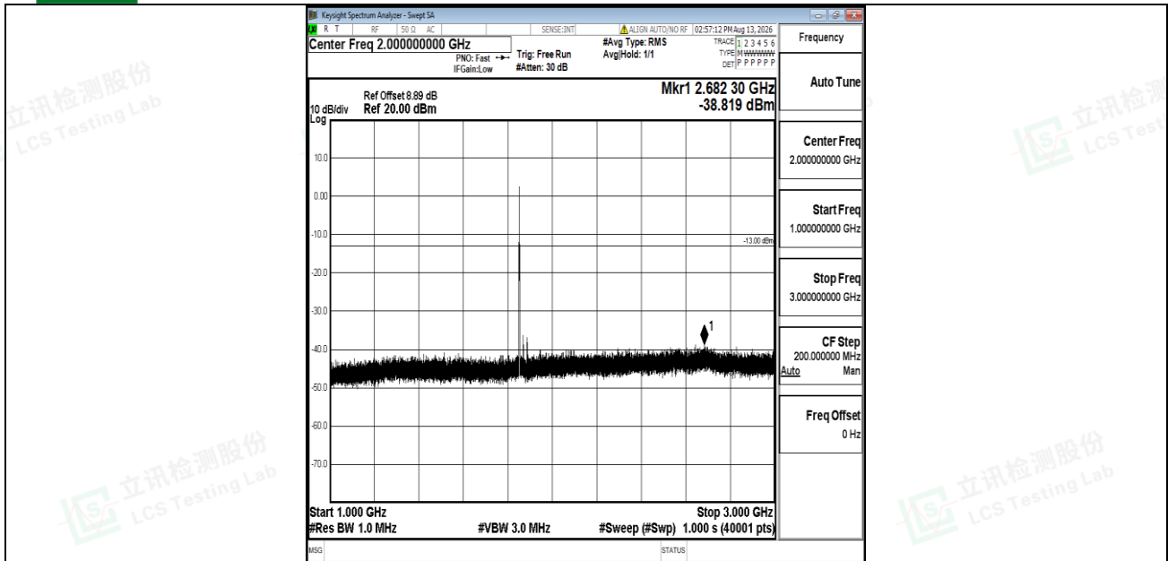
Band2-20MHz-16QAM-18700-1RB#0-1000~3000-PASS
