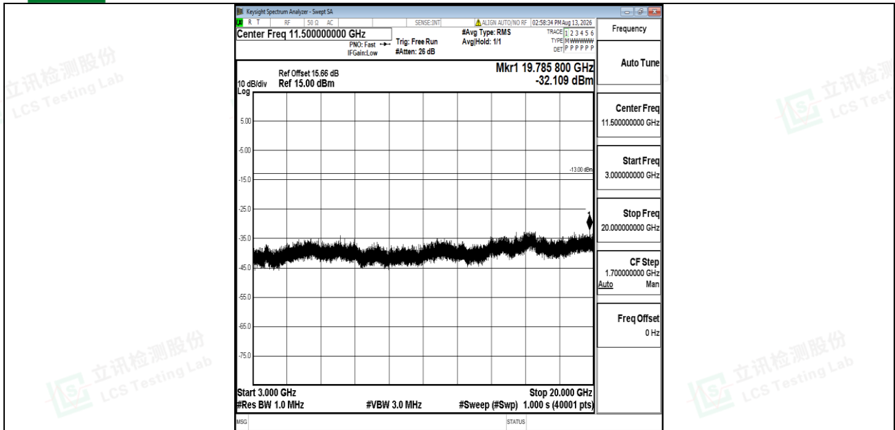
Band2-20MHz-QPSK-18900-1RB#0-3000~20000-PASS
