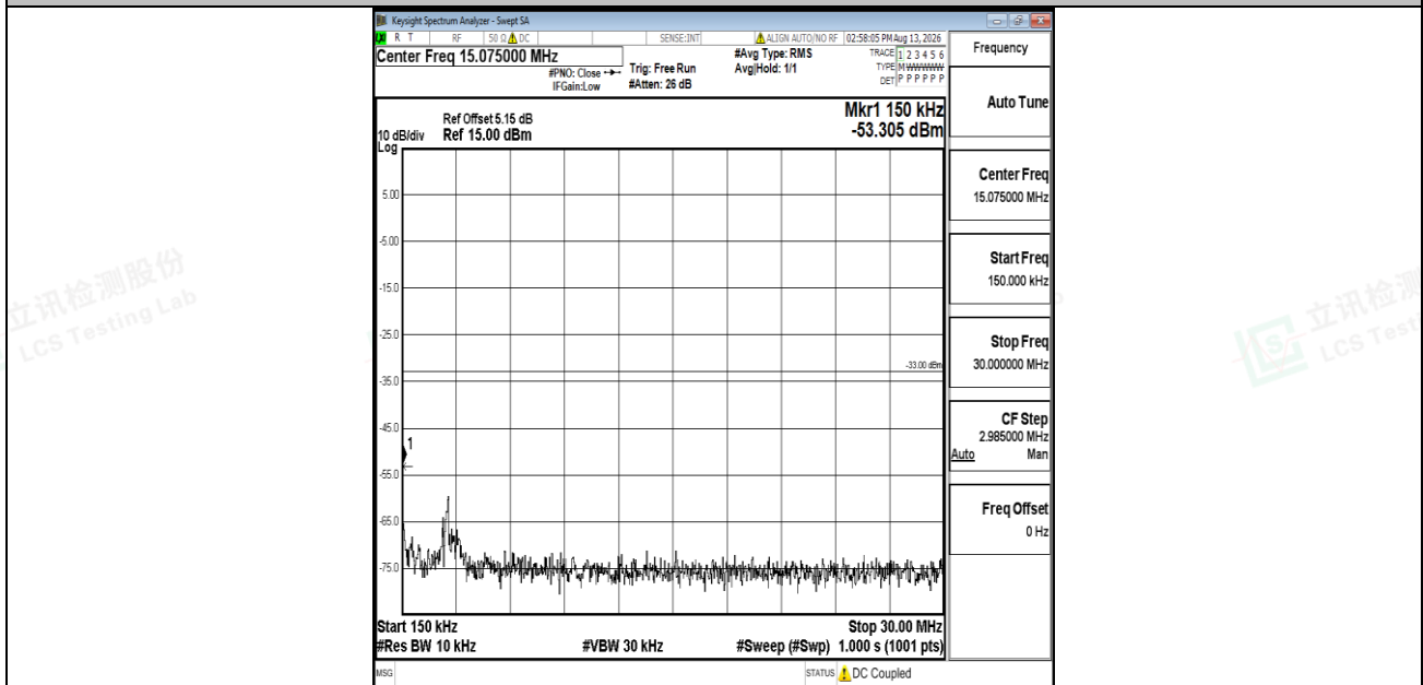
Band2-20MHz-QPSK-18900-1RB#0-0.15~30-PASS
