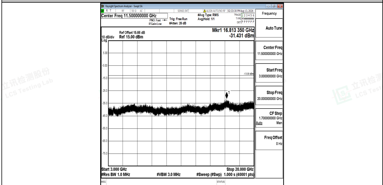
Band2-15MHz-16QAM-18675-1RB#0-3000~20000-PASS
