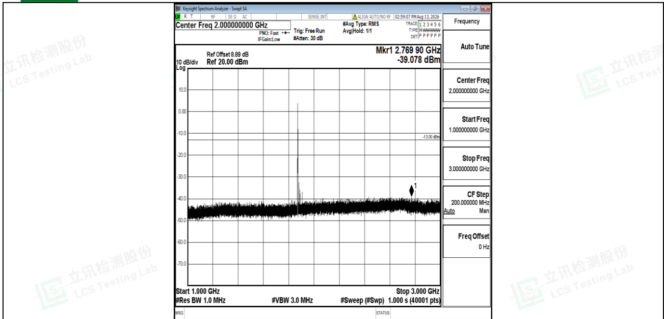
Band2-20MHz-16QAM-18900-1RB#0-1000~3000-PASS
