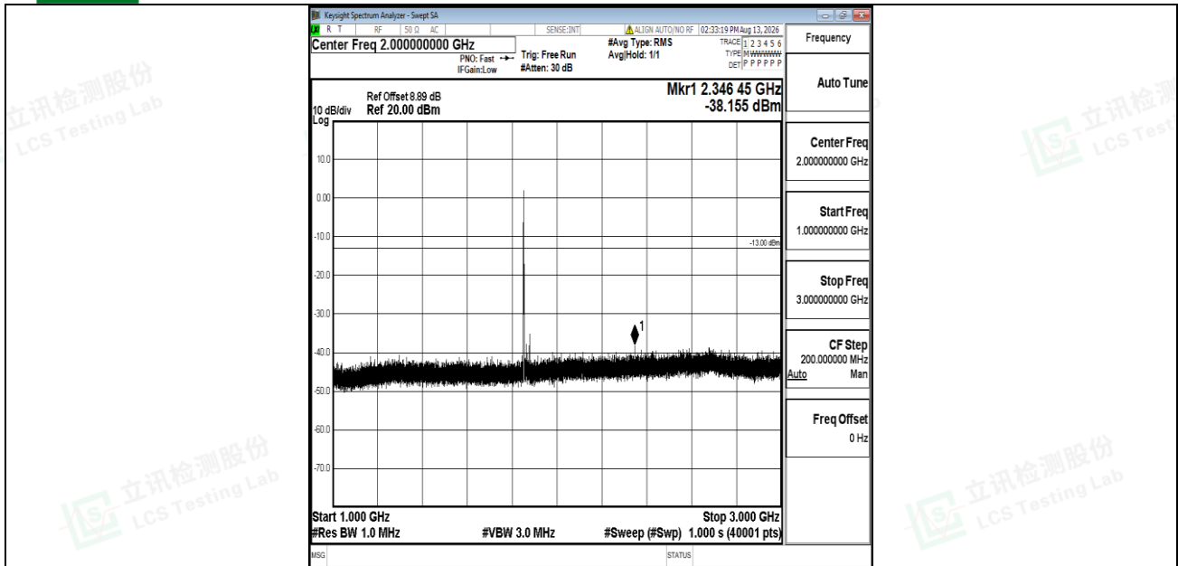
Band2-15MHz-16QAM-18675-1RB#0-1000~3000-PASS
