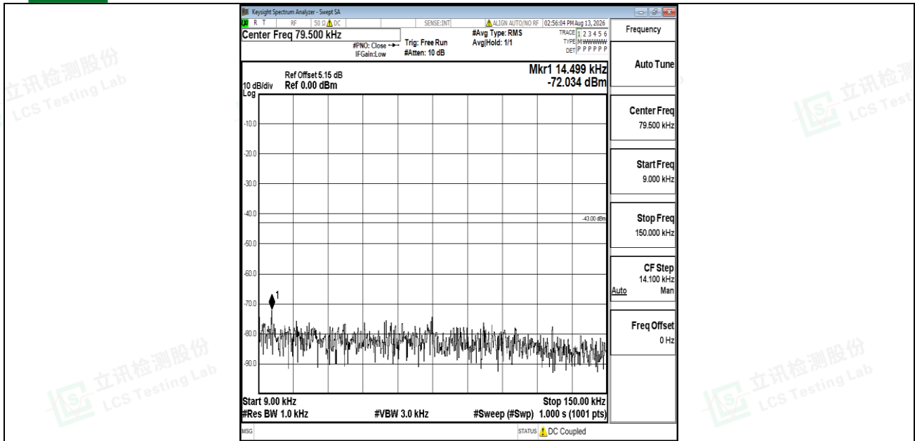
Band2-20MHz-QPSK-18700-1RB#0-0.009~0.15-PASS
