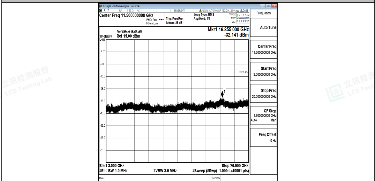
Band2-10MHz-16QAM-18900-1RB#0-3000~20000-PASS
