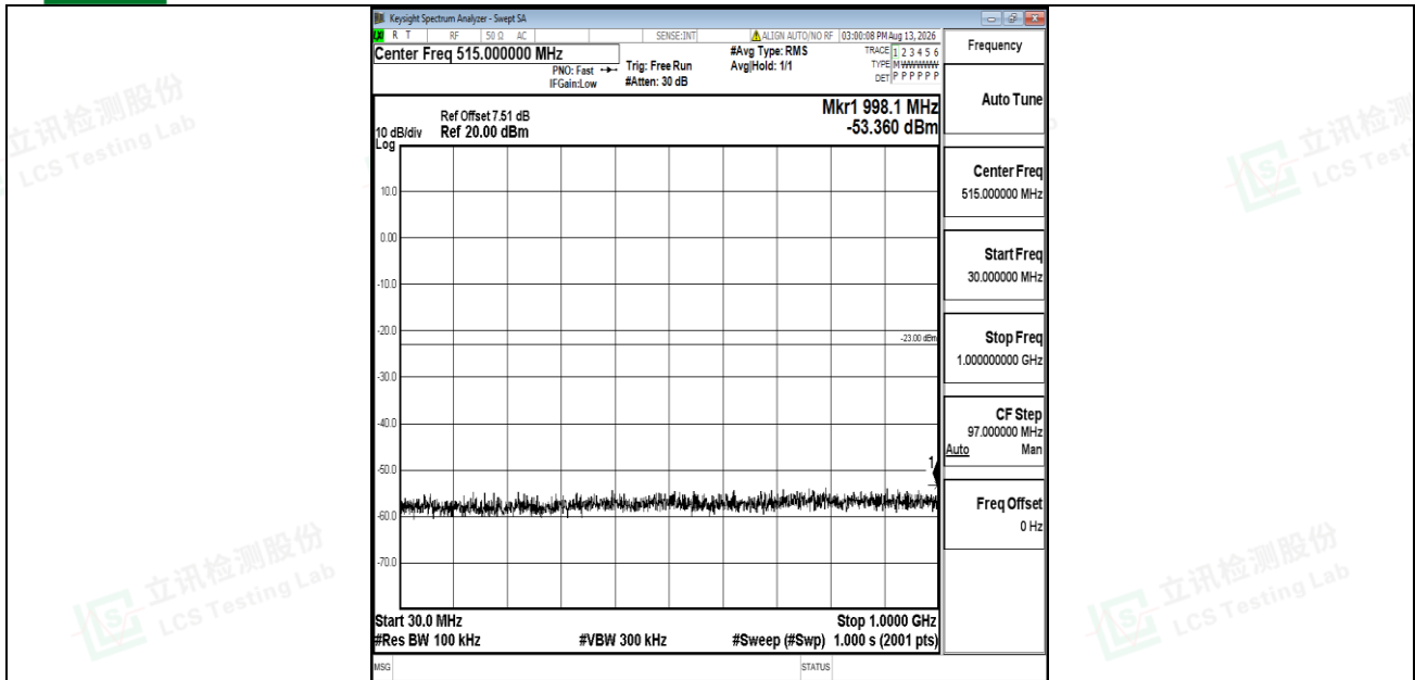
Band2-20MHz-QPSK-19100-1RB#0-30~1000-PASS
