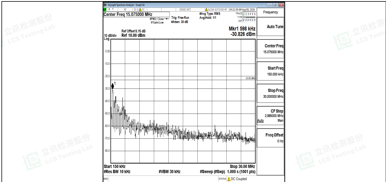
Band5-1.4MHz-16QAM-20643-1RB#0-0.15~30-PASS
