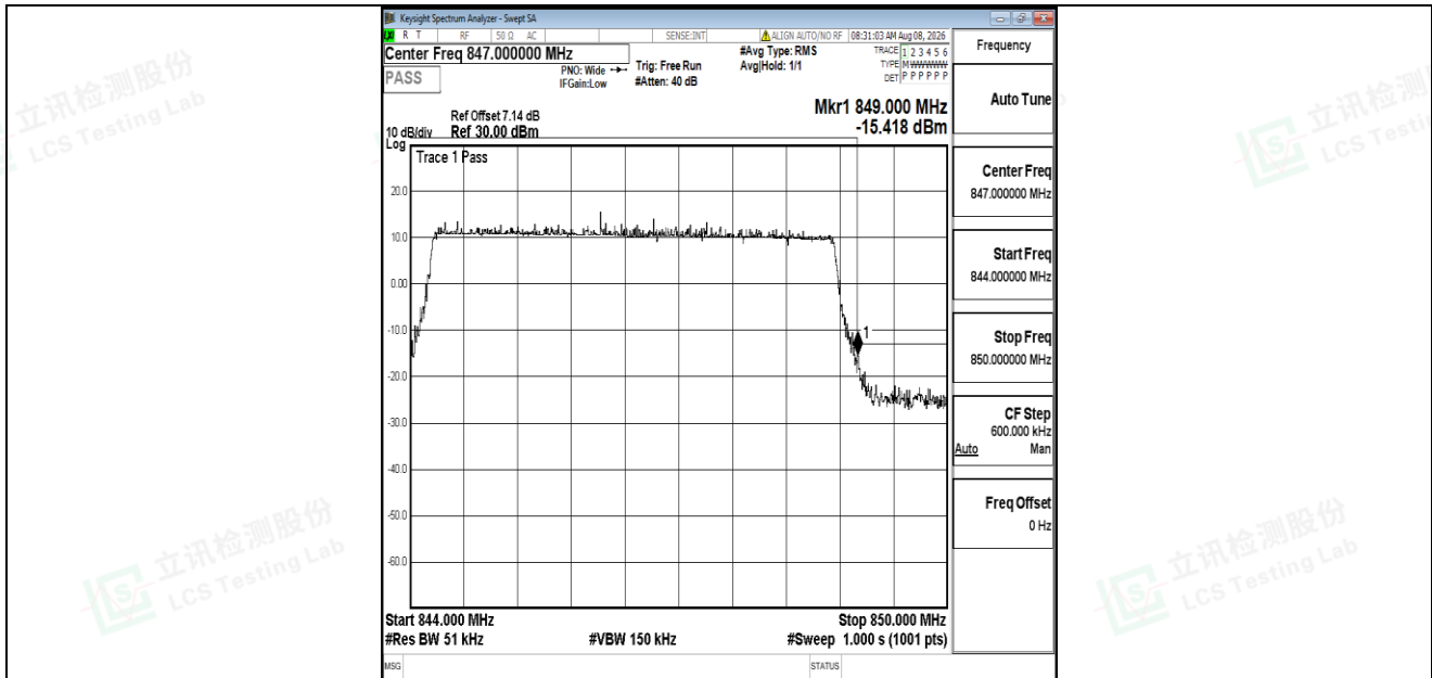
Band5-5MHz-16QAM-20625-25RB#0-PASS
