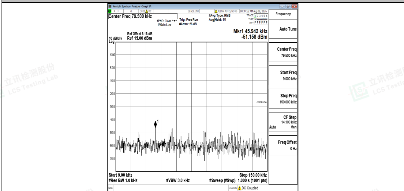
Band5-5MHz-16QAM-20425-1RB#0-0.009~0.15-PASS
