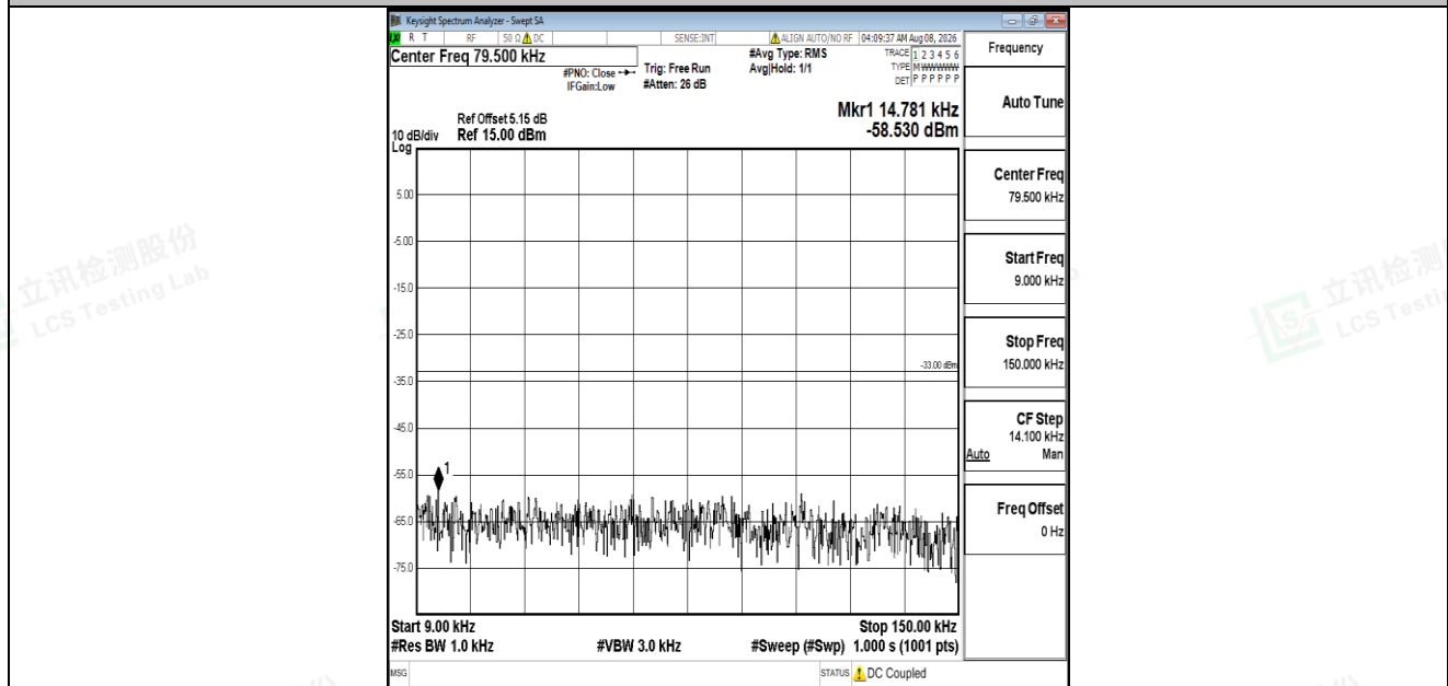
Band5-1.4MHz-16QAM-20525-1RB#0-0.009~0.15-PASS
