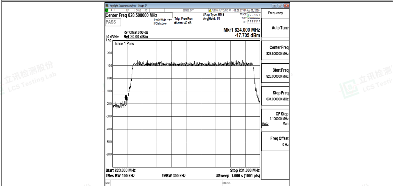
Band5-10MHz-QPSK-20450-50RB#0-PASS
