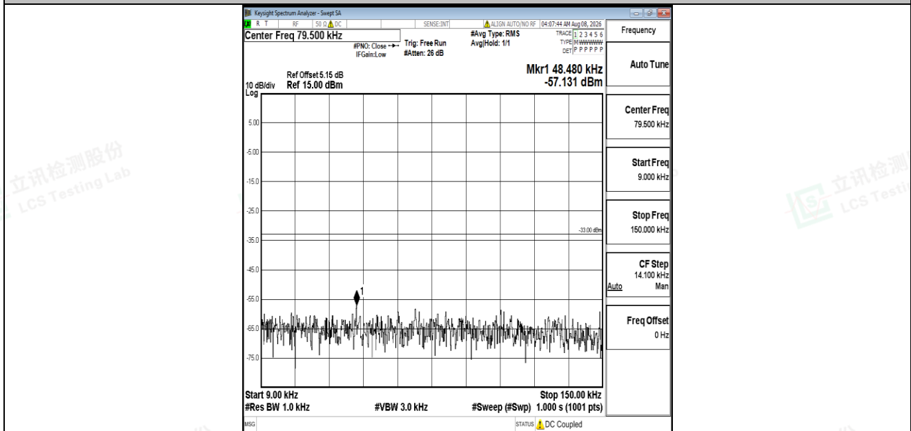
Band5-1.4MHz-16QAM-20407-1RB#0-0.009~0.15-PASS
