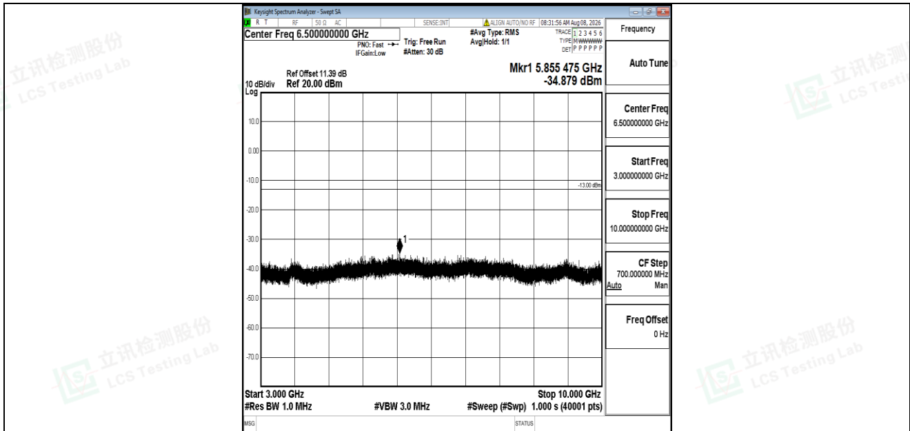
Band5-5MHz-QPSK-20425-1RB#0-3000~10000-PASS
