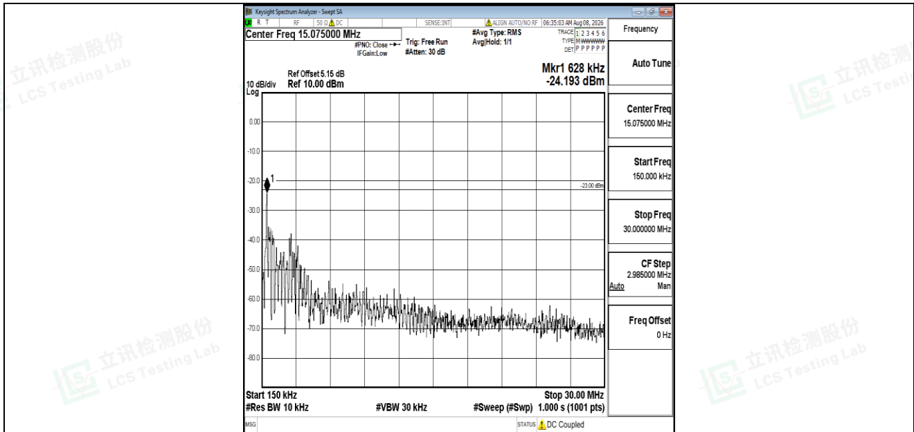
Band5-3MHz-16QAM-20525-1RB#0-0.15~30-PASS
