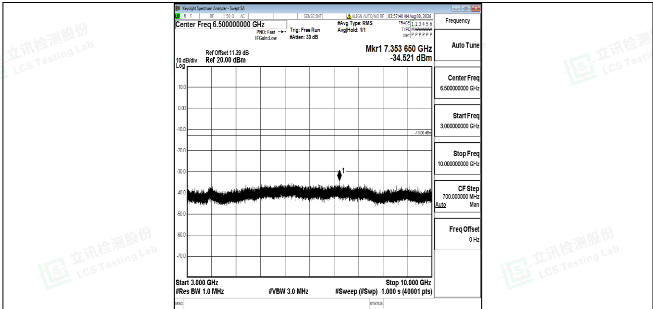
Band5-1.4MHz-QPSK-20407-1RB#0-3000~10000-PASS
