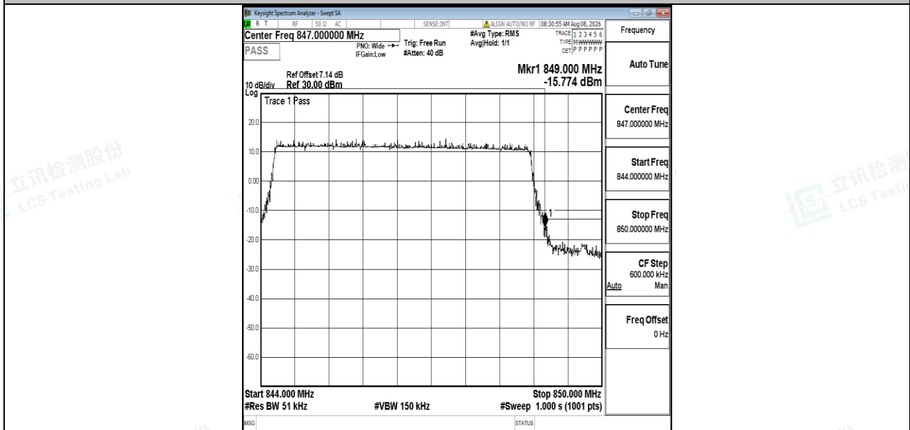
Band5-5MHz-QPSK-20625-25RB#0-PASS
