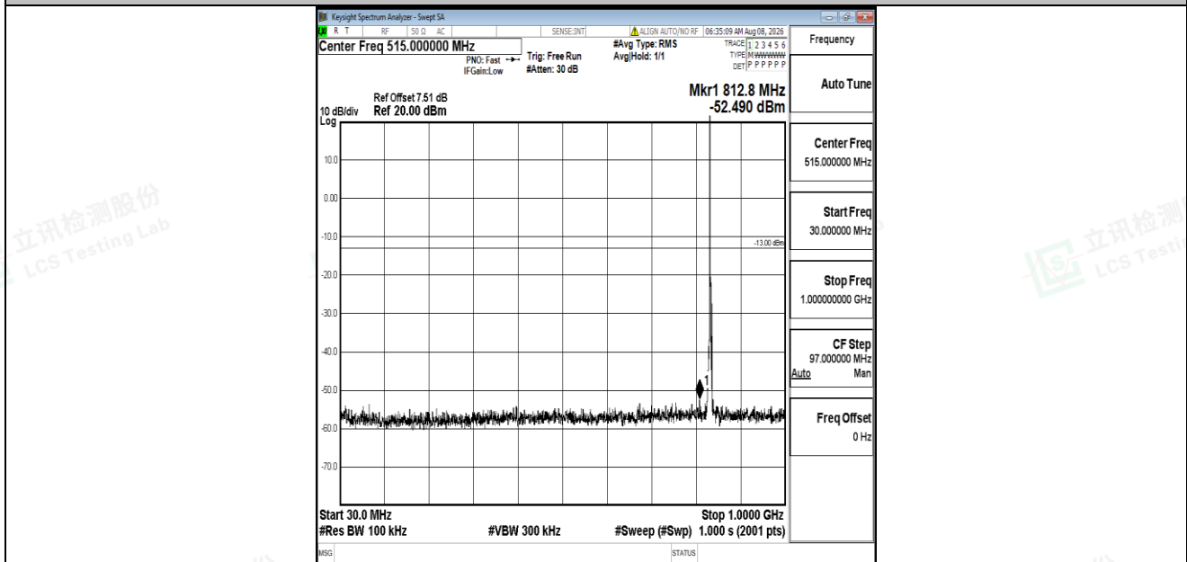
Band5-3MHz-16QAM-20525-1RB#0-30~1000-PASS
