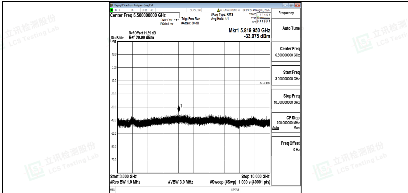
Band5-1.4MHz-QPSK-20525-1RB#0-3000~10000-PASS
