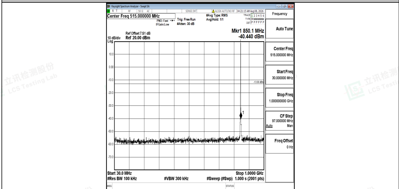
Band5-1.4MHz-16QAM-20643-1RB#0-30~1000-PASS
