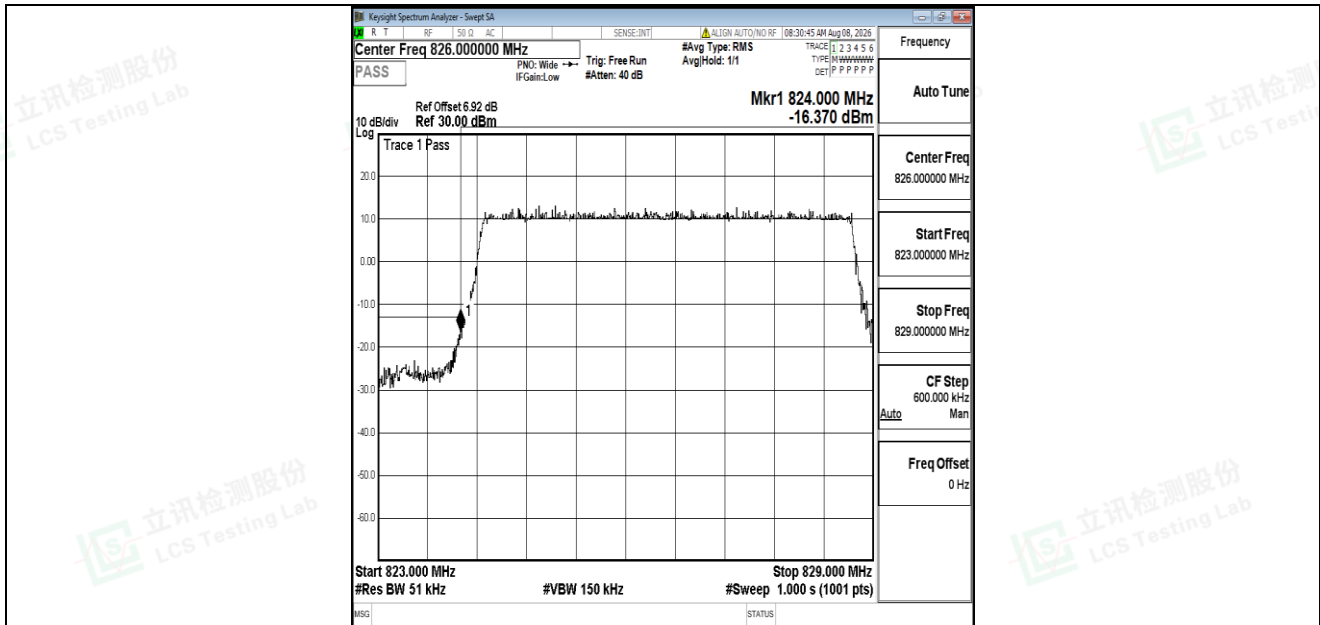
Band5-5MHz-16QAM-20425-25RB#0-PASS
