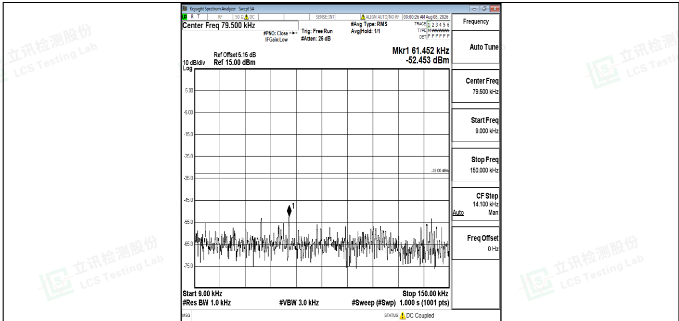
Band5-10MHz-QPSK-20525-1RB#0-0.009~0.15-PASS
