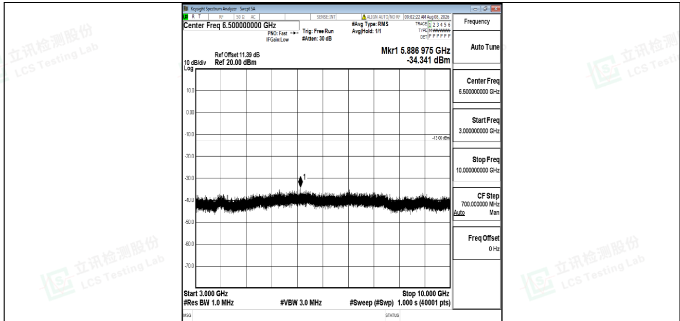
Band5-10MHz-QPSK-20600-1RB#0-3000~10000-PASS
