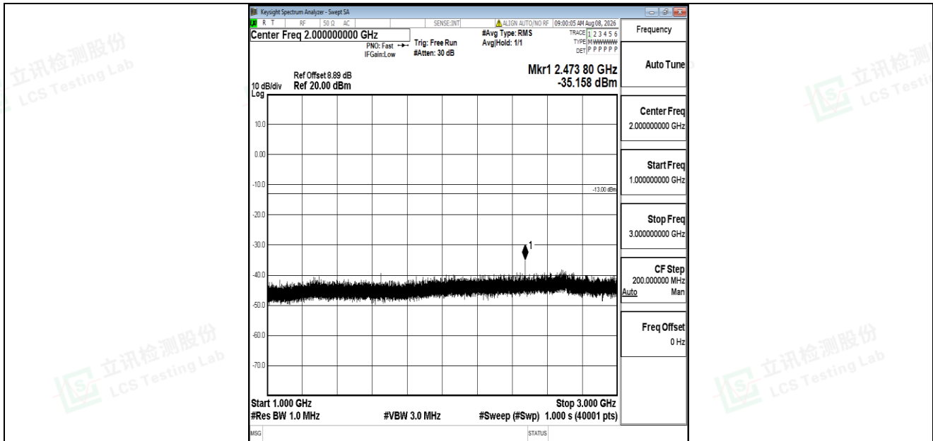
Band5-10MHz-16QAM-20450-1RB#0-1000~3000-PASS
