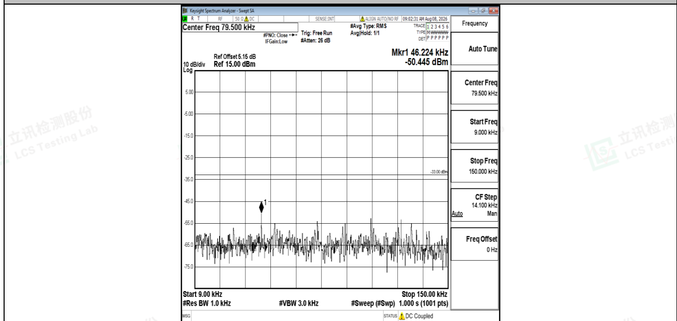
Band5-10MHz-16QAM-20600-1RB#0-0.009~0.15-PASS
