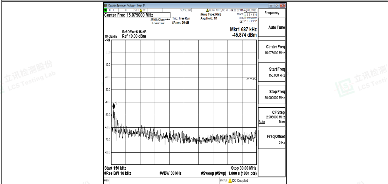
Band5-10MHz-QPSK-20525-1RB#0-0.15~30-PASS
