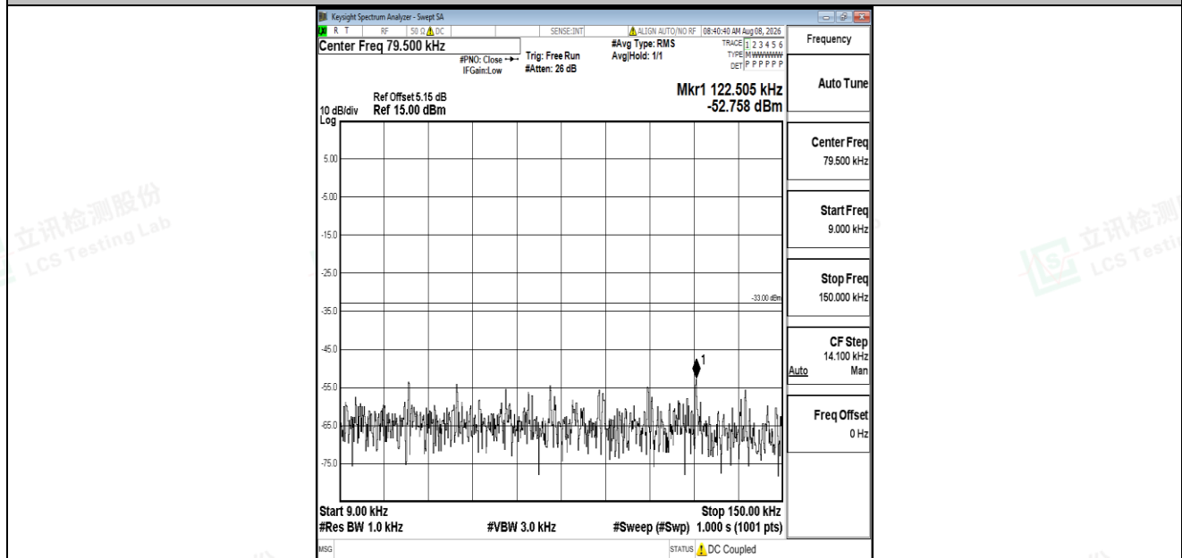
Band5-5MHz-16QAM-20625-1RB#0-0.009~0.15-PASS
