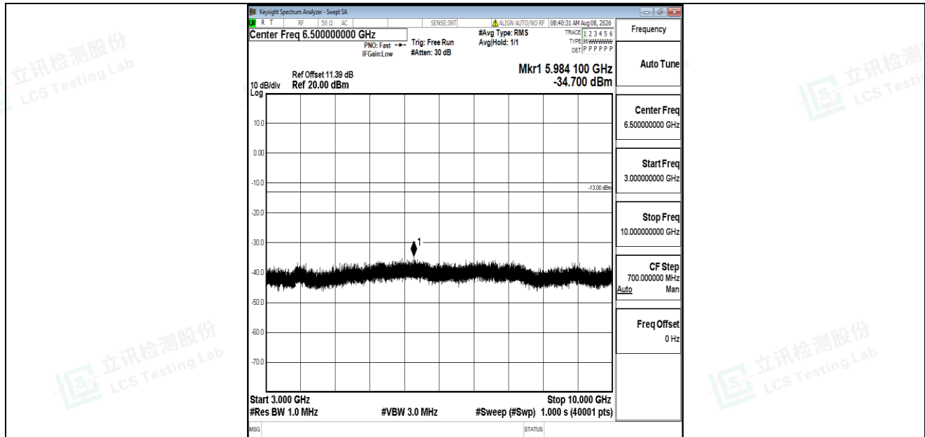
Band5-5MHz-QPSK-20625-1RB#0-3000~10000-PASS
