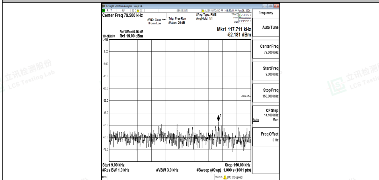
Band5-10MHz-16QAM-20450-1RB#0-0.009~0.15-PASS
