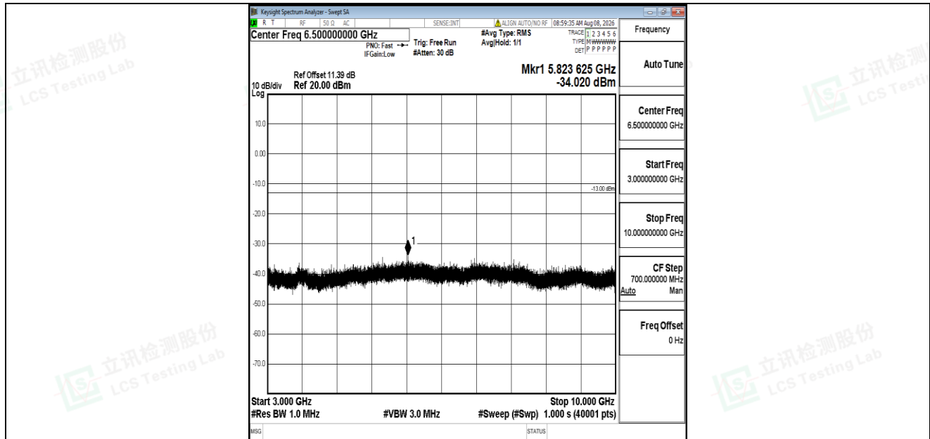
Band5-10MHz-QPSK-20450-1RB#0-3000~10000-PASS
