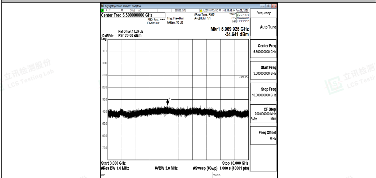
Band5-5MHz-16QAM-20525-1RB#0-3000~10000-PASS
