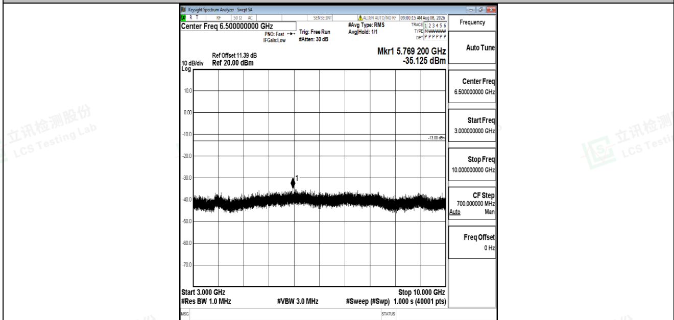
Band5-10MHz-16QAM-20450-1RB#0-3000~10000-PASS
