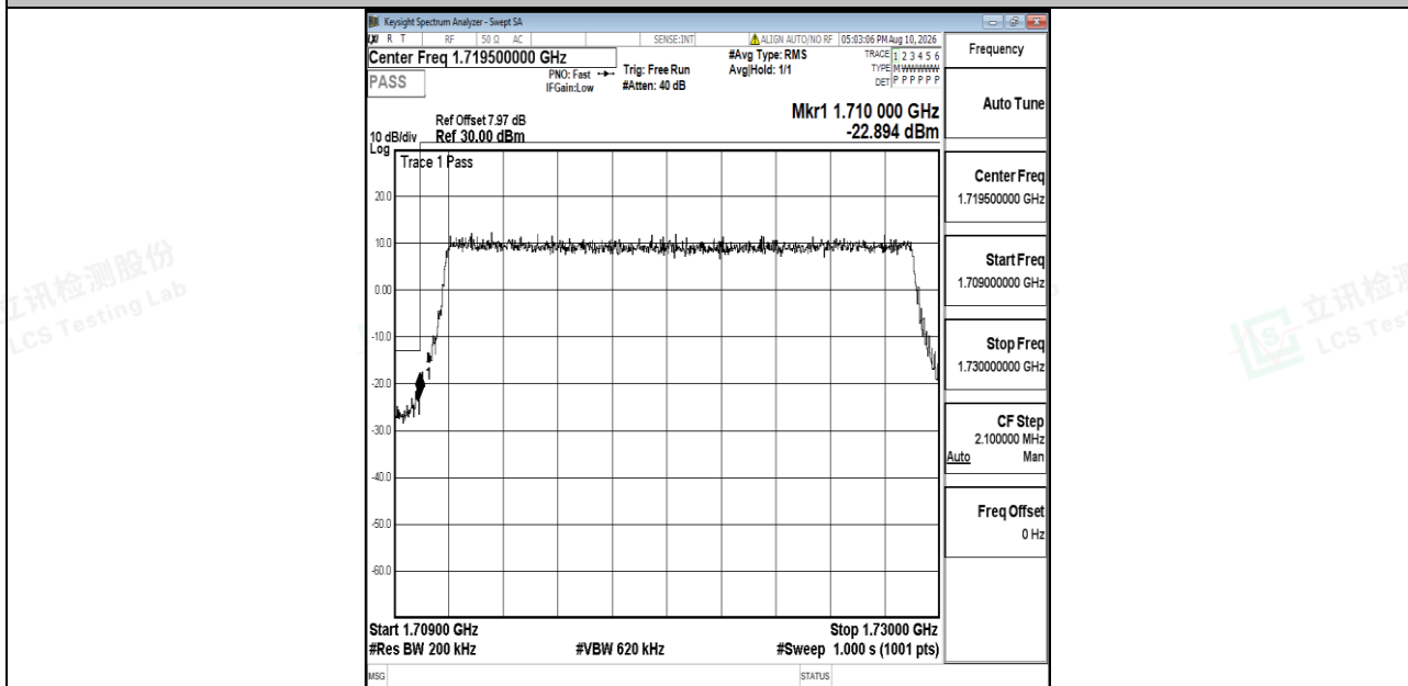
Band66-20MHz-16QAM-132072-100RB#0-PASS
