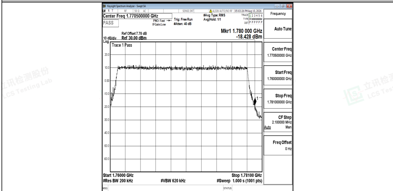
Band66-20MHz-16QAM-132572-100RB#0-PASS
