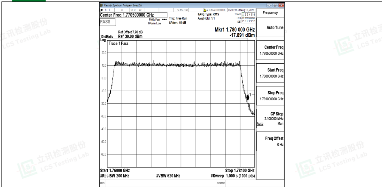
Band66-20MHz-QPSK-132572-100RB#0-PASS
