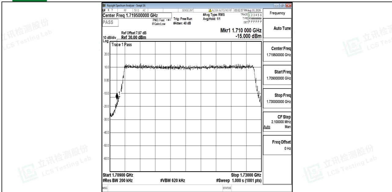
Band66-20MHz-QPSK-132072-100RB#0-PASS
