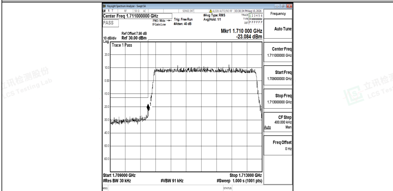
Band66-3MHz-16QAM-131987-15RB#0-PASS
