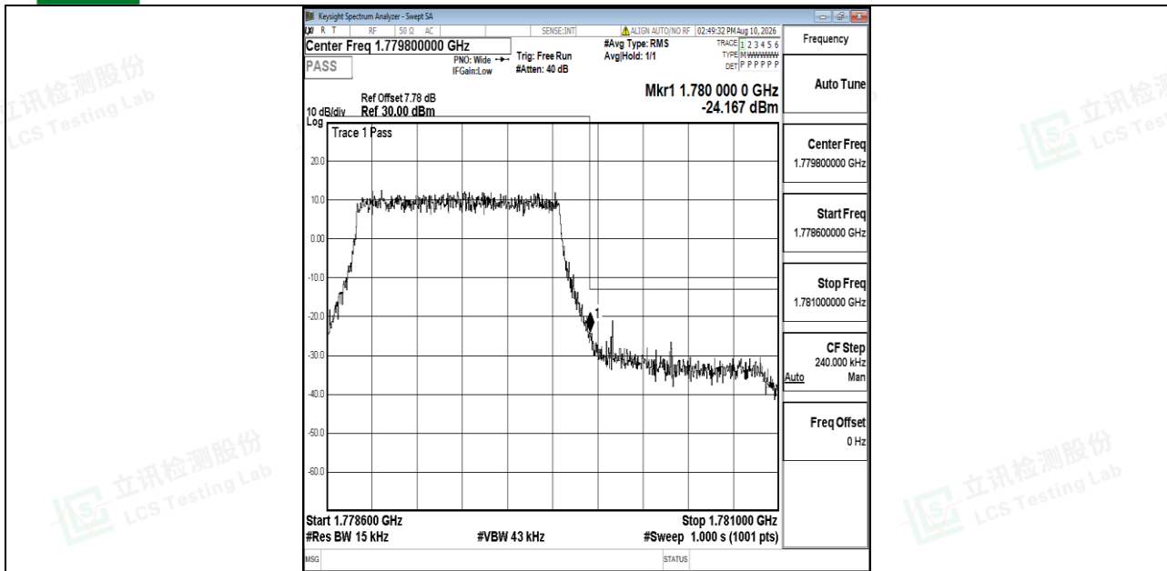
Band66-1.4MHz-QPSK-132665-6RB#0-PASS
