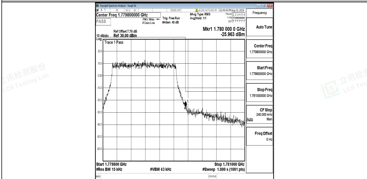
Band66-1.4MHz-16QAM-132665-6RB#0-PASS
