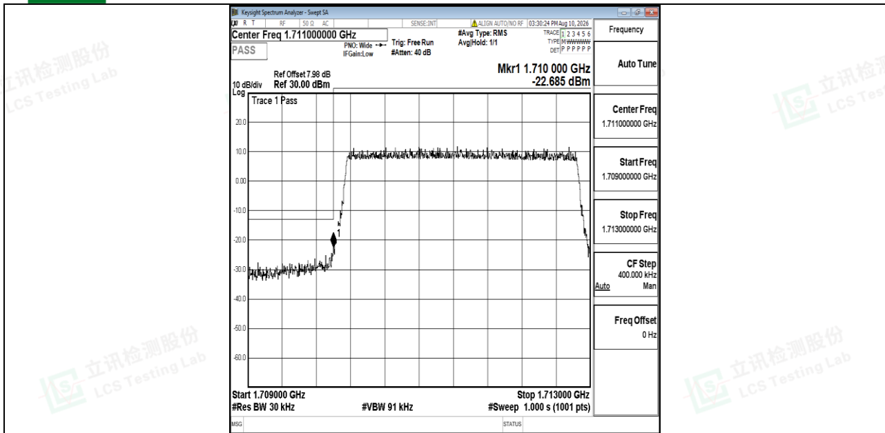
Band66-3MHz-QPSK-131987-15RB#0-PASS
