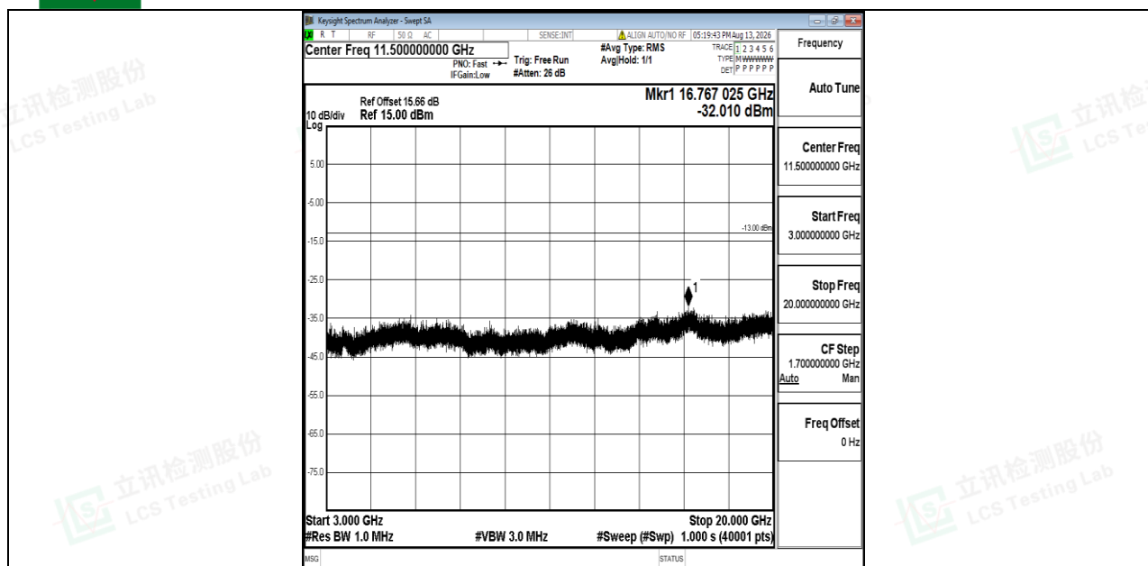
Band66-15MHz-16QAM-132322-1RB#0-3000~20000-PASS
