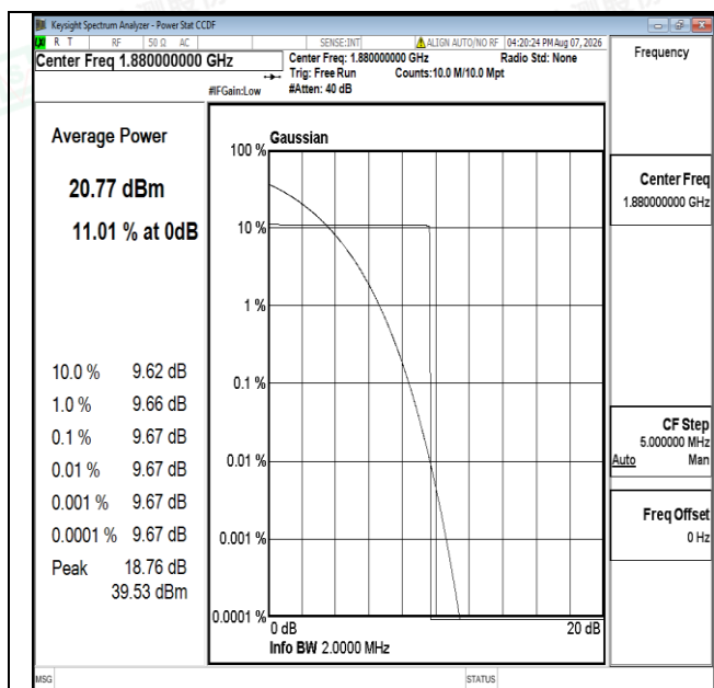
Channel 661 / 1880 MHz
