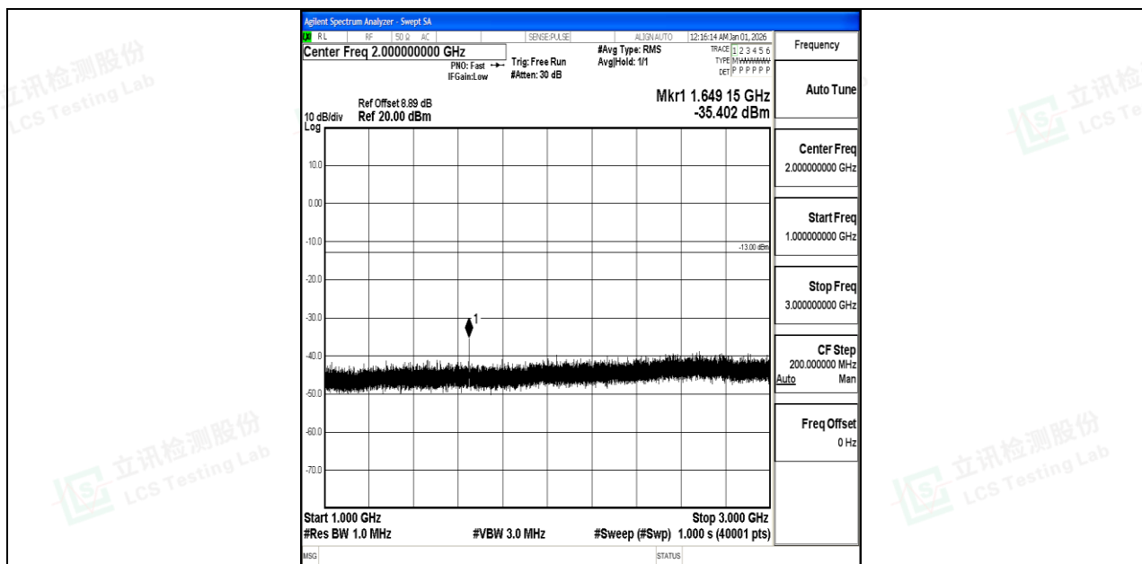
Band5_5MHz_16QAM_20425_1RB#0_1000~3000_1000~3000
