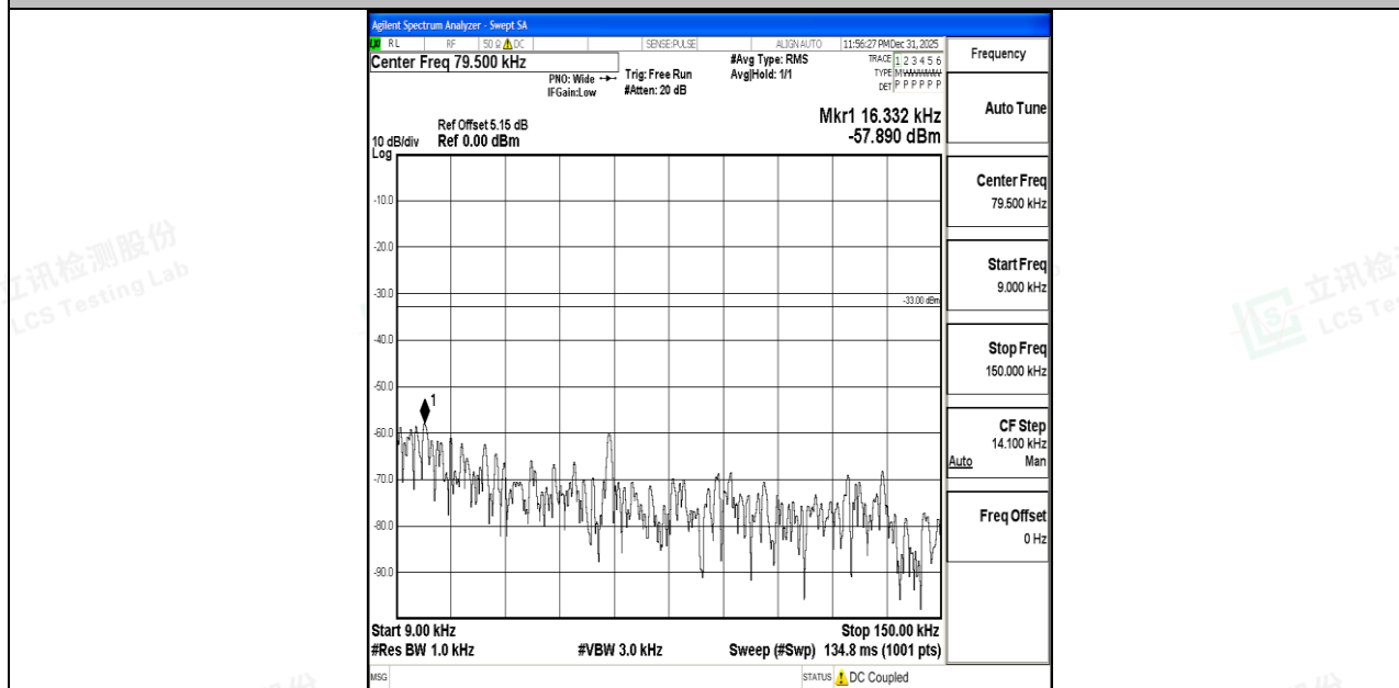
Band5_3MHz_16QAM_20635_1RB#0_0.009~0.15_0.009~0.15
