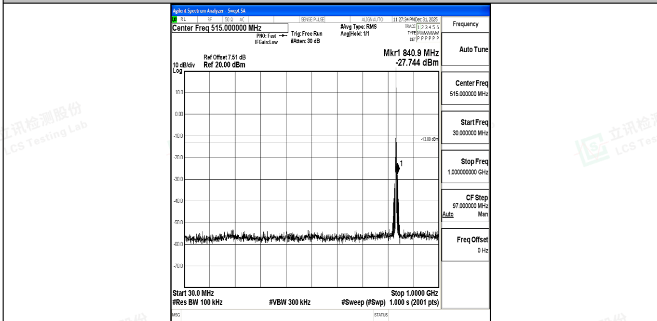
Band5_1.4MHz_16QAM_20525_1RB#0_30~1000_30~1000
