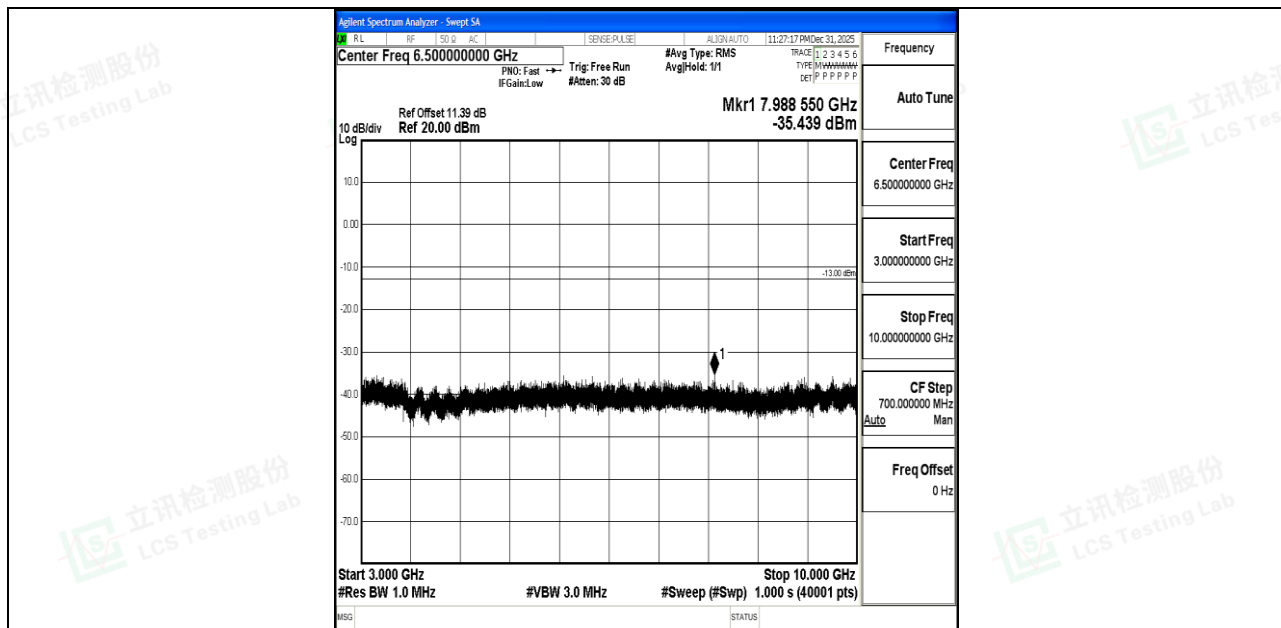
Band5_1.4MHz_QPSK_20525_1RB#0_3000~10000_3000~10000
