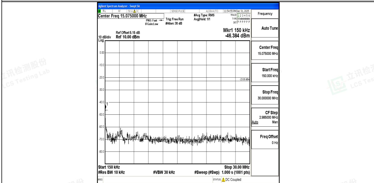
Band5_3MHz_QPSK_20525_1RB#0_0.15~30_0.15~30
