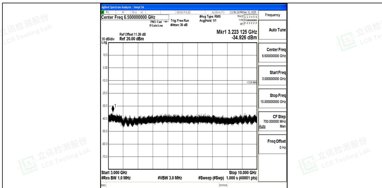
Band5_3MHz_QPSK_20635_1RB#0_3000~10000_3000~10000
