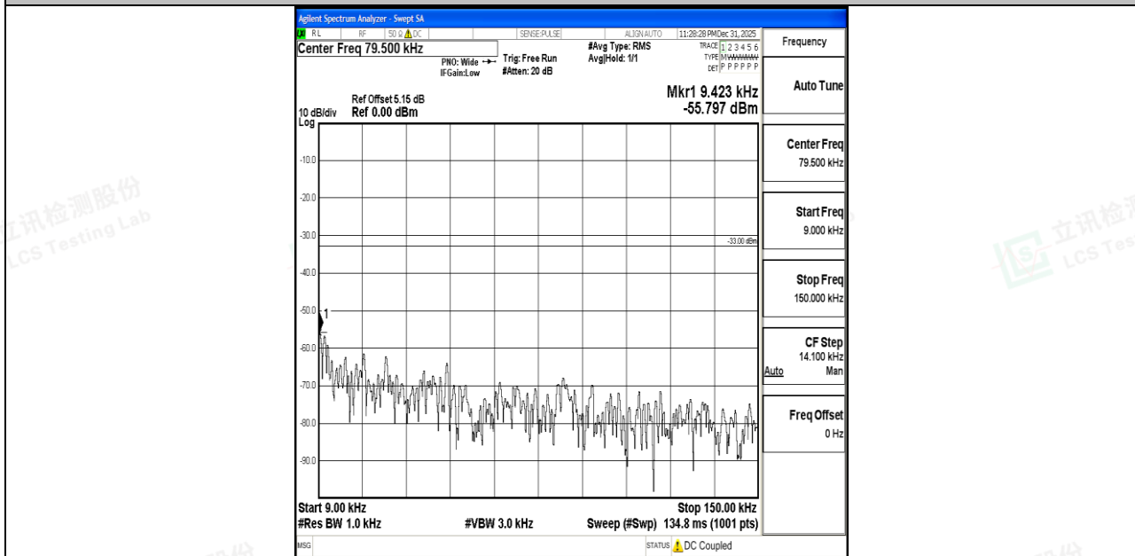
Band5_1.4MHz_16QAM_20643_1RB#0_0.009~0.15_0.009~0.15
