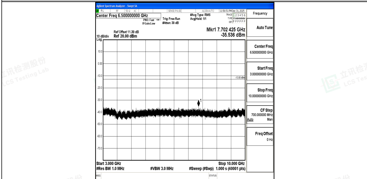
Band5_3MHz_16QAM_20635_1RB#0_3000~10000_3000~10000
