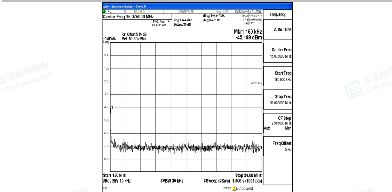
Band5_5MHz_QPSK_20425_1RB#0_0.15~30_0.15~30
