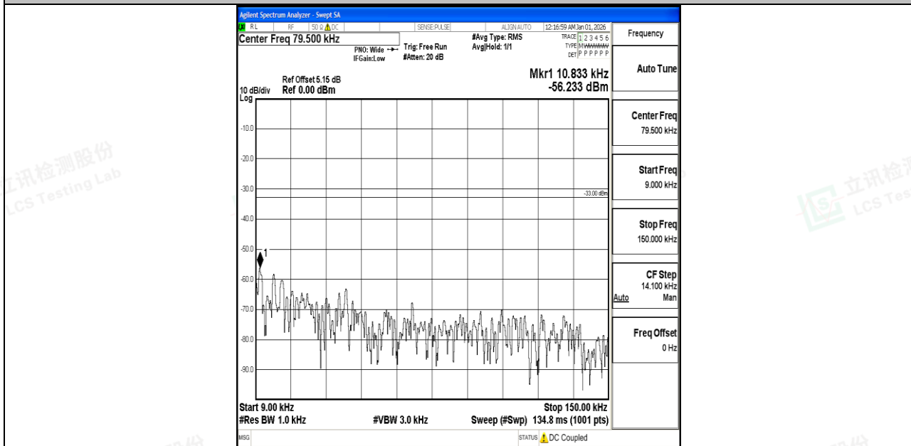
Band5_5MHz_16QAM_20525_1RB#0_0.009~0.15_0.009~0.15
