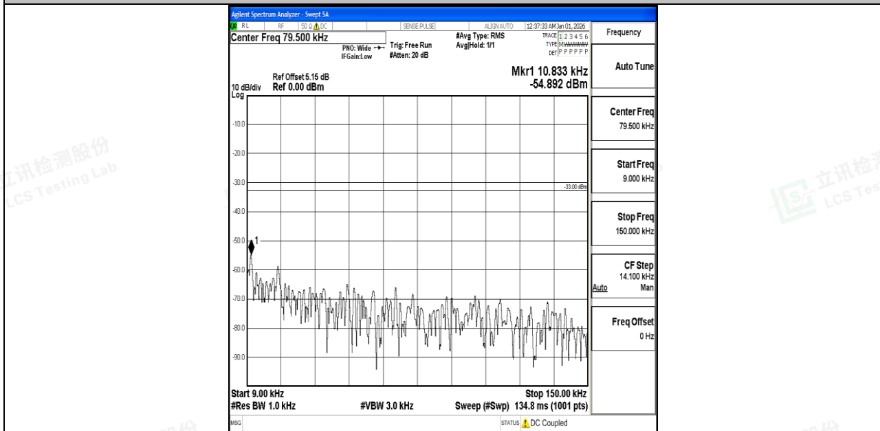
Band5_10MHz_16QAM_20525_1RB#0_0.009~0.15_0.009~0.15
