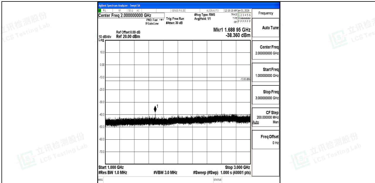
Band5_5MHz_16QAM_20625_1RB#0_1000~3000_1000~3000
