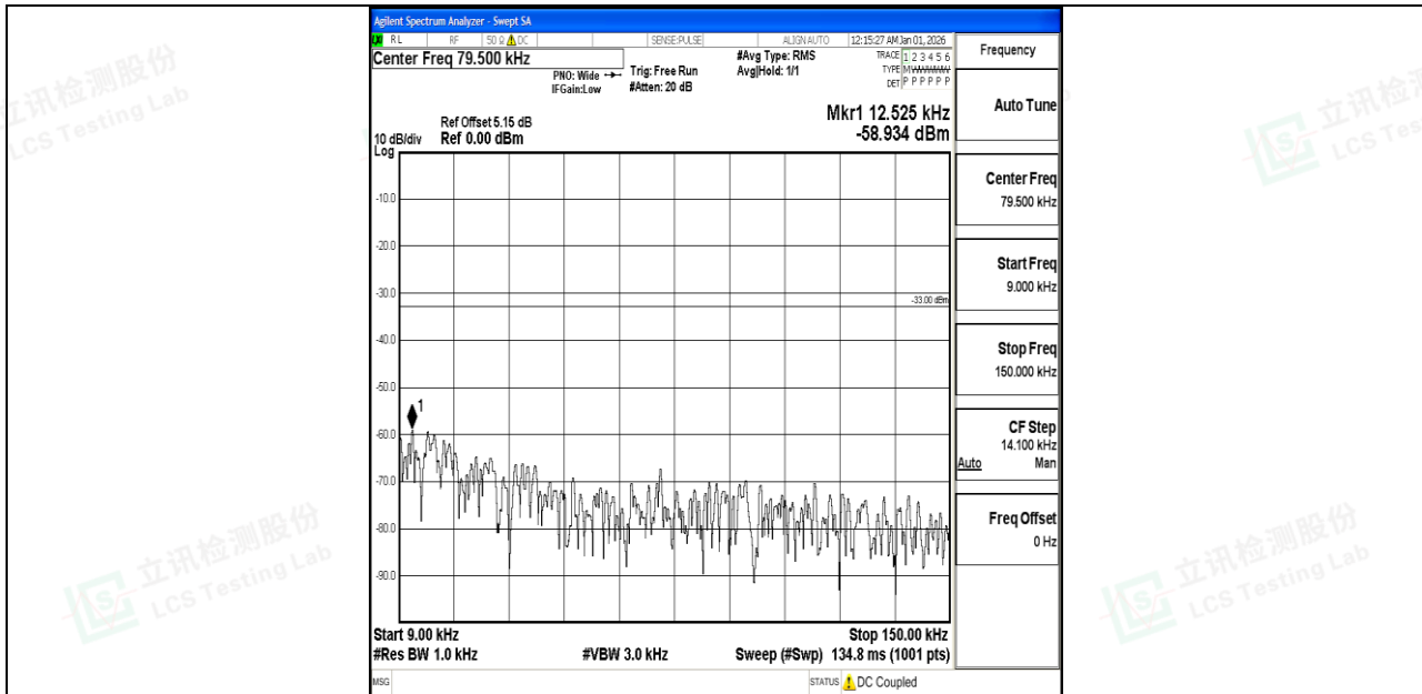
Band5_5MHz_QPSK_20425_1RB#0_0.009~0.15_0.009~0.15
