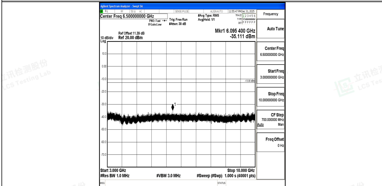
Band5_3MHz_16QAM_20525_1RB#0_3000~10000_3000~10000
