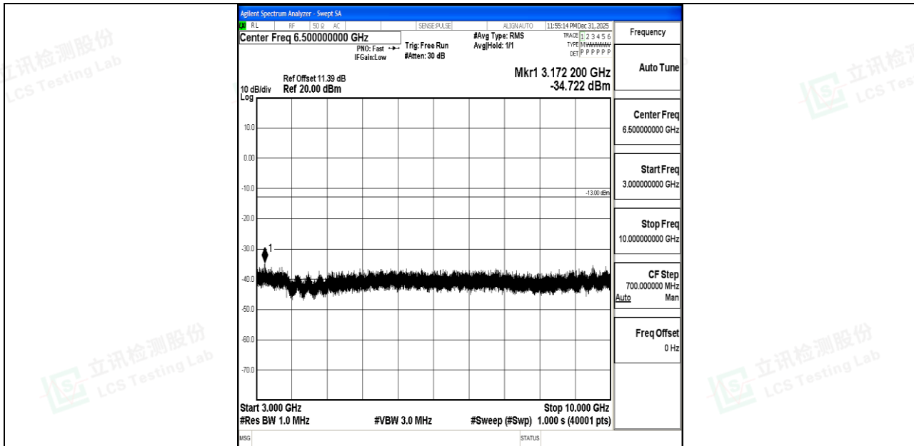
Band5_3MHz_QPSK_20525_1RB#0_3000~10000_3000~10000
