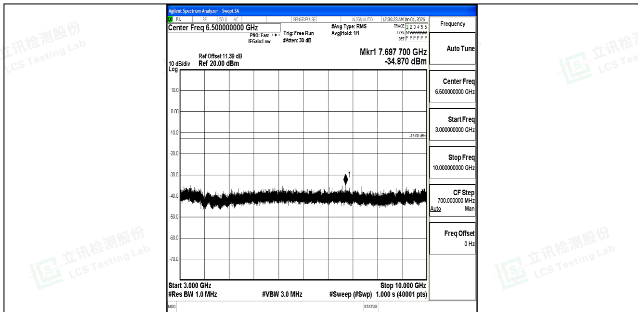
Band5_10MHz_QPSK_20450_1RB#0_3000~10000_3000~10000
