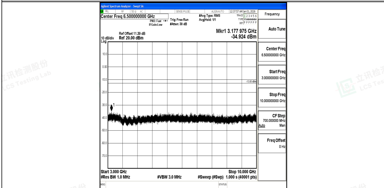
Band5_10MHz_16QAM_20525_1RB#0_3000~10000_3000~10000
