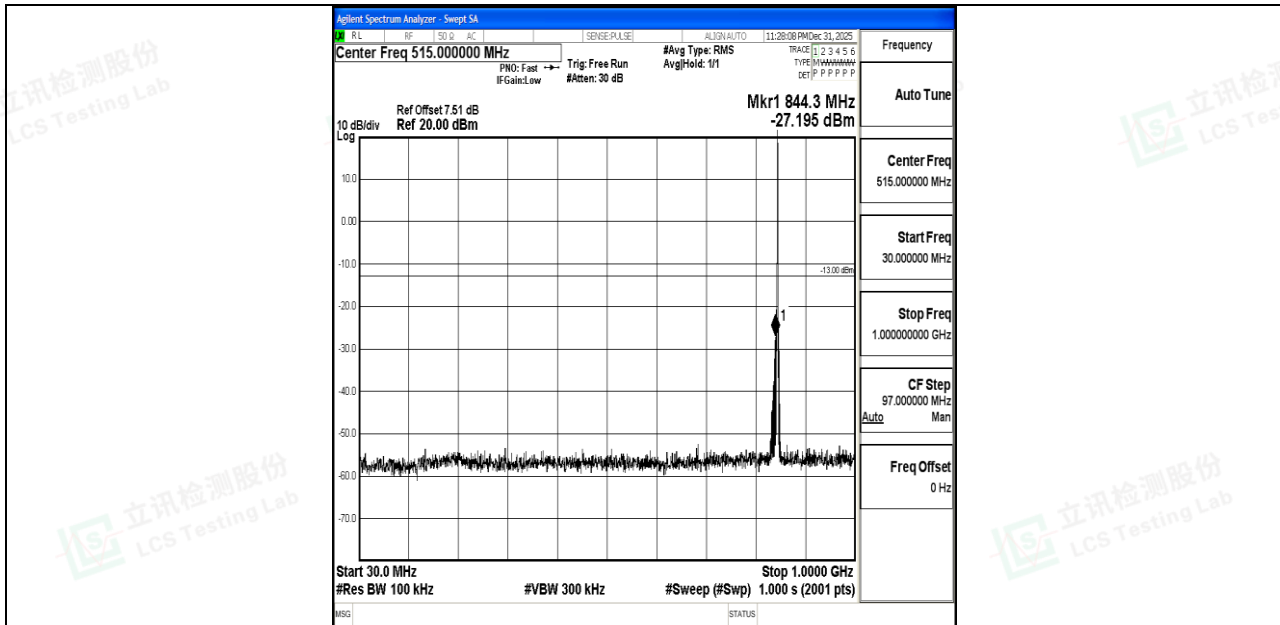
Band5_1.4MHz_QPSK_20643_1RB#0_30~1000_30~1000
