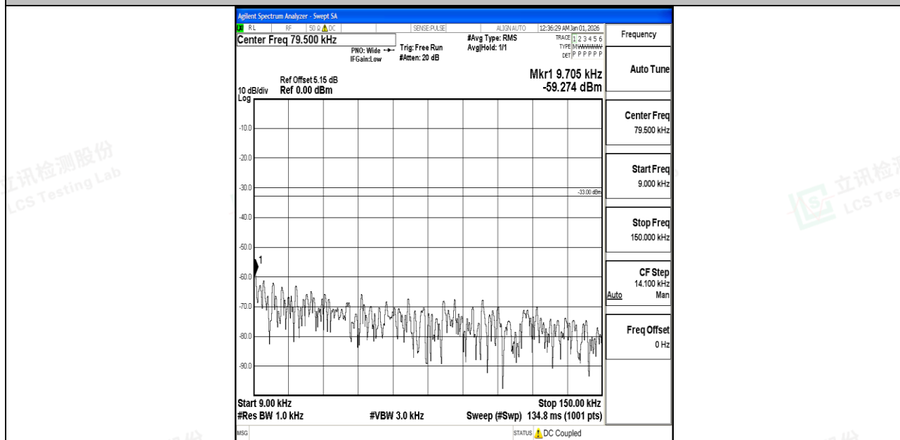
Band5_10MHz_16QAM_20450_1RB#0_0.009~0.15_0.009~0.15
