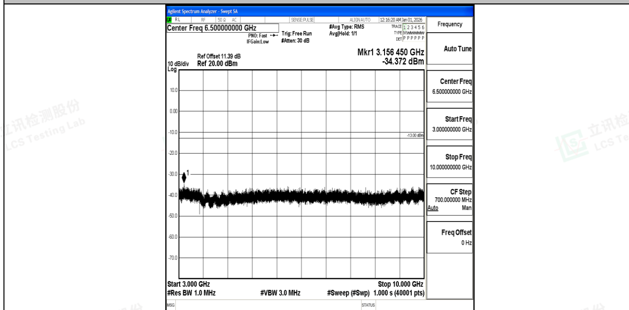
Band5_5MHz_16QAM_20425_1RB#0_3000~10000_3000~10000
