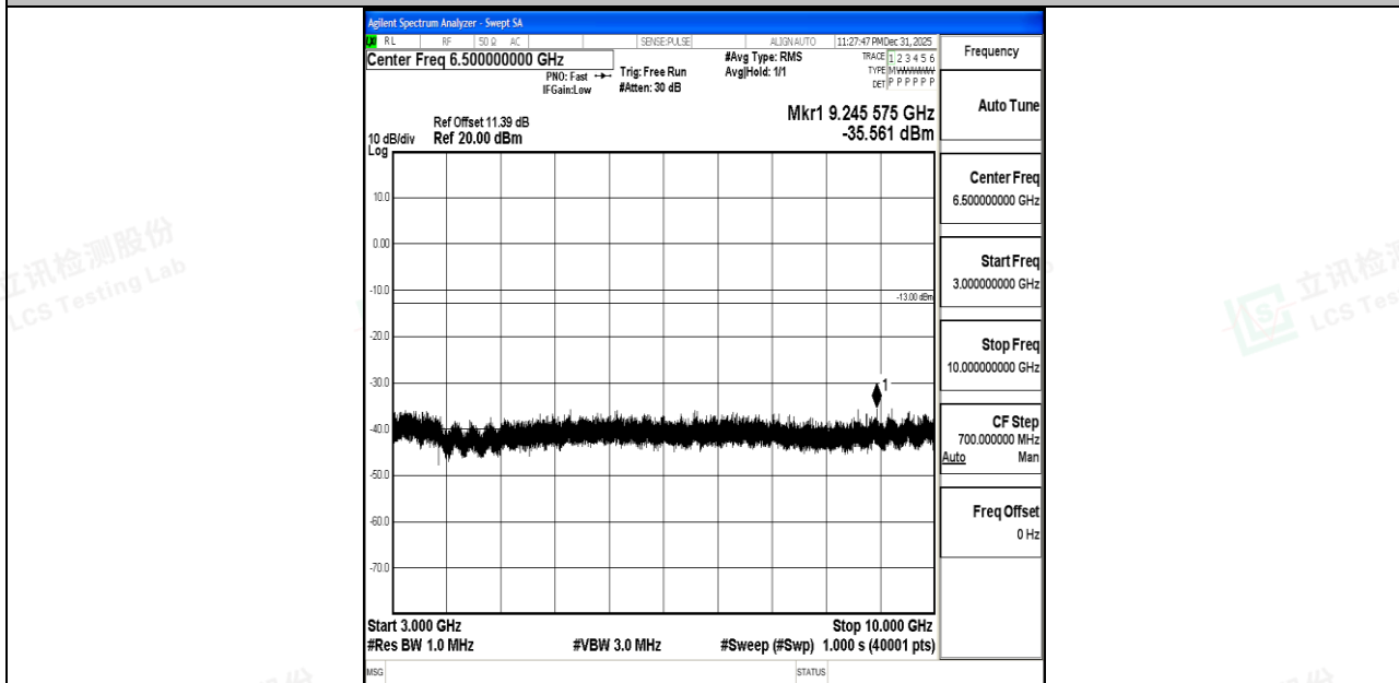
Band5_1.4MHz_16QAM_20525_1RB#0_3000~10000_3000~10000
