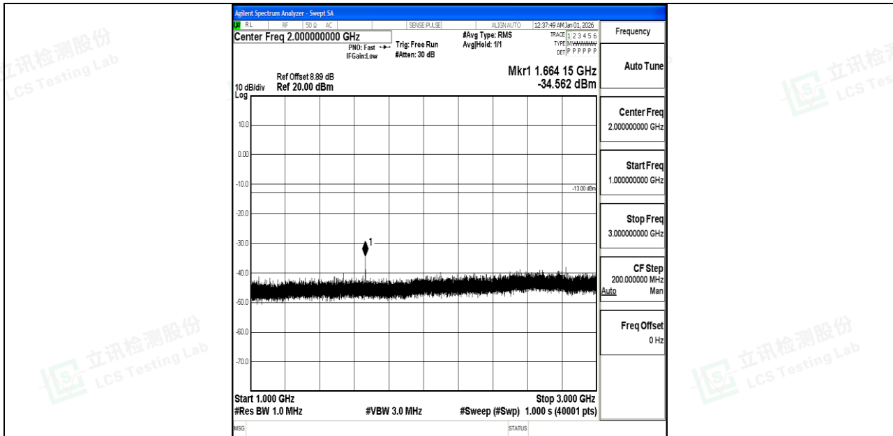
Band5_10MHz_16QAM_20525_1RB#0_1000~3000_1000~3000
