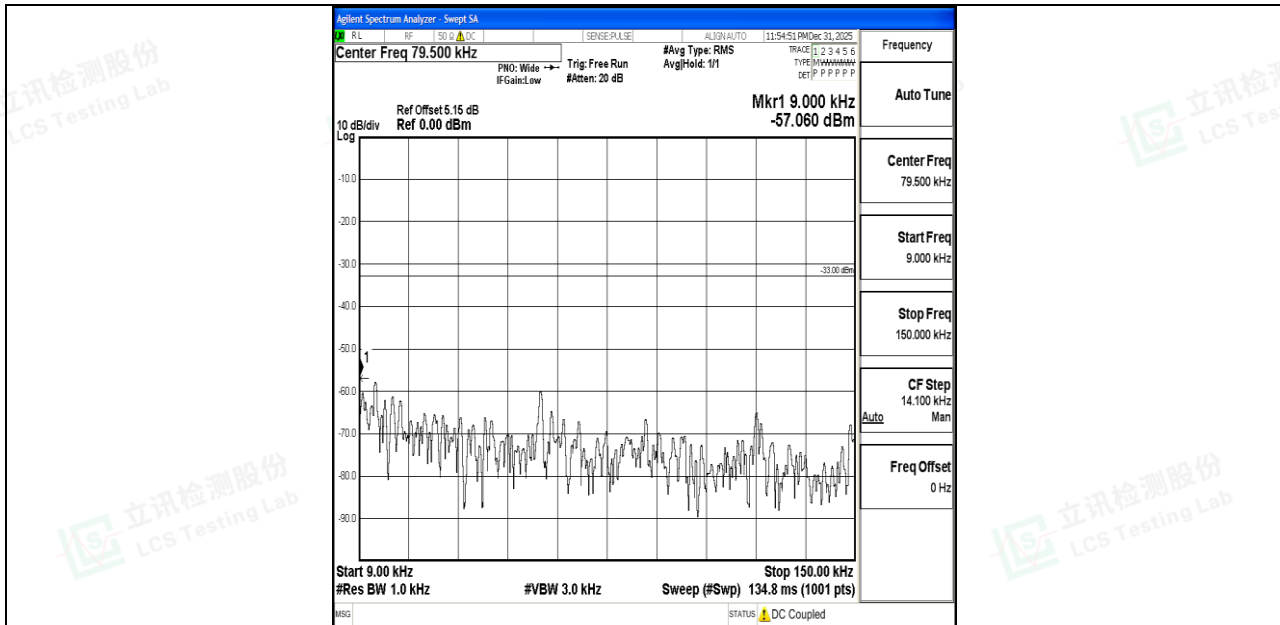
Band5_3MHz_QPSK_20525_1RB#0_0.009~0.15_0.009~0.15
