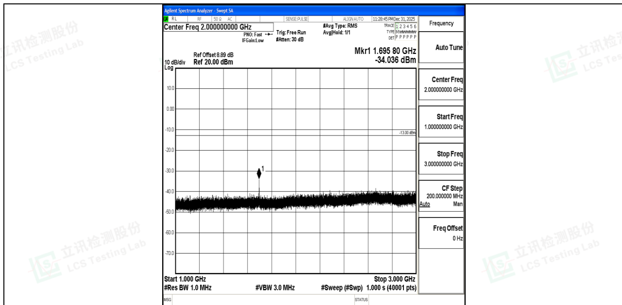
Band5_1.4MHz_16QAM_20643_1RB#0_1000~3000_1000~3000
