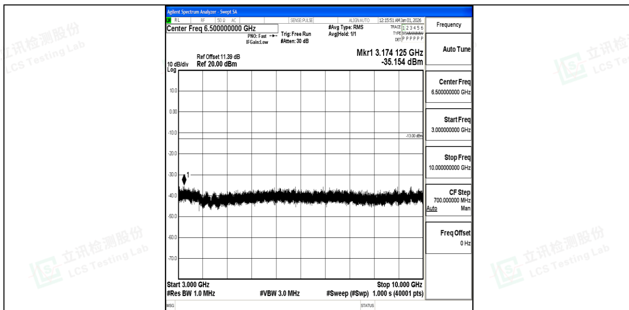
Band5_5MHz_QPSK_20425_1RB#0_3000~10000_3000~10000
