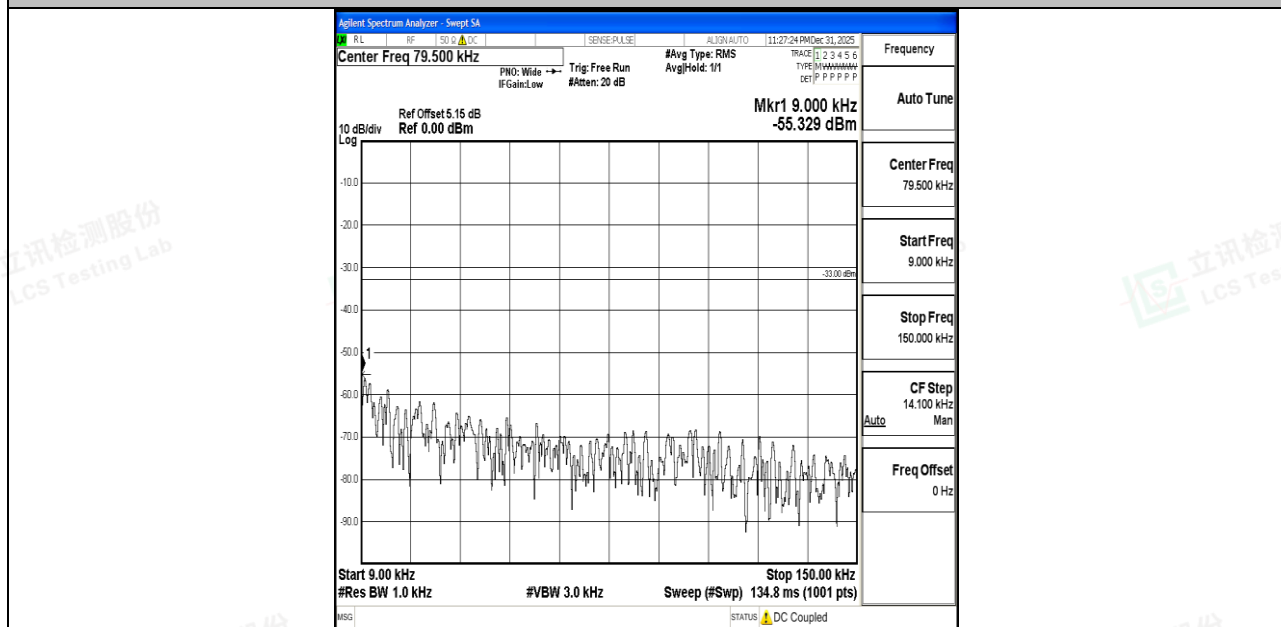
Band5_1.4MHz_16QAM_20525_1RB#0_0.009~0.15_0.009~0.15
