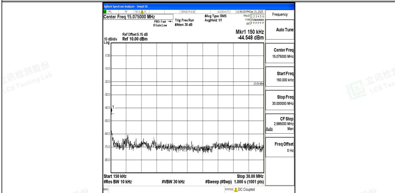
Band5_3MHz_QPSK_20635_1RB#0_0.15~30_0.15~30
