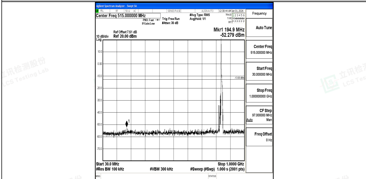
Band5_10MHz_16QAM_20600_1RB#0_30~1000_30~1000
