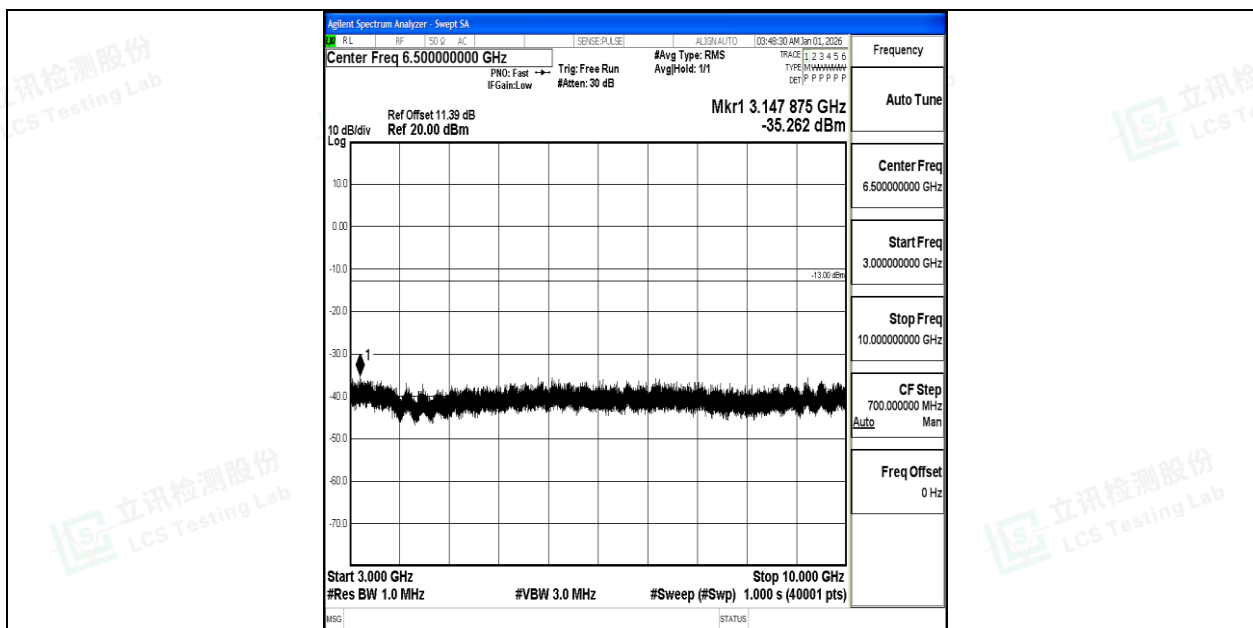
Band12_10MHz_QPSK_23060_1RB#0_3000~10000_3000~10000
