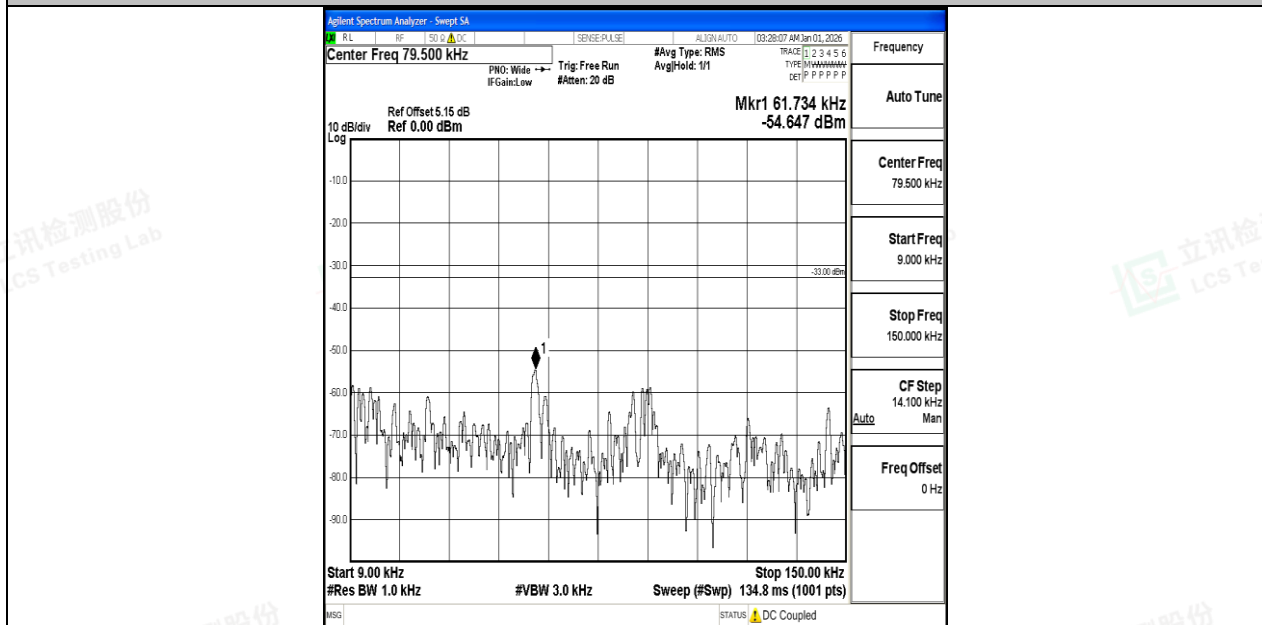
Band12_5MHz_16QAM_23155_1RB#0_0.009~0.15_0.009~0.15
