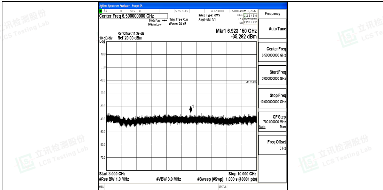
Band12_5MHz_QPSK_23155_1RB#0_3000~10000_3000~10000
