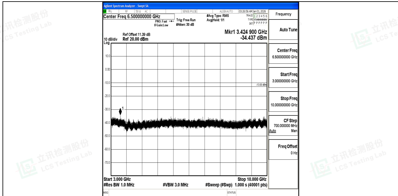
Band12_5MHz_QPSK_23095_1RB#0_3000~10000_3000~10000
