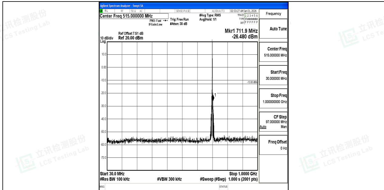
Band12_1.4MHz_QPSK_23095_1RB#0_30~1000_30~1000
