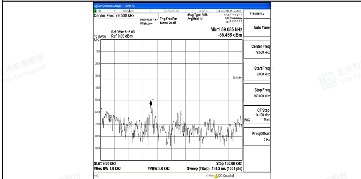
Band12_5MHz_16QAM_23095_1RB#0_0.009~0.15_0.009~0.15
