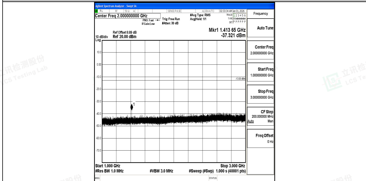
Band12_1.4MHz_QPSK_23095_1RB#0_1000~3000_1000~3000
