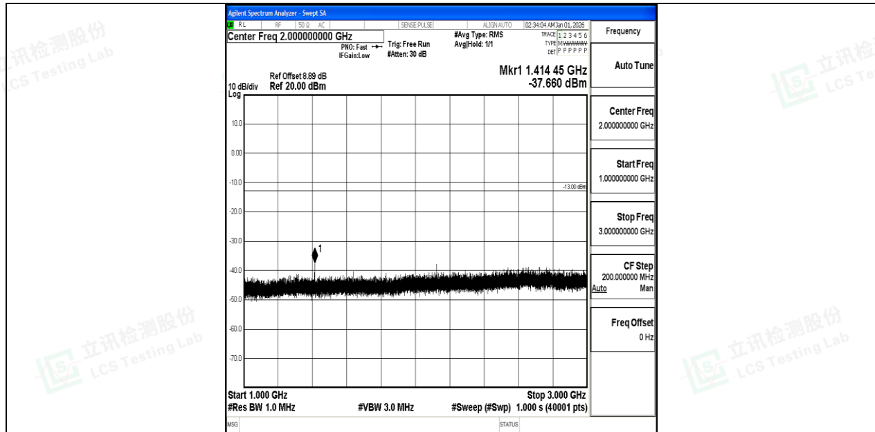
Band12_1.4MHz_16QAM_23095_1RB#0_1000~3000_1000~3000
