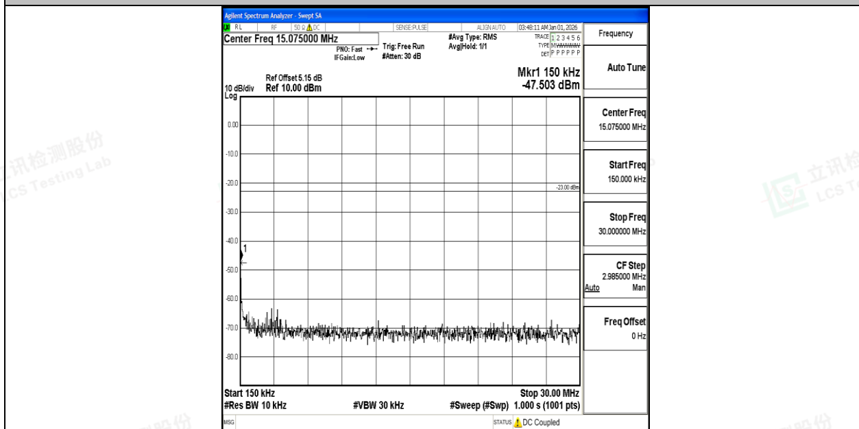
Band12_10MHz_QPSK_23060_1RB#0_0.15~30_0.15~30
