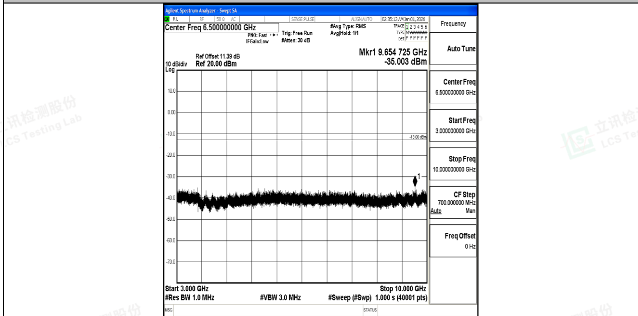
Band12_1.4MHz_16QAM_23173_1RB#0_3000~10000_3000~10000
