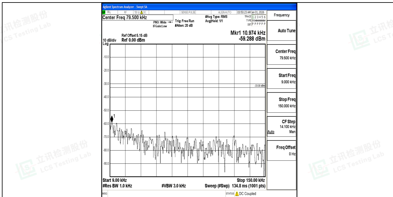
Band12_10MHz_QPSK_23130_1RB#0_0.009~0.15_0.009~0.15
