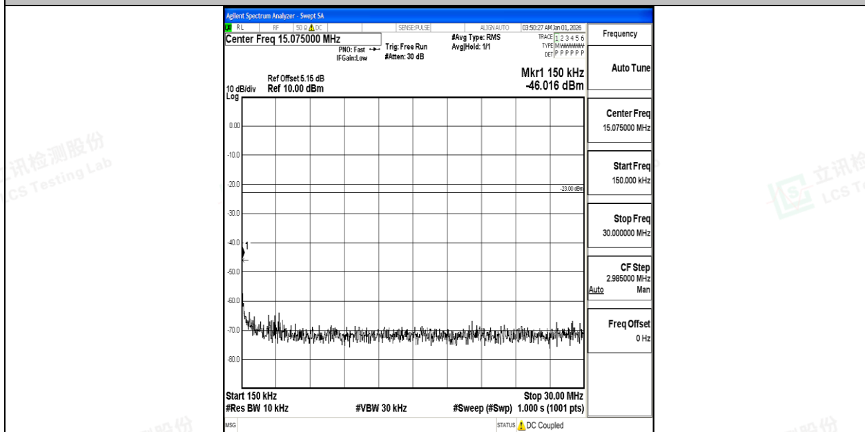
Band12_10MHz_QPSK_23130_1RB#0_0.15~30_0.15~30
