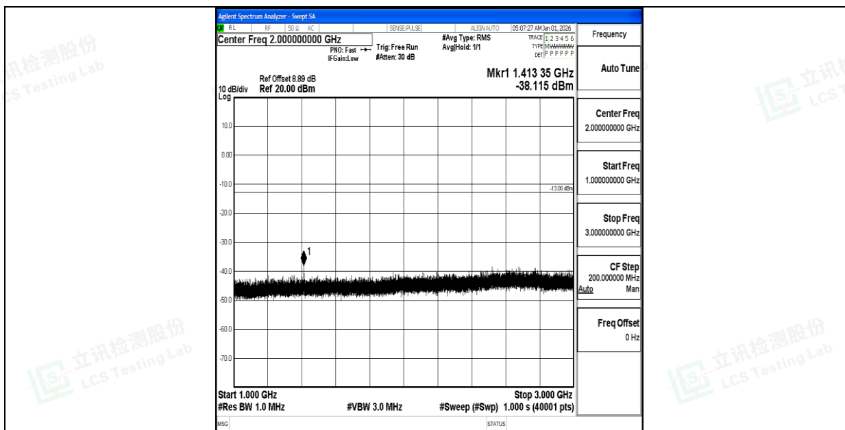
Band17_10MHz_QPSK_23800_1RB#0_1000~3000_1000~3000
