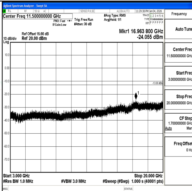
Band66_20MHz_QPSK_132572_1RB#0_3000~20000_3000~20000
