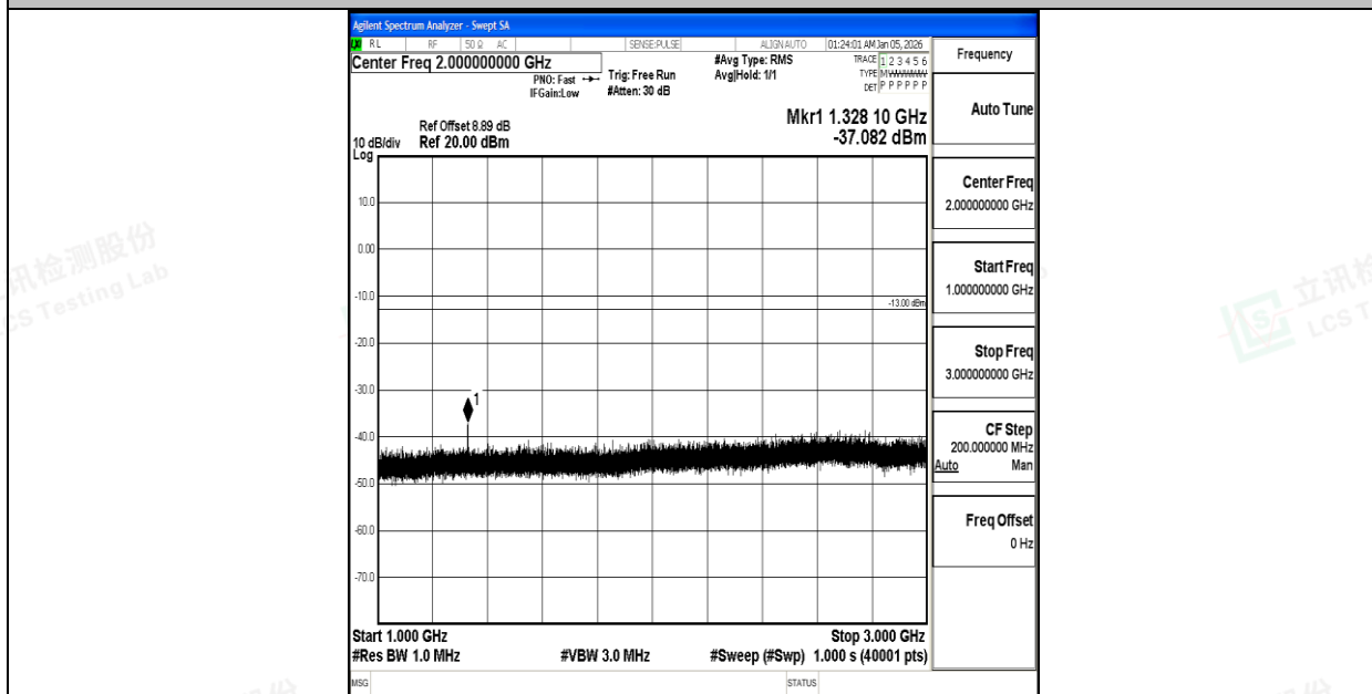
Band71_20MHz_QPSK_133222_1RB#0_1000~3000_1000~3000
