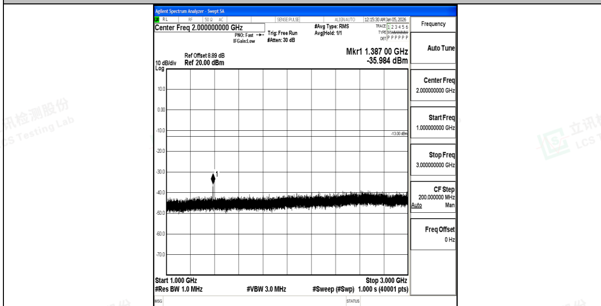
Band71_5MHz_QPSK_133447_1RB#0_1000~3000_1000~3000
