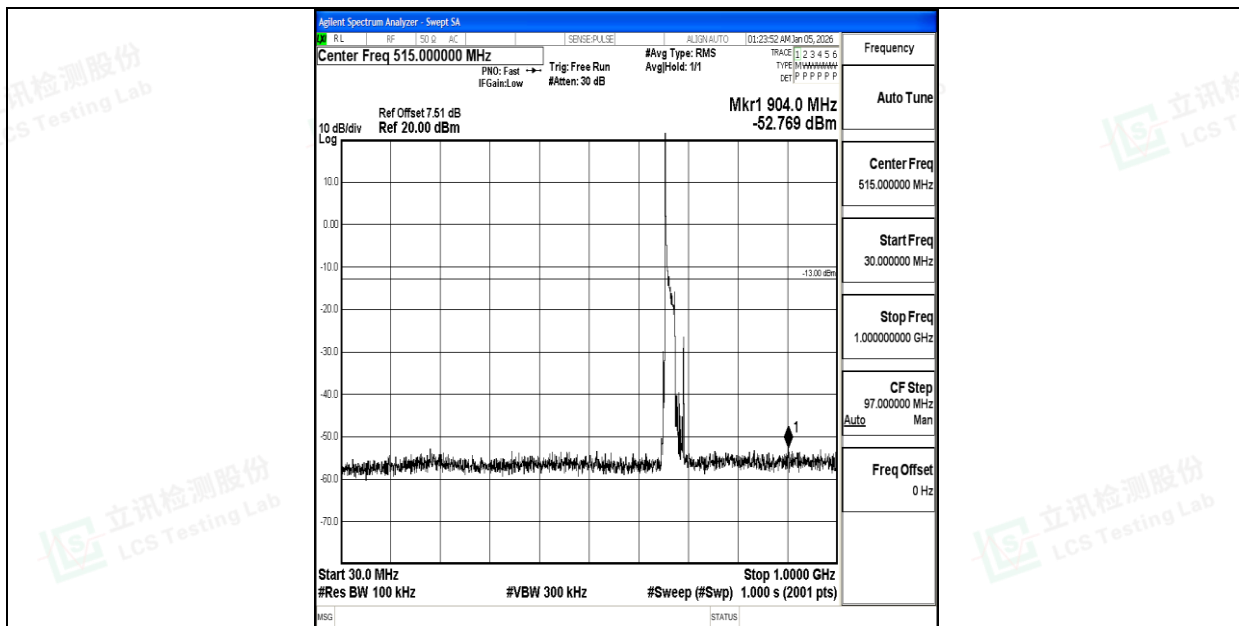
Band71_20MHz_QPSK_133222_1RB#0_30~1000_30~1000
