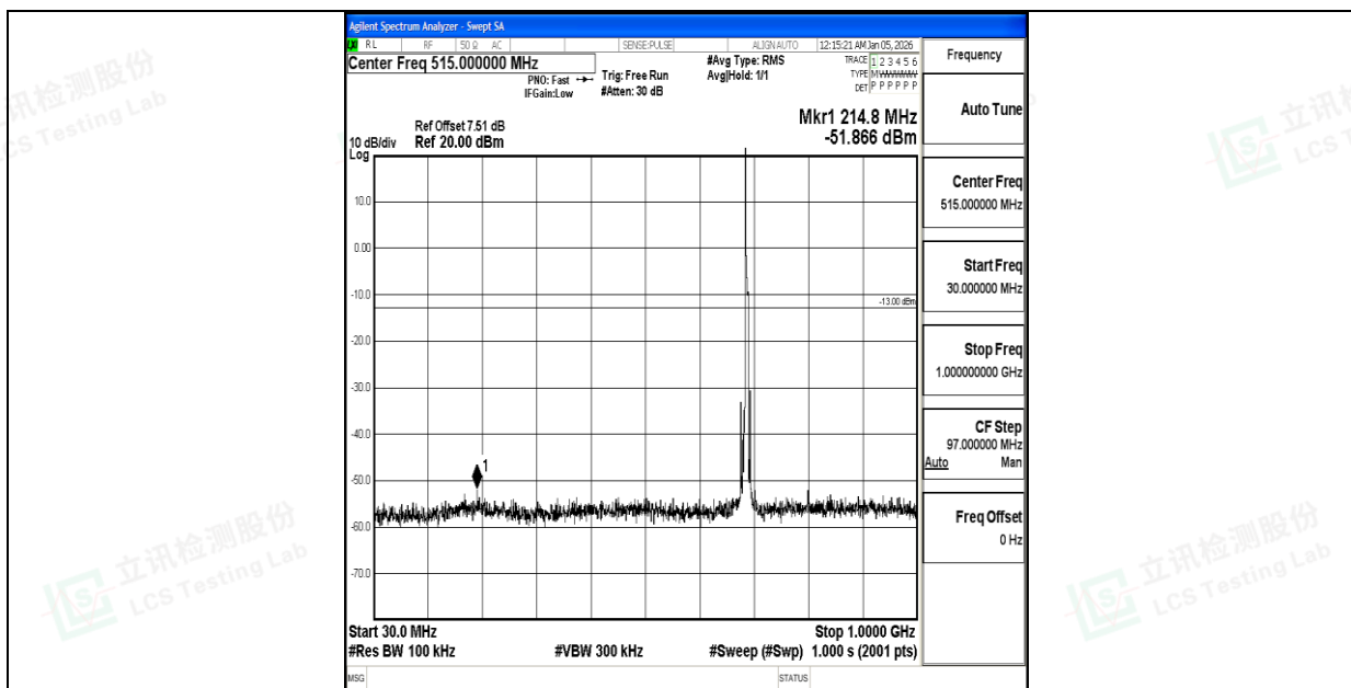
Band71_5MHz_QPSK_133447_1RB#0_30~1000_30~1000
