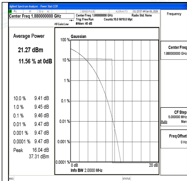
Channel 661 / 1880 MHz
