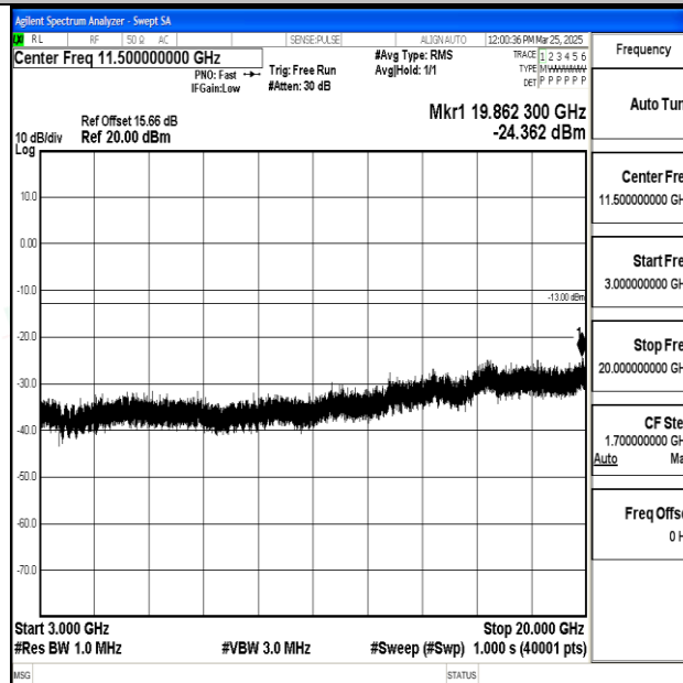
Band2_15MHz_QPSK_18675_1RB#0_3000~20000_3000~20000
