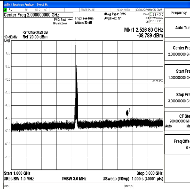
Band2_15MHz_QPSK_18675_1RB#0_1000~3000_1000~3000
