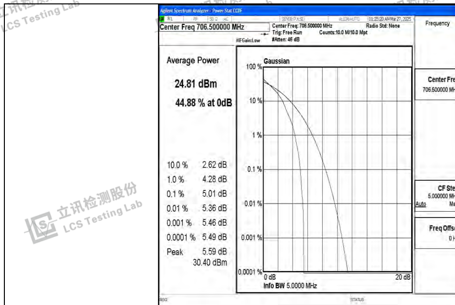
Band17-5MHz-QPSK-23755-1RB#0-PASS
