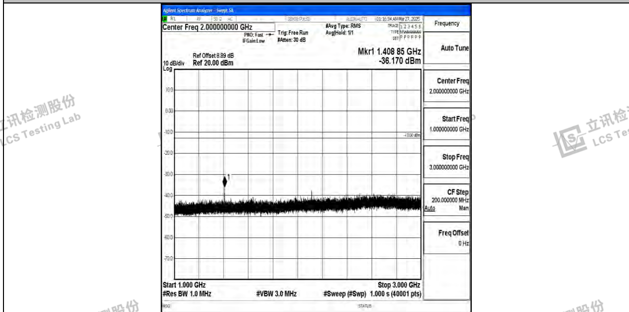
Band17_5MHz_16QAM_23755_1RB#0_1000~3000_1000~3000
