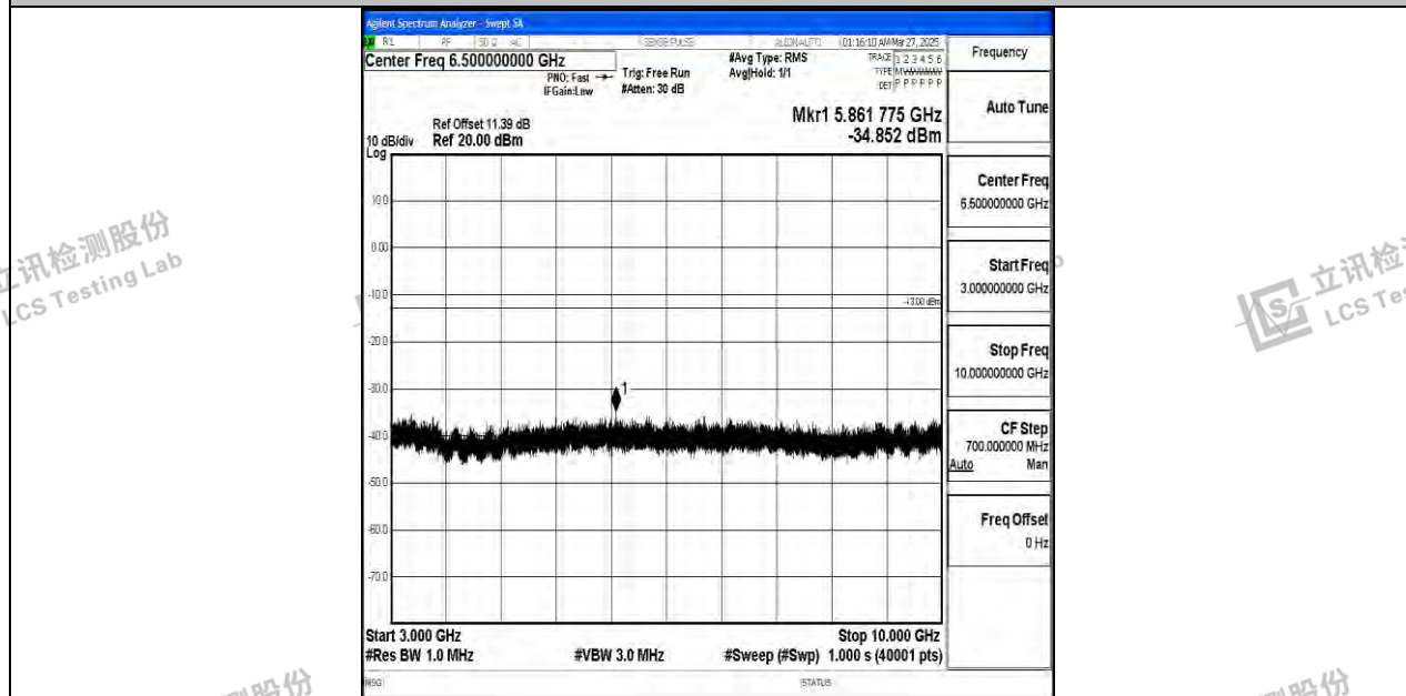
Band17_5MHz_QPSK_23755_1RB#0_3000~10000_3000~10000
