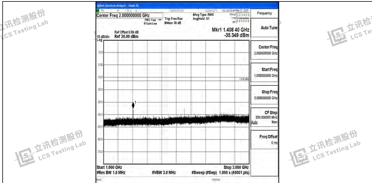
Band17_5MHz_QPSK_23755_1RB#0_1000~3000_1000~3000
