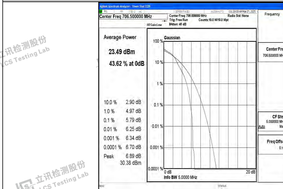
Band17-5MHz-16QAM-23755-1RB#0-PASS
