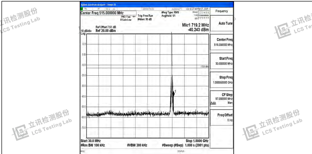
Band17_5MHz_16QAM_23755_1RB#0_30~1000_30~1000
