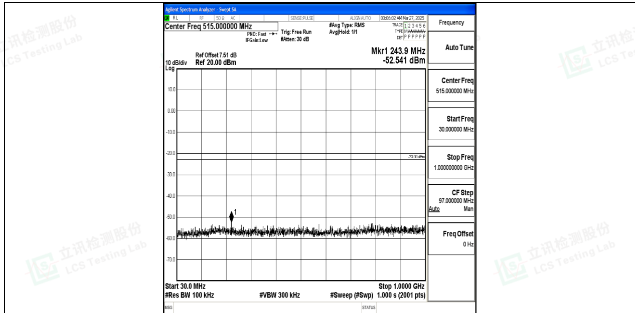
Band66_5MHz_16QAM_132647_1RB#0_30~1000_30~1000
