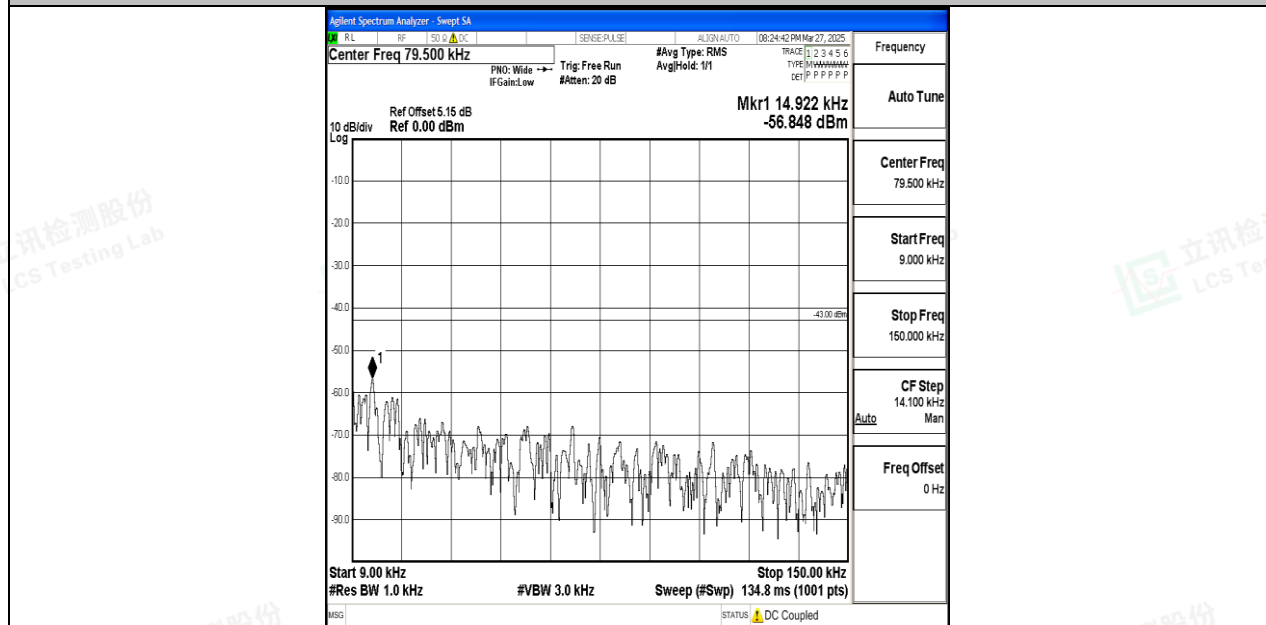
Band66_10MHz_QPSK_132622_1RB#0_0.009~0.15_0.009~0.15
