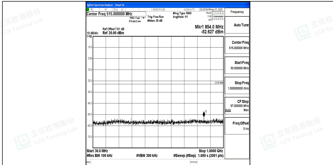
Band66_3MHz_16QAM_132657_1RB#0_30~1000_30~1000
