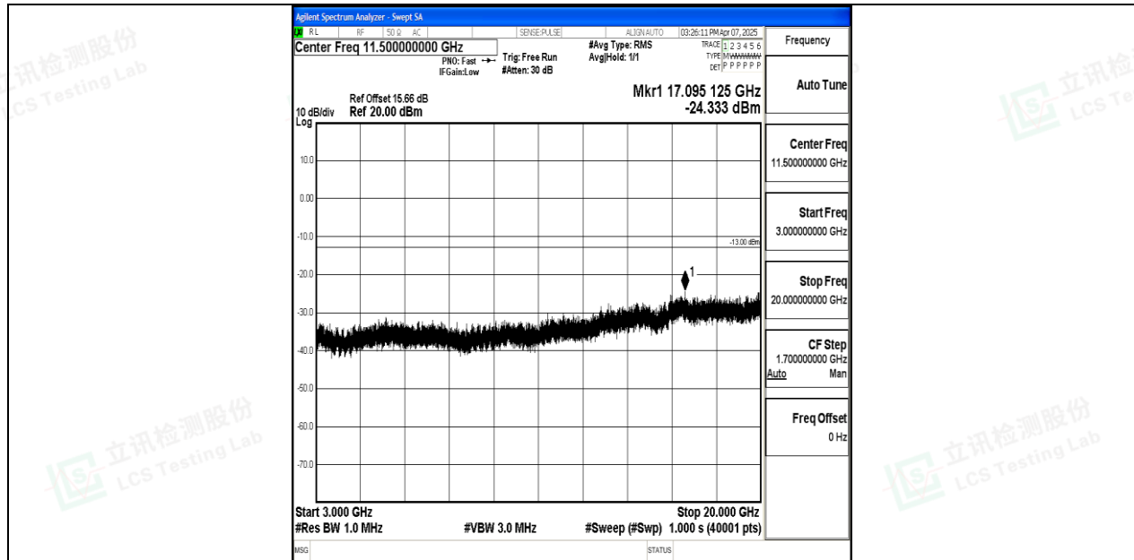
Band66_3MHz_16QAM_132657_1RB#0_3000~20000_3000~20000
