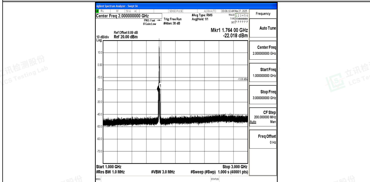
Band66_5MHz_16QAM_132647_1RB#0_1000~3000_1000~3000
