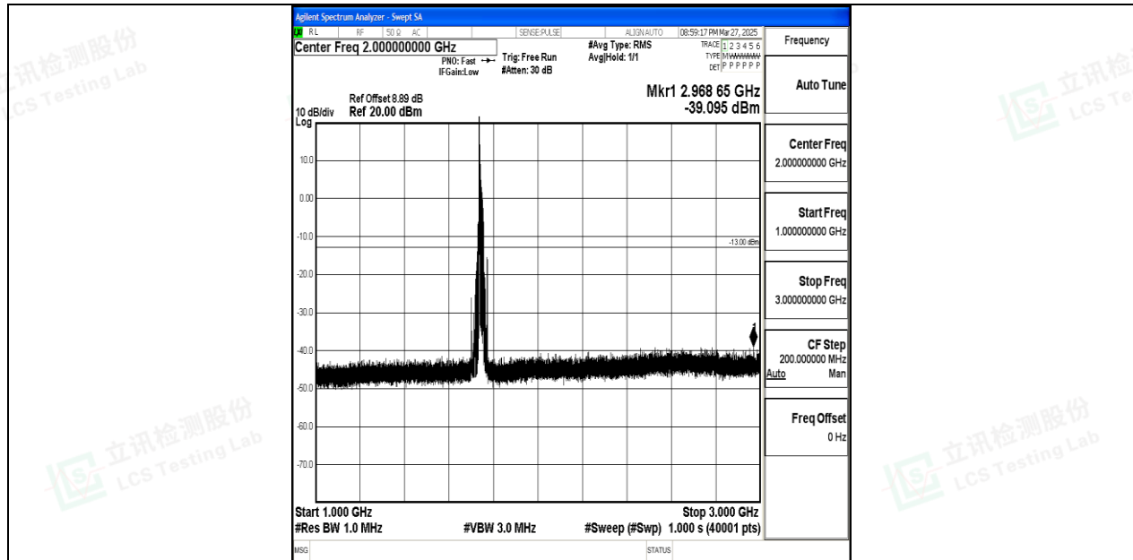
Band66_20MHz_QPSK_132322_1RB#0_1000~3000_1000~3000
