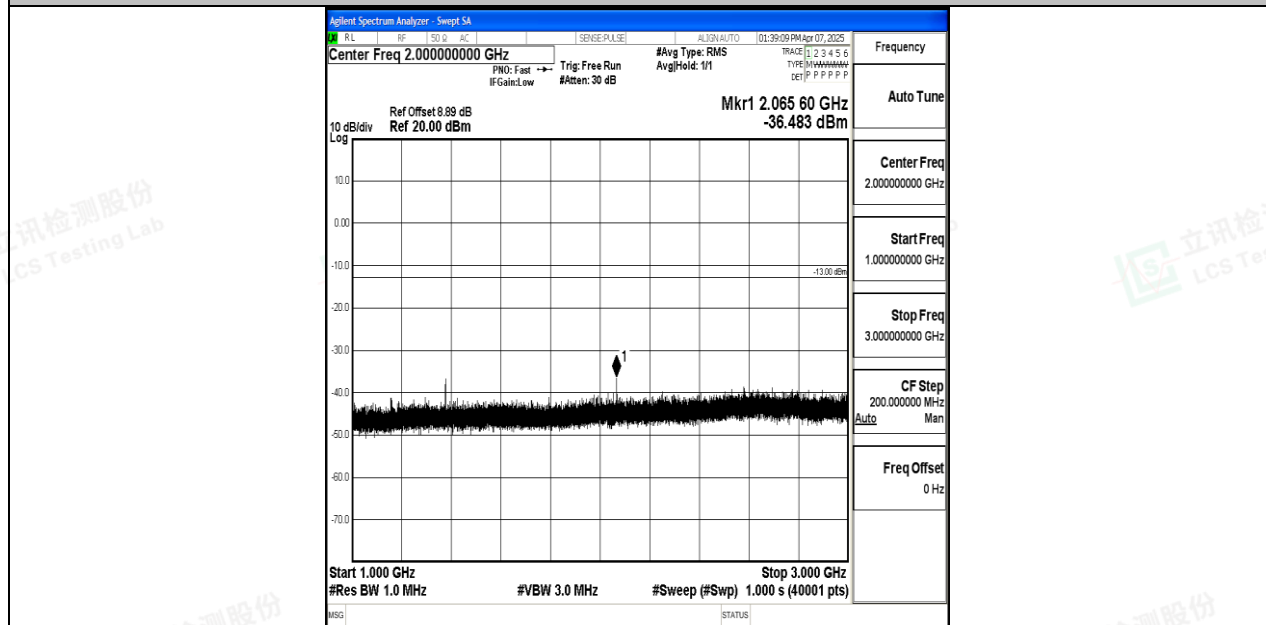
Band71_10MHz_QPSK_133422_1RB#0_1000~3000_1000~3000
