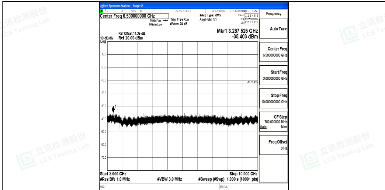
Band71_10MHz_QPSK_133297_1RB#0_3000~10000_3000~10000
