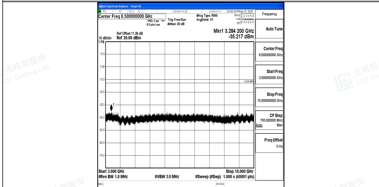
Band71_15MHz_16QAM_133197_1RB#0_3000~10000_3000~10000
