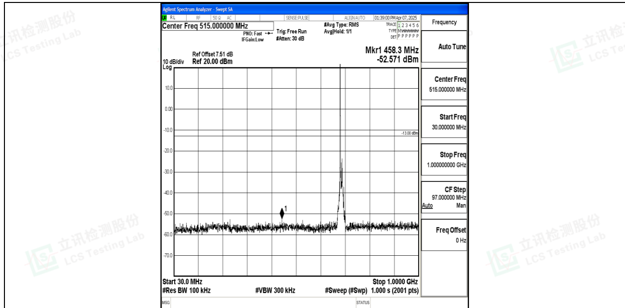
Band71_10MHz_QPSK_133422_1RB#0_30~1000_30~1000
