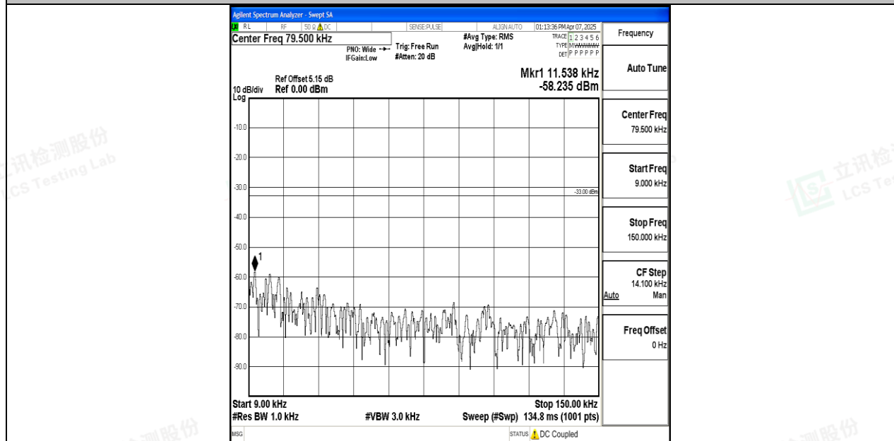
Band71_5MHz_16QAM_133447_1RB#0_0.009~0.15_0.009~0.15
