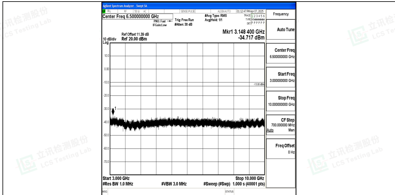
Band71_5MHz_QPSK_133447_1RB#0_3000~10000_3000~10000
