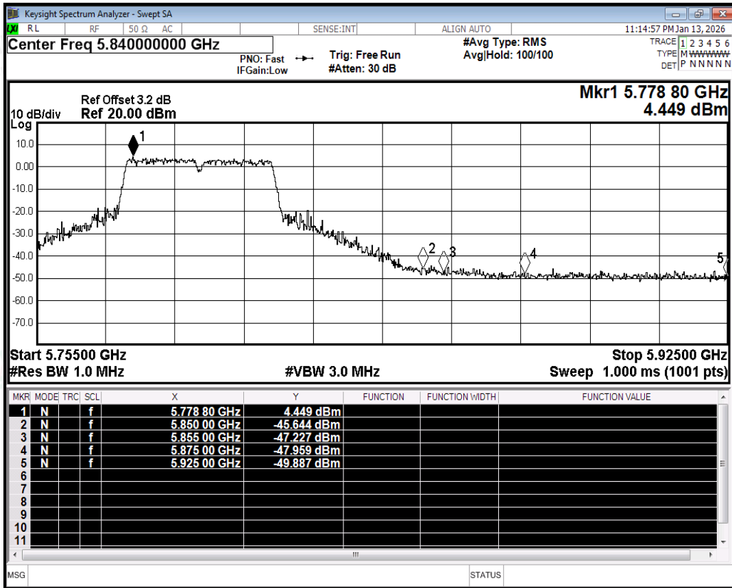
Restrict Band NVNT n40 5795MHz Ant1 Peak
