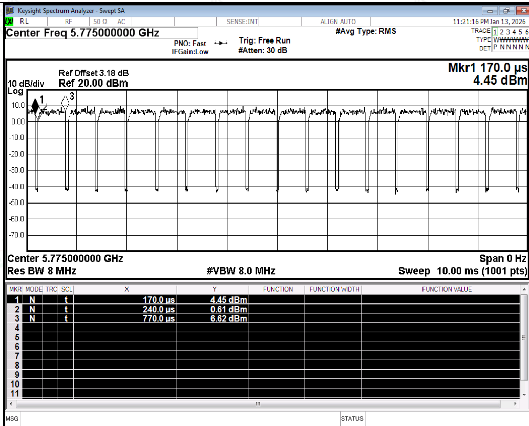
Duty Cycle NVNT ac80 5775MHz Ant1
