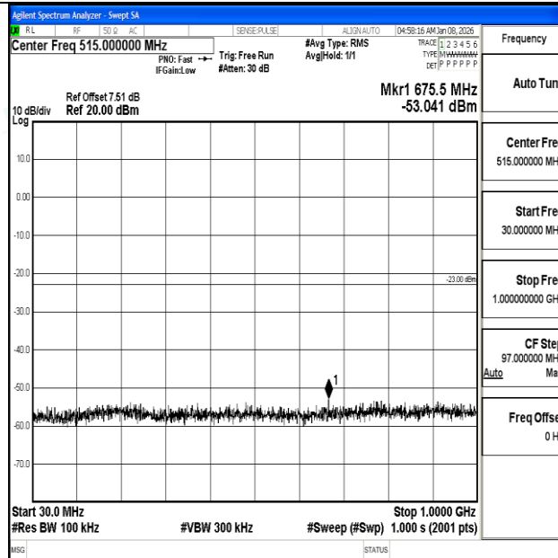
Band4_5MHz_16QAM_20175_1RB#0_30~1000_30~1000
