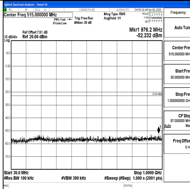
Band4_5MHz_16QAM_20375_1RB#0_30~1000_30~1000
