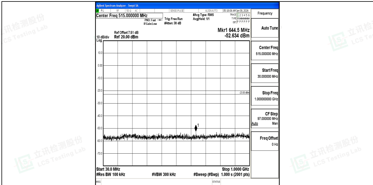
Band4_10MHz_16QAM_20175_1RB#0_30~1000_30~1000
