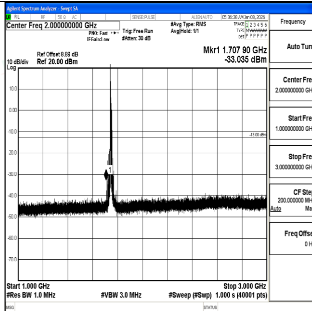
Band4_15MHz_QPSK_20325_1RB#0_1000~3000_1000~3000
