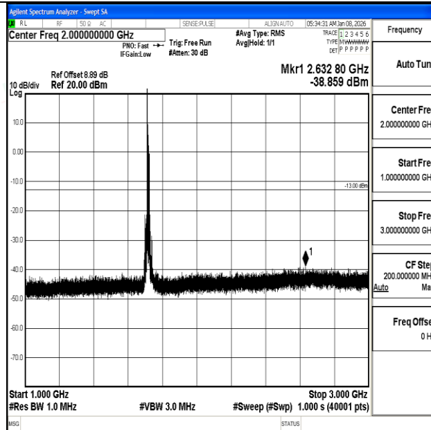
Band4_15MHz_QPSK_20025_1RB#0_1000~3000_1000~3000
