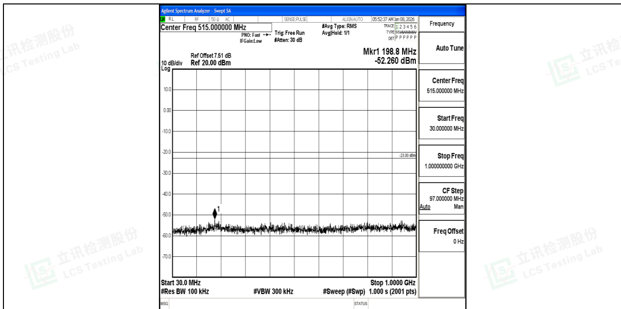
Band4_20MHz_16QAM_20050_1RB#0_30~1000_30~1000
