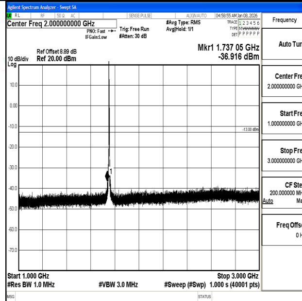
Band4_5MHz_QPSK_20375_1RB#0_1000~3000_1000~3000
