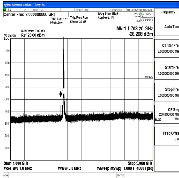
Band4_10MHz_QPSK_20350_1RB#0_1000~3000_1000~3000
