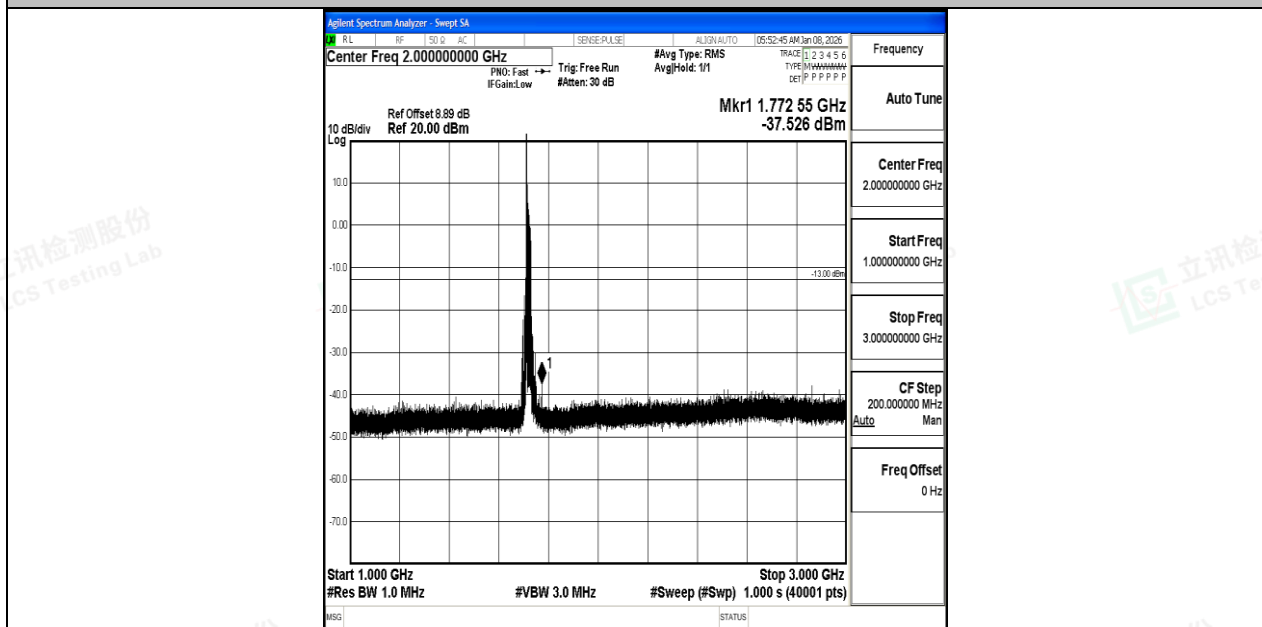
Band4_20MHz_16QAM_20050_1RB#0_1000~3000_1000~3000
