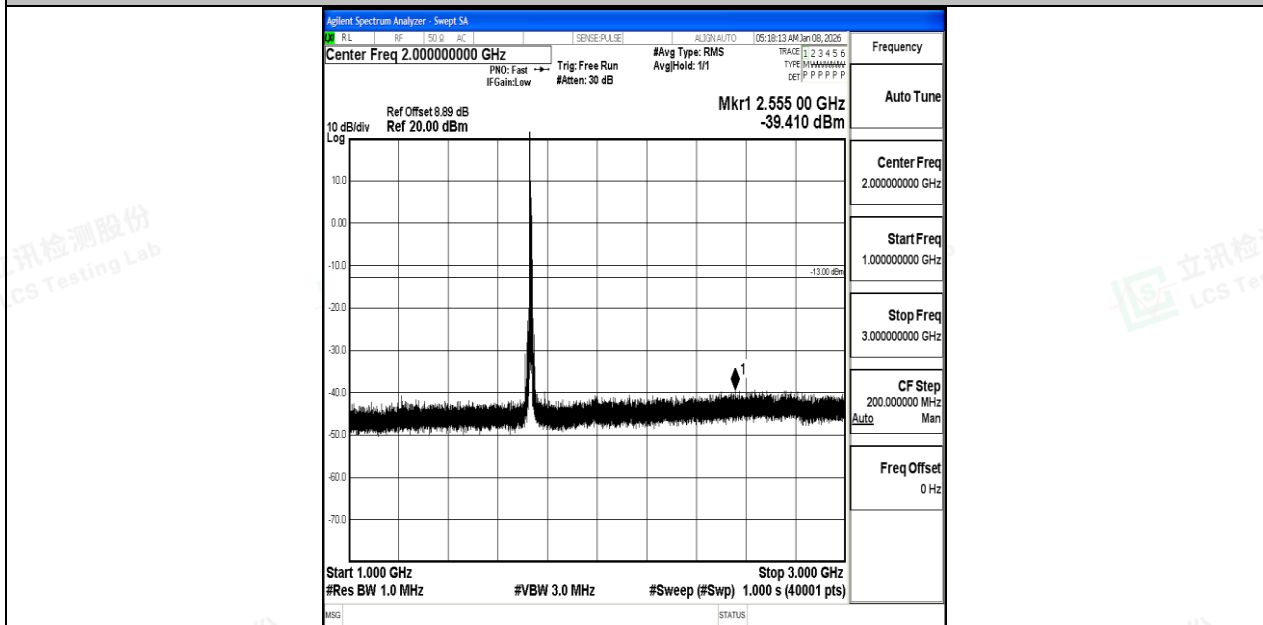
Band4_10MHz_16QAM_20175_1RB#0_1000~3000_1000~3000
