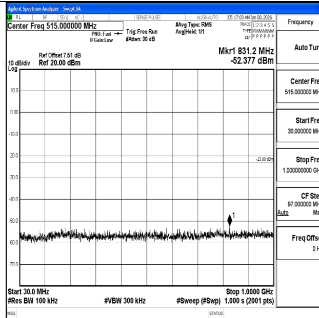
Band4_10MHz_16QAM_20000_1RB#0_30~1000_30~1000
