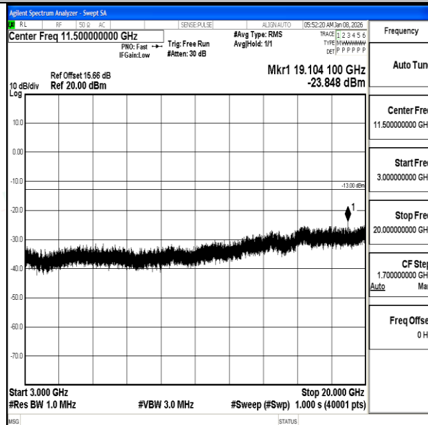
Band4_20MHz_QPSK_20050_1RB#0_3000~20000_3000~20000
