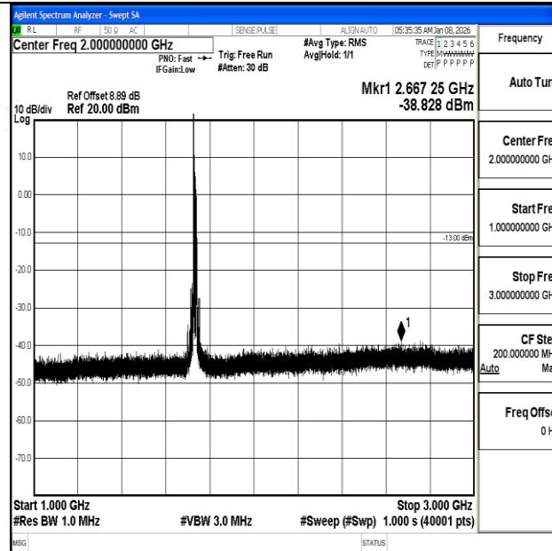
Band4_15MHz_QPSK_20175_1RB#0_1000~3000_1000~3000
