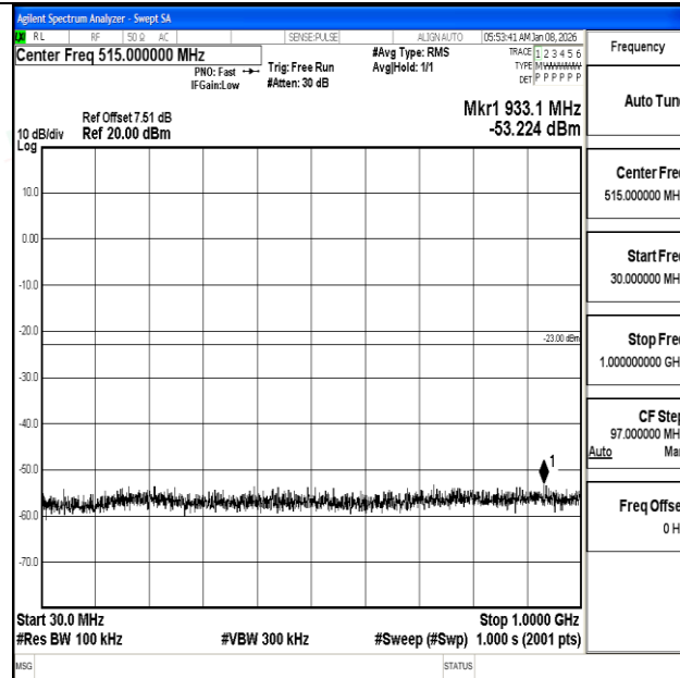
Band4_20MHz_16QAM_20175_1RB#0_30~1000_30~1000
