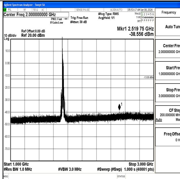
Band4_20MHz_QPSK_20175_1RB#0_1000~3000_1000~3000
