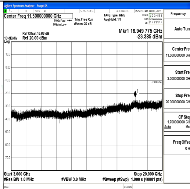
Band4_20MHz_QPSK_20175_1RB#0_3000~20000_3000~20000
