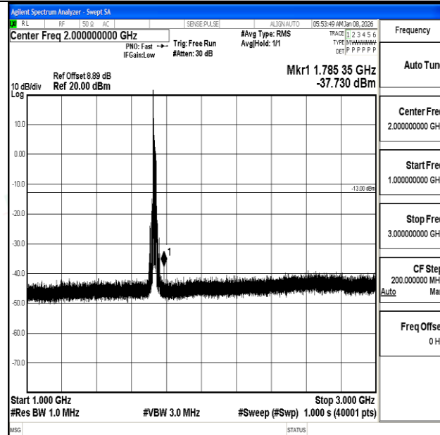
Band4_20MHz_16QAM_20175_1RB#0_1000~3000_1000~3000
