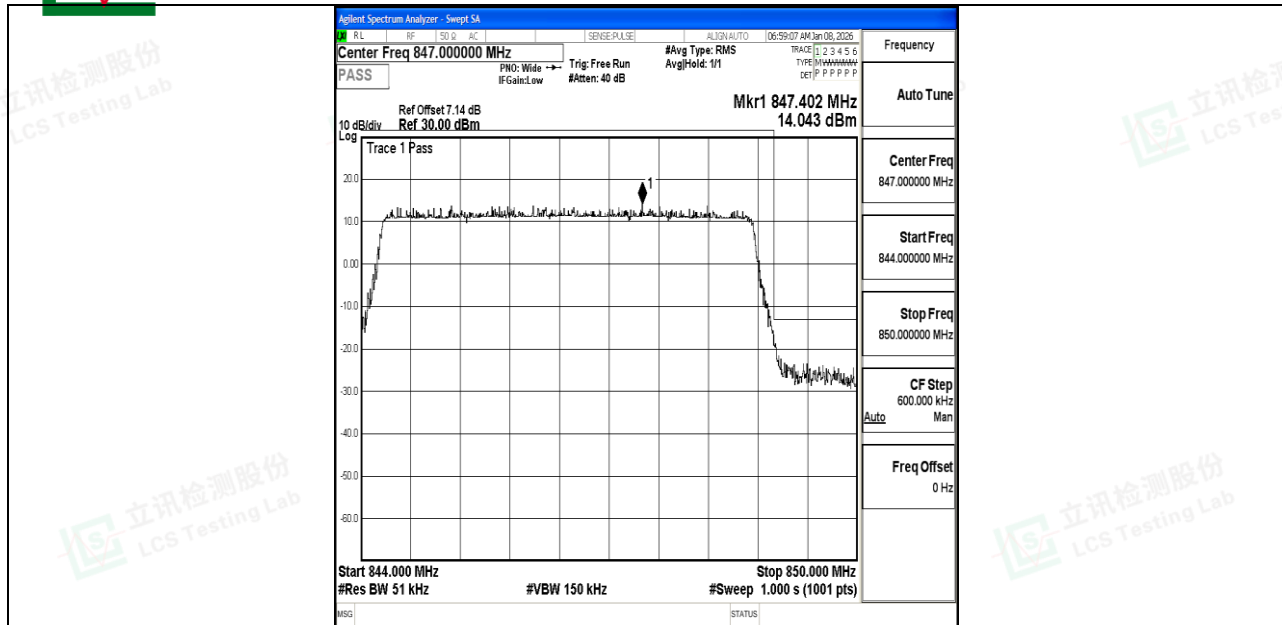
Band5_5MHz_16QAM_20625_25RB#0
