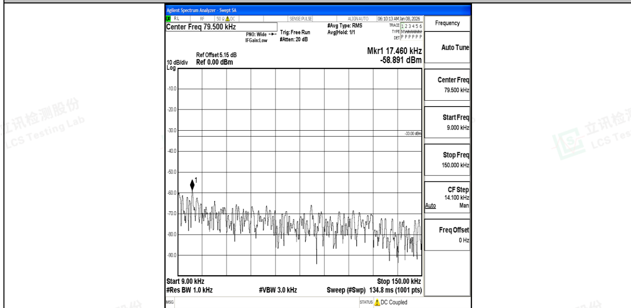
Band5_1.4MHz_16QAM_20407_1RB#0_0.009~0.15_0.009~0.15
