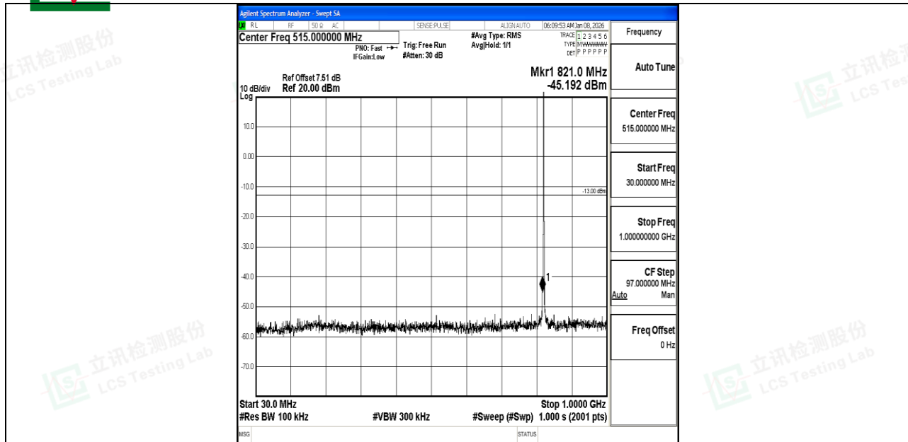
Band5_1.4MHz_QPSK_20407_1RB#0_30~1000_30~1000
