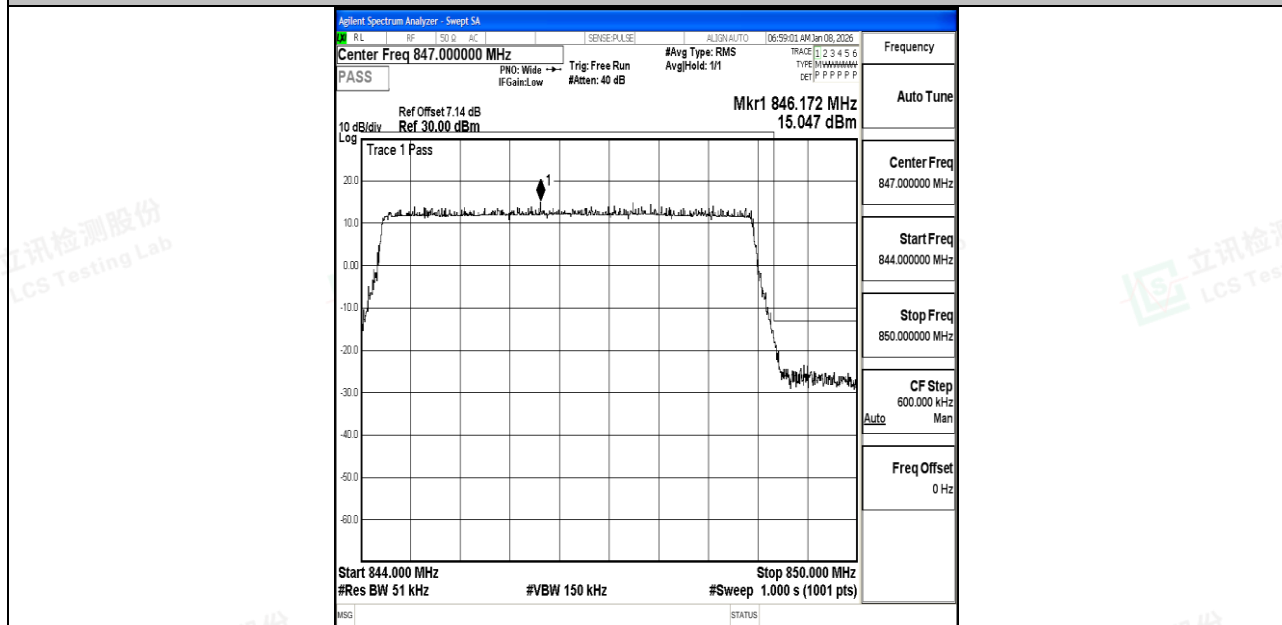
Band5_5MHz_QPSK_20625_25RB#0
