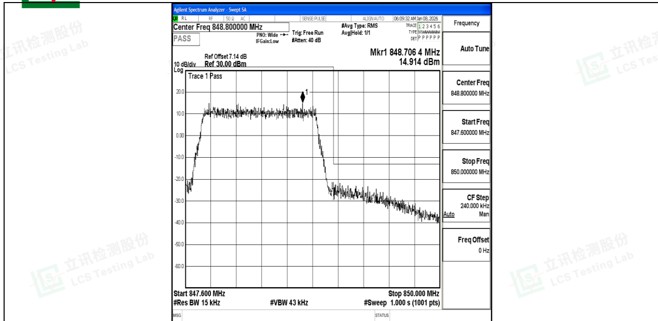
Band5_1.4MHz_16QAM_20643_6RB#0
