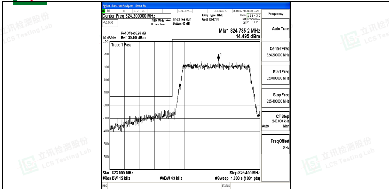
Band5_1.4MHz_16QAM_20407_6RB#0
