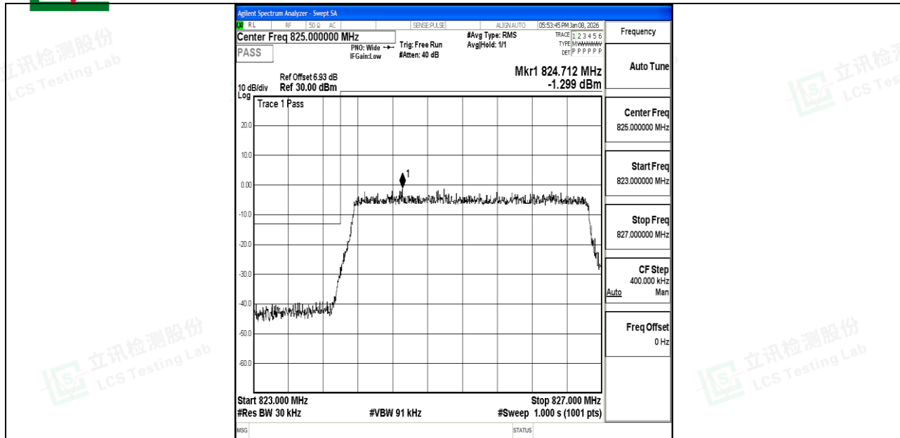
Band5_3MHz_16QAM_20415_15RB#0
