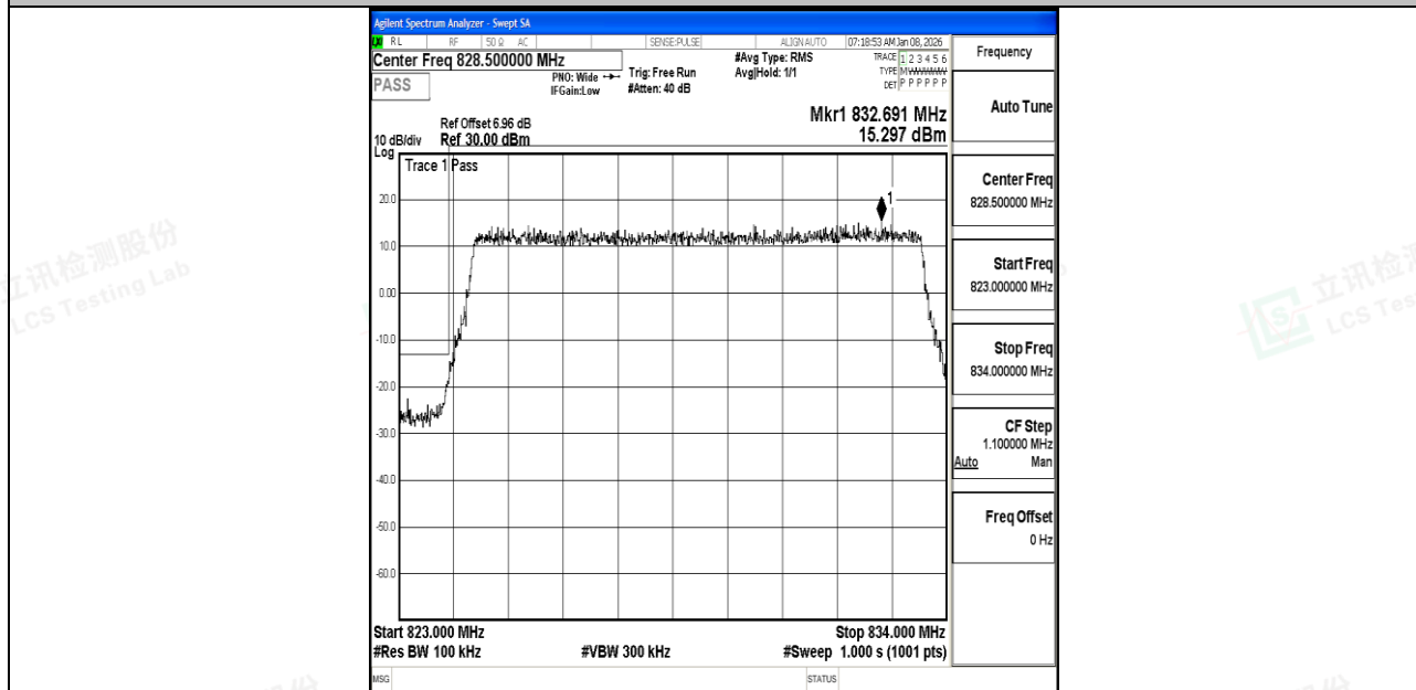
Band5_10MHz_QPSK_20450_50RB#0
