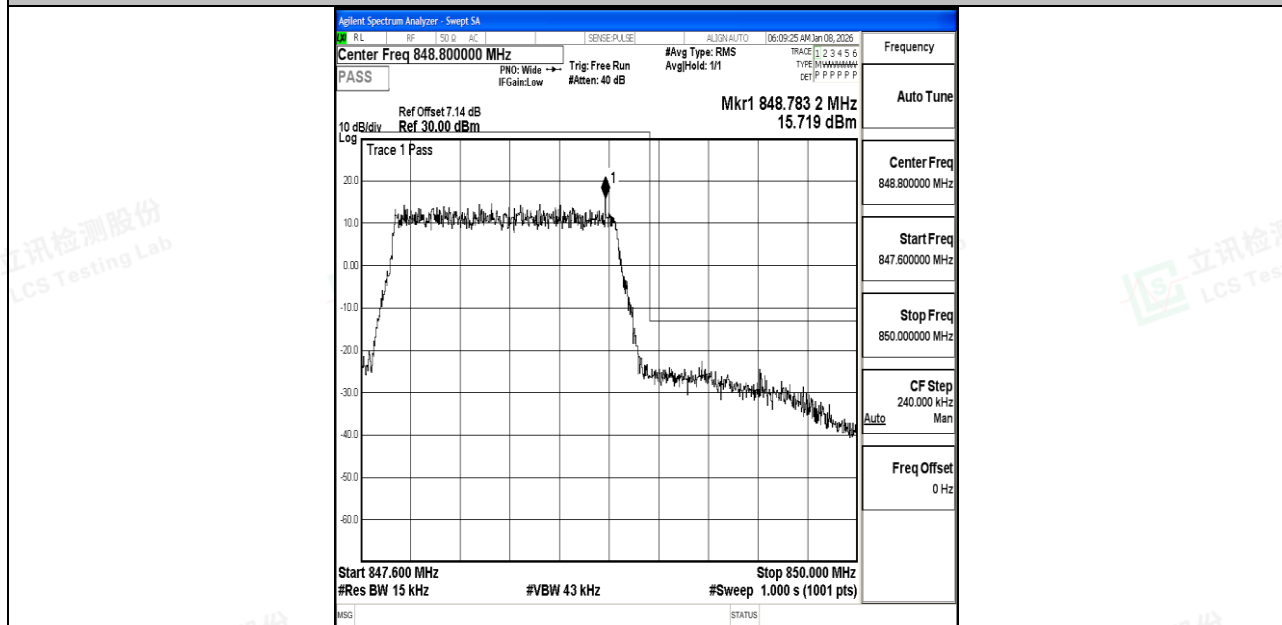
Band5_1.4MHz_QPSK_20643_6RB#0
