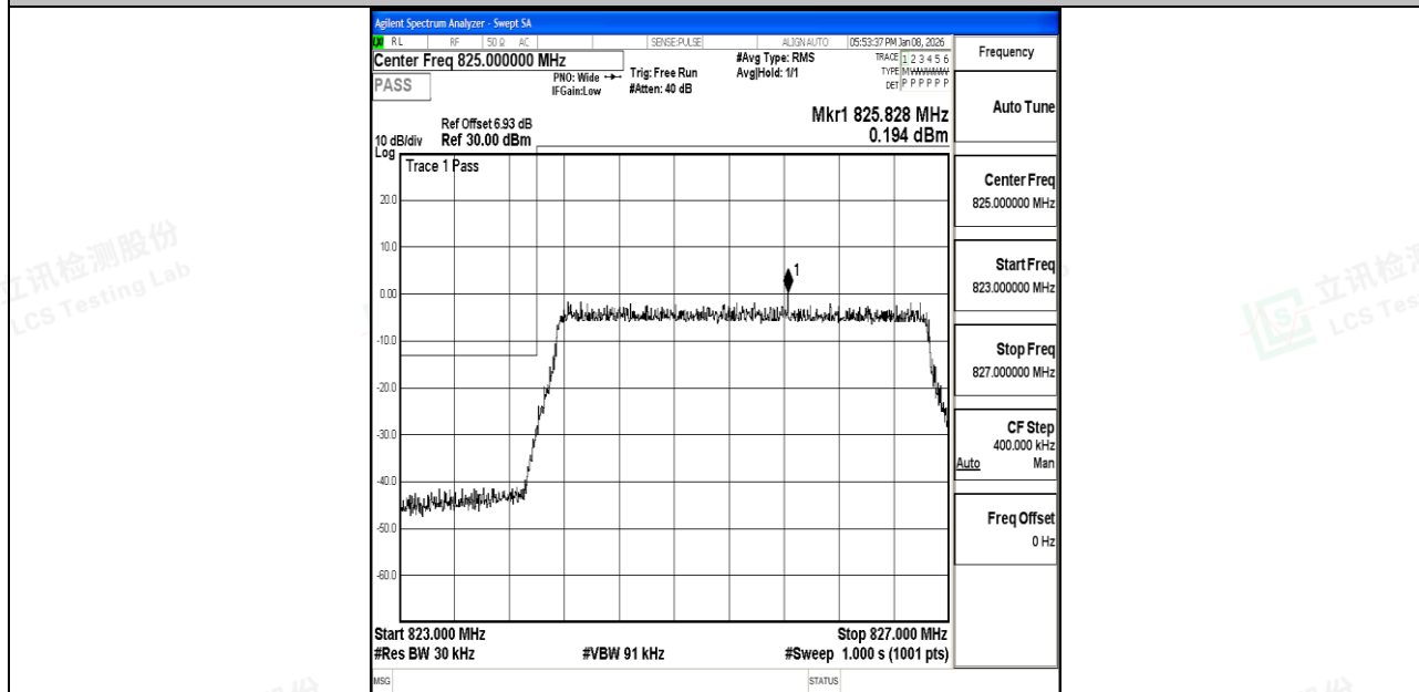
Band5_3MHz_QPSK_20415_15RB#0
