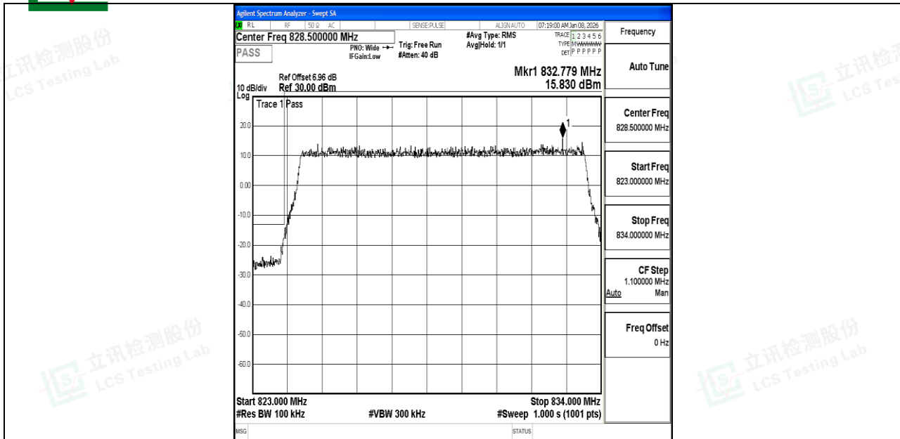
Band5_10MHz_16QAM_20450_50RB#0
