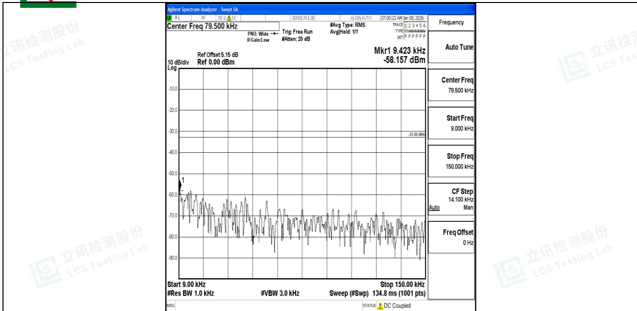
Band5_5MHz_QPSK_20525_1RB#0_0.009~0.15_0.009~0.15
