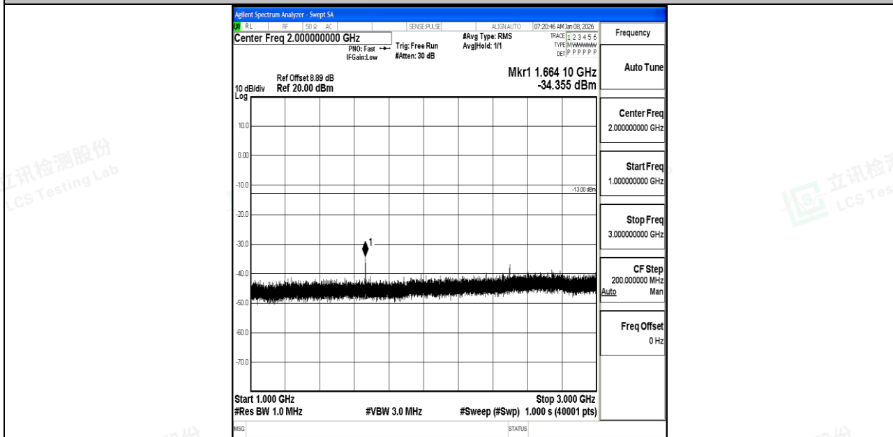
Band5_10MHz_QPSK_20525_1RB#0_1000~3000_1000~3000
