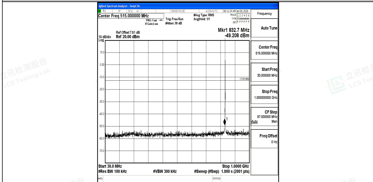
Band5_1.4MHz_16QAM_20525_1RB#0_30~1000_30~1000
