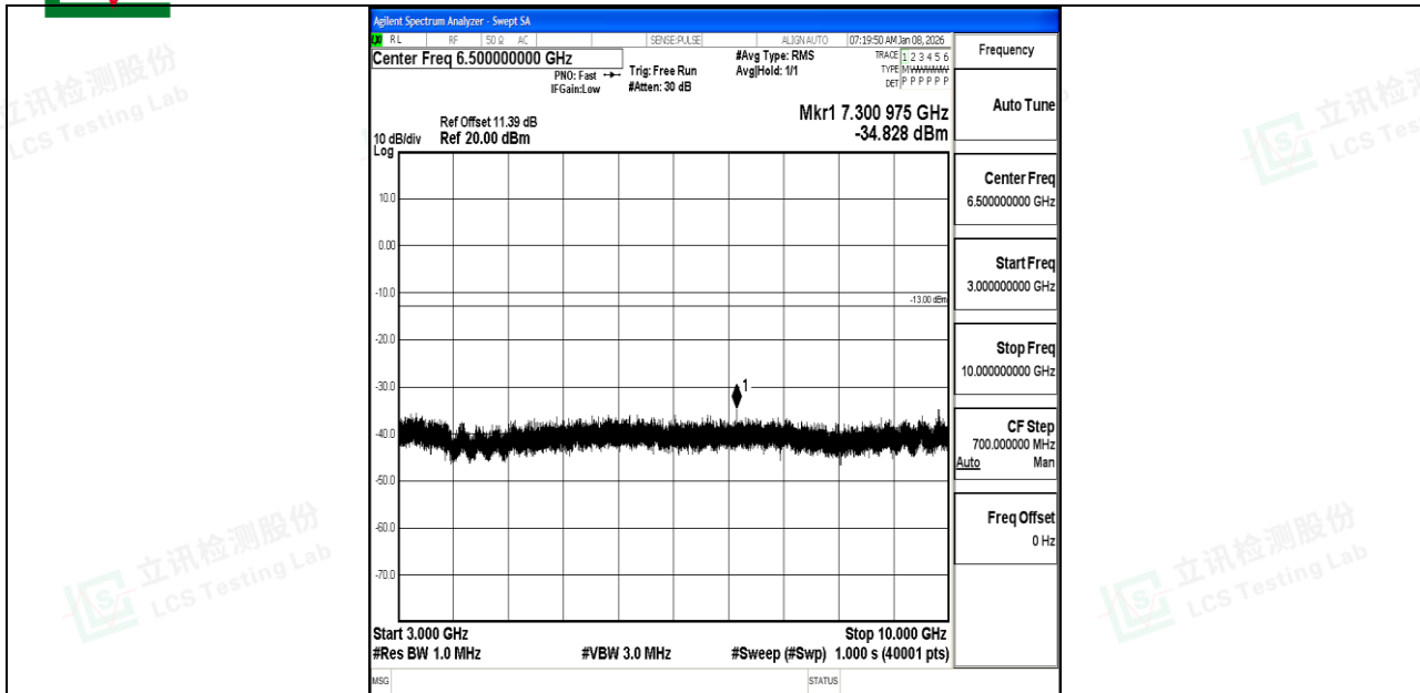
Band5_10MHz_QPSK_20450_1RB#0_3000~10000_3000~10000
