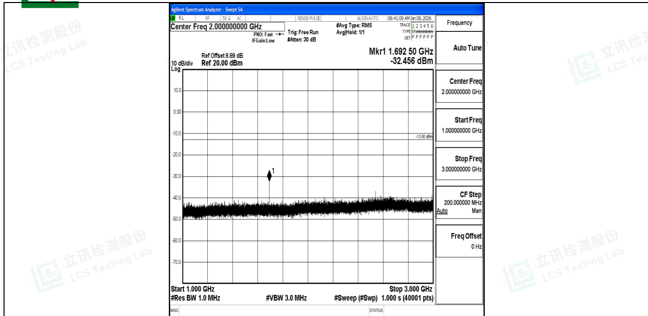
Band5_3MHz_16QAM_20635_1RB#0_1000~3000_1000~3000
