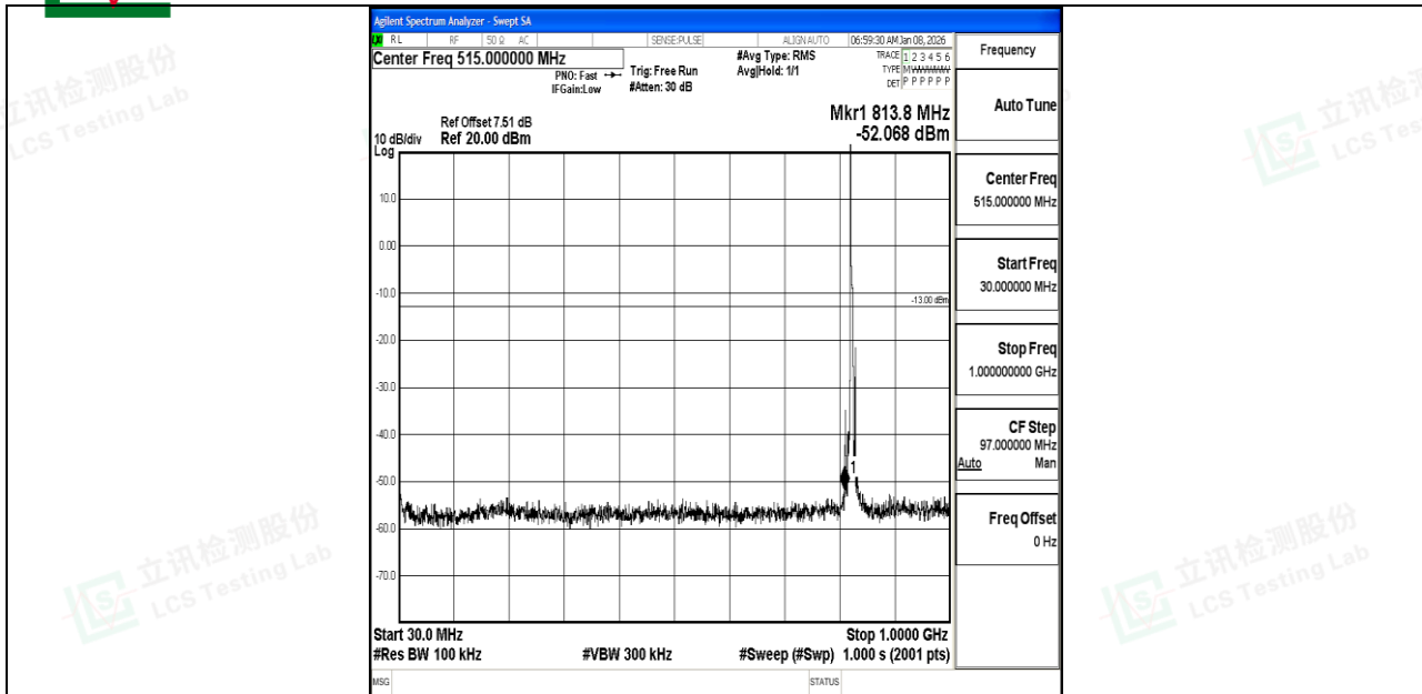
Band5_5MHz_QPSK_20425_1RB#0_30~1000_30~1000
