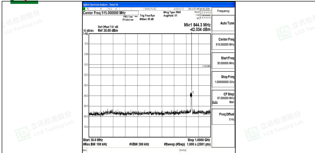
Band5_1.4MHz_QPSK_20643_1RB#0_30~1000_30~1000
