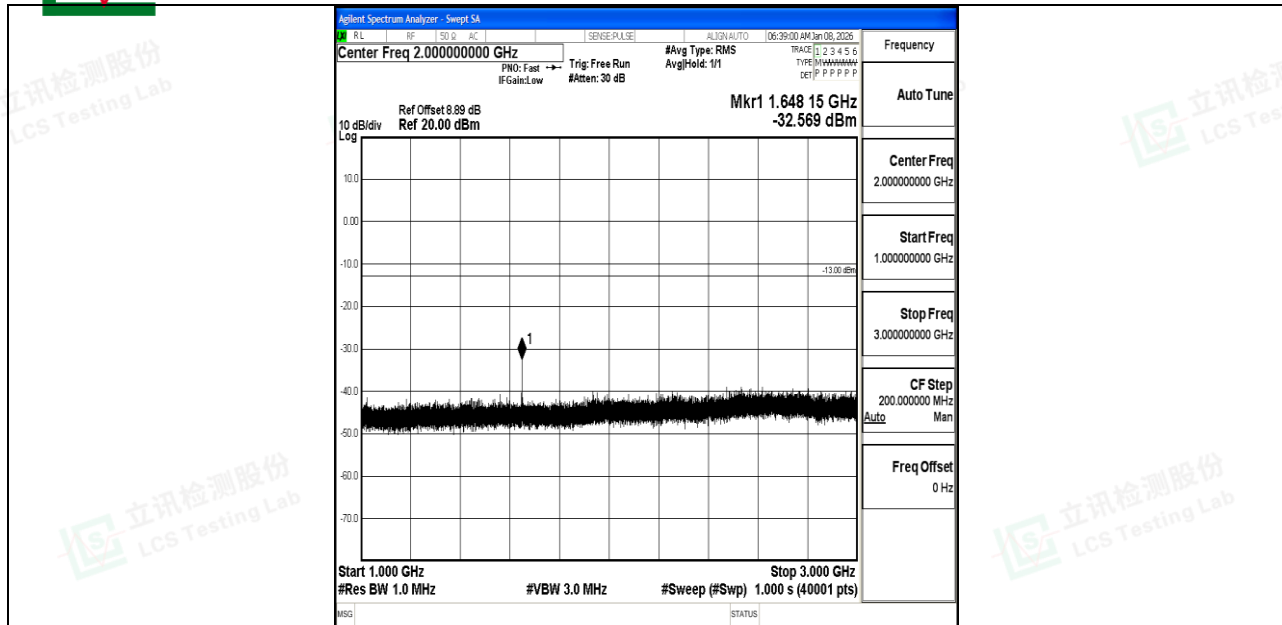
Band5_3MHz_16QAM_20415_1RB#0_1000~3000_1000~3000
