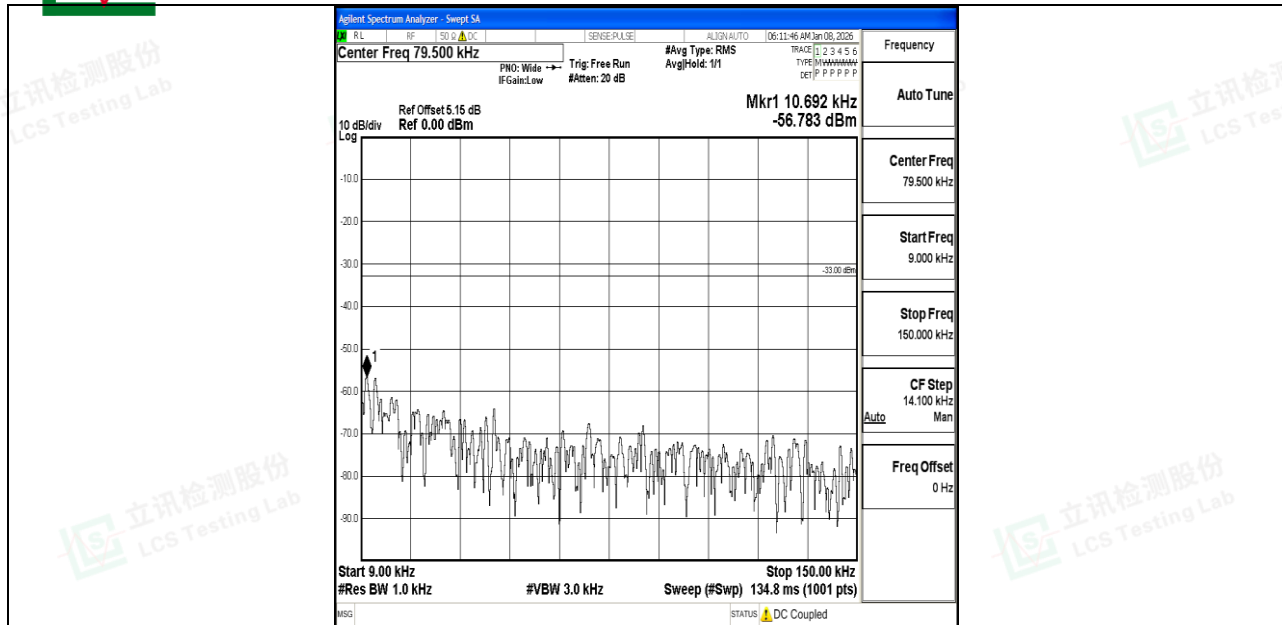
Band5_1.4MHz_QPSK_20643_1RB#0_0.009~0.15_0.009~0.15
