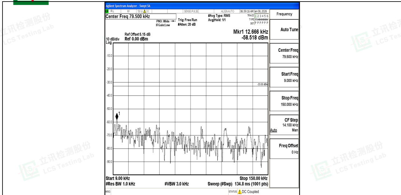
Band5_3MHz_QPSK_20525_1RB#0_0.009~0.15_0.009~0.15
