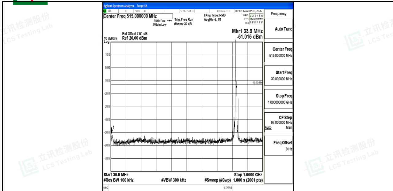
Band5_10MHz_QPSK_20450_1RB#0_30~1000_30~1000
