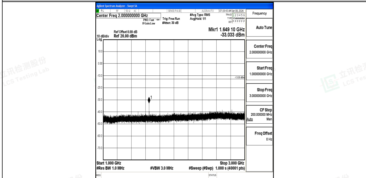
Band5_10MHz_QPSK_20450_1RB#0_1000~3000_1000~3000
