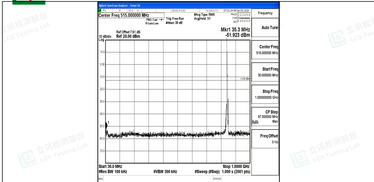
Band5_5MHz_QPSK_20625_1RB#0_30~1000_30~1000
