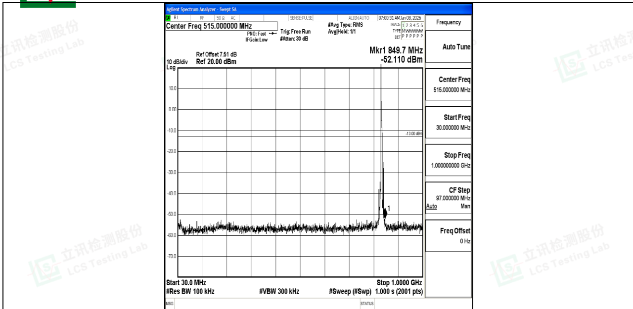
Band5_5MHz_QPSK_20525_1RB#0_30~1000_30~1000
