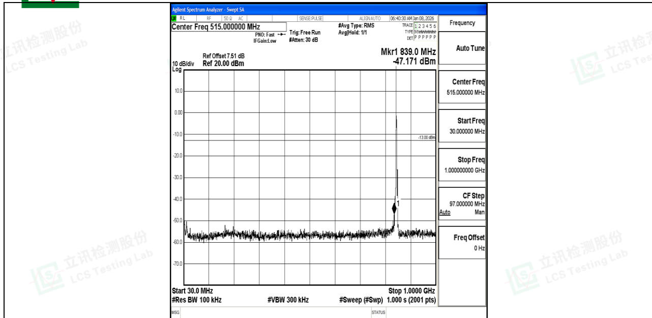
Band5_3MHz_QPSK_20635_1RB#0_30~1000_30~1000
