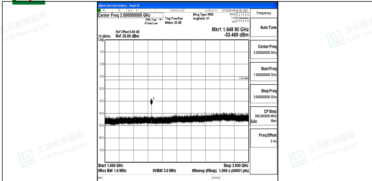
Band5_5MHz_16QAM_20425_1RB#0_1000~3000_1000~3000
