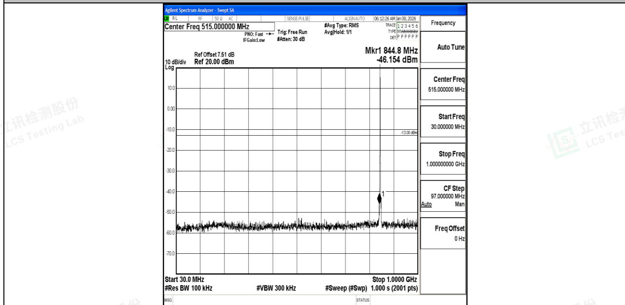
Band5_1.4MHz_16QAM_20643_1RB#0_30~1000_30~1000
