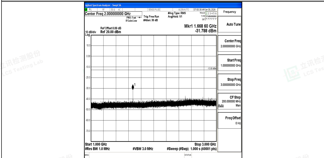
Band5_5MHz_QPSK_20525_1RB#0_1000~3000_1000~3000
