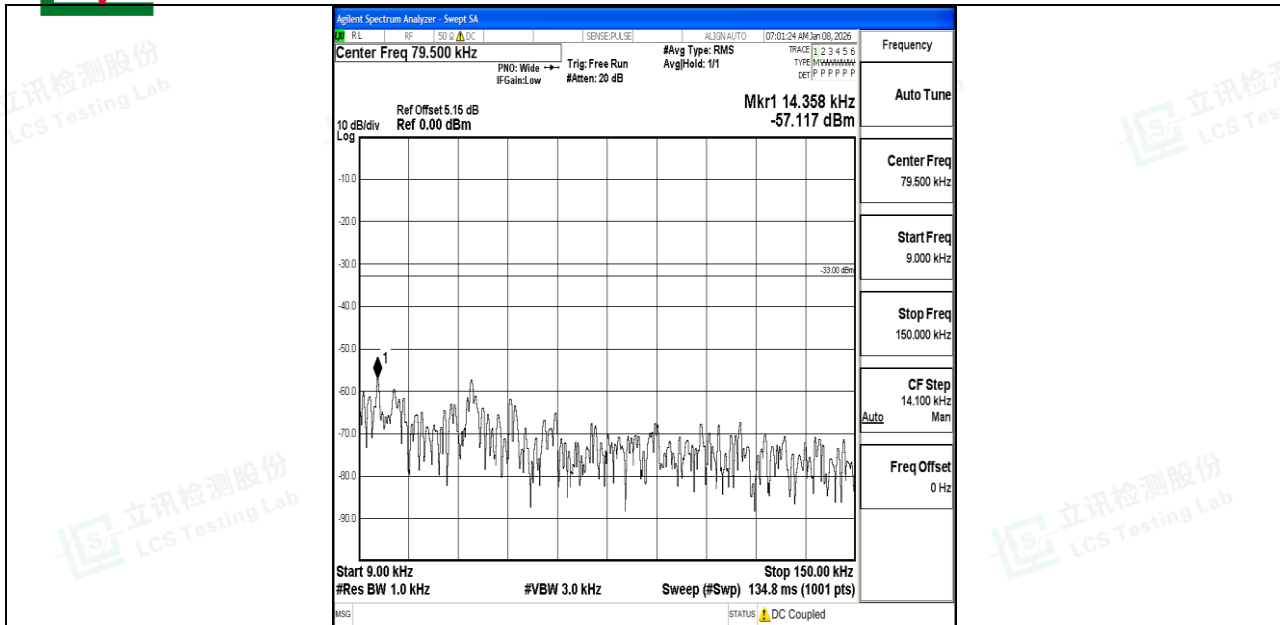
Band5_5MHz_QPSK_20625_1RB#0_0.009~0.15_0.009~0.15
