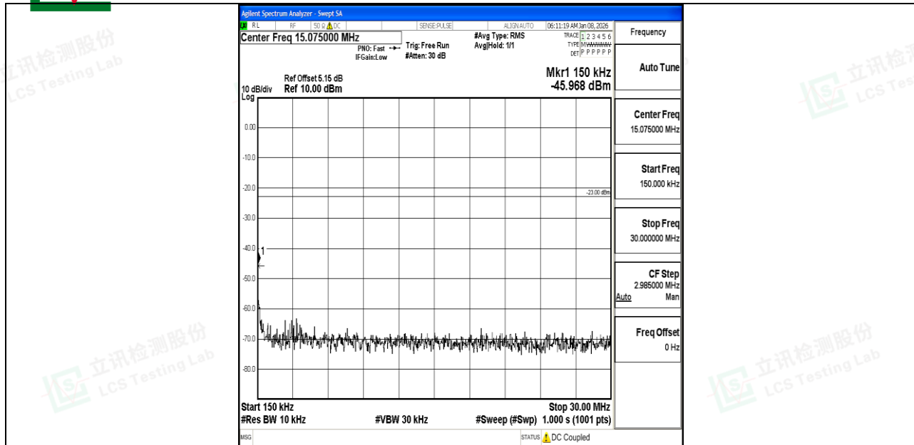
Band5_1.4MHz_16QAM_20525_1RB#0_0.15~30_0.15~30
