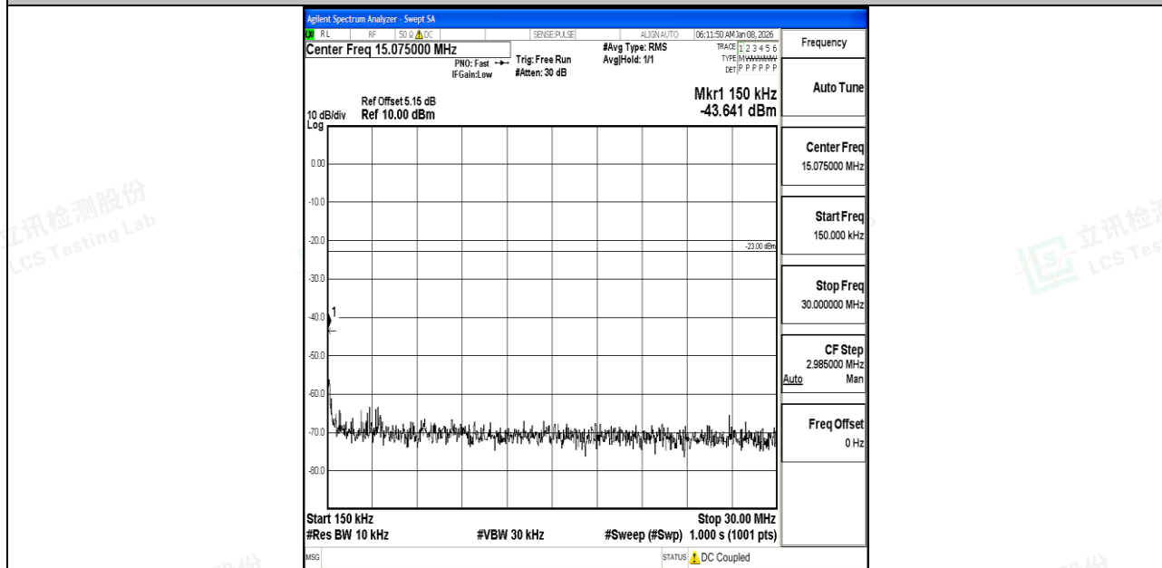
Band5_1.4MHz_QPSK_20643_1RB#0_0.15~30_0.15~30
