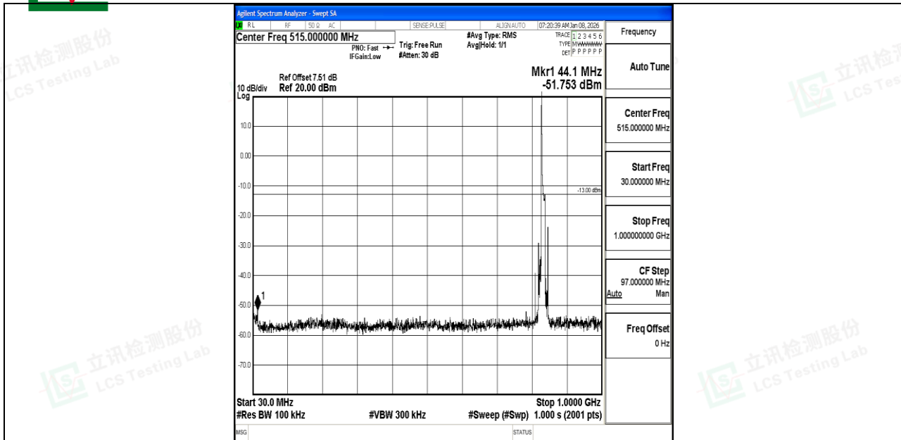
Band5_10MHz_QPSK_20525_1RB#0_30~1000_30~1000
