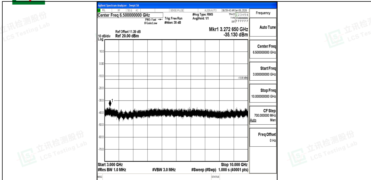
Band5_5MHz_QPSK_20425_1RB#0_3000~10000_3000~10000
