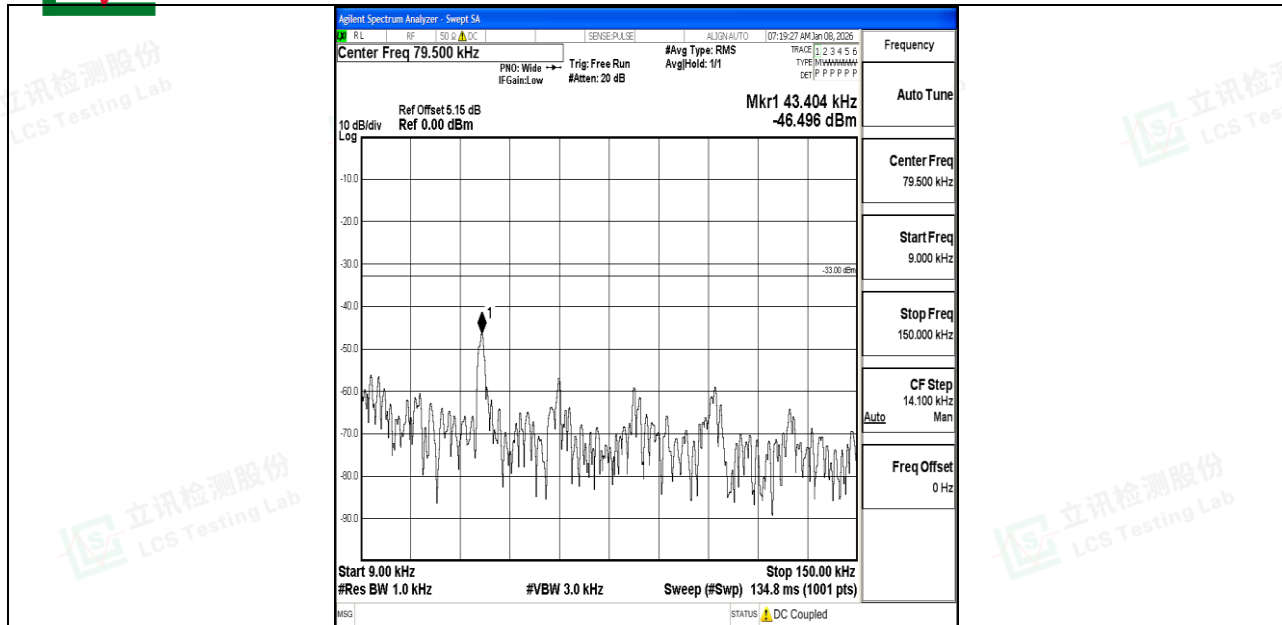
Band5_10MHz_QPSK_20450_1RB#0_0.009~0.15_0.009~0.15
