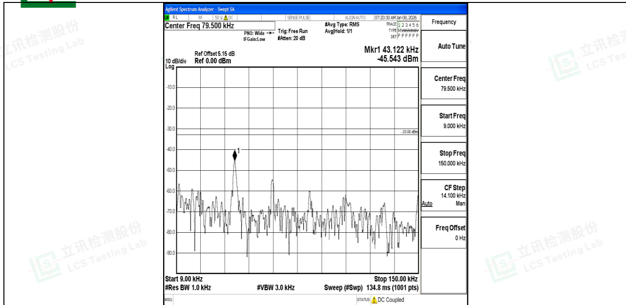
Band5_10MHz_QPSK_20525_1RB#0_0.009~0.15_0.009~0.15
