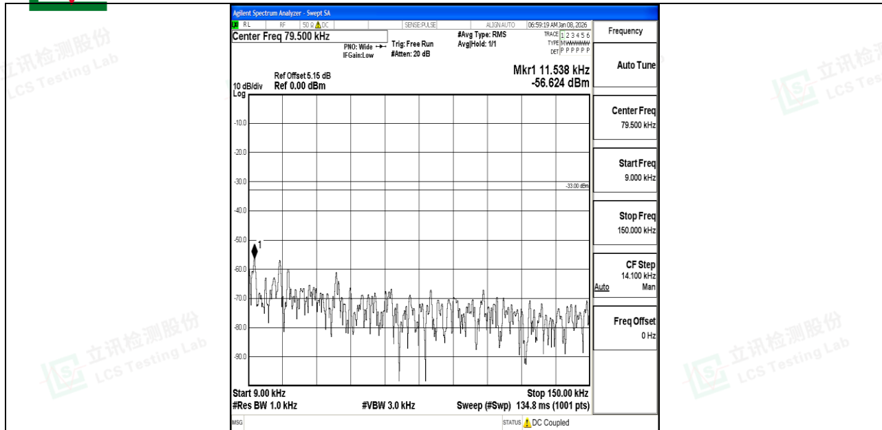
Band5_5MHz_QPSK_20425_1RB#0_0.009~0.15_0.009~0.15
