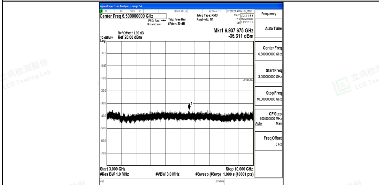
Band5_10MHz_16QAM_20450_1RB#0_3000~10000_3000~10000
