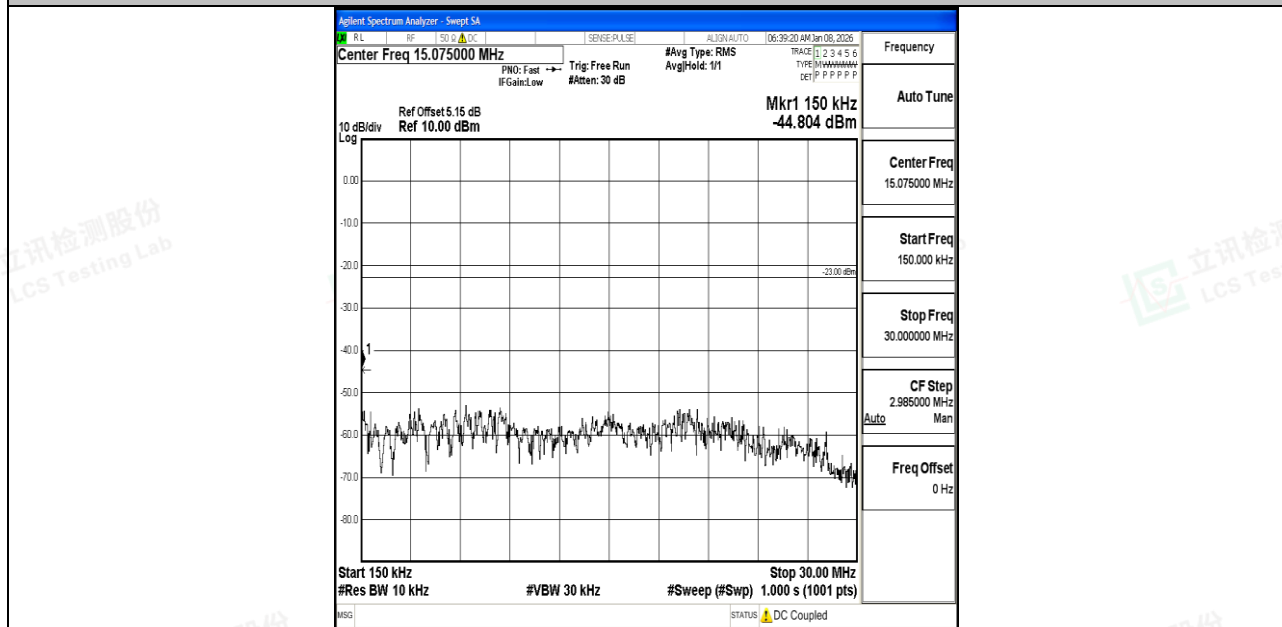
Band5_3MHz_QPSK_20525_1RB#0_0.15~30_0.15~30
