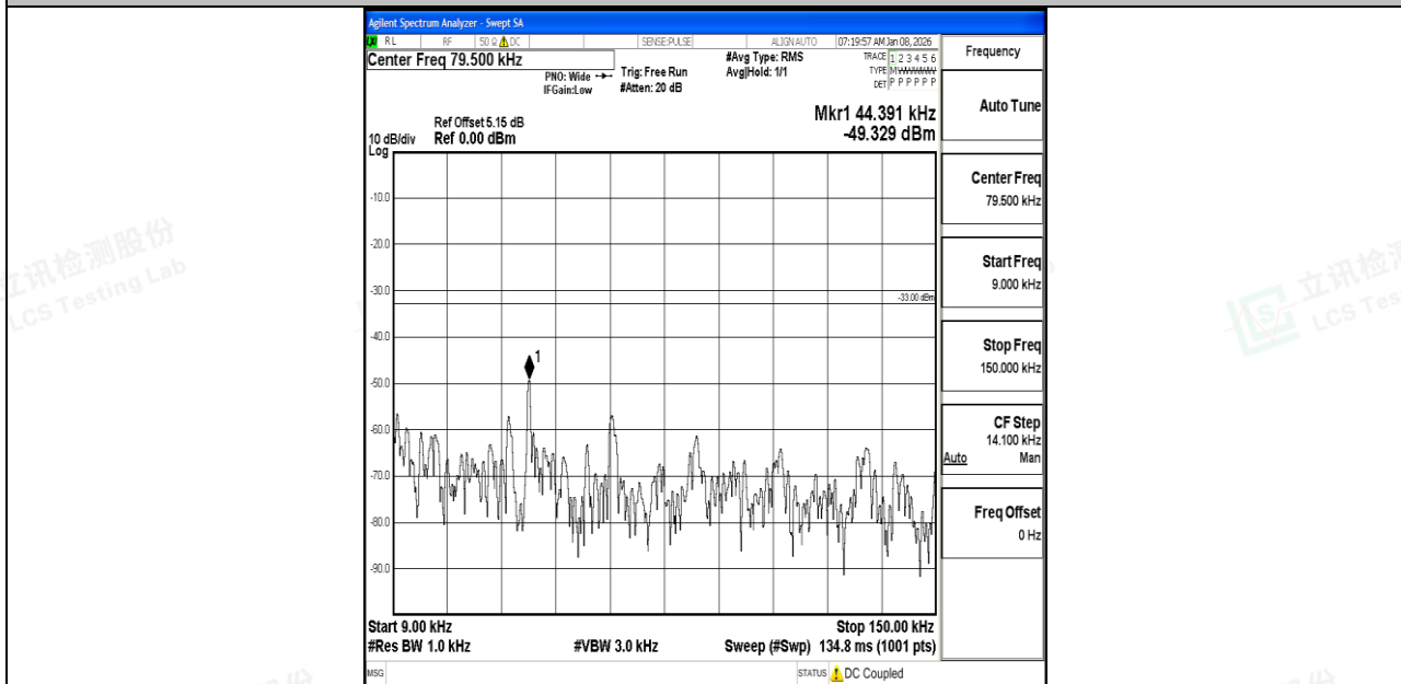
Band5_10MHz_16QAM_20450_1RB#0_0.009~0.15_0.009~0.15
