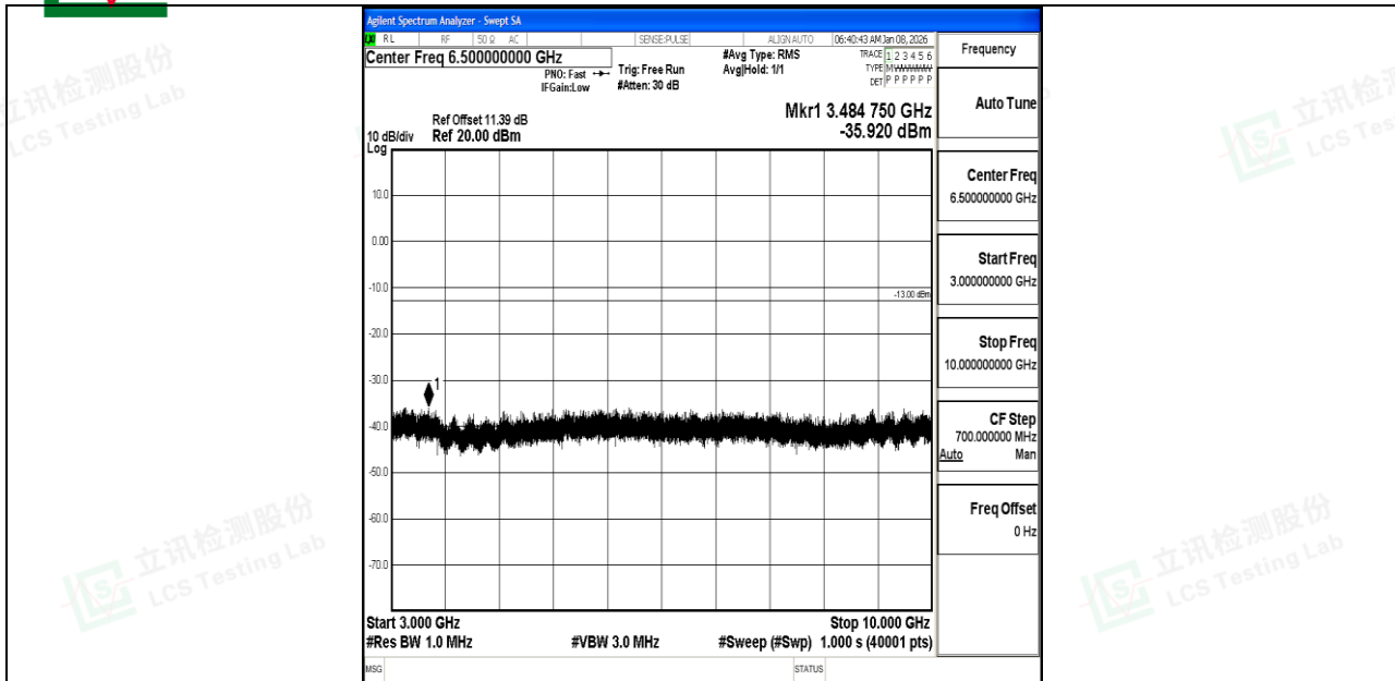
Band5_3MHz_QPSK_20635_1RB#0_3000~10000_3000~10000
