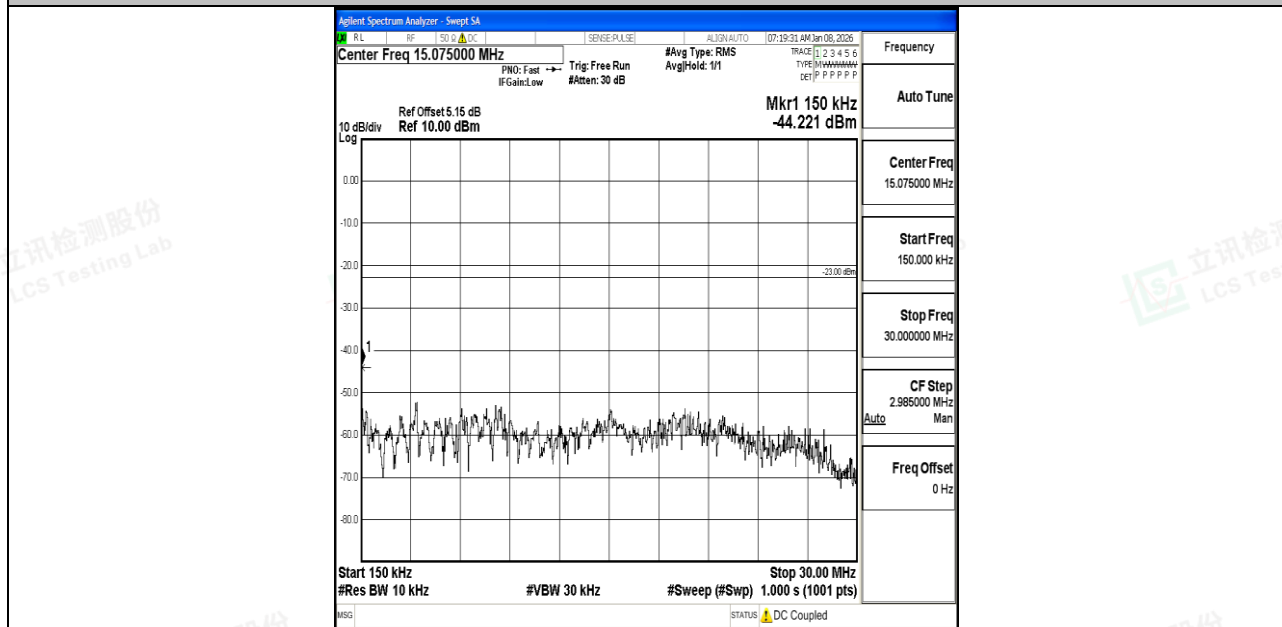
Band5_10MHz_QPSK_20450_1RB#0_0.15~30_0.15~30
