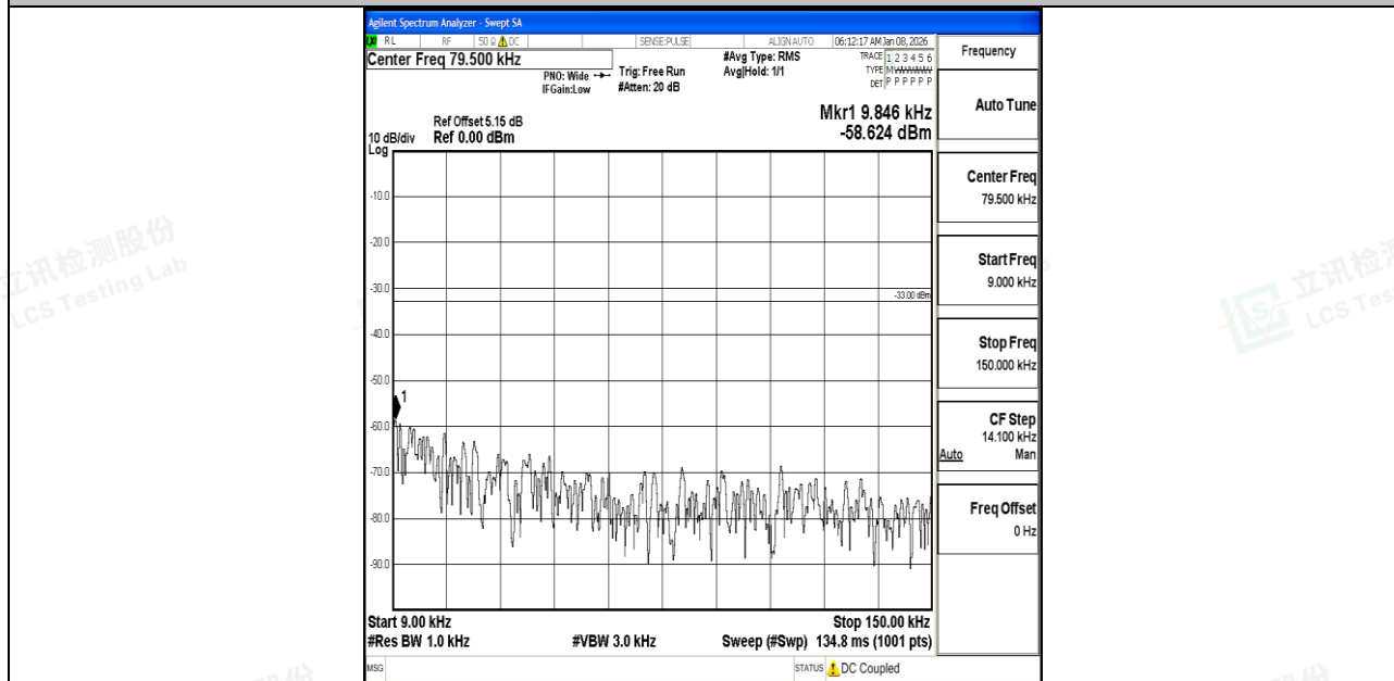
Band5_1.4MHz_16QAM_20643_1RB#0_0.009~0.15_0.009~0.15
