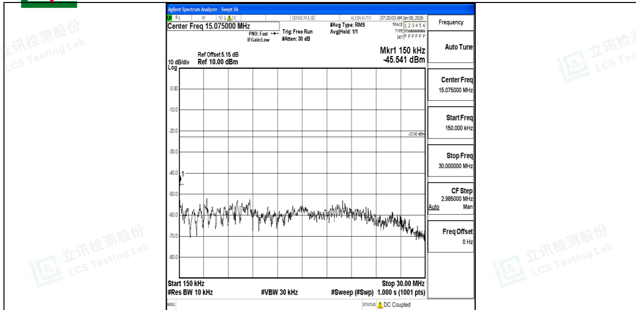
Band5_10MHz_16QAM_20450_1RB#0_0.15~30_0.15~30
