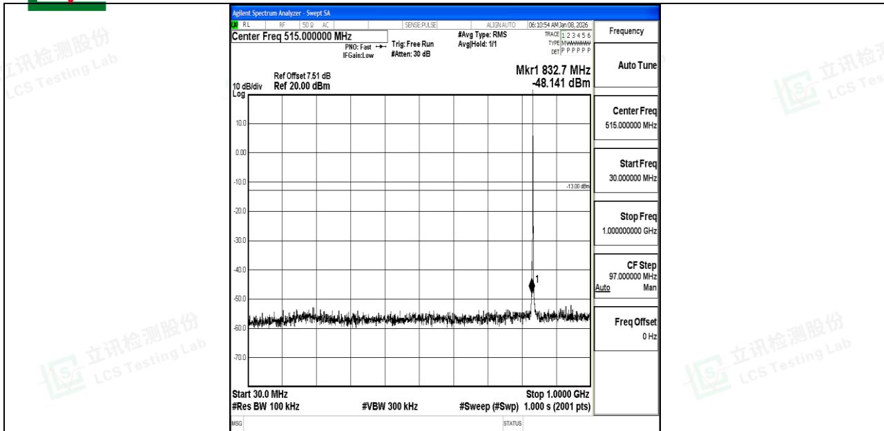
Band5_1.4MHz_QPSK_20525_1RB#0_30~1000_30~1000
