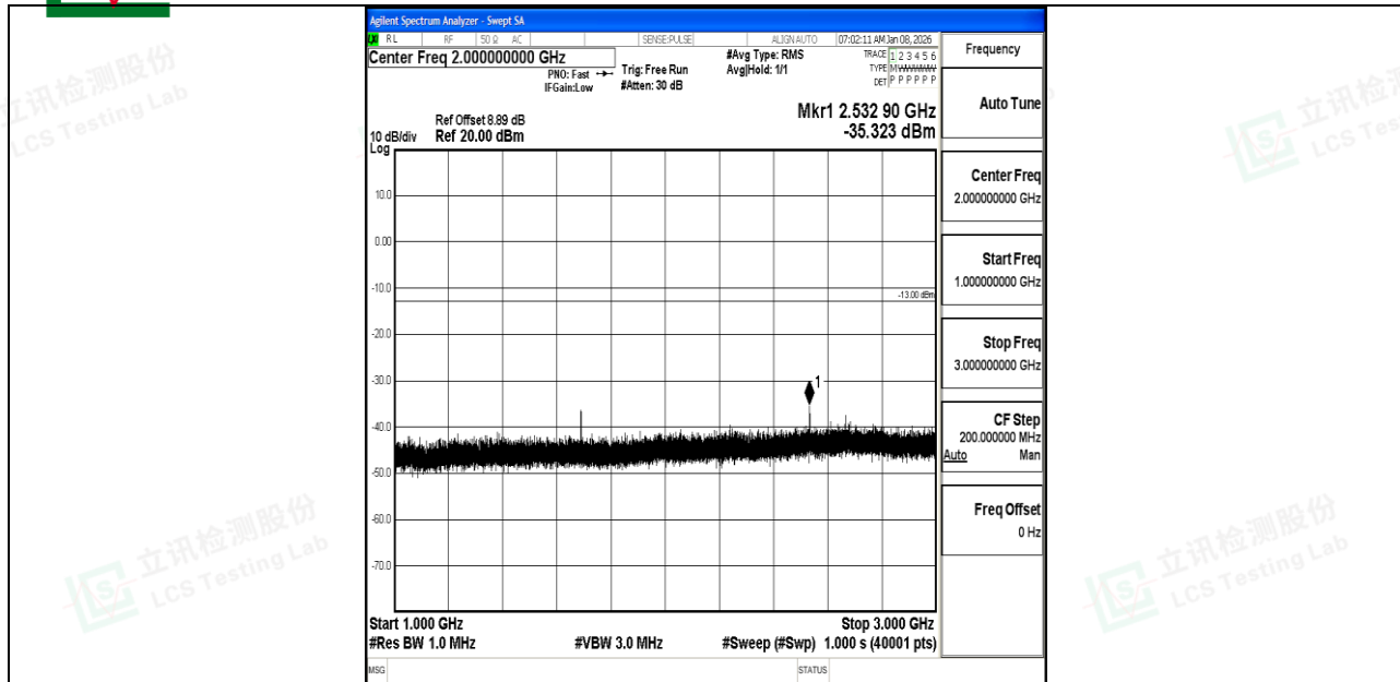
Band5_5MHz_16QAM_20625_1RB#0_1000~3000_1000~3000
