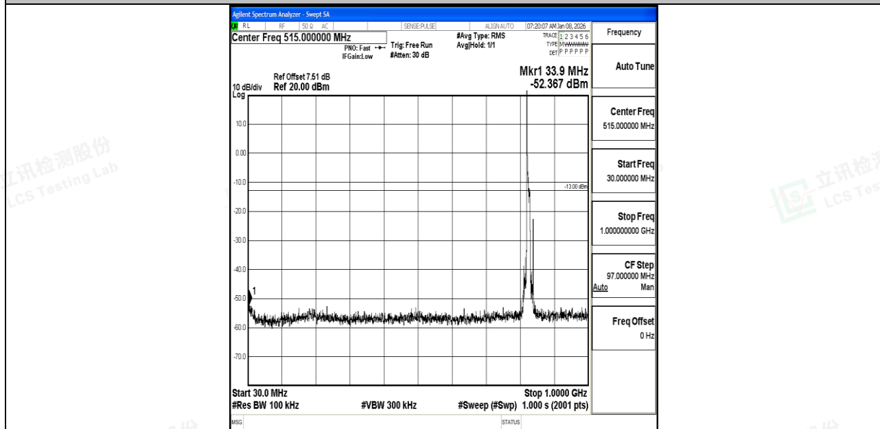
Band5_10MHz_16QAM_20450_1RB#0_30~1000_30~1000
