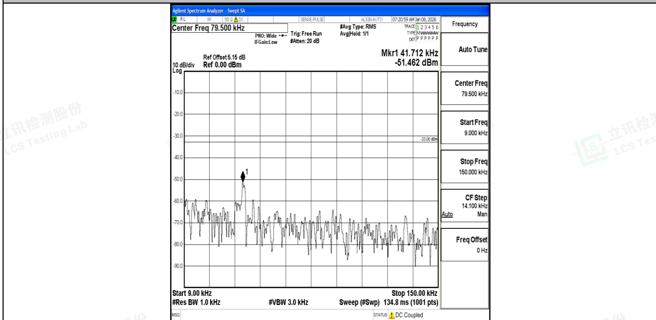
Band5_10MHz_16QAM_20525_1RB#0_0.009~0.15_0.009~0.15
