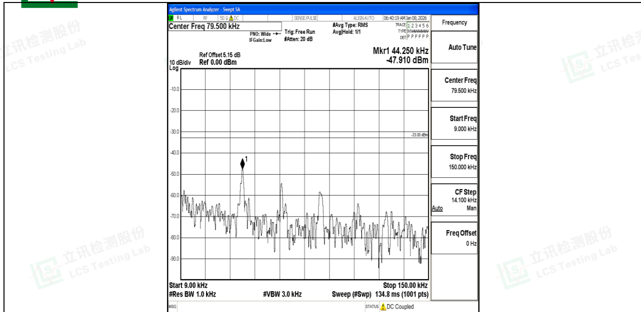
Band5_3MHz_QPSK_20635_1RB#0_0.009~0.15_0.009~0.15
