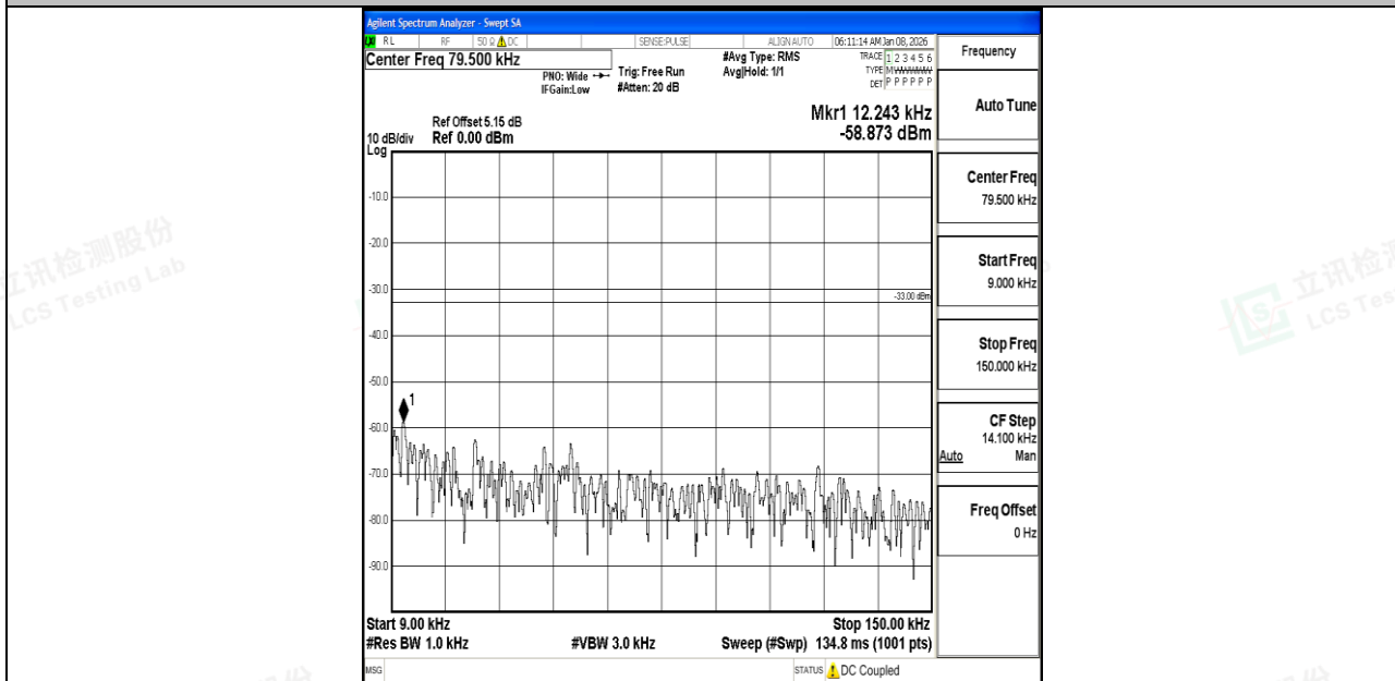
Band5_1.4MHz_16QAM_20525_1RB#0_0.009~0.15_0.009~0.15
