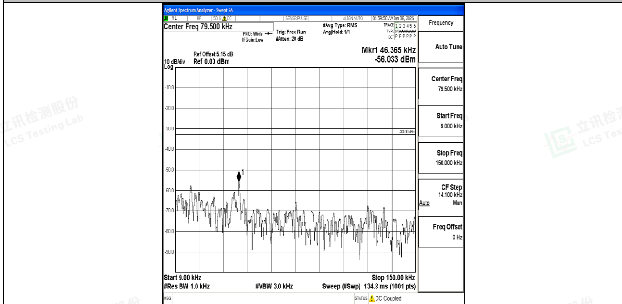
Band5_5MHz_16QAM_20425_1RB#0_0.009~0.15_0.009~0.15
