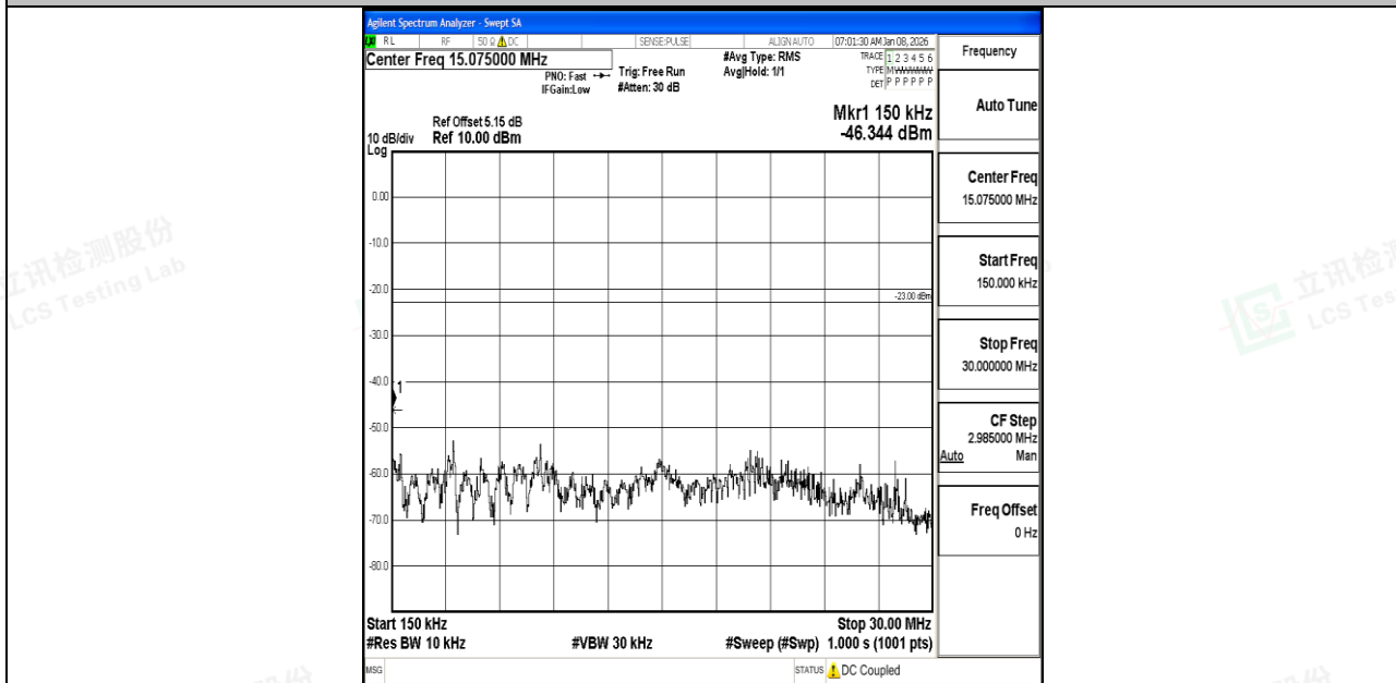
Band5_5MHz_QPSK_20625_1RB#0_0.15~30_0.15~30
