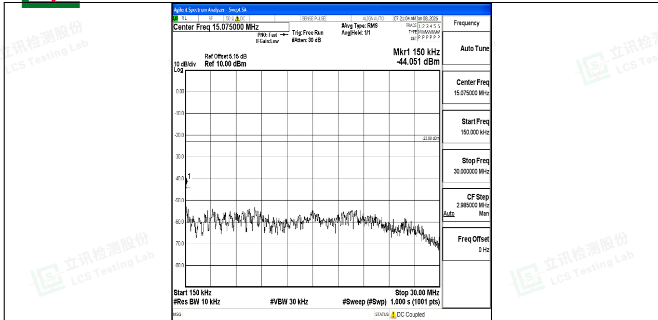
Band5_10MHz_16QAM_20525_1RB#0_0.15~30_0.15~30
