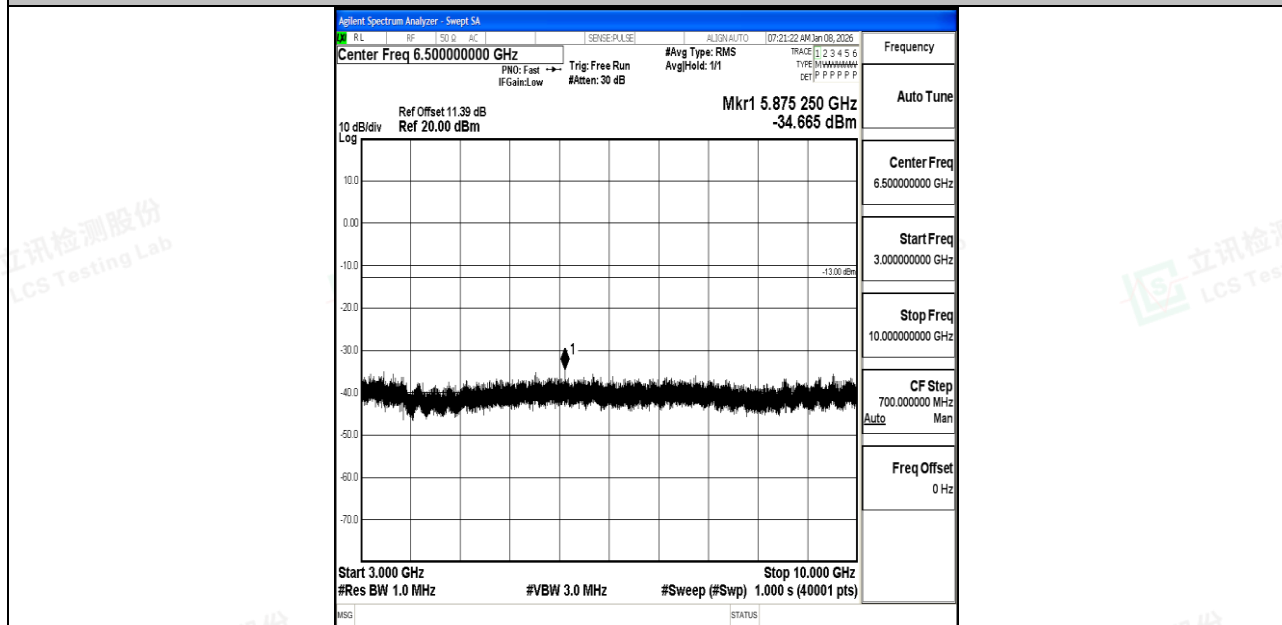
Band5_10MHz_16QAM_20525_1RB#0_3000~10000_3000~10000
