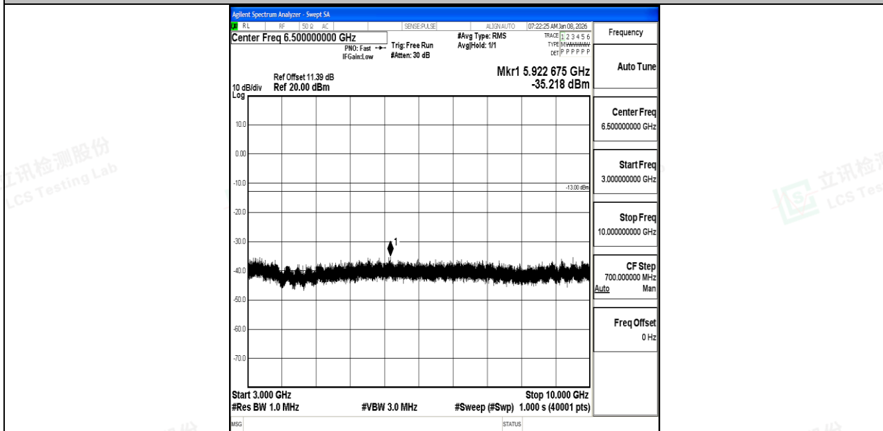
Band5_10MHz_16QAM_20600_1RB#0_3000~10000_3000~10000
