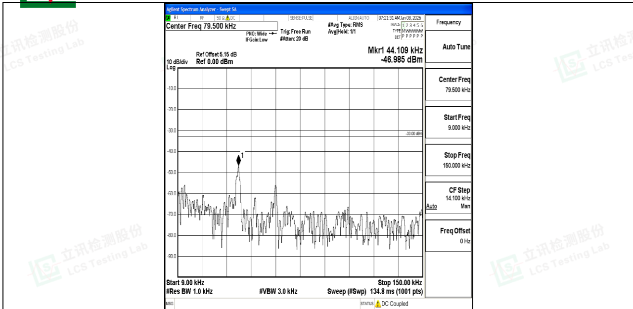
Band5_10MHz_QPSK_20600_1RB#0_0.009~0.15_0.009~0.15
