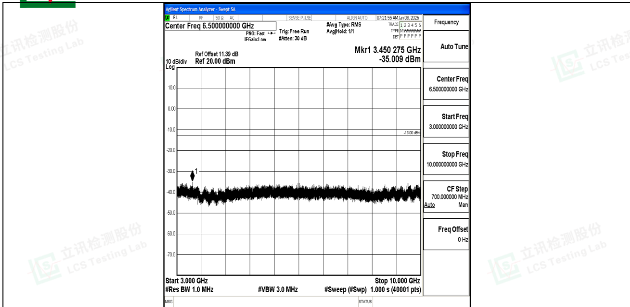
Band5_10MHz_QPSK_20600_1RB#0_3000~10000_3000~10000
