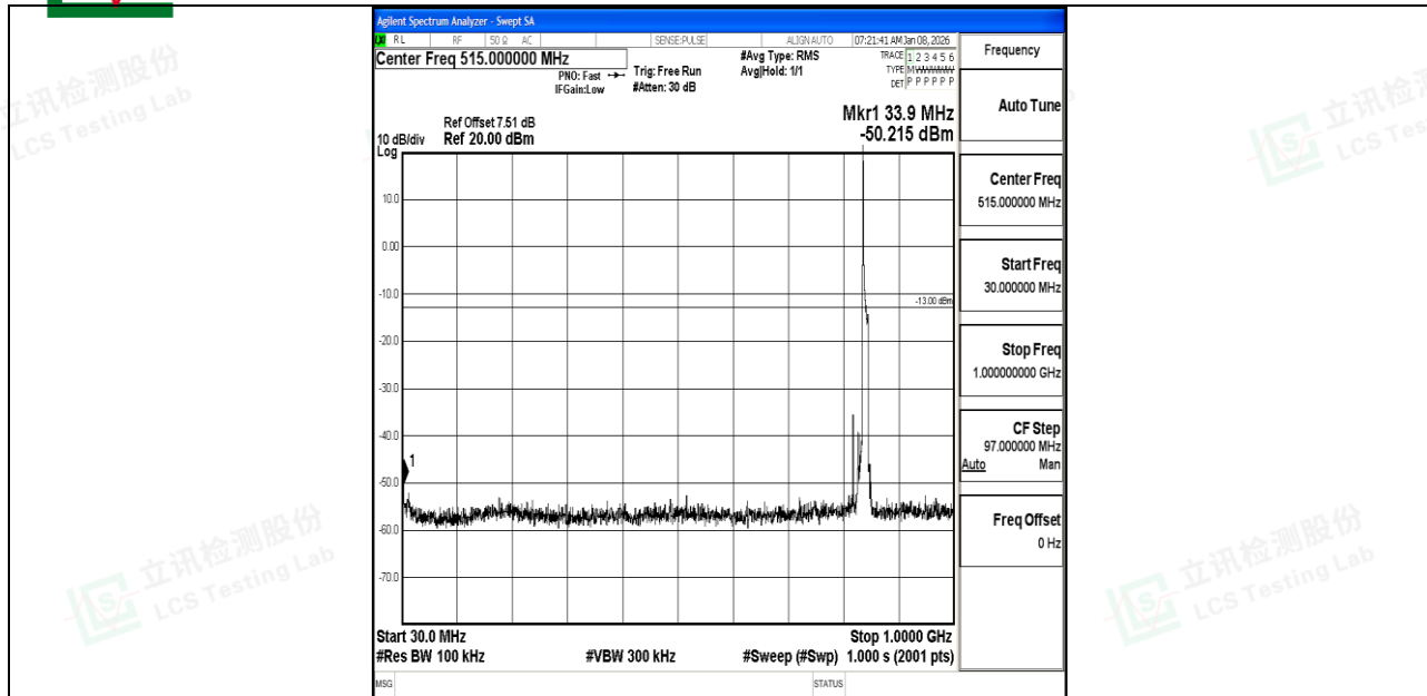
Band5_10MHz_QPSK_20600_1RB#0_30~1000_30~1000
