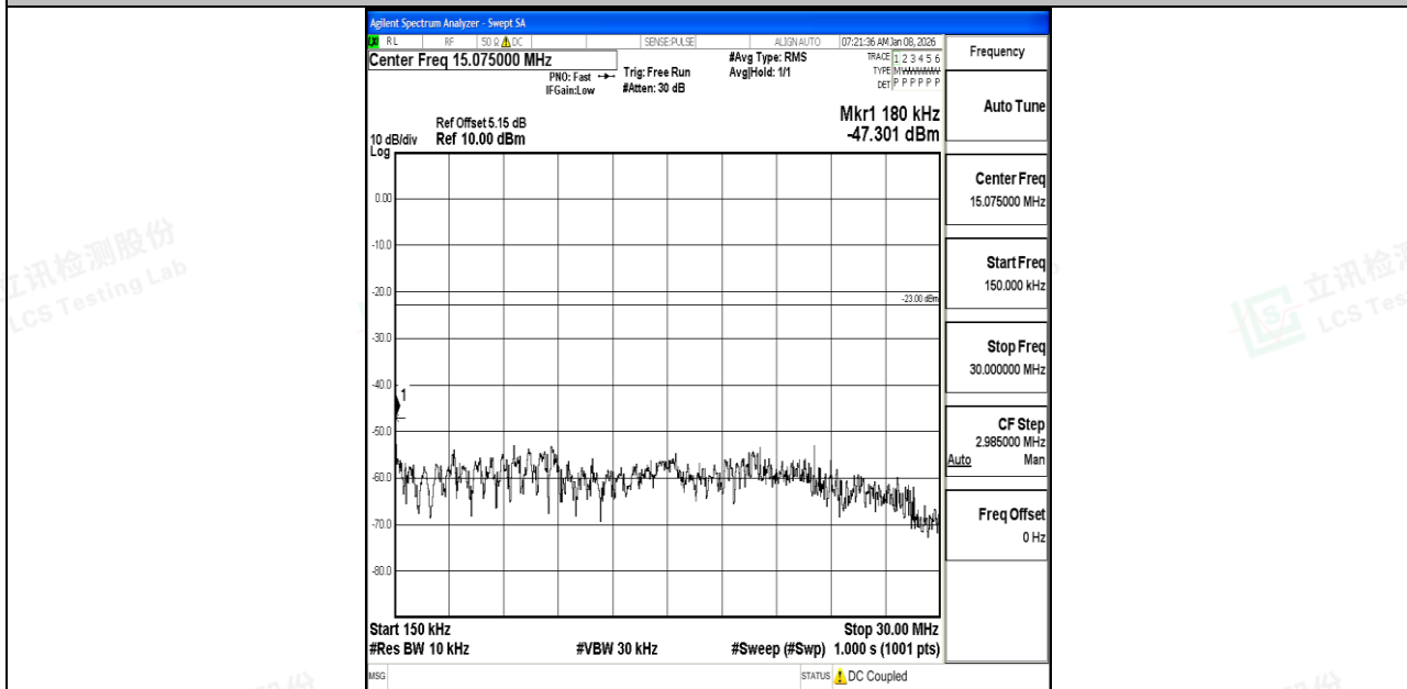
Band5_10MHz_QPSK_20600_1RB#0_0.15~30_0.15~30
