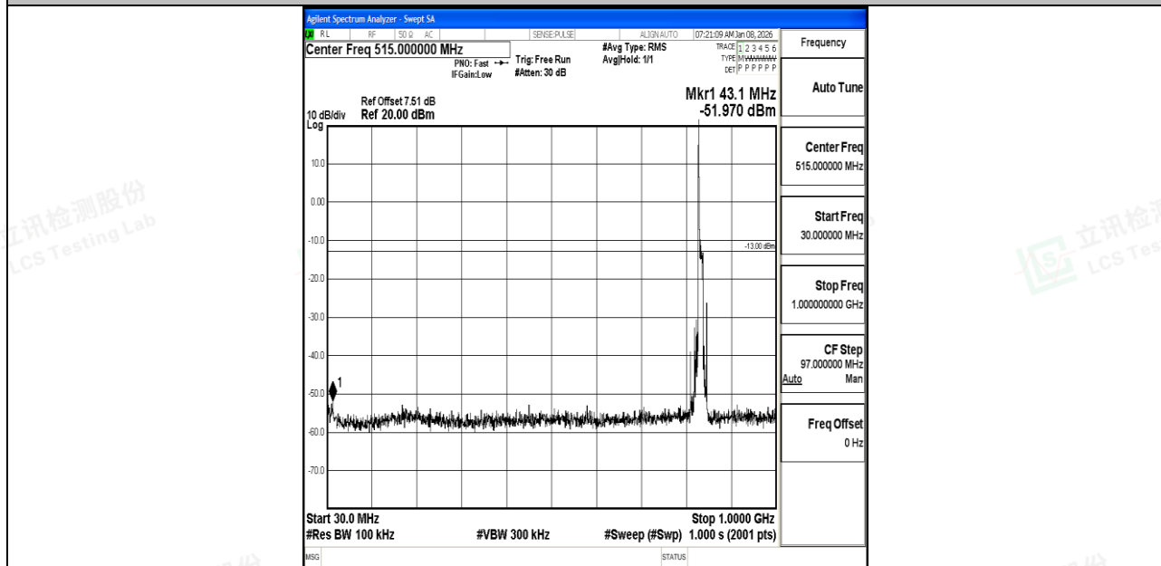
Band5_10MHz_16QAM_20525_1RB#0_30~1000_30~1000
