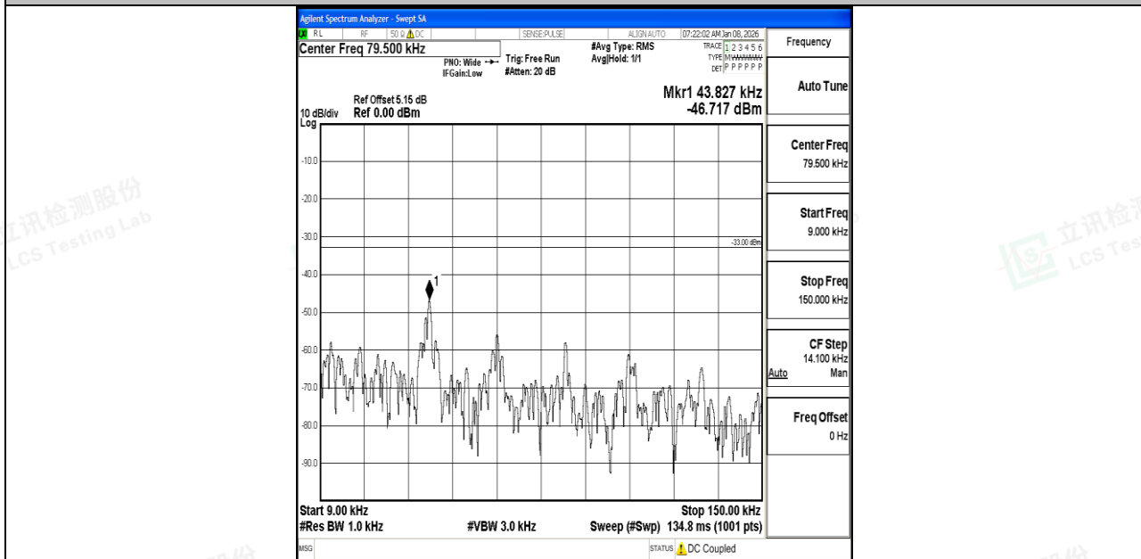
Band5_10MHz_16QAM_20600_1RB#0_0.009~0.15_0.009~0.15
