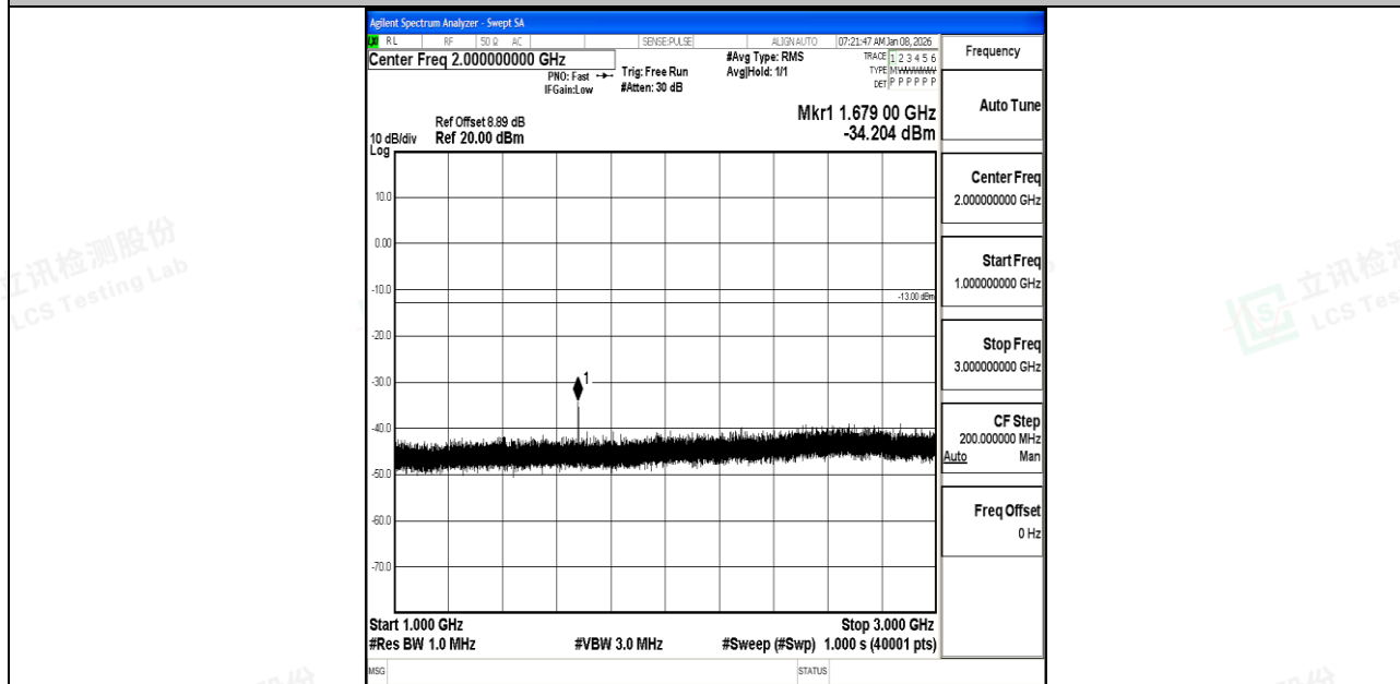
Band5_10MHz_QPSK_20600_1RB#0_1000~3000_1000~3000
