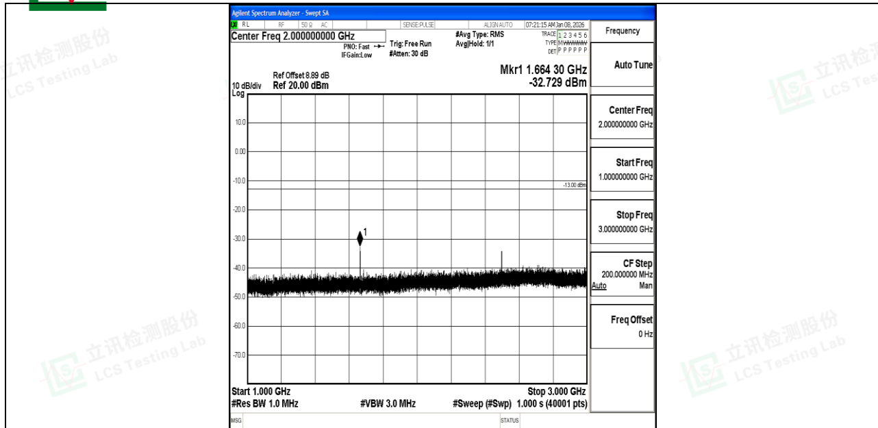
Band5_10MHz_16QAM_20525_1RB#0_1000~3000_1000~3000
