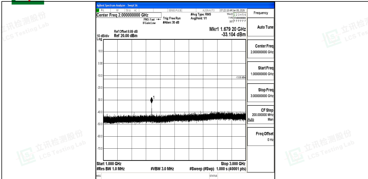
Band5_10MHz_16QAM_20600_1RB#0_1000~3000_1000~3000
