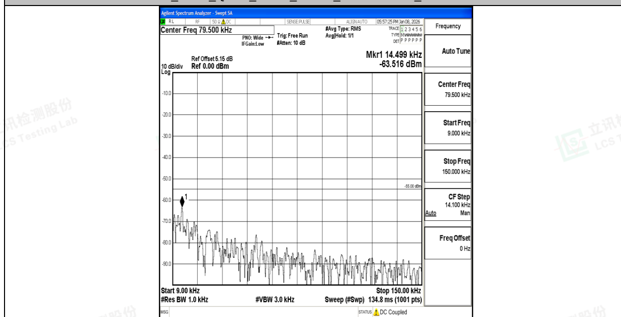
Band7_5MHz_16QAM_21425_1RB#0_0.009~0.15_0.009~0.15
