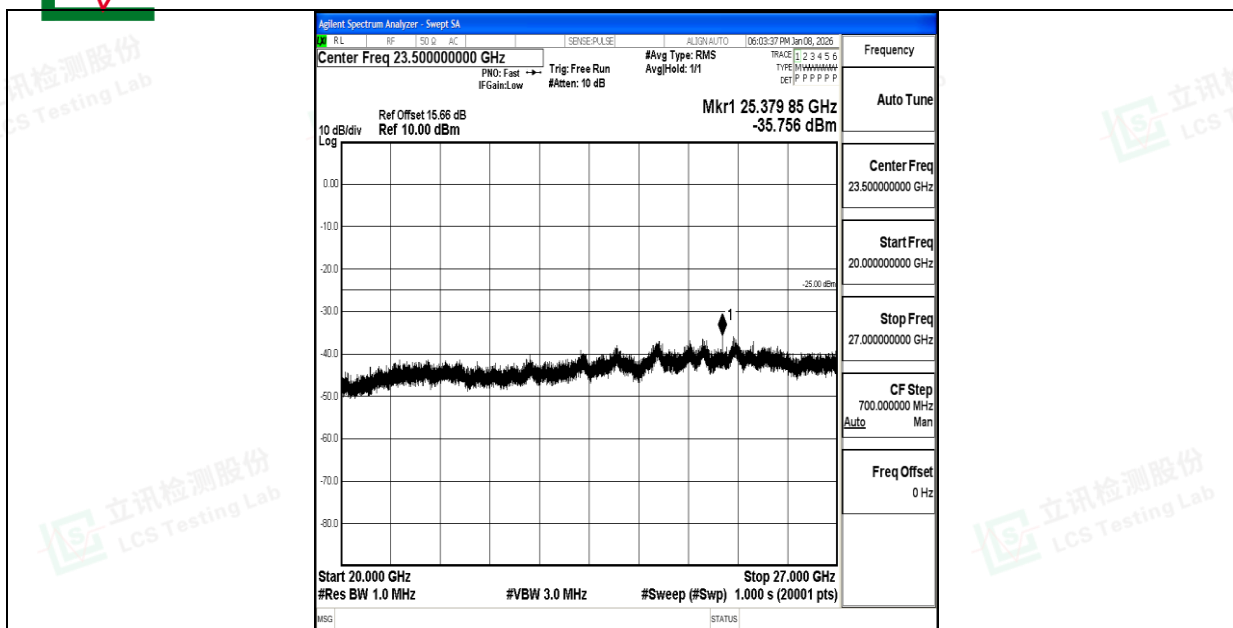
Band7_15MHz_QPSK_21100_1RB#0_20000~27000_20000~27000
