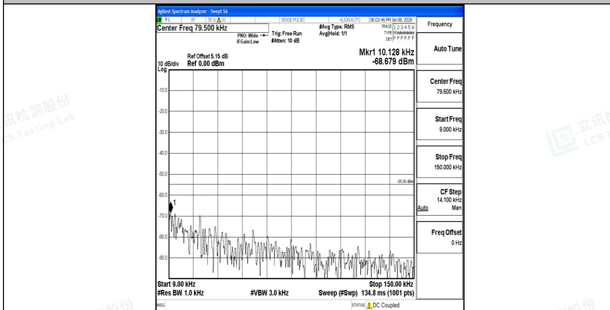
Band7_15MHz_16QAM_21100_1RB#0_0.009~0.15_0.009~0.15
