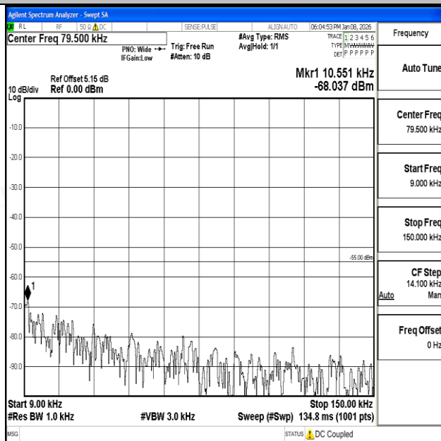
Band7_15MHz_16QAM_21375_1RB#0_0.009~0.15_0.009~0.15
