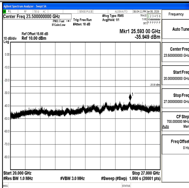
Band7_15MHz_16QAM_21100_1RB#0_20000~27000_20000~27000
