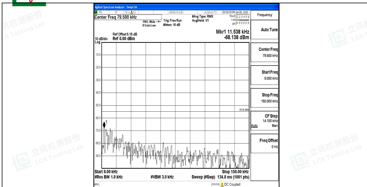
Band7_10MHz_QPSK_21100_1RB#0_0.009~0.15_0.009~0.15
