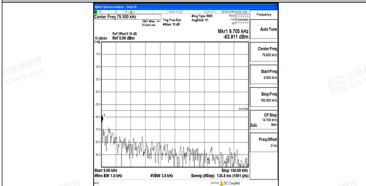
Band7_10MHz_16QAM_20800_1RB#0_0.009~0.15_0.009~0.15
