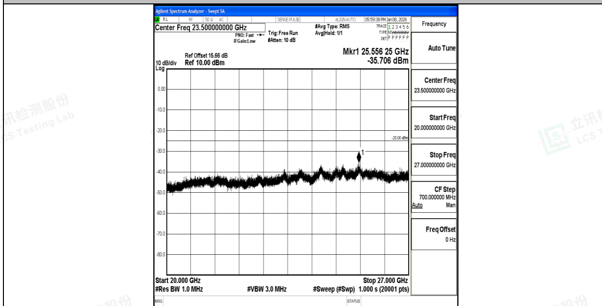
Band7_10MHz_16QAM_20800_1RB#0_20000~27000_20000~27000
