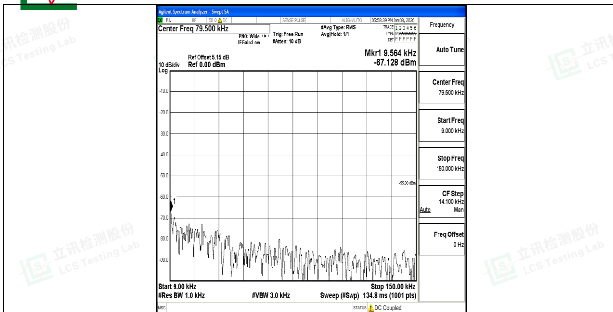
Band7_10MHz_QPSK_20800_1RB#0_0.009~0.15_0.009~0.15
