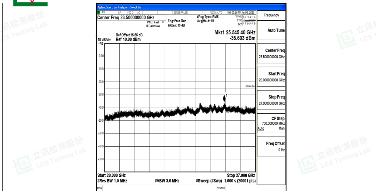
Band7_10MHz_QPSK_21100_1RB#0_20000~27000_20000~27000
