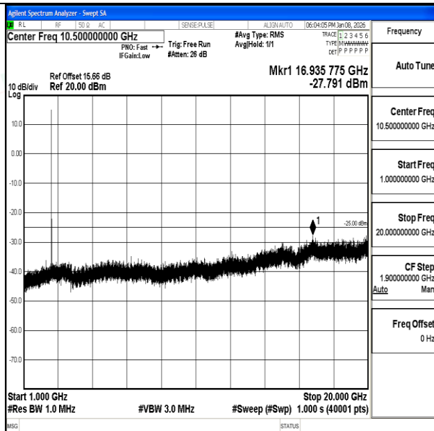
Band7_15MHz_16QAM_21100_1RB#0_1000~20000_1000~20000
