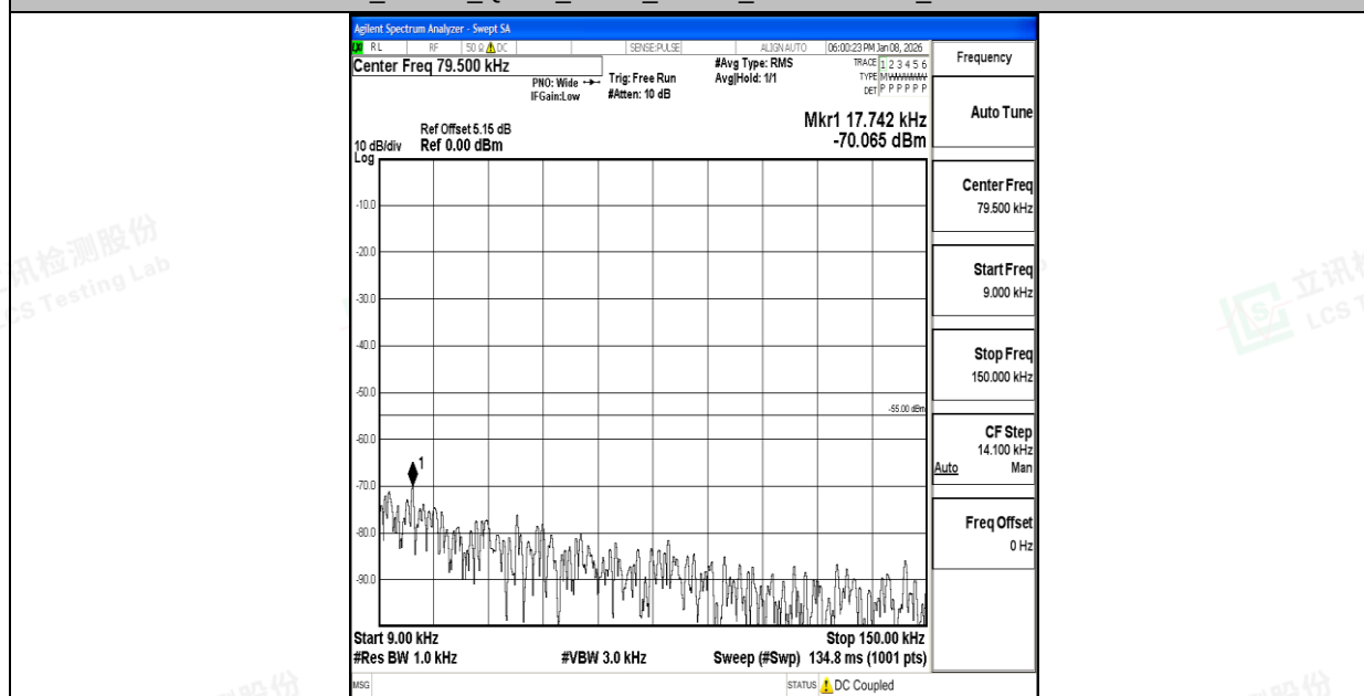
Band7_10MHz_16QAM_21100_1RB#0_0.009~0.15_0.009~0.15
