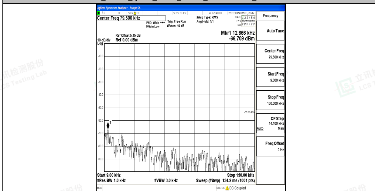
Band7_10MHz_16QAM_21400_1RB#0_0.009~0.15_0.009~0.15
