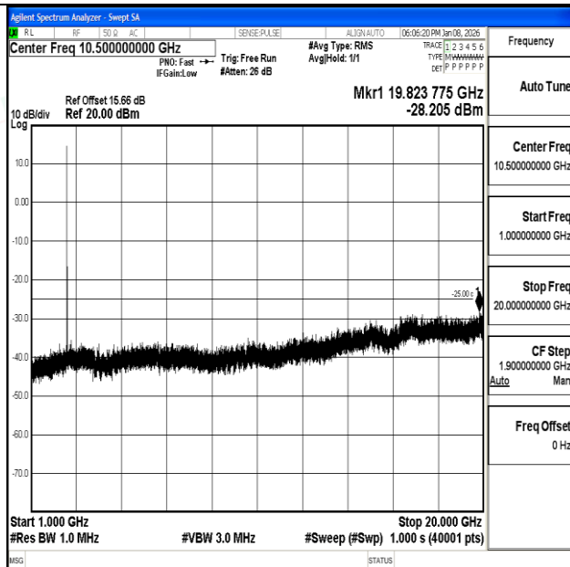
Band7_20MHz_16QAM_20850_1RB#0_1000~20000_1000~20000
