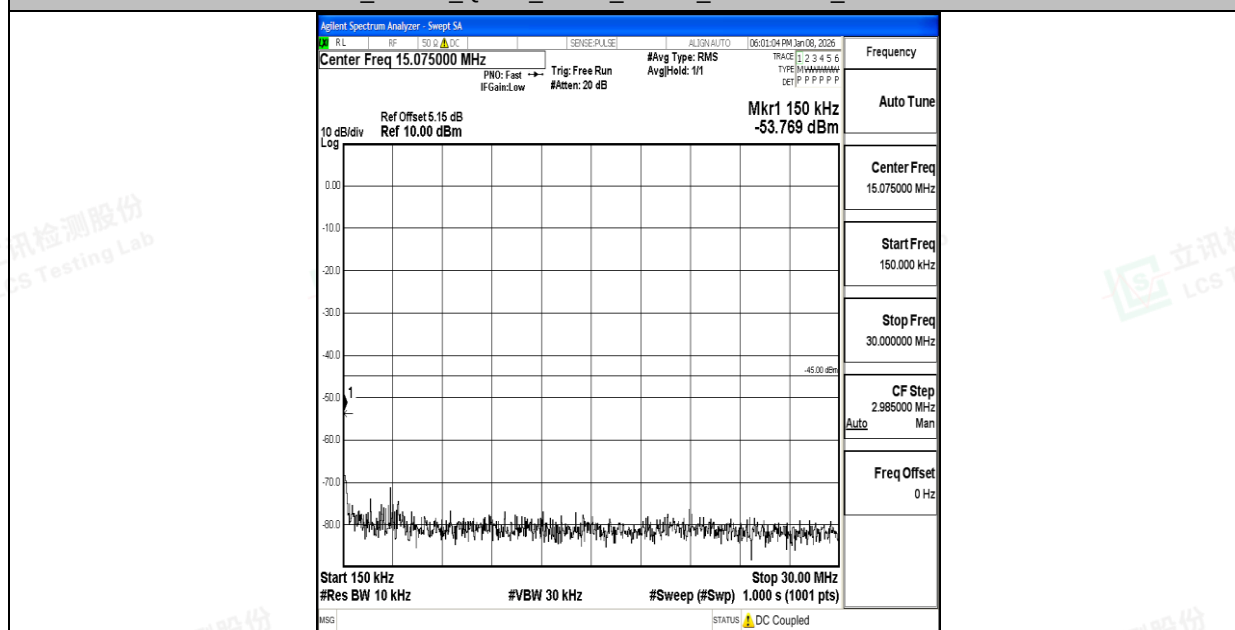
Band7_10MHz_QPSK_21400_1RB#0_0.15~30_0.15~30
