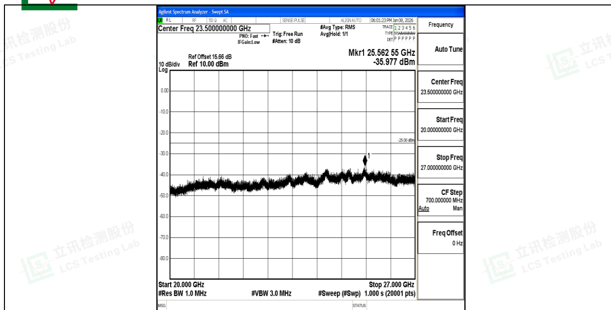
Band7_10MHz_QPSK_21400_1RB#0_20000~27000_20000~27000
