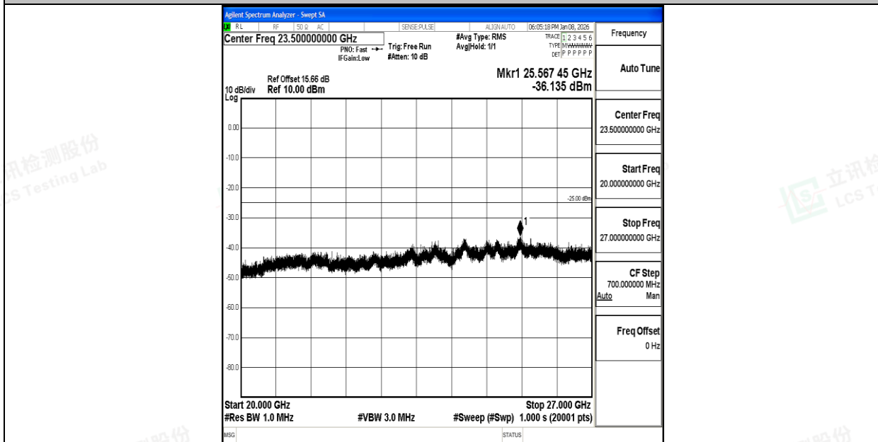
Band7_15MHz_16QAM_21375_1RB#0_20000~27000_20000~27000
