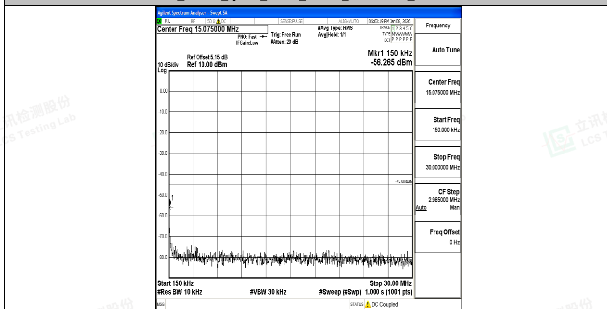
Band7_15MHz_QPSK_21100_1RB#0_0.15~30_0.15~30
