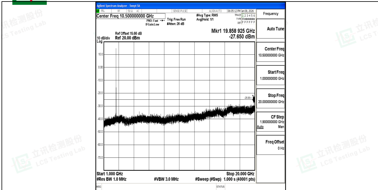
Band7_15MHz_16QAM_21375_1RB#0_1000~20000_1000~20000
