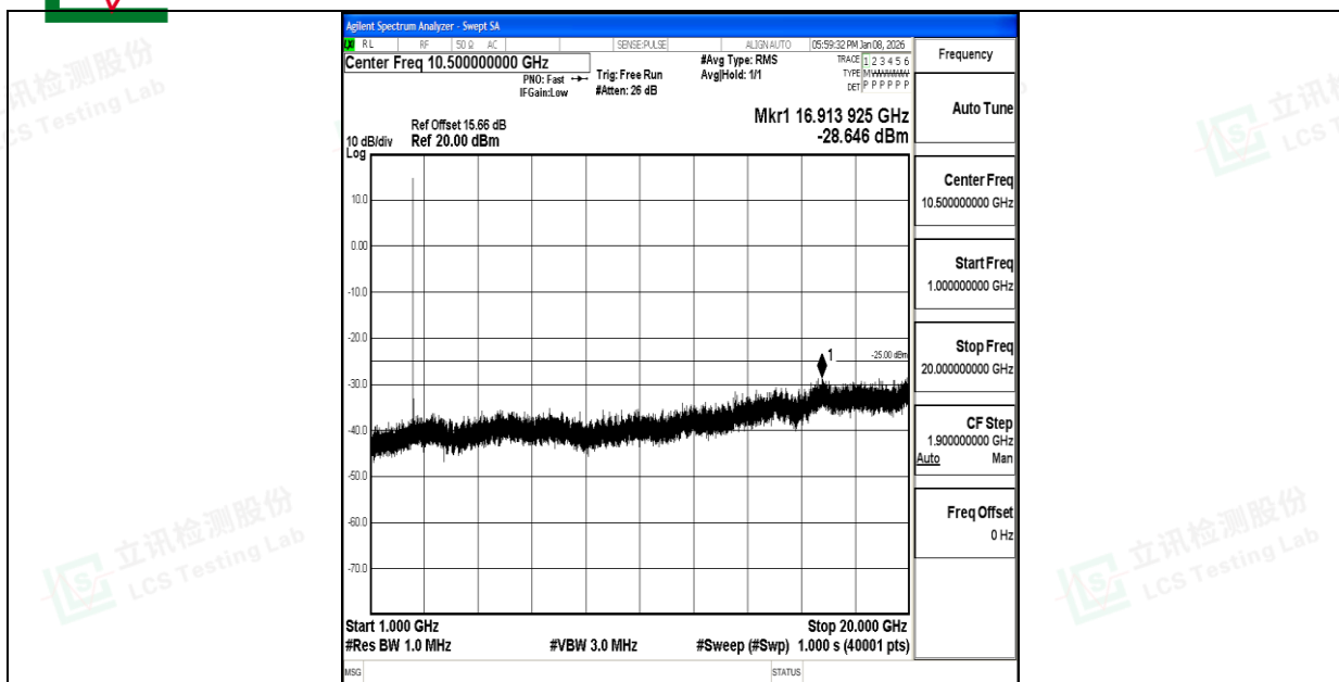
Band7_10MHz_16QAM_20800_1RB#0_1000~20000_1000~20000
