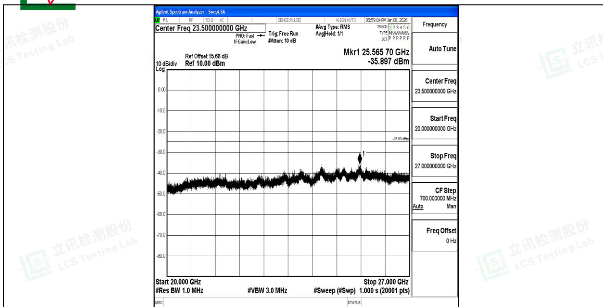
Band7_10MHz_QPSK_20800_1RB#0_20000~27000_20000~27000
