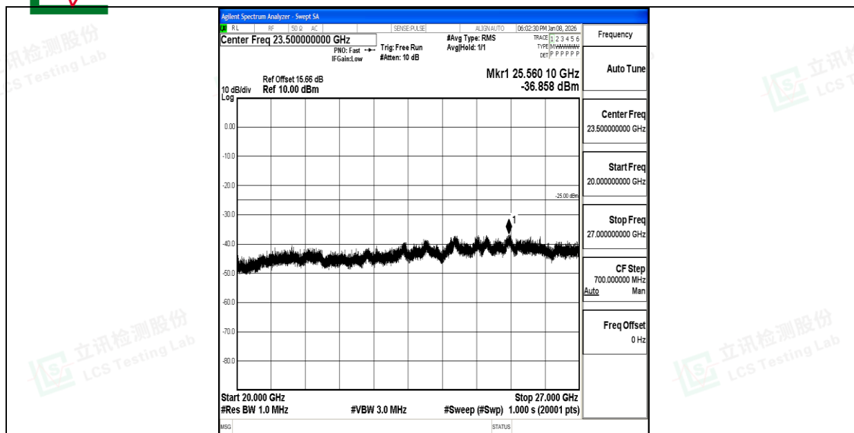
Band7_15MHz_QPSK_20825_1RB#0_20000~27000_20000~27000
