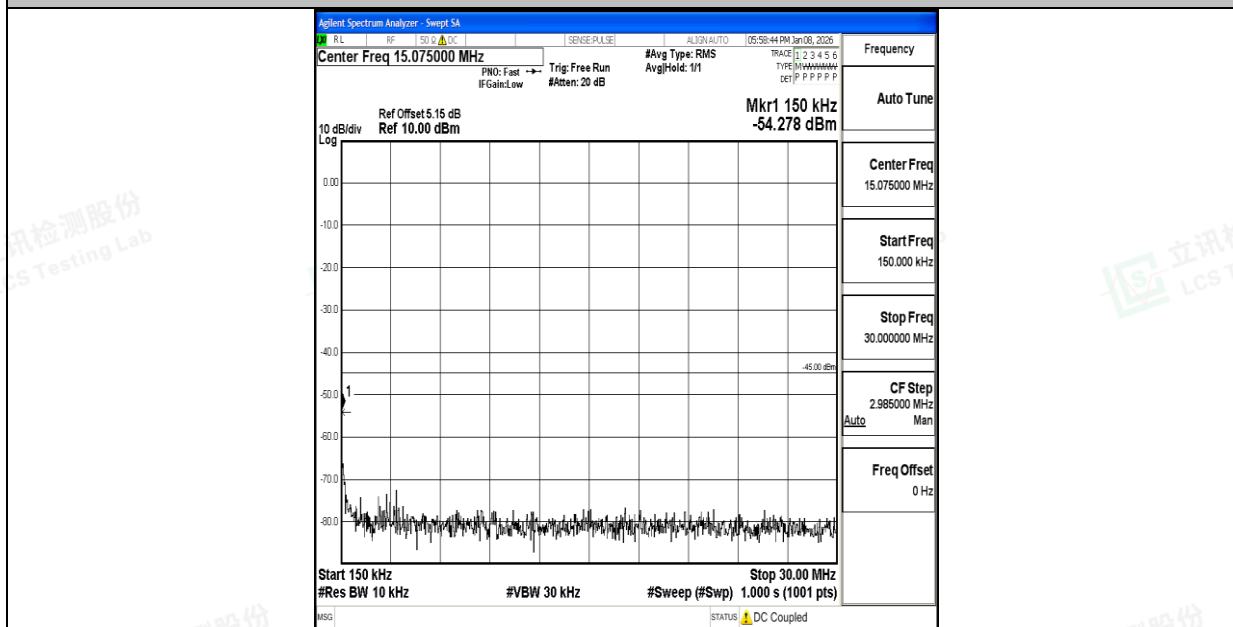
Band7_10MHz_QPSK_20800_1RB#0_0.15~30_0.15~30
