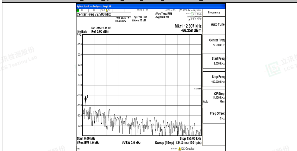
Band7_15MHz_16QAM_20825_1RB#0_0.009~0.15_0.009~0.15
