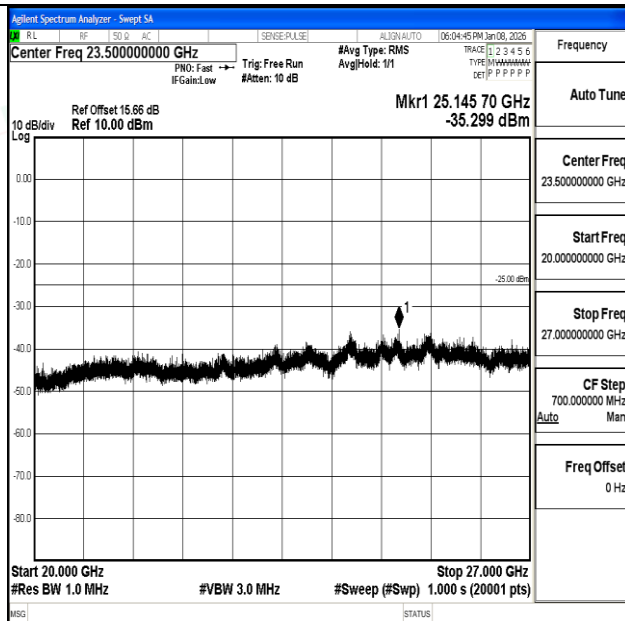
Band7_15MHz_QPSK_21375_1RB#0_20000~27000_20000~27000
