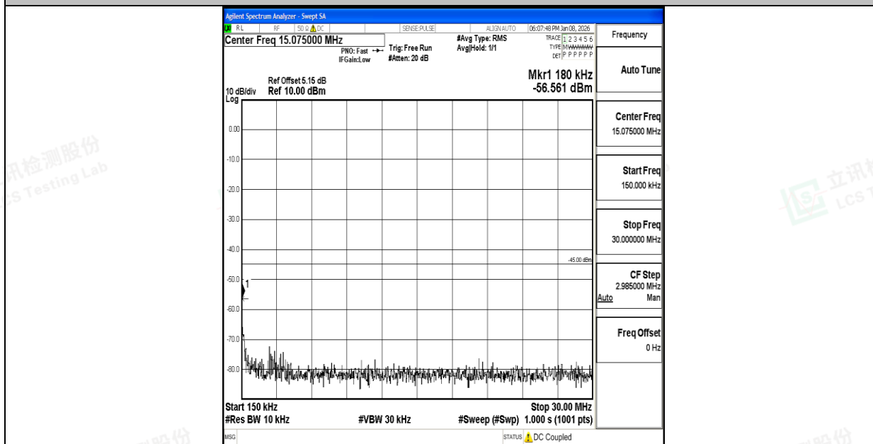
Band7_20MHz_QPSK_21350_1RB#0_0.15~30_0.15~30
