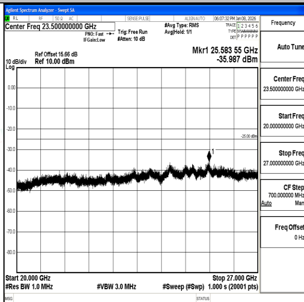
Band7_20MHz_16QAM_21100_1RB#0_20000~27000_20000~27000
