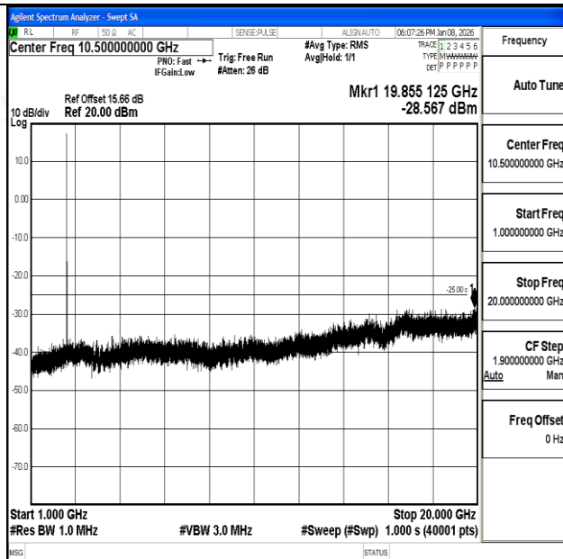
Band7_20MHz_16QAM_21100_1RB#0_1000~20000_1000~20000
