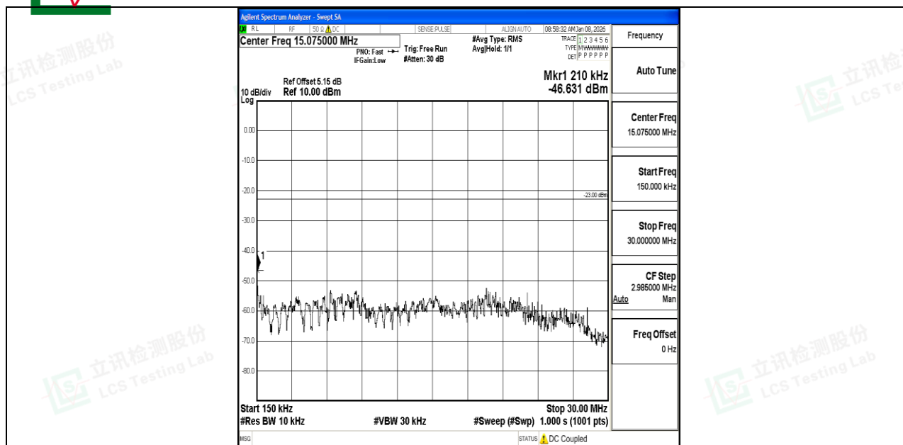
Band12_1.4MHz_16QAM_23095_1RB#0_0.15~30_0.15~30
