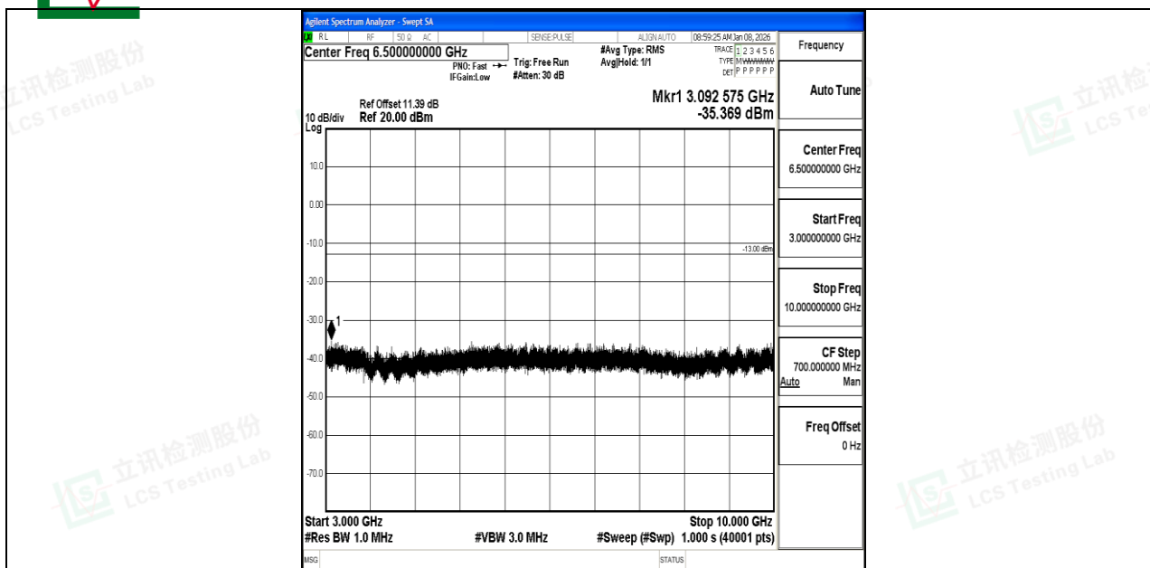
Band12_1.4MHz_QPSK_23173_1RB#0_3000~10000_3000~10000
