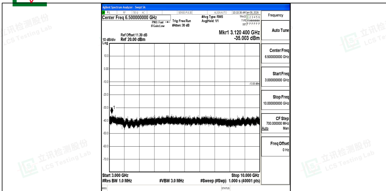
Band12_10MHz_QPSK_23095_1RB#0_3000~10000_3000~10000
