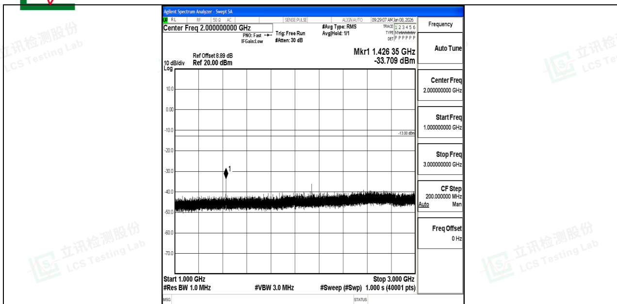
Band12_3MHz_16QAM_23165_1RB#0_1000~3000_1000~3000
