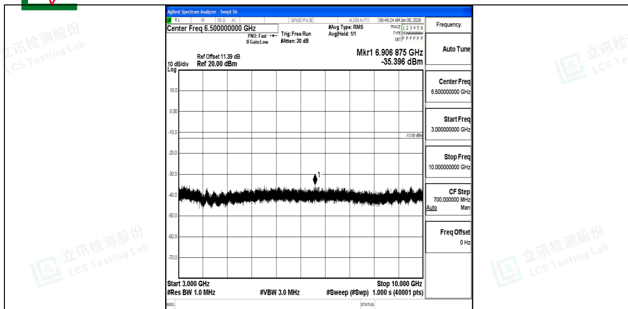
Band12_5MHz_QPSK_23095_1RB#0_3000~10000_3000~10000
