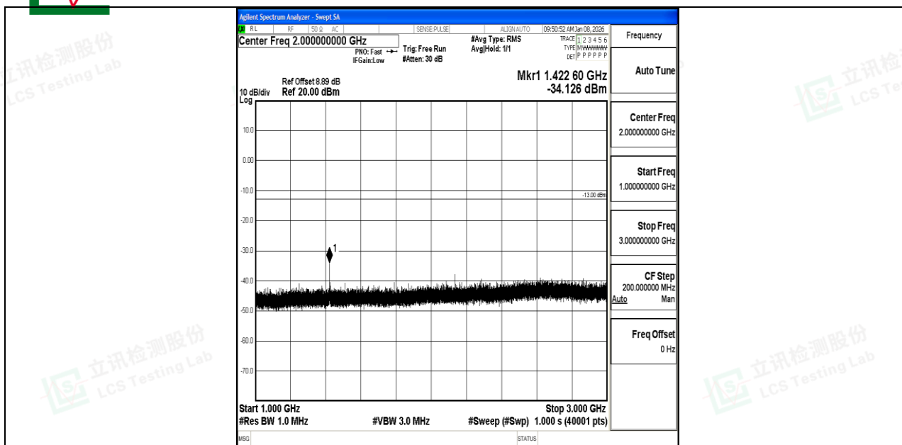
Band12_5MHz_16QAM_23155_1RB#0_1000~3000_1000~3000
