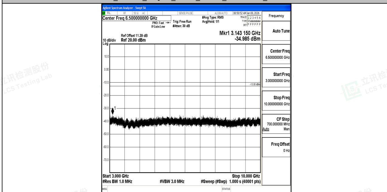
Band12_1.4MHz_16QAM_23095_1RB#0_3000~10000_3000~10000
