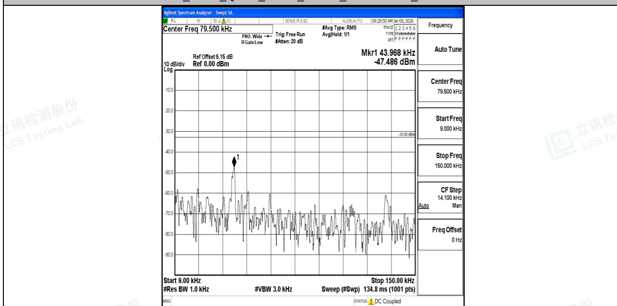
Band12_3MHz_16QAM_23165_1RB#0_0.009~0.15_0.009~0.15
