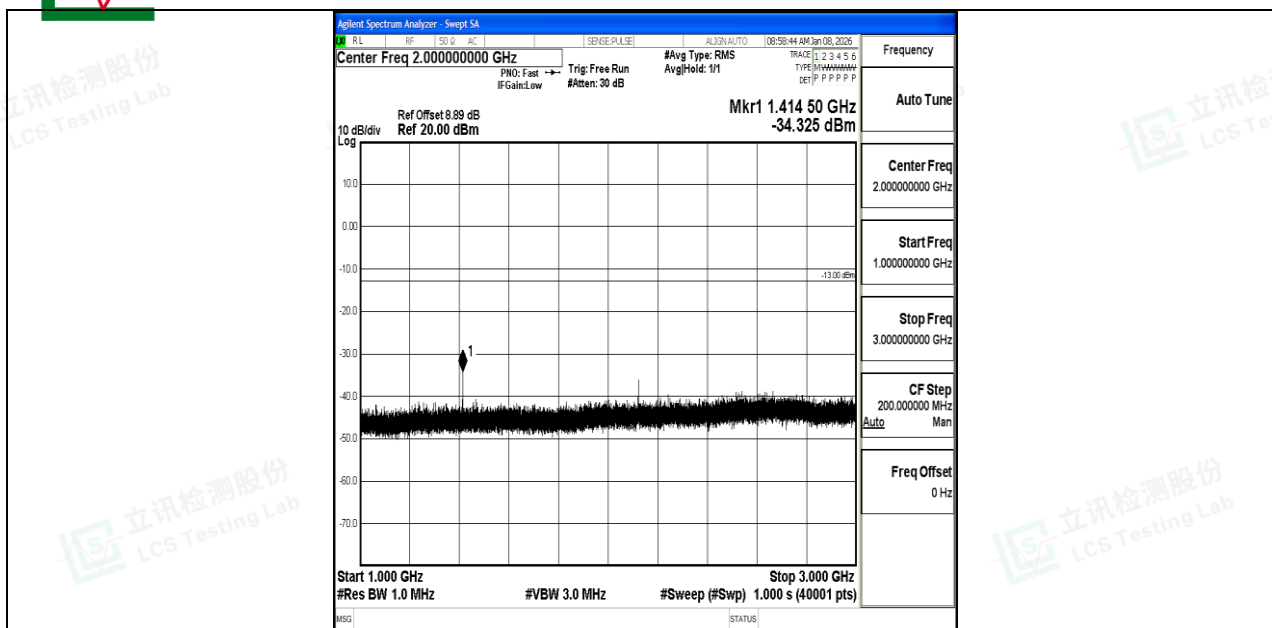
Band12_1.4MHz_16QAM_23095_1RB#0_1000~3000_1000~3000
