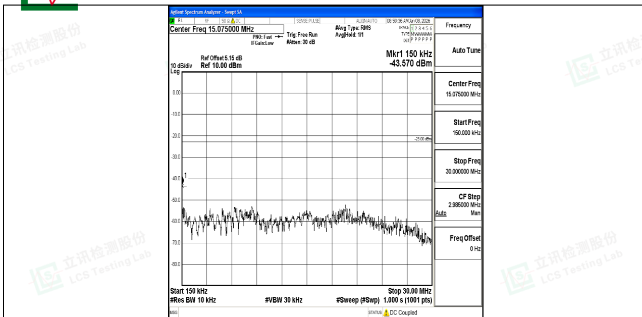
Band12_1.4MHz_16QAM_23173_1RB#0_0.15~30_0.15~30
