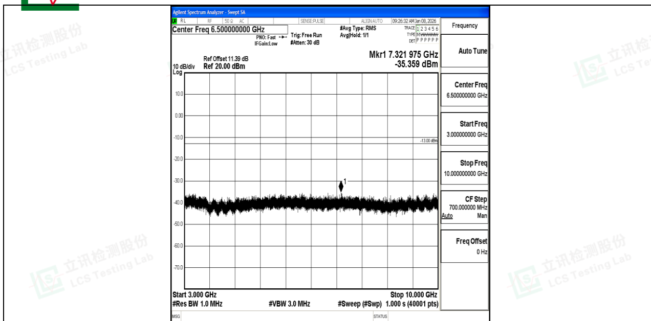
Band12_3MHz_QPSK_23025_1RB#0_3000~10000_3000~10000
