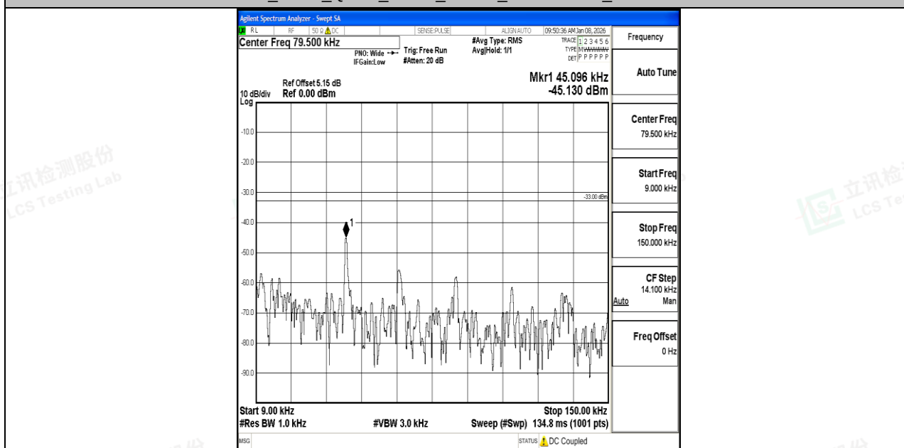
Band12_5MHz_16QAM_23155_1RB#0_0.009~0.15_0.009~0.15
