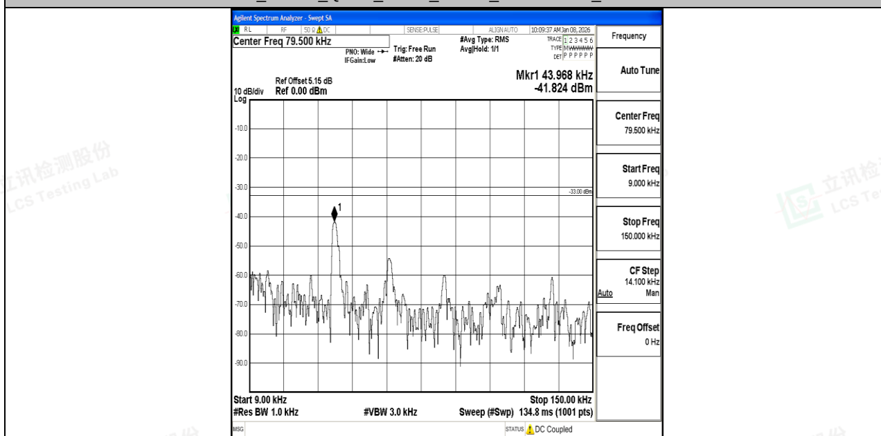
Band12_10MHz_16QAM_23060_1RB#0_0.009~0.15_0.009~0.15
