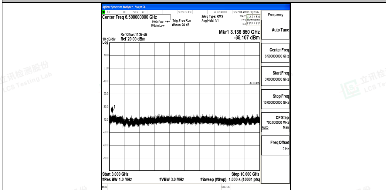
Band12_3MHz_16QAM_23025_1RB#0_3000~10000_3000~10000
