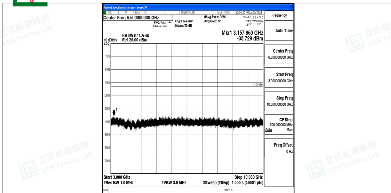
Band12_10MHz_QPSK_23060_1RB#0_3000~10000_3000~10000
