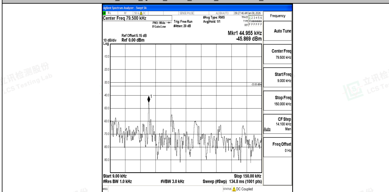
Band12_3MHz_16QAM_23095_1RB#0_0.009~0.15_0.009~0.15
