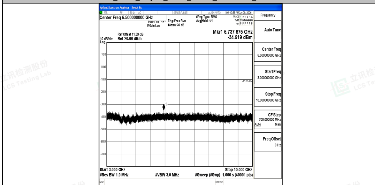
Band12_5MHz_16QAM_23095_1RB#0_3000~10000_3000~10000
