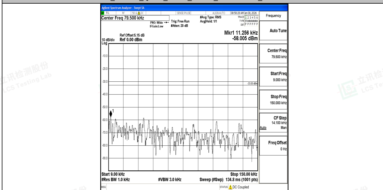
Band12_1.4MHz_16QAM_23095_1RB#0_0.009~0.15_0.009~0.15
