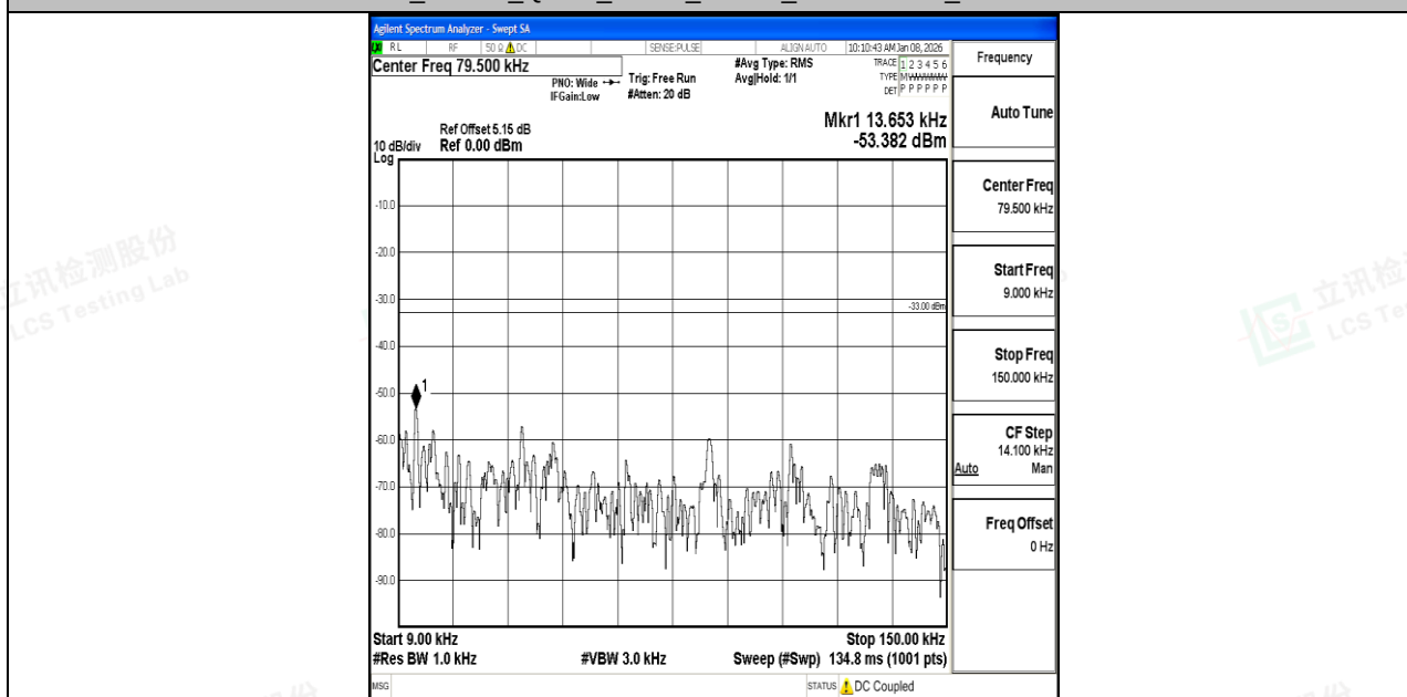
Band12_10MHz_16QAM_23095_1RB#0_0.009~0.15_0.009~0.15
