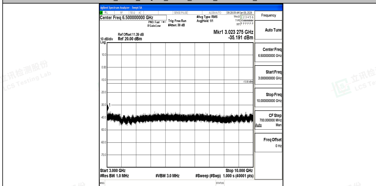
Band12_3MHz_16QAM_23095_1RB#0_3000~10000_3000~10000
