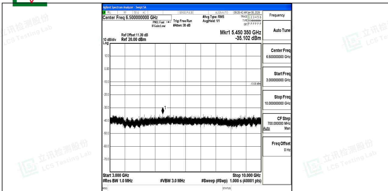
Band12_3MHz_QPSK_23165_1RB#0_3000~10000_3000~10000
