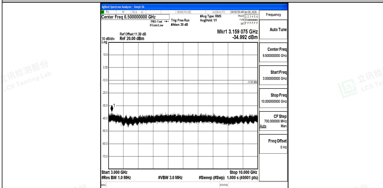
Band12_5MHz_16QAM_23155_1RB#0_3000~10000_3000~10000
