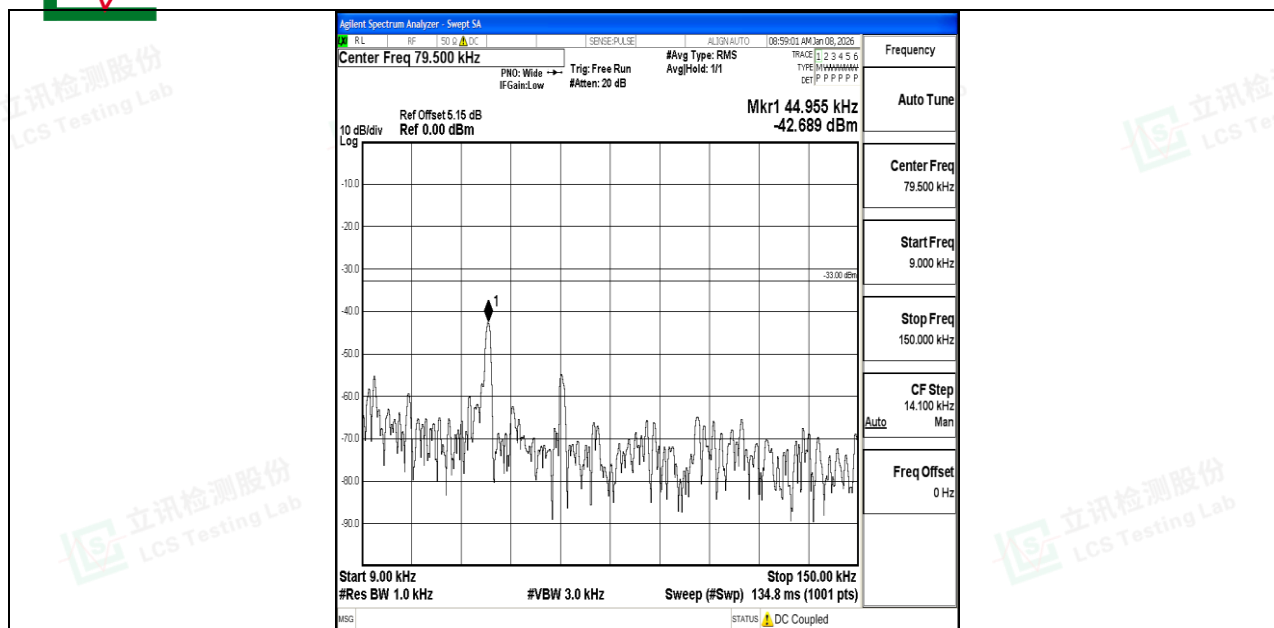
Band12_1.4MHz_QPSK_23173_1RB#0_0.009~0.15_0.009~0.15
