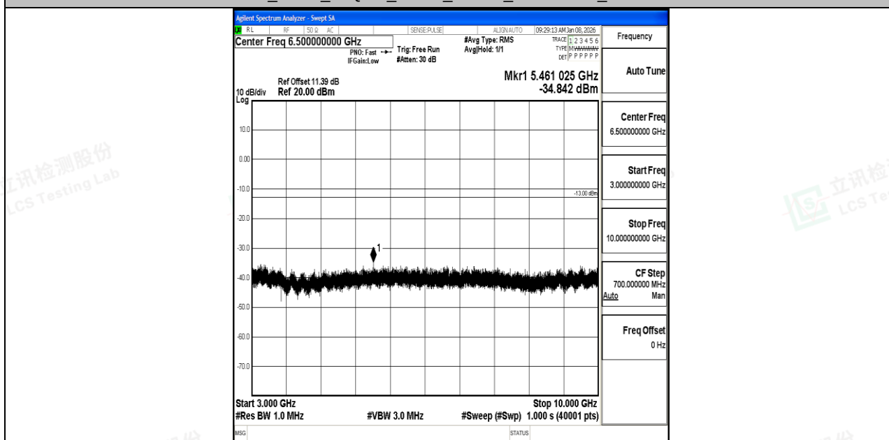
Band12_3MHz_16QAM_23165_1RB#0_3000~10000_3000~10000
