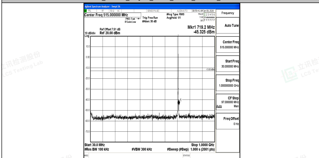
Band12_1.4MHz_16QAM_23173_1RB#0_30~1000_30~1000
