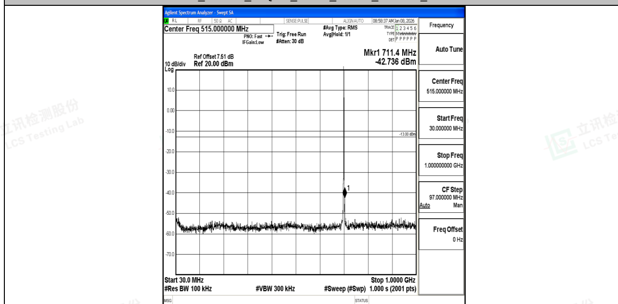
Band12_1.4MHz_16QAM_23095_1RB#0_30~1000_30~1000
