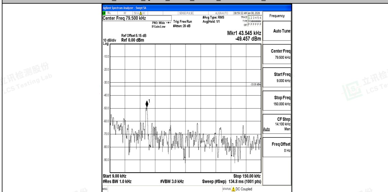
Band12_1.4MHz_16QAM_23173_1RB#0_0.009~0.15_0.009~0.15
