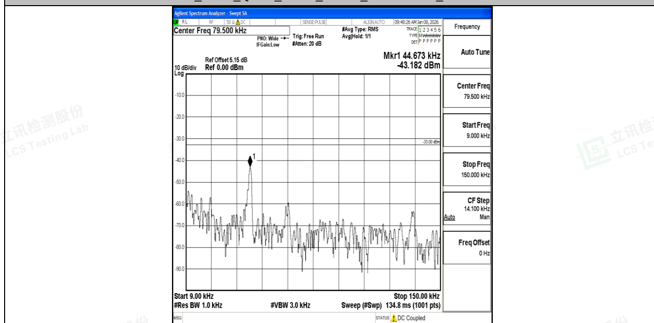
Band12_5MHz_16QAM_23035_1RB#0_0.009~0.15_0.009~0.15
