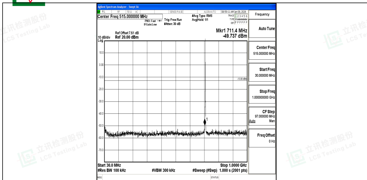
Band12_1.4MHz_QPSK_23173_1RB#0_30~1000_30~1000
