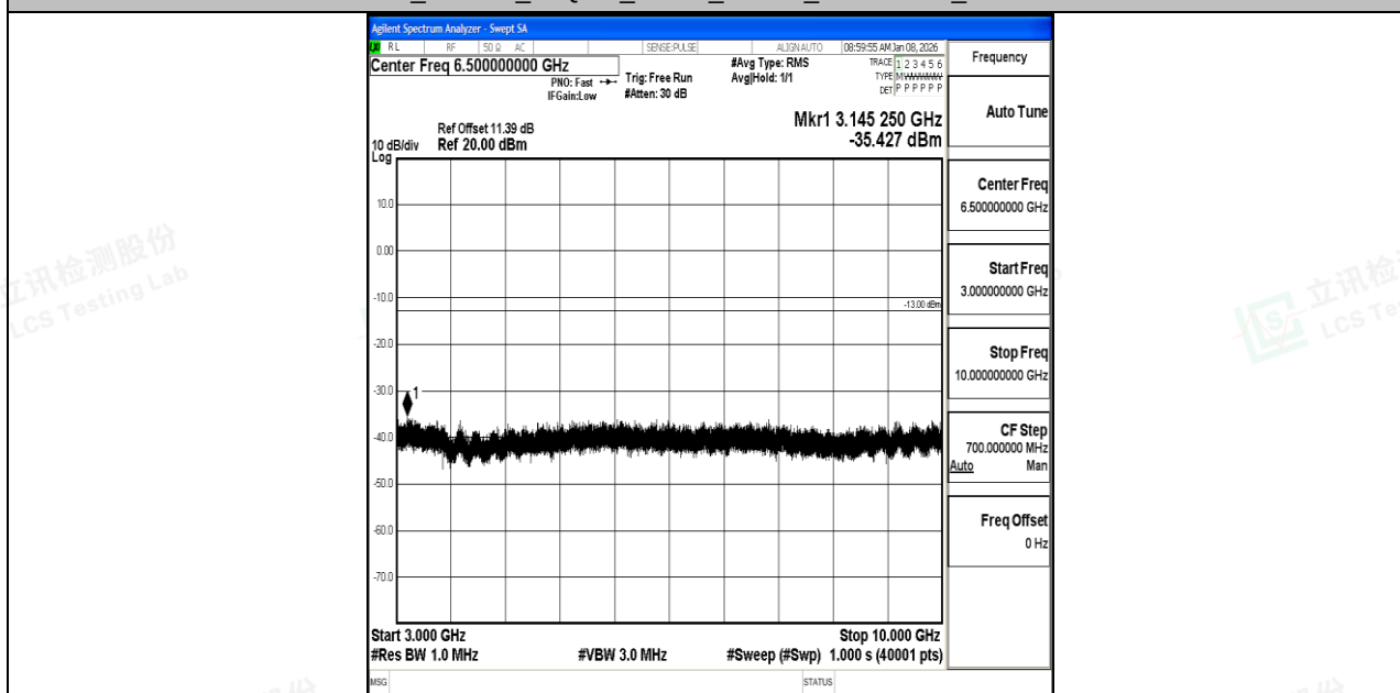
Band12_1.4MHz_16QAM_23173_1RB#0_3000~10000_3000~10000
