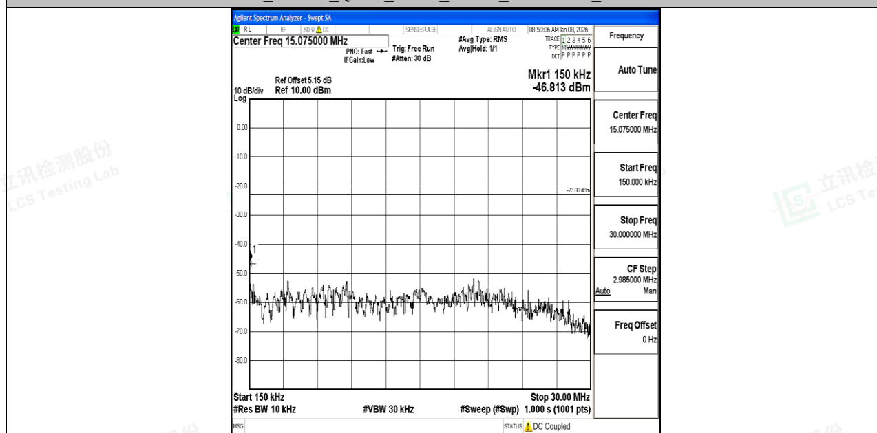
Band12_1.4MHz_QPSK_23173_1RB#0_0.15~30_0.15~30
