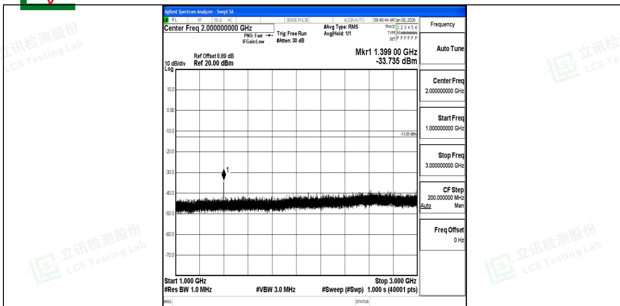
Band12_5MHz_16QAM_23035_1RB#0_1000~3000_1000~3000
