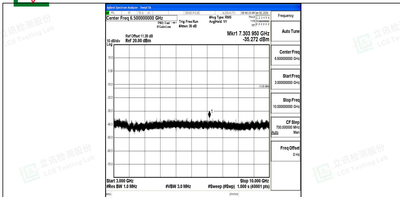
Band12_5MHz_QPSK_23035_1RB#0_3000~10000_3000~10000
