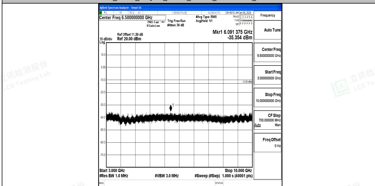
Band12_5MHz_16QAM_23035_1RB#0_3000~10000_3000~10000
