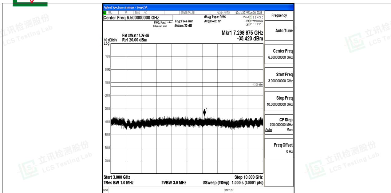
Band12_10MHz_QPSK_23130_1RB#0_3000~10000_3000~10000
