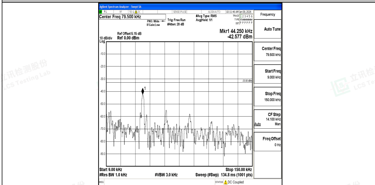
Band12_10MHz_16QAM_23130_1RB#0_0.009~0.15_0.009~0.15
