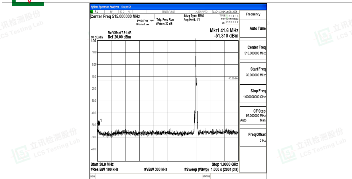
Band17_10MHz_16QAM_23800_1RB#0_30~1000_30~1000
