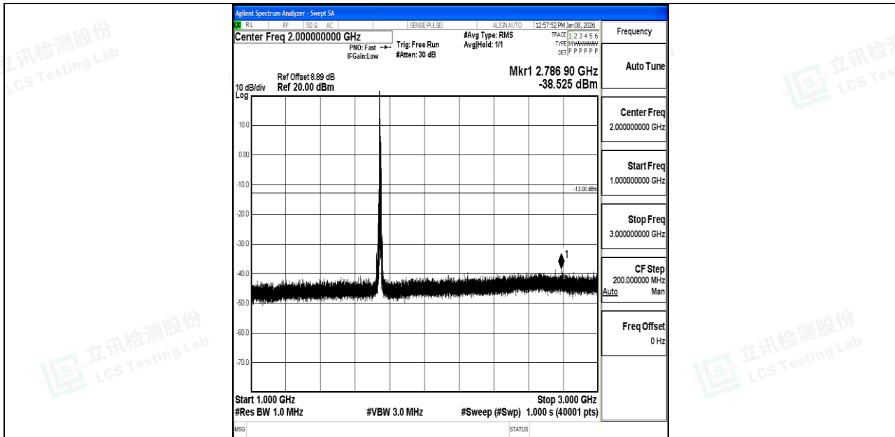
Band66_10MHz_16QAM_132322_1RB#0_1000~3000_1000~3000
