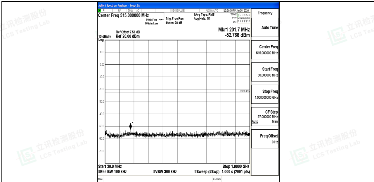
Band66_10MHz_QPSK_132022_1RB#0_30~1000_30~1000
