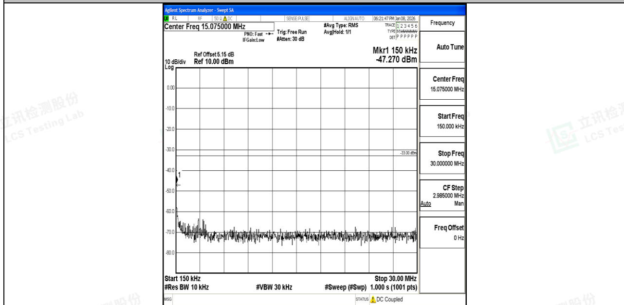
Band66_15MHz_16QAM_132322_1RB#0_0.15~30_0.15~30
