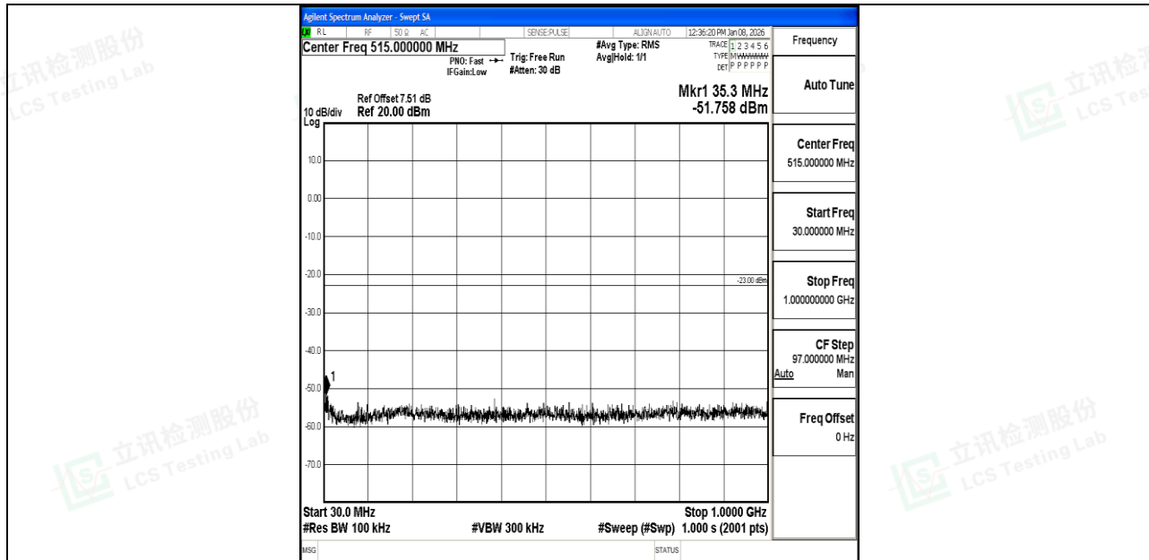
Band66_5MHz_QPSK_132647_1RB#0_30~1000_30~1000
