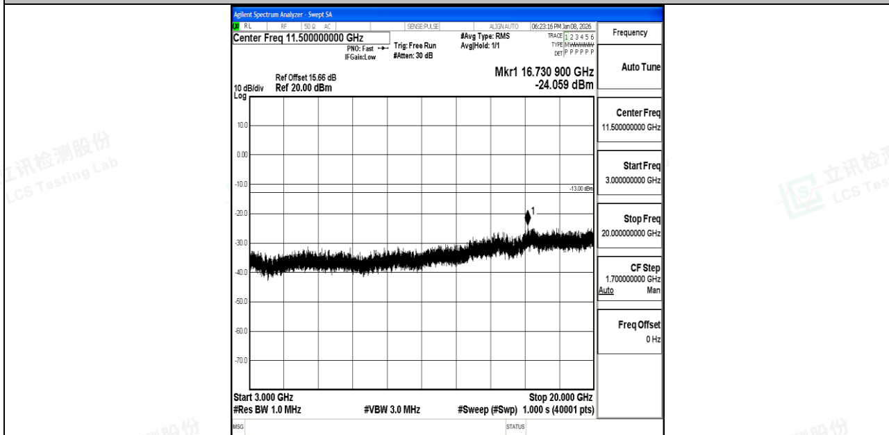
Band66_15MHz_16QAM_132597_1RB#0_3000~20000_3000~20000
