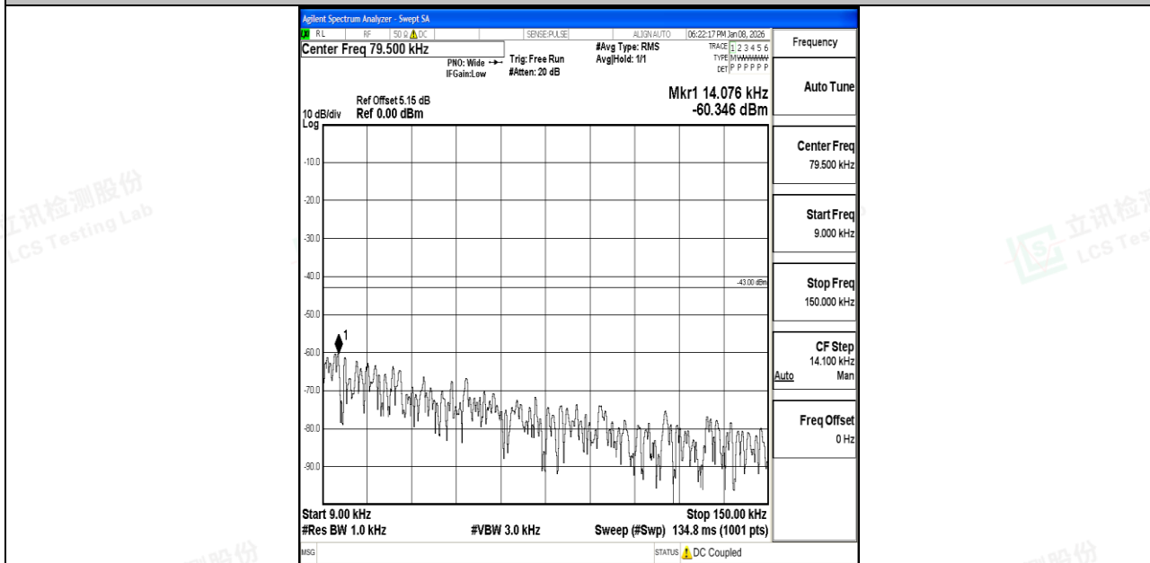
Band66_15MHz_QPSK_132597_1RB#0_0.009~0.15_0.009~0.15
