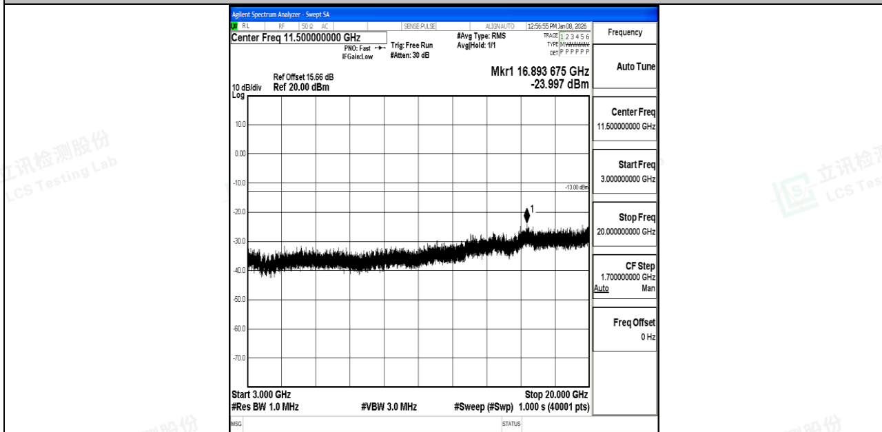
Band66_10MHz_16QAM_132022_1RB#0_3000~20000_3000~20000
