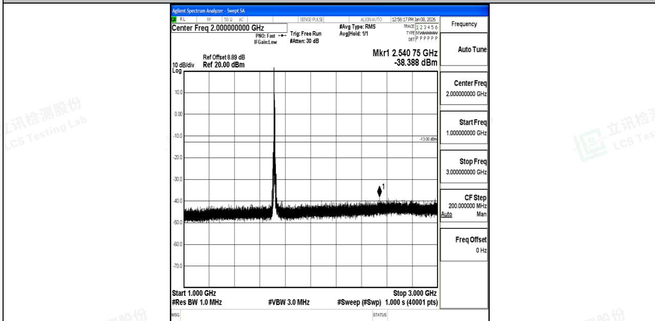
Band66_10MHz_QPSK_132022_1RB#0_1000~3000_1000~3000
