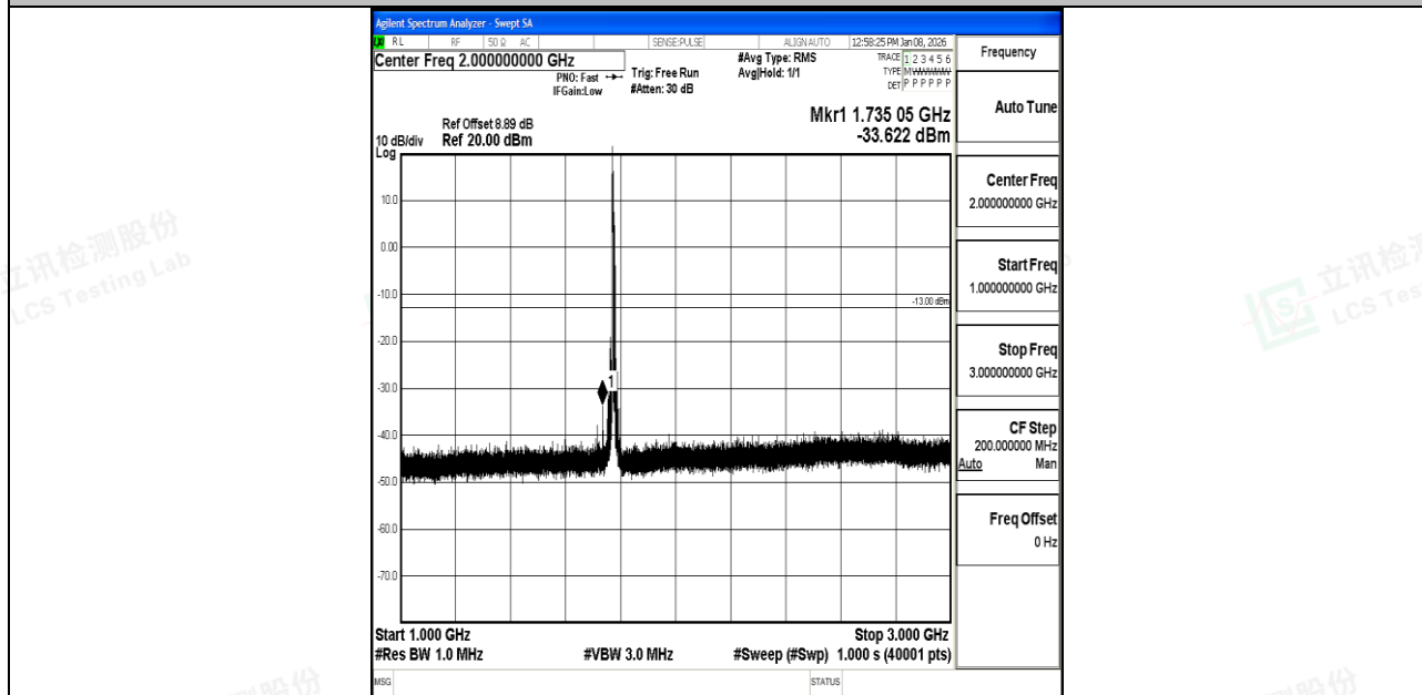
Band66_10MHz_QPSK_132622_1RB#0_1000~3000_1000~3000
