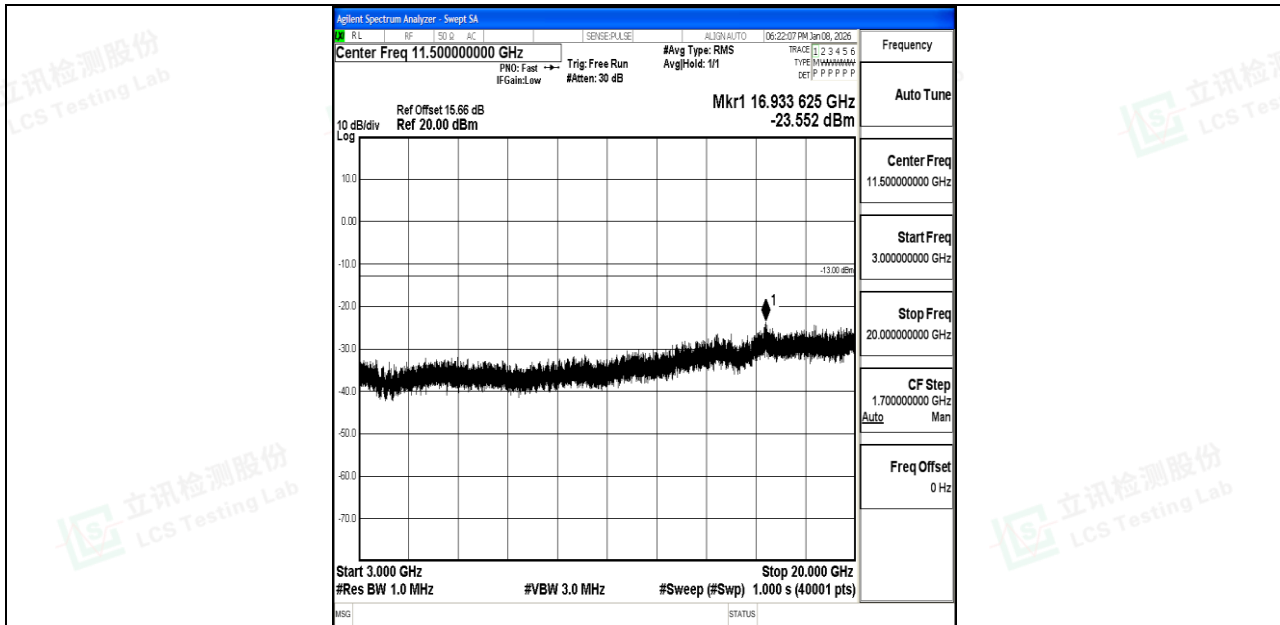
Band66_15MHz_16QAM_132322_1RB#0_3000~20000_3000~20000
