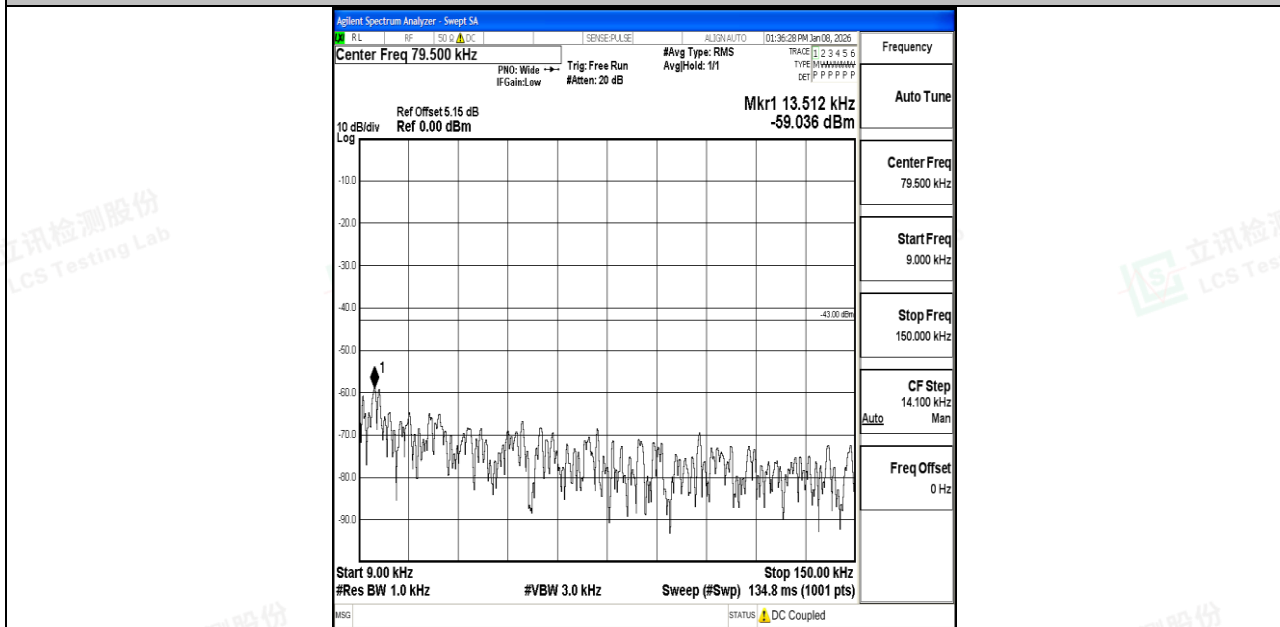
Band66_20MHz_QPSK_132322_1RB#0_0.009~0.15_0.009~0.15
