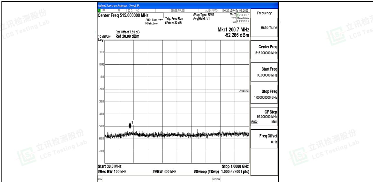
Band66_15MHz_QPSK_132047_1RB#0_30~1000_30~1000
