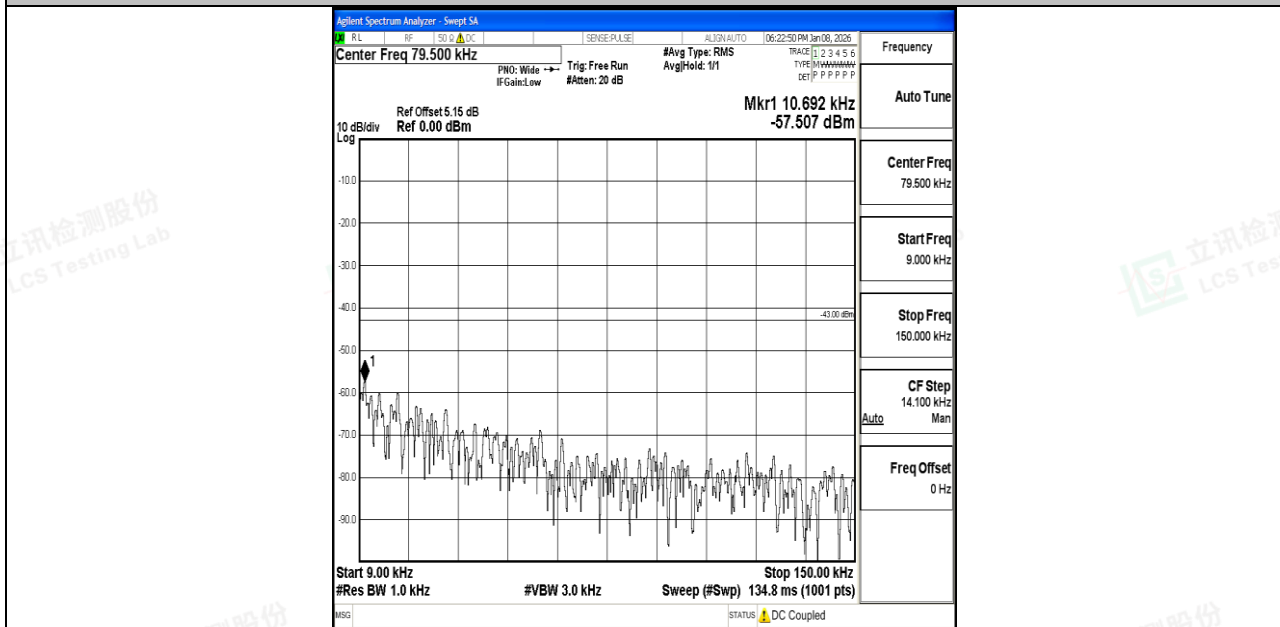
Band66_15MHz_16QAM_132597_1RB#0_0.009~0.15_0.009~0.15
