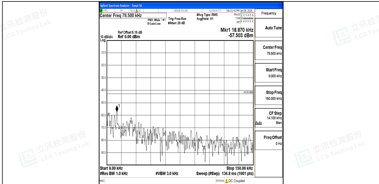
Band66_15MHz_16QAM_132322_1RB#0_0.009~0.15_0.009~0.15
