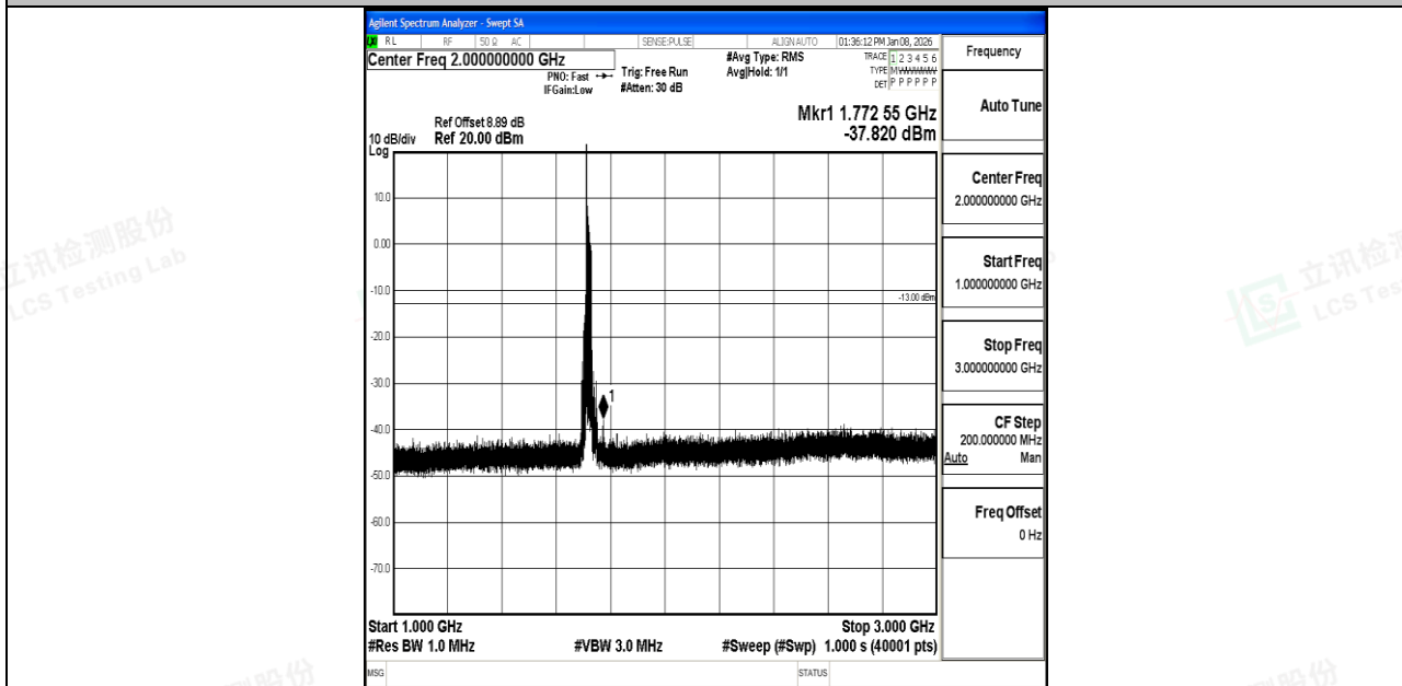
Band66_20MHz_16QAM_132072_1RB#0_1000~3000_1000~3000
