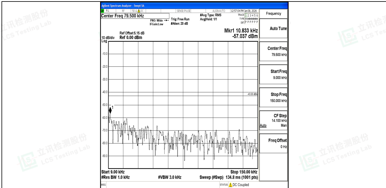
Band66_10MHz_QPSK_132322_1RB#0_0.009~0.15_0.009~0.15
