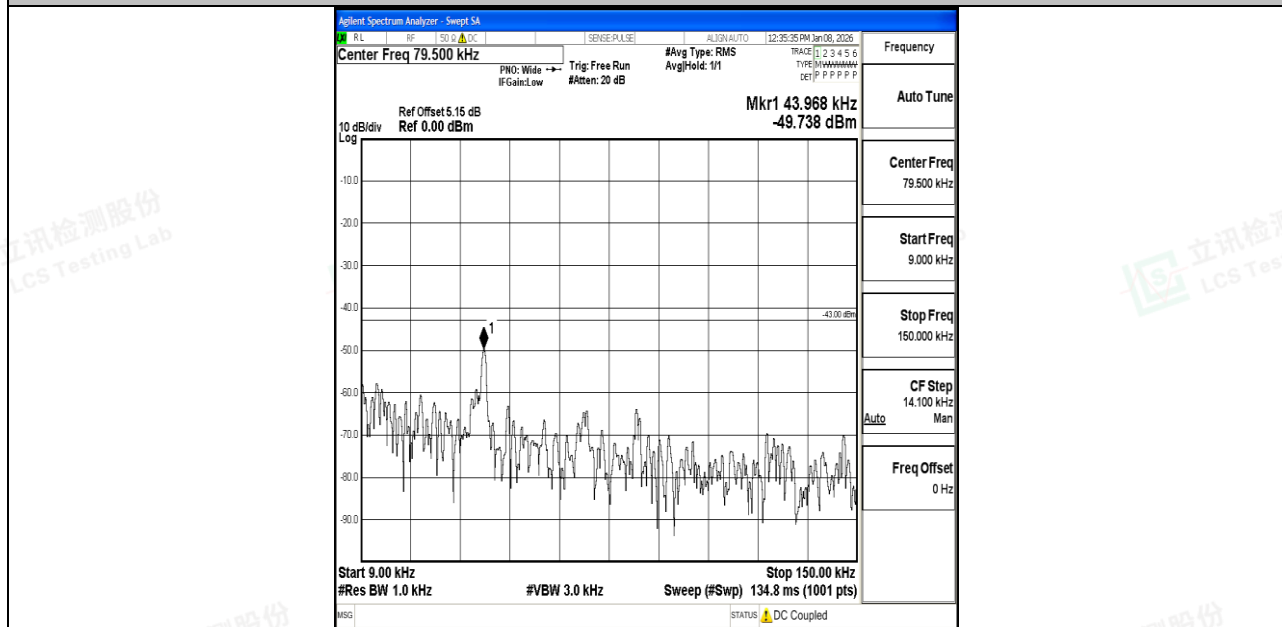
Band66_5MHz_16QAM_132322_1RB#0_0.009~0.15_0.009~0.15
