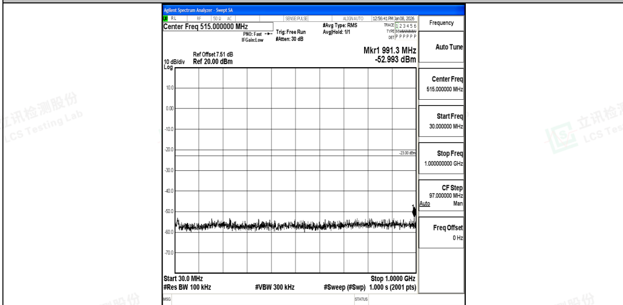
Band66_10MHz_16QAM_132022_1RB#0_30~1000_30~1000
