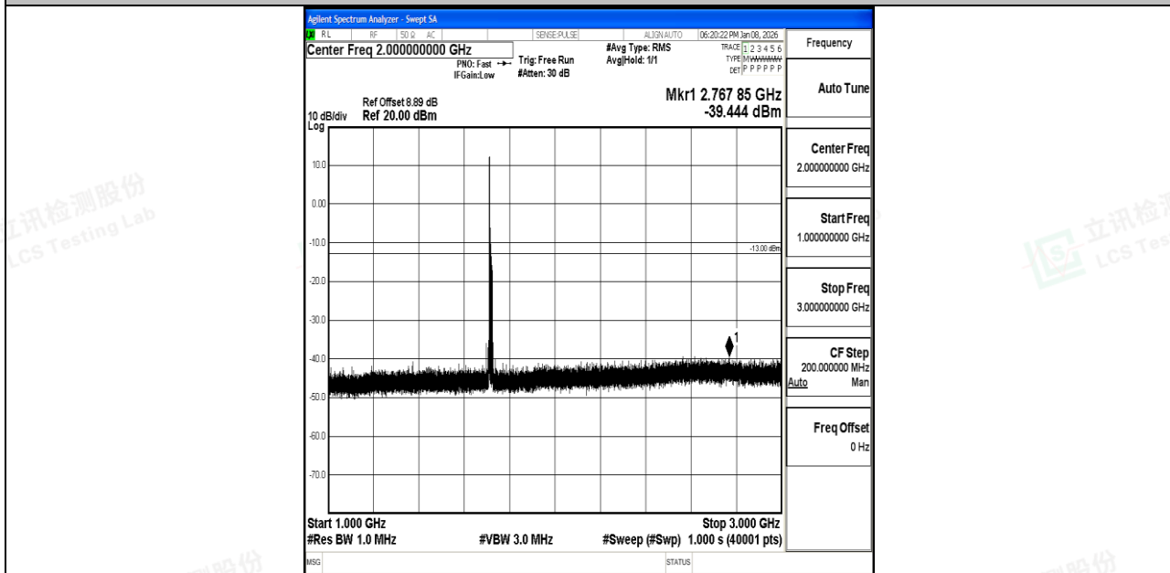
Band66_15MHz_QPSK_132047_1RB#0_1000~3000_1000~3000
