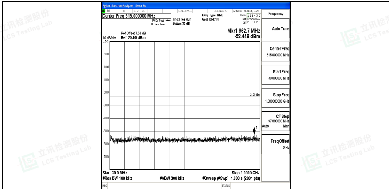
Band66_10MHz_QPSK_132622_1RB#0_30~1000_30~1000
