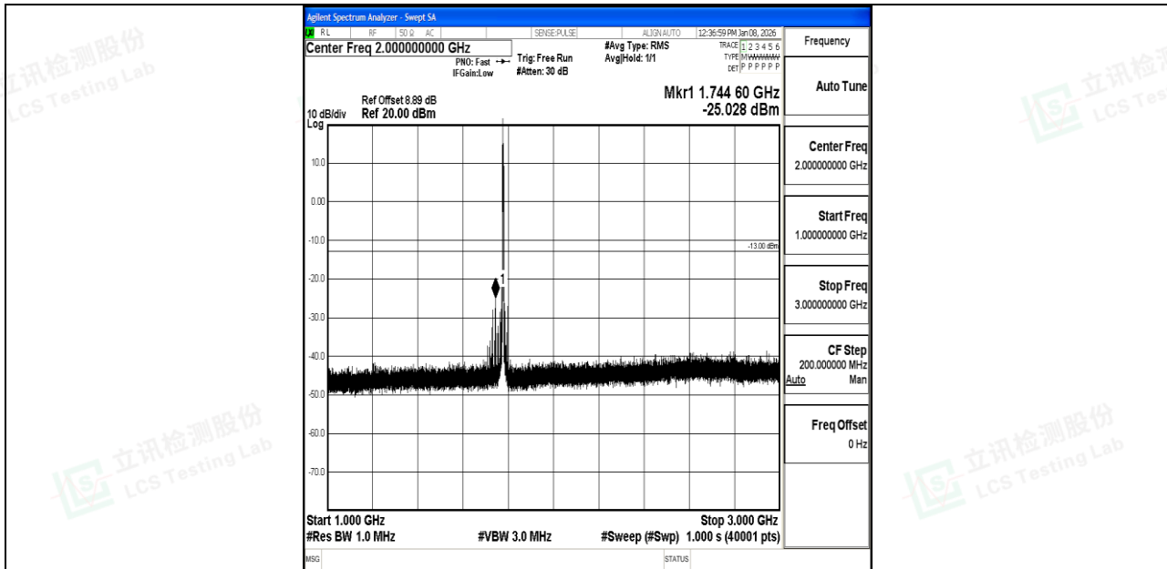
Band66_5MHz_16QAM_132647_1RB#0_1000~3000_1000~3000
