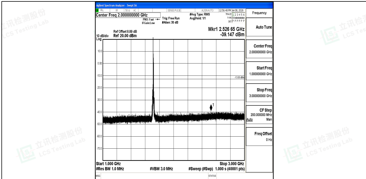
Band66_10MHz_16QAM_132022_1RB#0_1000~3000_1000~3000
