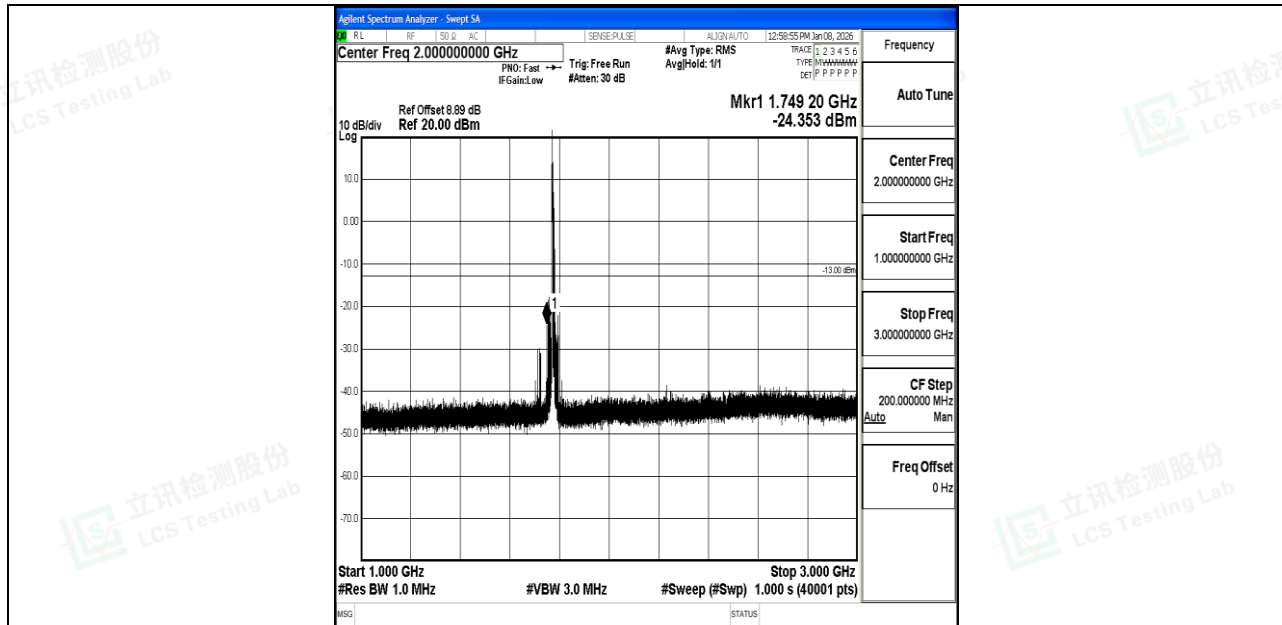
Band66_10MHz_16QAM_132622_1RB#0_1000~3000_1000~3000
