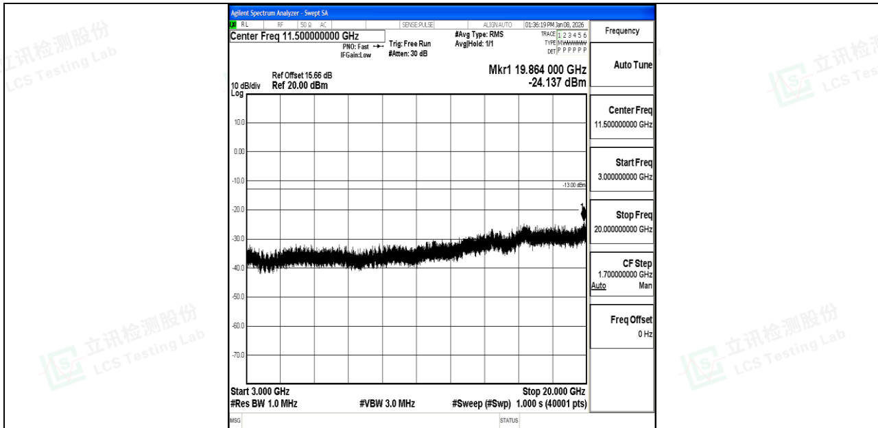
Band66_20MHz_16QAM_132072_1RB#0_3000~20000_3000~20000
