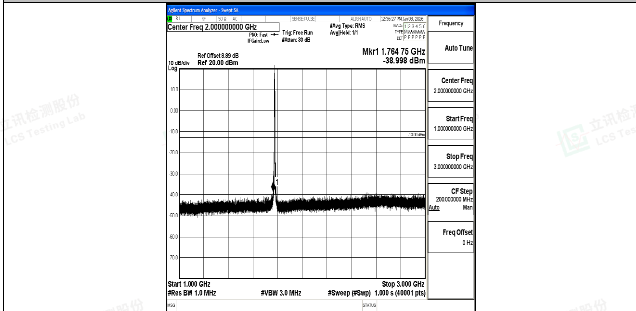
Band66_5MHz_QPSK_132647_1RB#0_1000~3000_1000~3000
