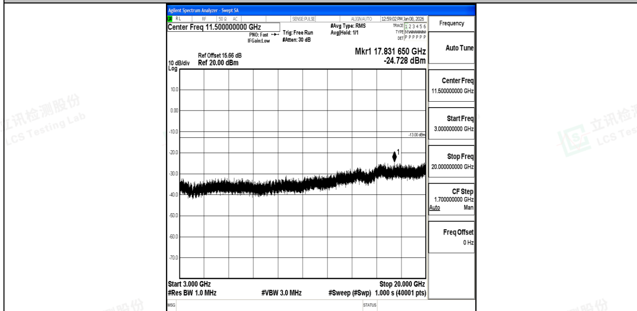
Band66_10MHz_16QAM_132622_1RB#0_3000~20000_3000~20000
