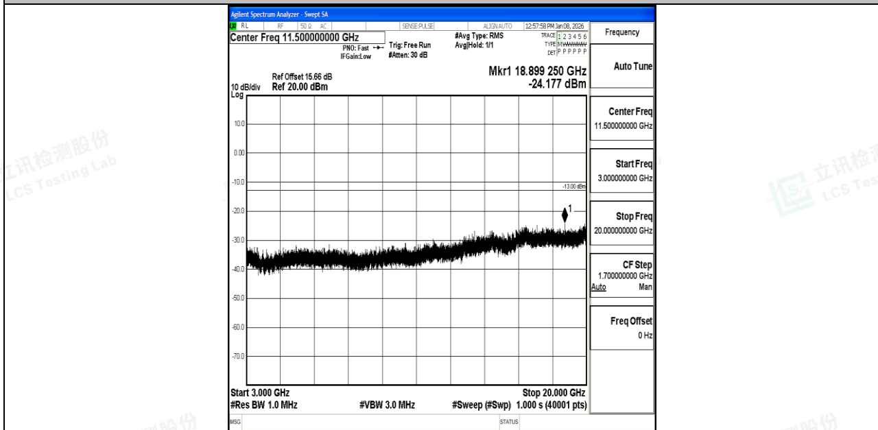
Band66_10MHz_16QAM_132322_1RB#0_3000~20000_3000~20000
