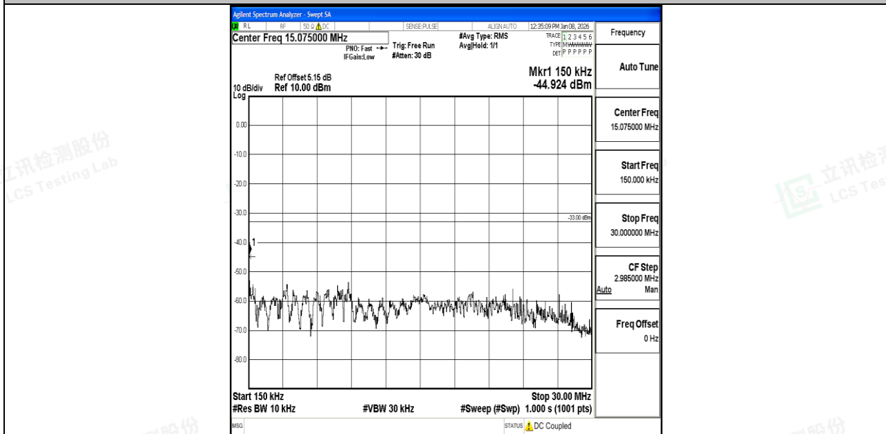
Band66_5MHz_QPSK_132322_1RB#0_0.15~30_0.15~30
