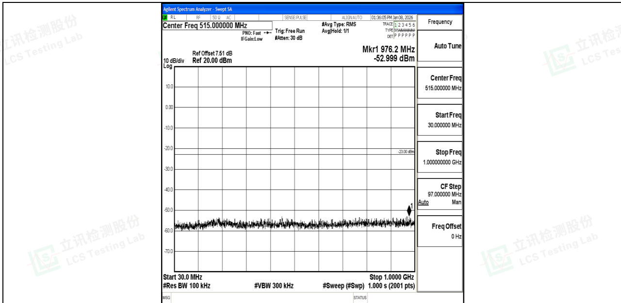
Band66_20MHz_16QAM_132072_1RB#0_30~1000_30~1000
