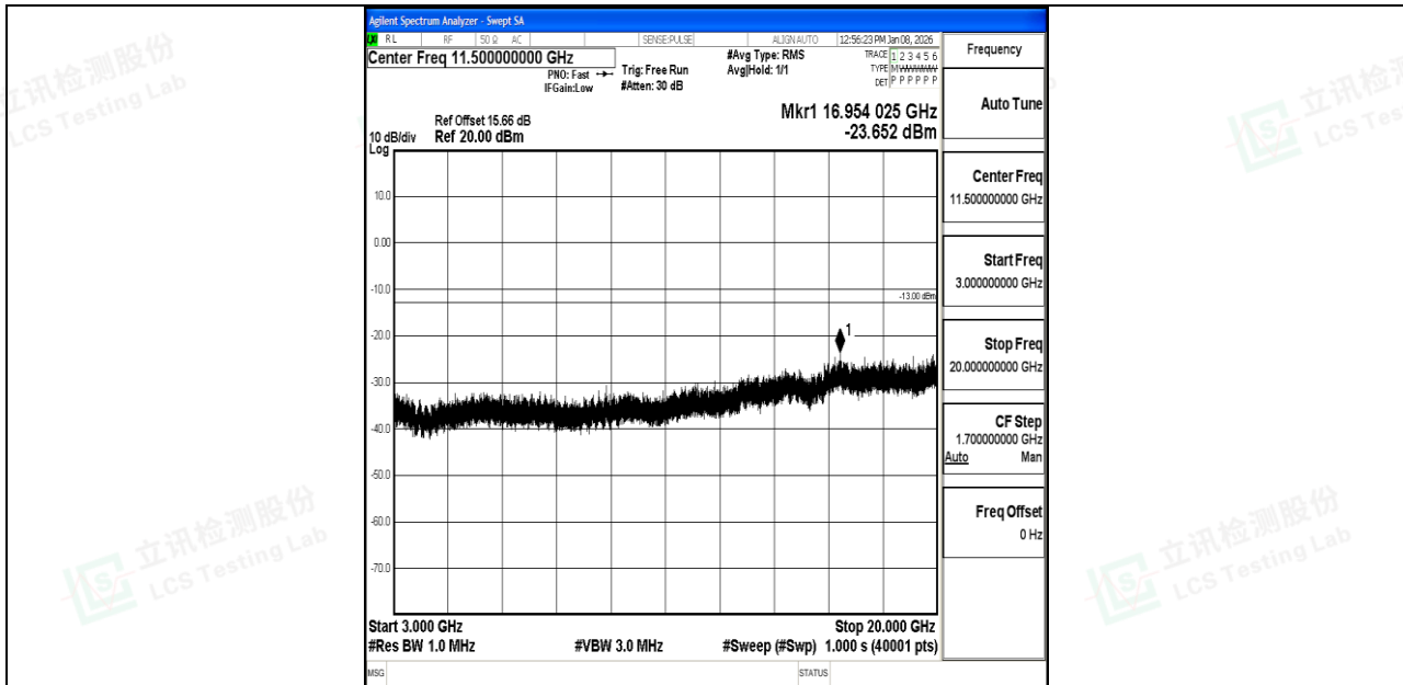
Band66_10MHz_QPSK_132022_1RB#0_3000~20000_3000~20000
