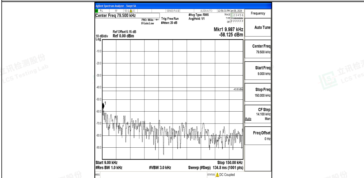
Band66_10MHz_16QAM_132022_1RB#0_0.009~0.15_0.009~0.15
