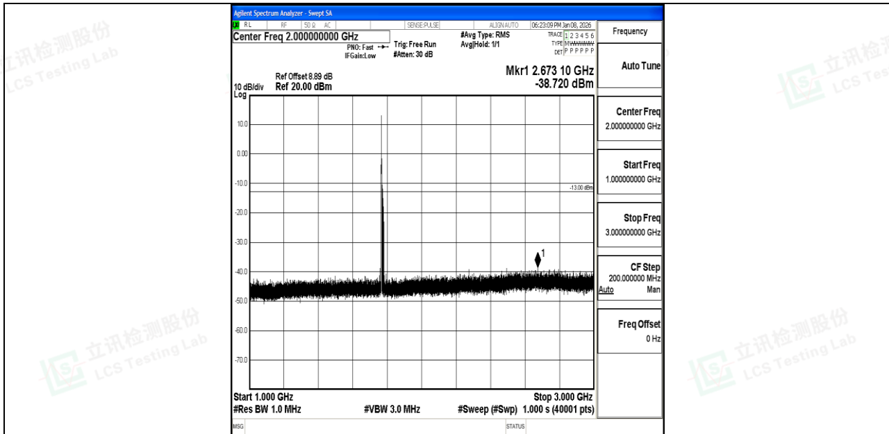
Band66_15MHz_16QAM_132597_1RB#0_1000~3000_1000~3000
