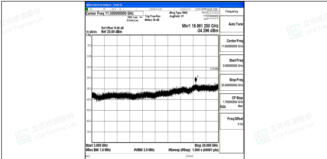
Band66_10MHz_QPSK_132322_1RB#0_3000~20000_3000~20000
