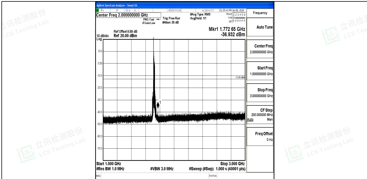
Band66_20MHz_QPSK_132072_1RB#0_1000~3000_1000~3000
