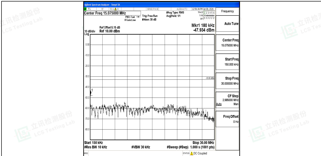
Band66_10MHz_16QAM_132022_1RB#0_0.15~30_0.15~30
