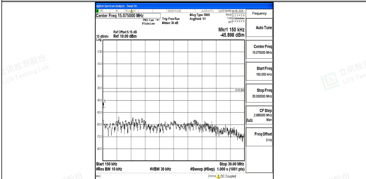
Band66_10MHz_QPSK_132322_1RB#0_0.15~30_0.15~30
