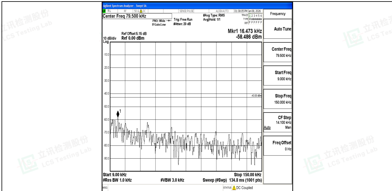
Band66_20MHz_16QAM_132572_1RB#0_0.009~0.15_0.009~0.15
