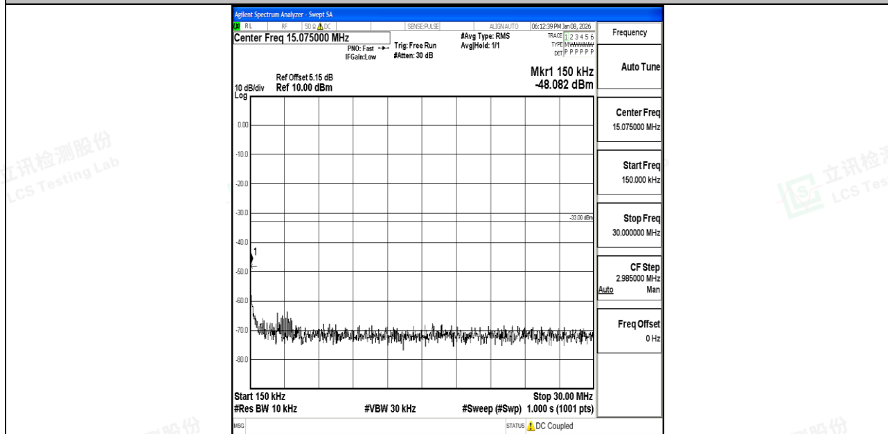
Band66_1.4MHz_QPSK_131979_1RB#0_0.15~30_0.15~30
