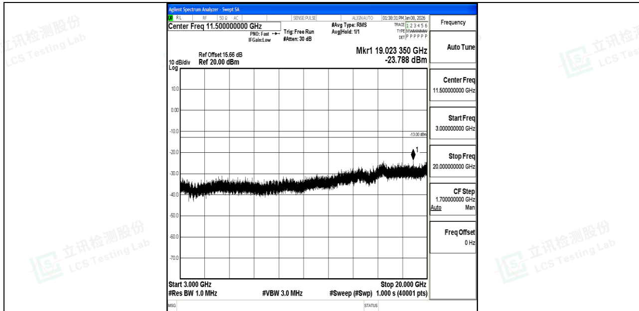
Band66_20MHz_16QAM_132572_1RB#0_3000~20000_3000~20000
