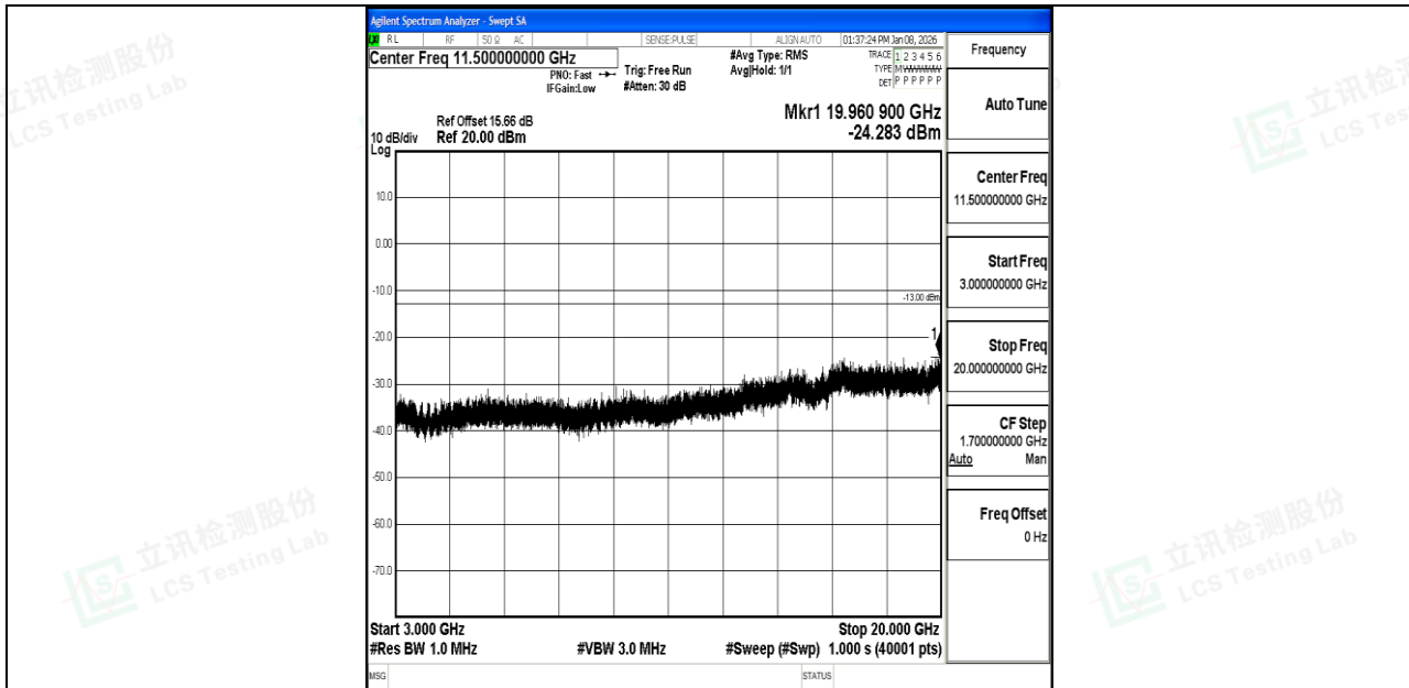
Band66_20MHz_16QAM_132322_1RB#0_3000~20000_3000~20000
