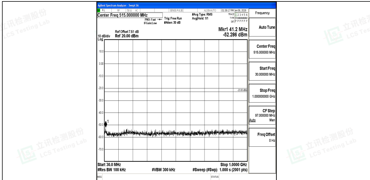
Band66_20MHz_16QAM_132572_1RB#0_30~1000_30~1000
