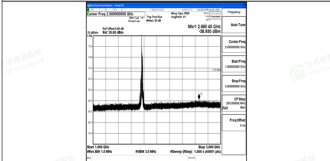
Band66_20MHz_16QAM_132572_1RB#0_1000~3000_1000~3000
