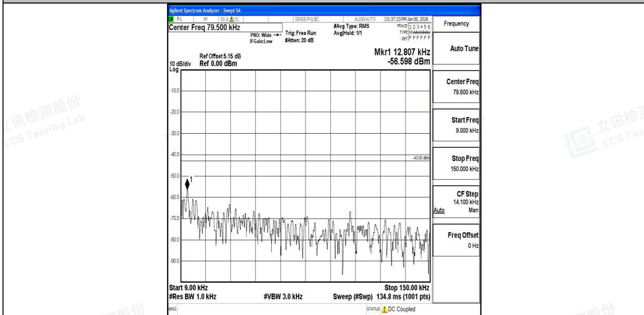
Band66_20MHz_QPSK_132572_1RB#0_0.009~0.15_0.009~0.15
