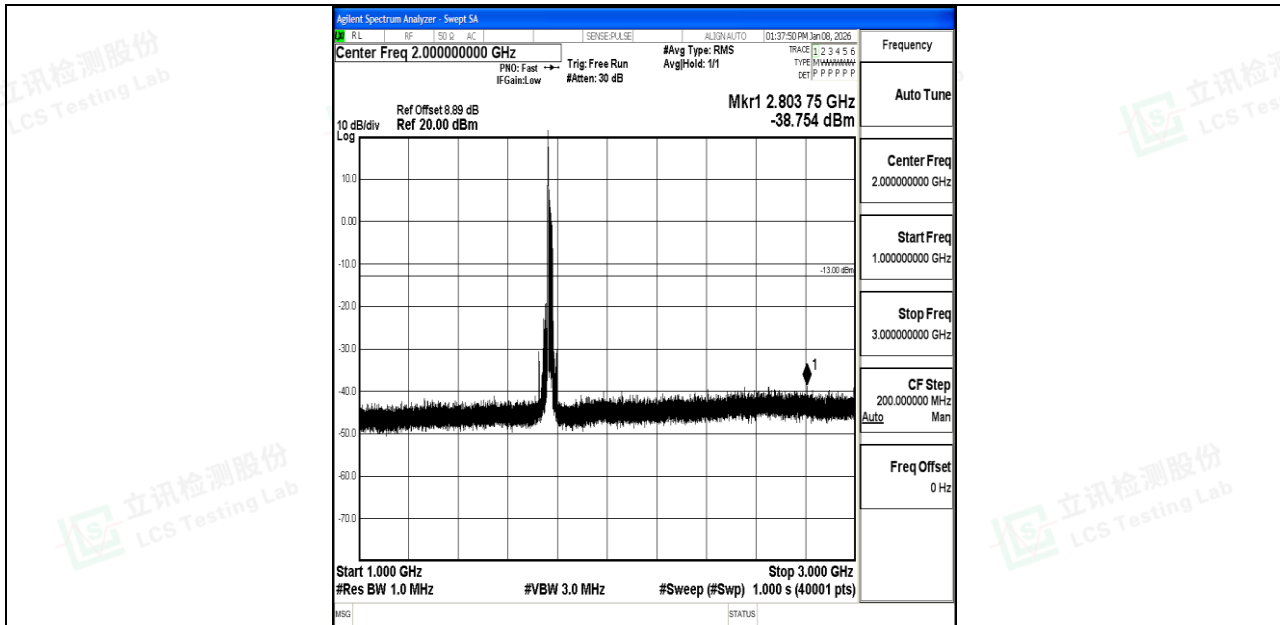
Band66_20MHz_QPSK_132572_1RB#0_1000~3000_1000~3000
