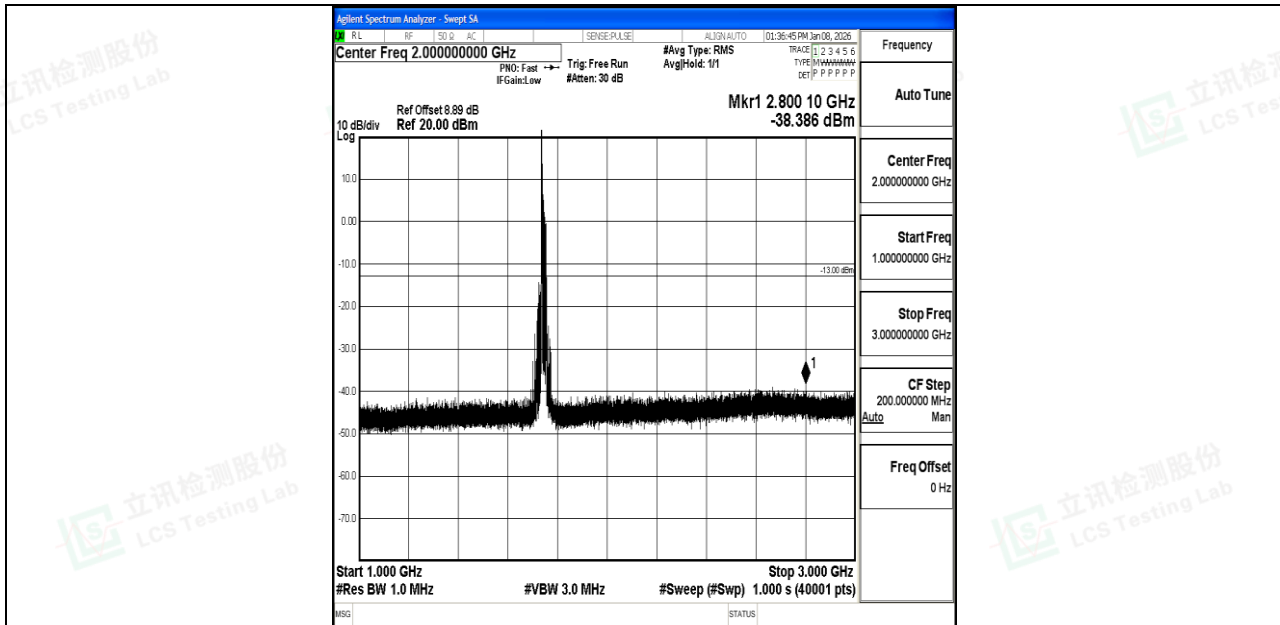
Band66_20MHz_QPSK_132322_1RB#0_1000~3000_1000~3000
