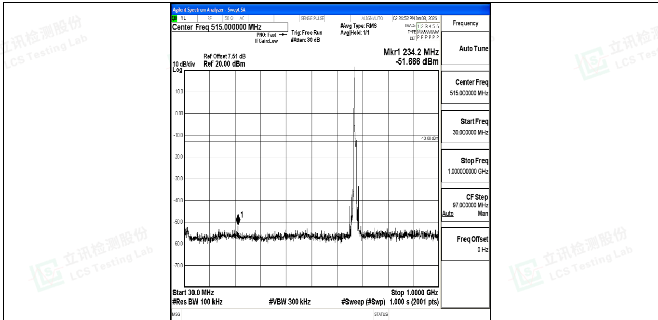
Band71_10MHz_QPSK_133297_1RB#0_30~1000_30~1000
