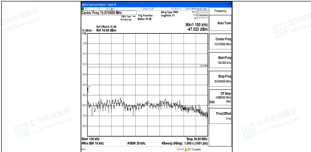
Band71_20MHz_16QAM_133322_1RB#0_0.15~30_0.15~30
