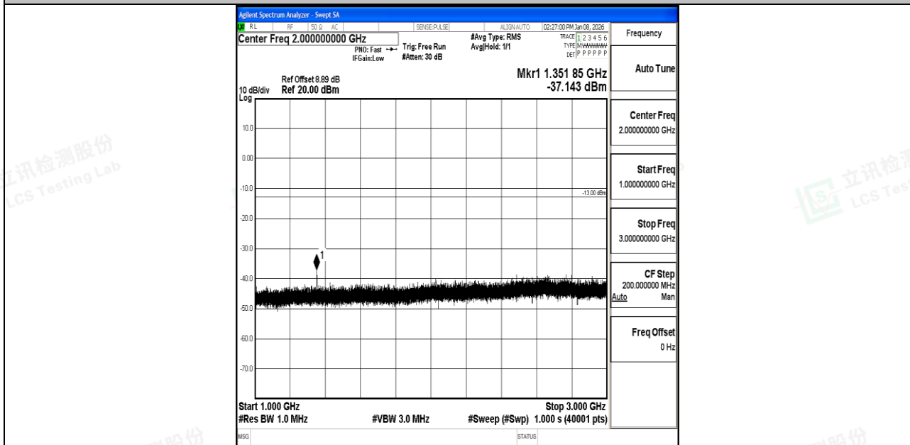
Band71_10MHz_QPSK_133297_1RB#0_1000~3000_1000~3000
