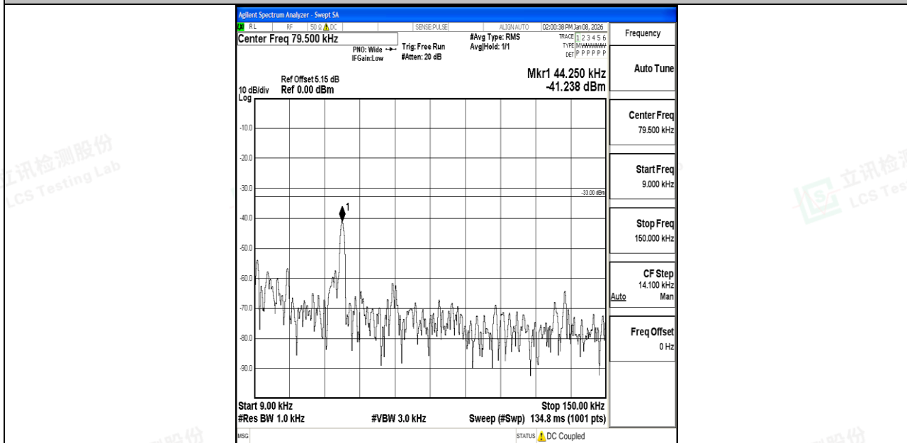
Band71_5MHz_16QAM_133297_1RB#0_0.009~0.15_0.009~0.15
