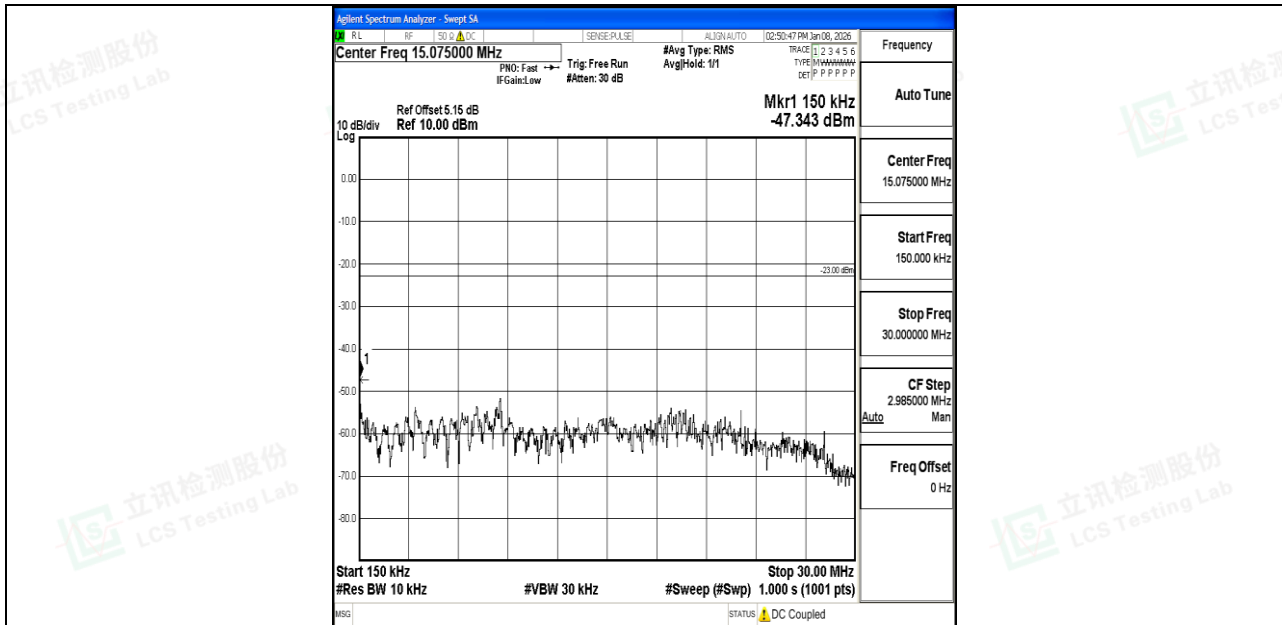
Band71_15MHz_16QAM_133197_1RB#0_0.15~30_0.15~30
