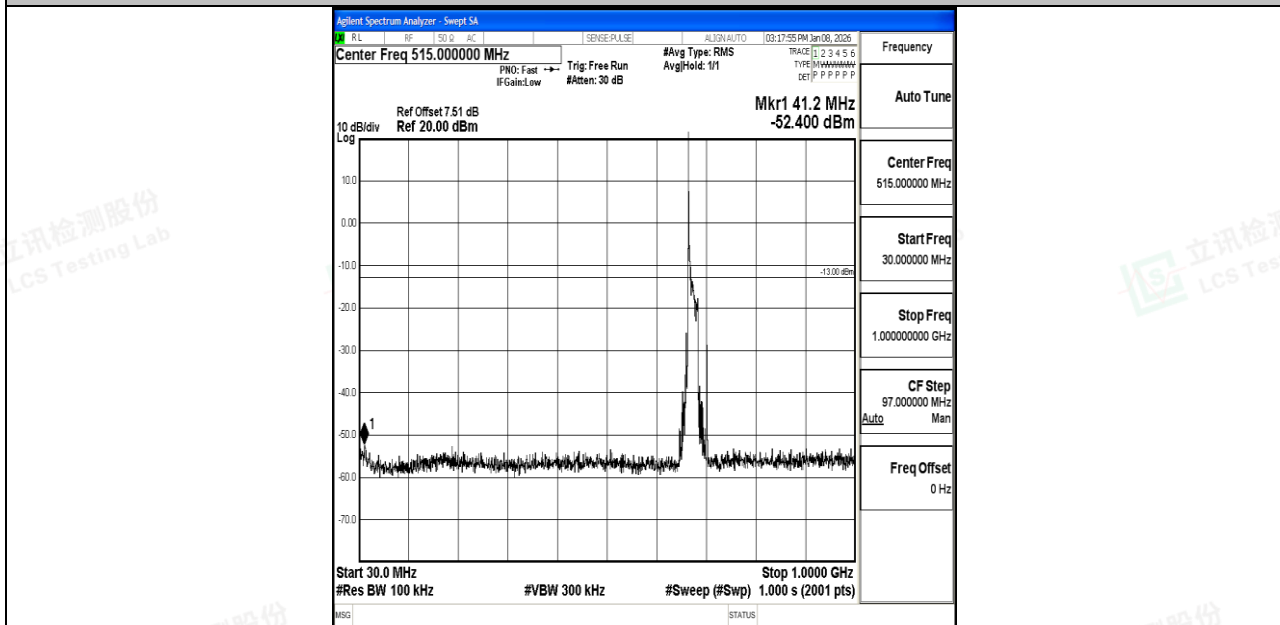
Band71_20MHz_16QAM_133322_1RB#0_30~1000_30~1000
