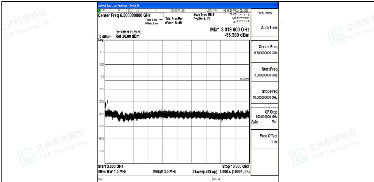
Band71_15MHz_QPSK_133197_1RB#0_3000~10000_3000~10000
