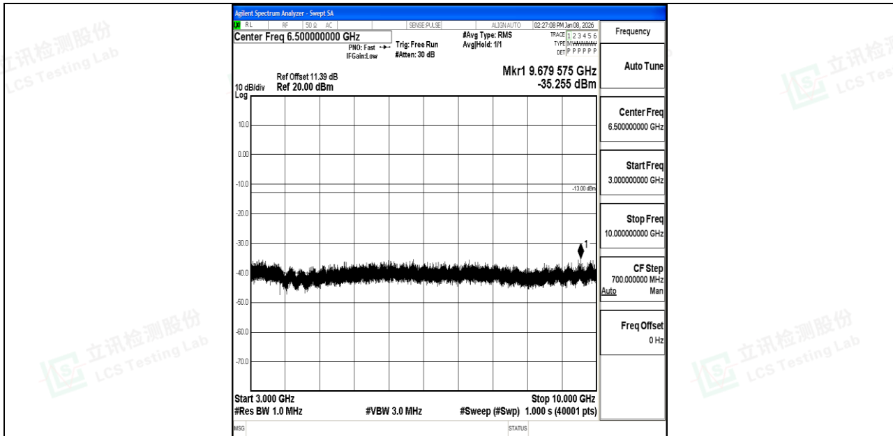
Band71_10MHz_QPSK_133297_1RB#0_3000~10000_3000~10000
