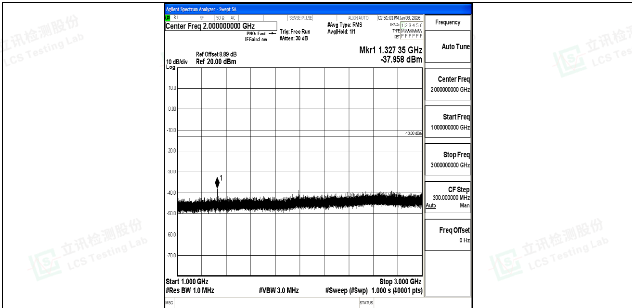
Band71_15MHz_16QAM_133197_1RB#0_1000~3000_1000~3000
