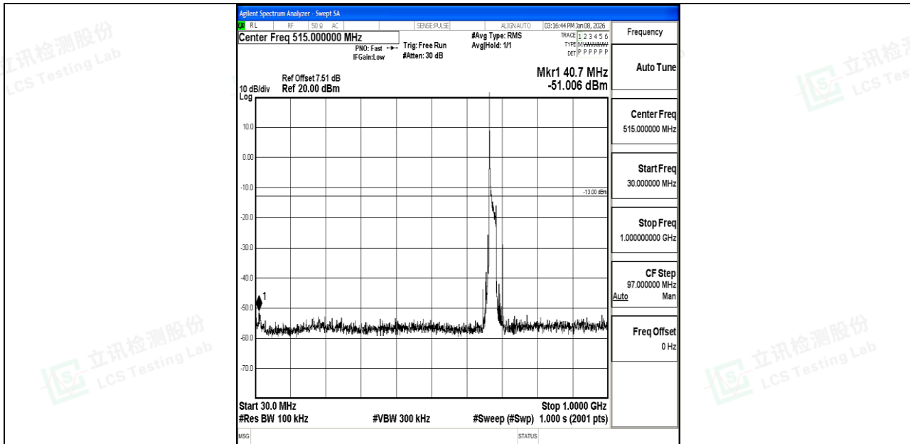
Band71_20MHz_QPSK_133322_1RB#0_30~1000_30~1000
