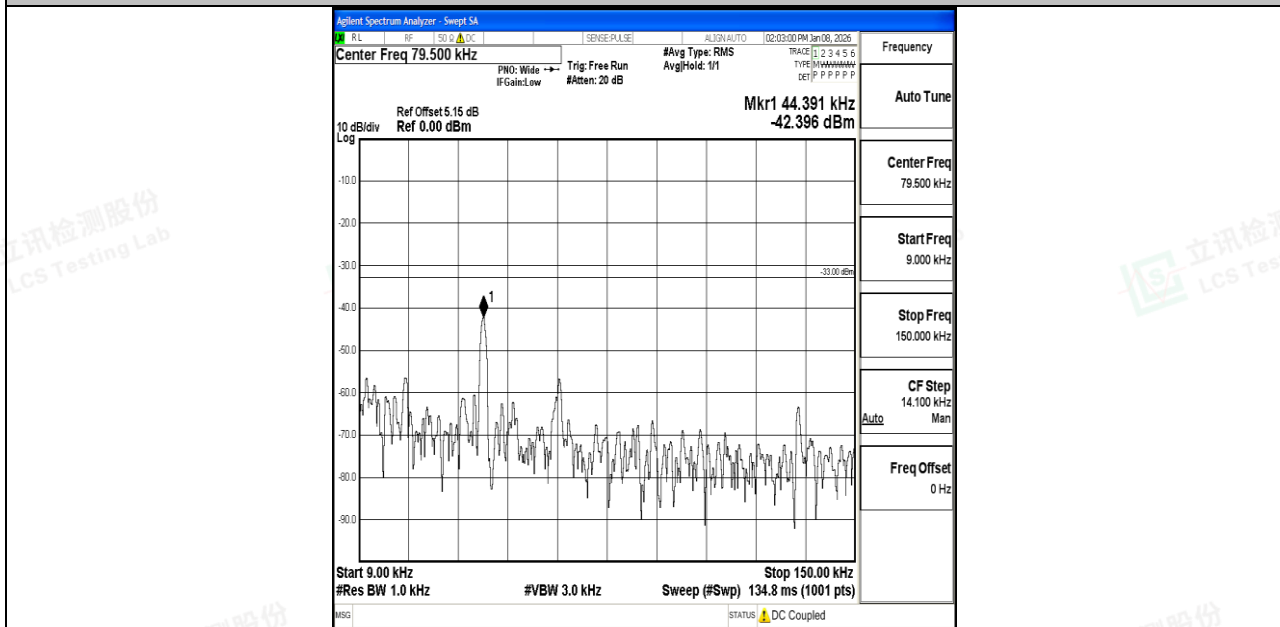
Band71_5MHz_16QAM_133447_1RB#0_0.009~0.15_0.009~0.15
