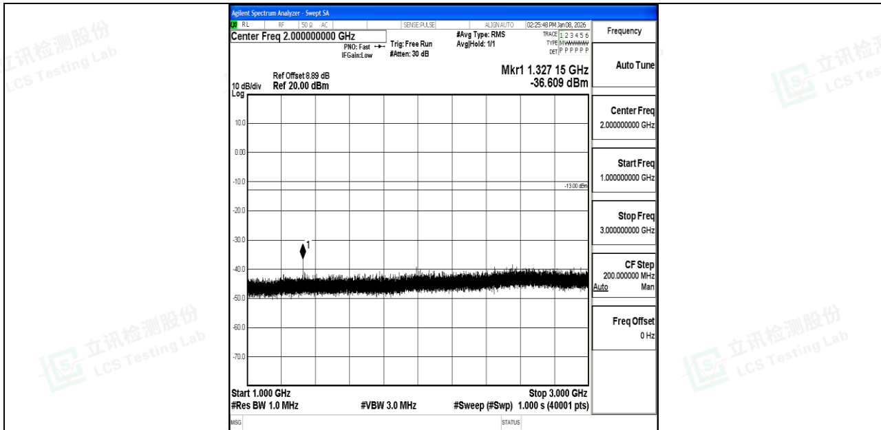
Band71_10MHz_16QAM_133172_1RB#0_1000~3000_1000~3000
