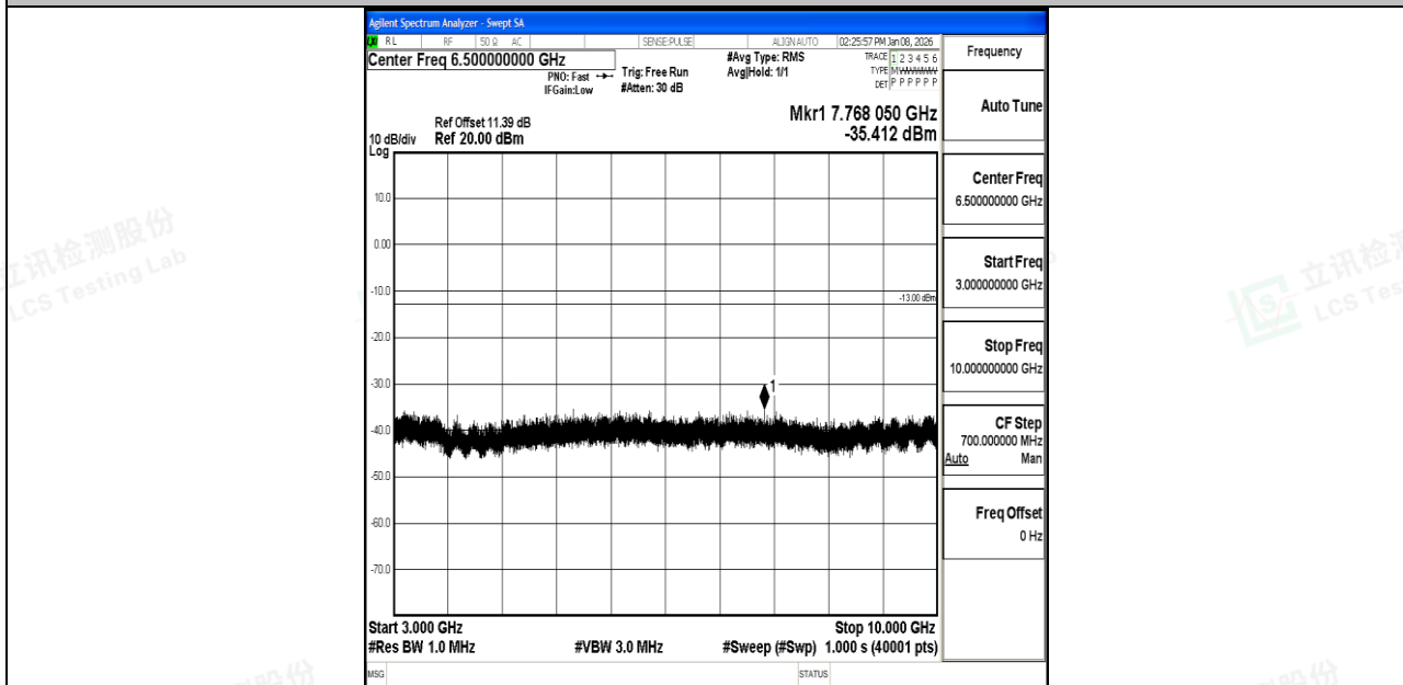
Band71_10MHz_16QAM_133172_1RB#0_3000~10000_3000~10000
