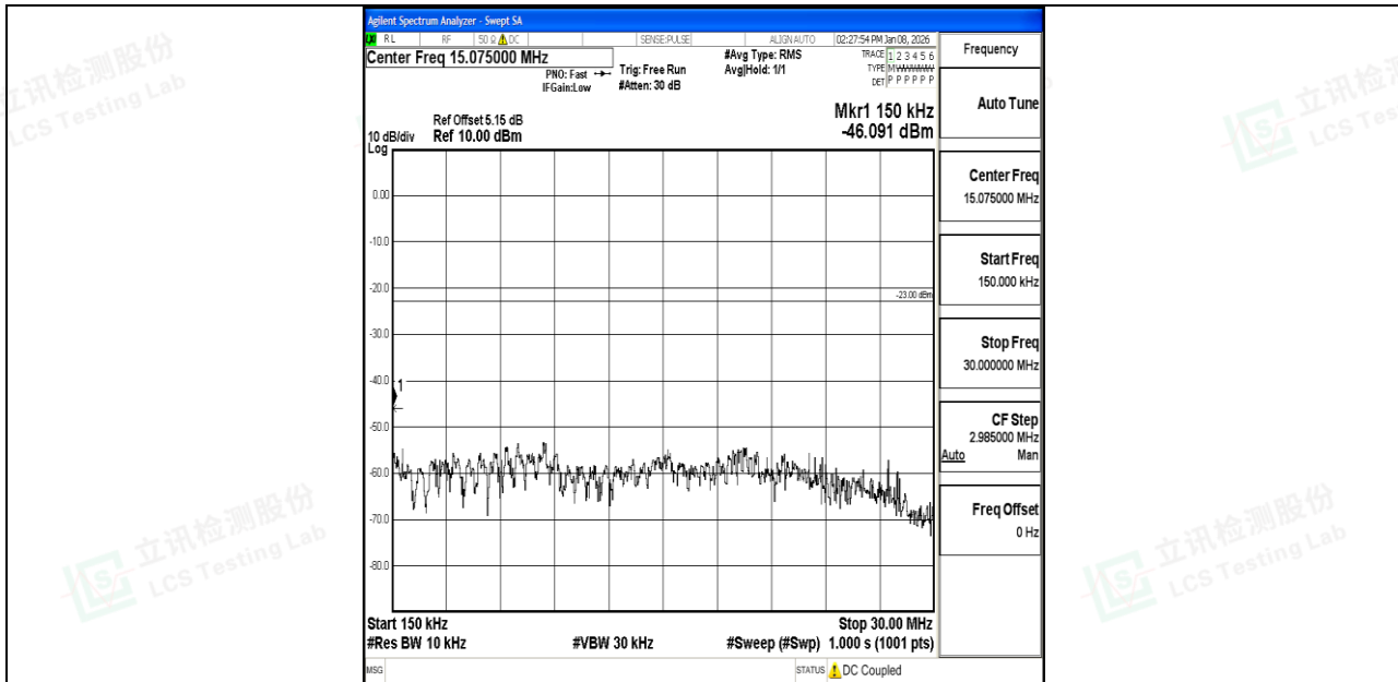
Band71_10MHz_16QAM_133297_1RB#0_0.15~30_0.15~30
