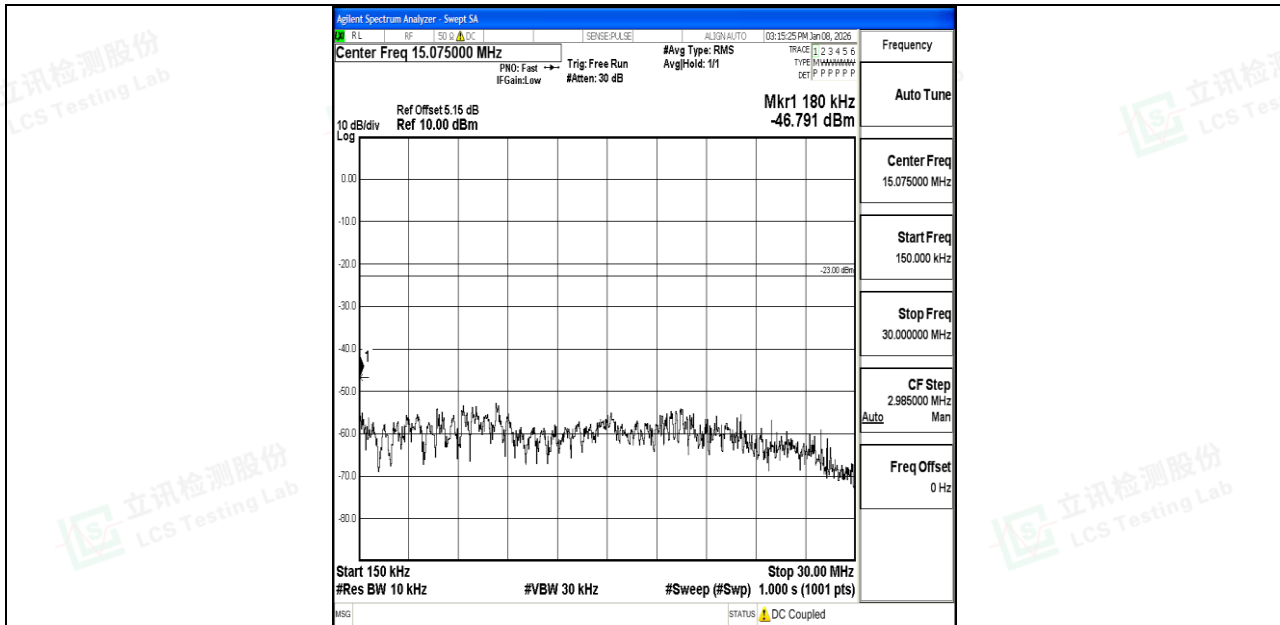
Band71_20MHz_16QAM_133222_1RB#0_0.15~30_0.15~30
