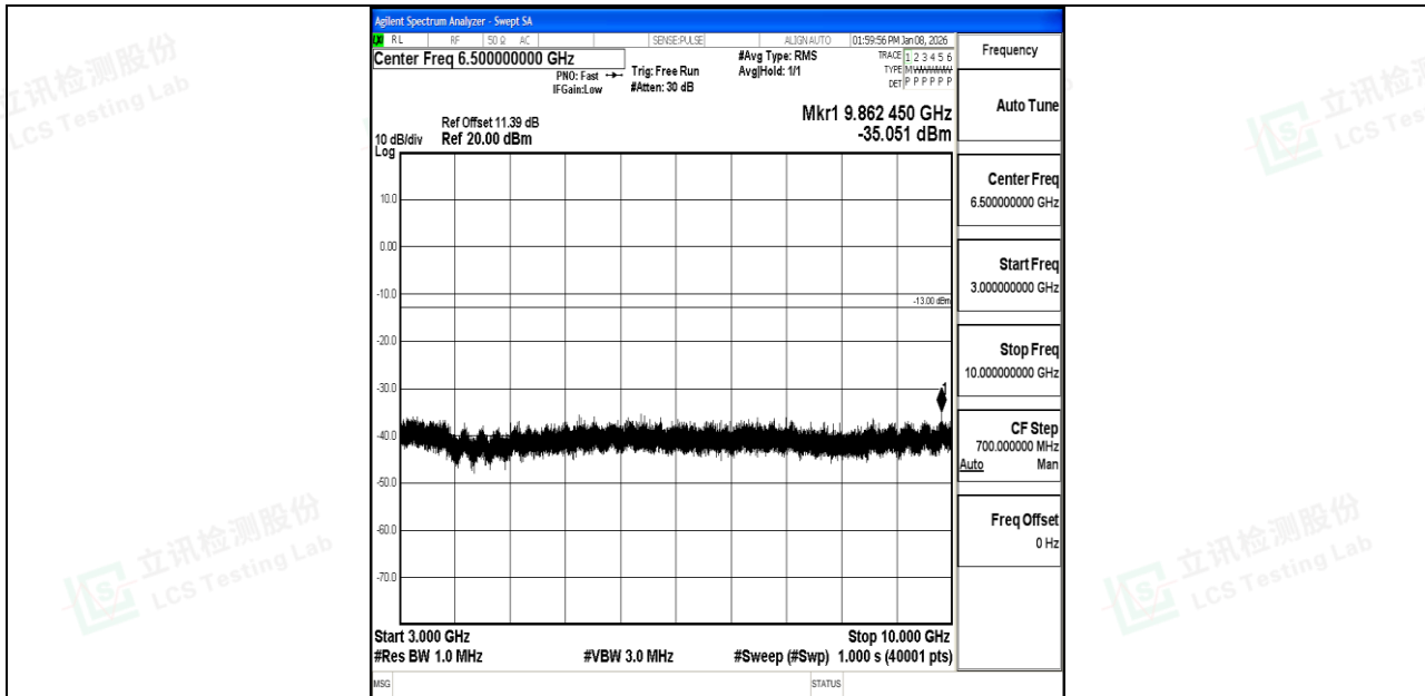
Band71_5MHz_QPSK_133297_1RB#0_3000~10000_3000~10000
