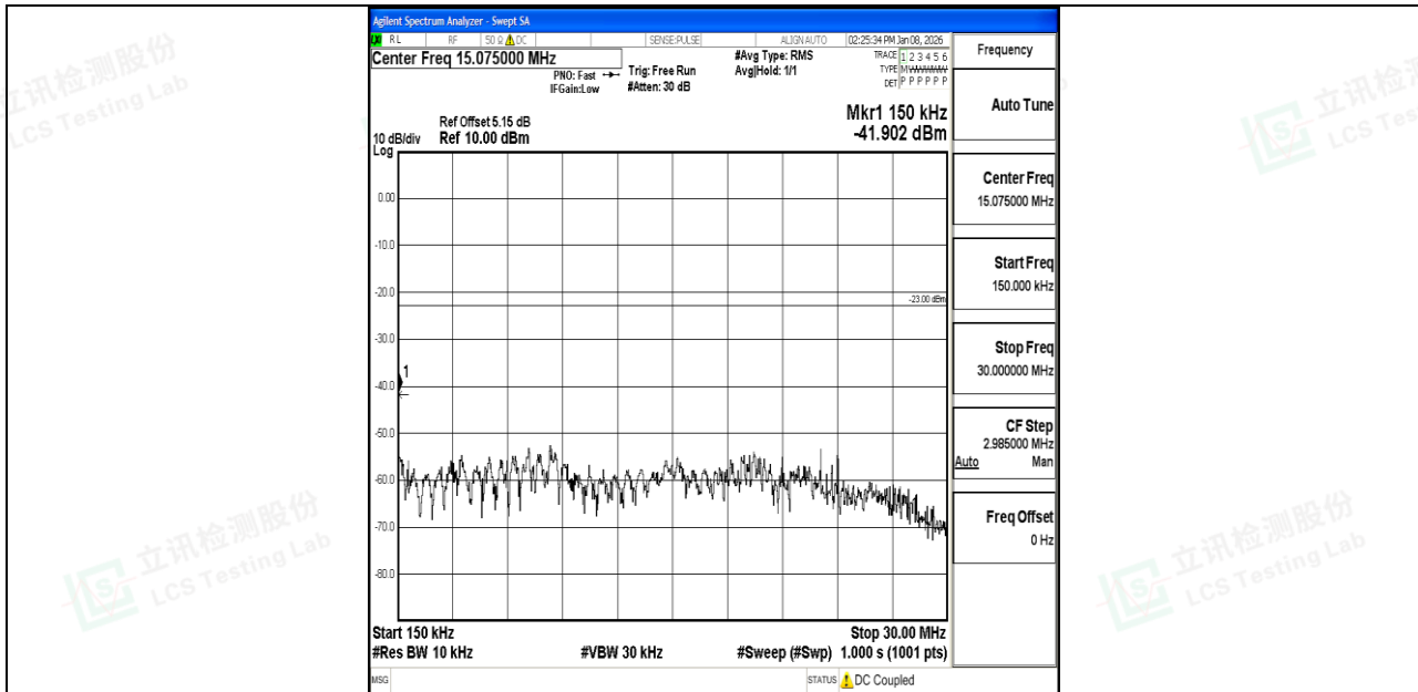
Band71_10MHz_16QAM_133172_1RB#0_0.15~30_0.15~30
