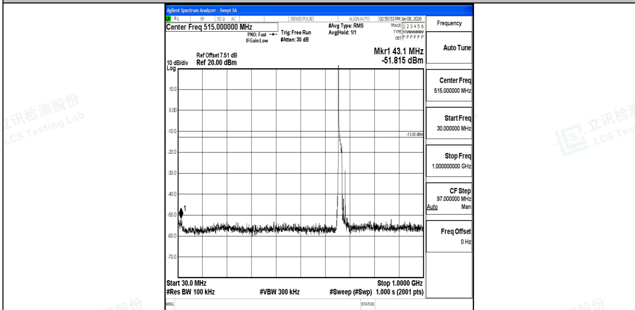
Band71_15MHz_16QAM_133197_1RB#0_30~1000_30~1000
