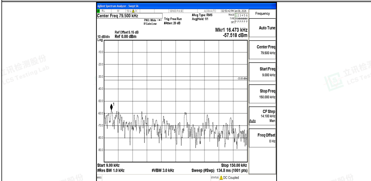
Band71_15MHz_16QAM_133197_1RB#0_0.009~0.15_0.009~0.15
