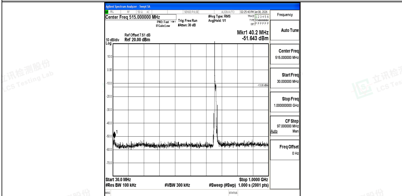
Band71_10MHz_16QAM_133172_1RB#0_30~1000_30~1000
