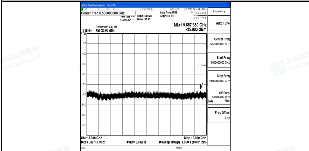
Band71_10MHz_16QAM_133297_1RB#0_3000~10000_3000~10000
