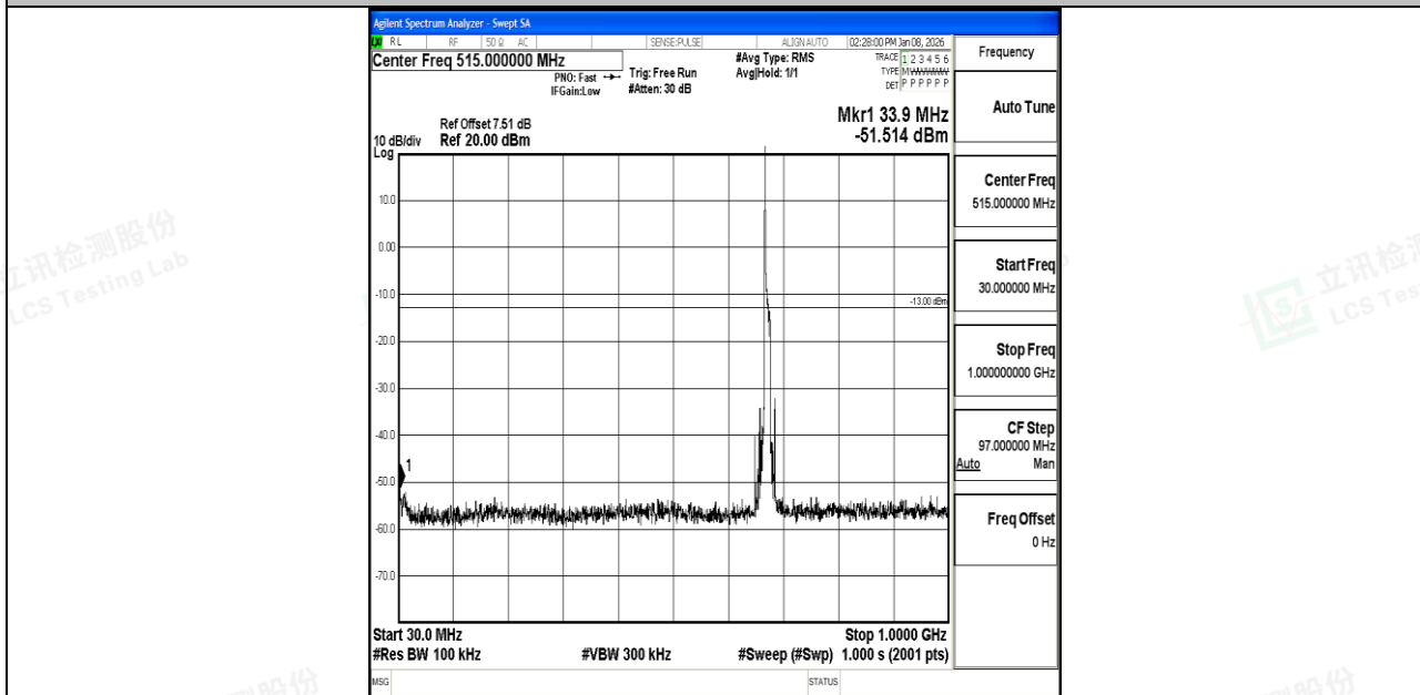
Band71_10MHz_16QAM_133297_1RB#0_30~1000_30~1000
