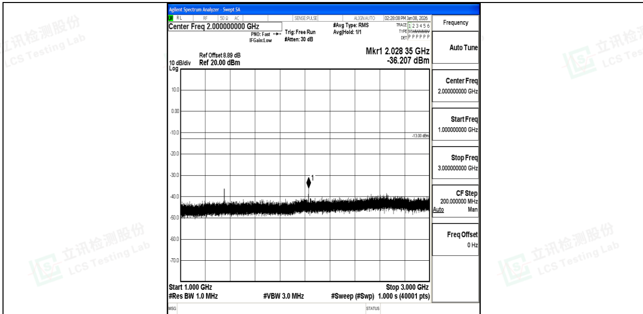
Band71_10MHz_16QAM_133297_1RB#0_1000~3000_1000~3000
