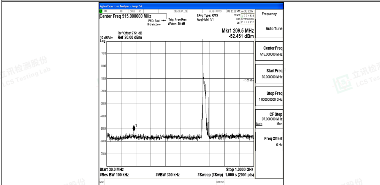
Band71_20MHz_16QAM_133222_1RB#0_30~1000_30~1000
