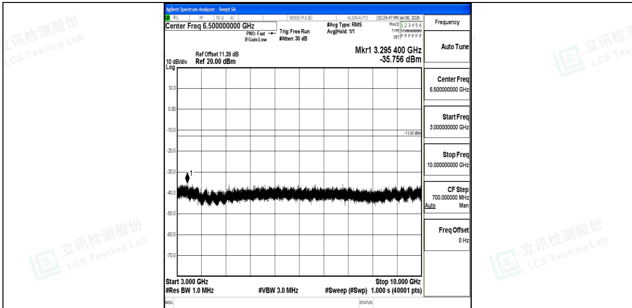
Band71_10MHz_QPSK_133172_1RB#0_3000~10000_3000~10000
