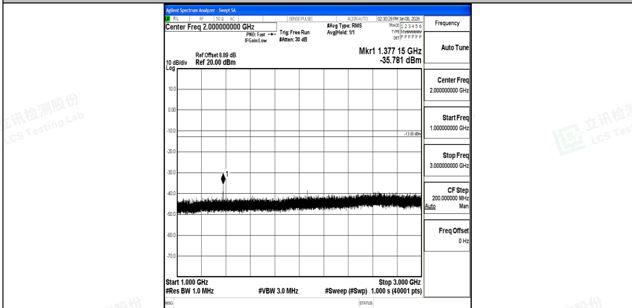
Band71_10MHz_16QAM_133422_1RB#0_1000~3000_1000~3000
