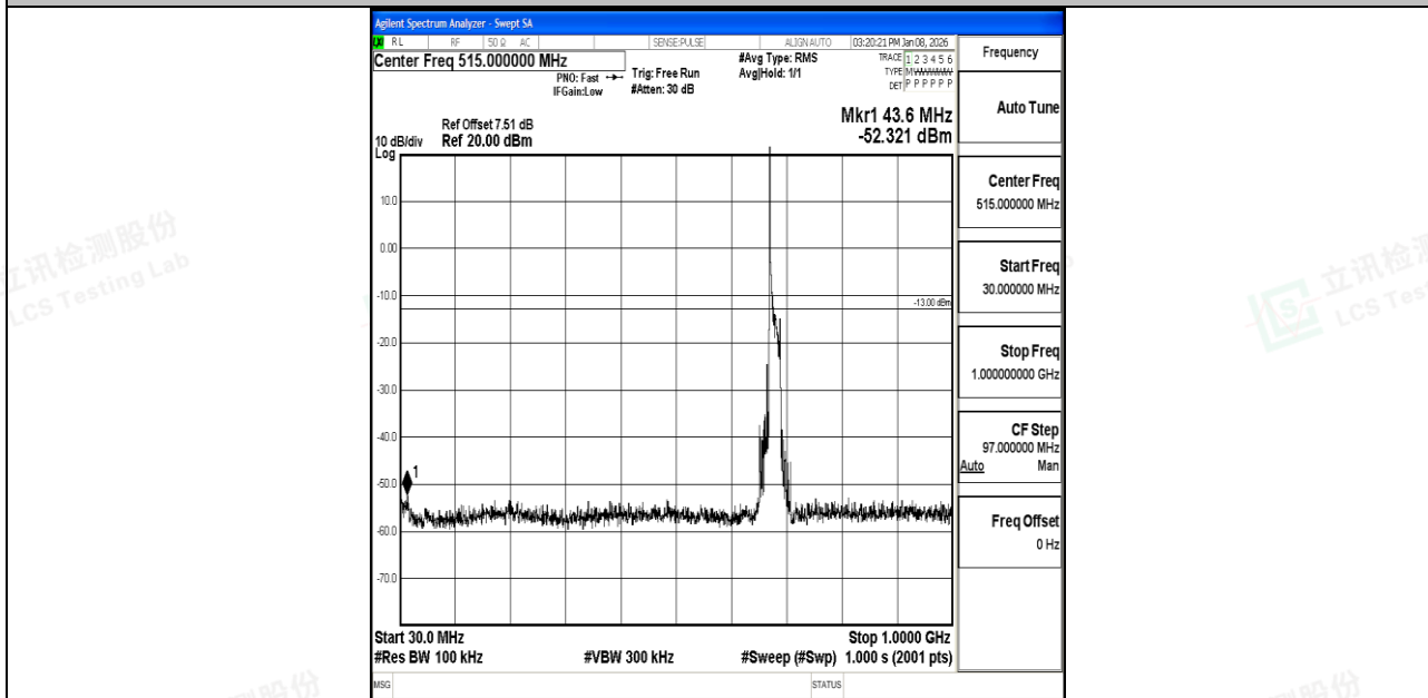
Band71_20MHz_16QAM_133372_1RB#0_30~1000_30~1000
