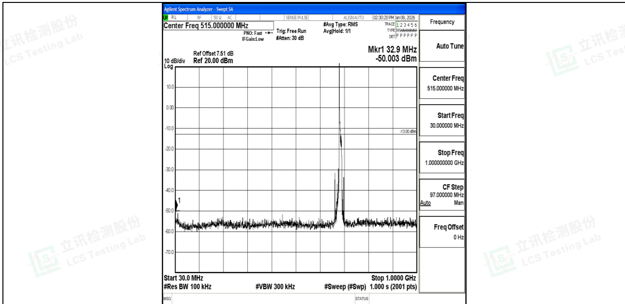
Band71_10MHz_16QAM_133422_1RB#0_30~1000_30~1000
