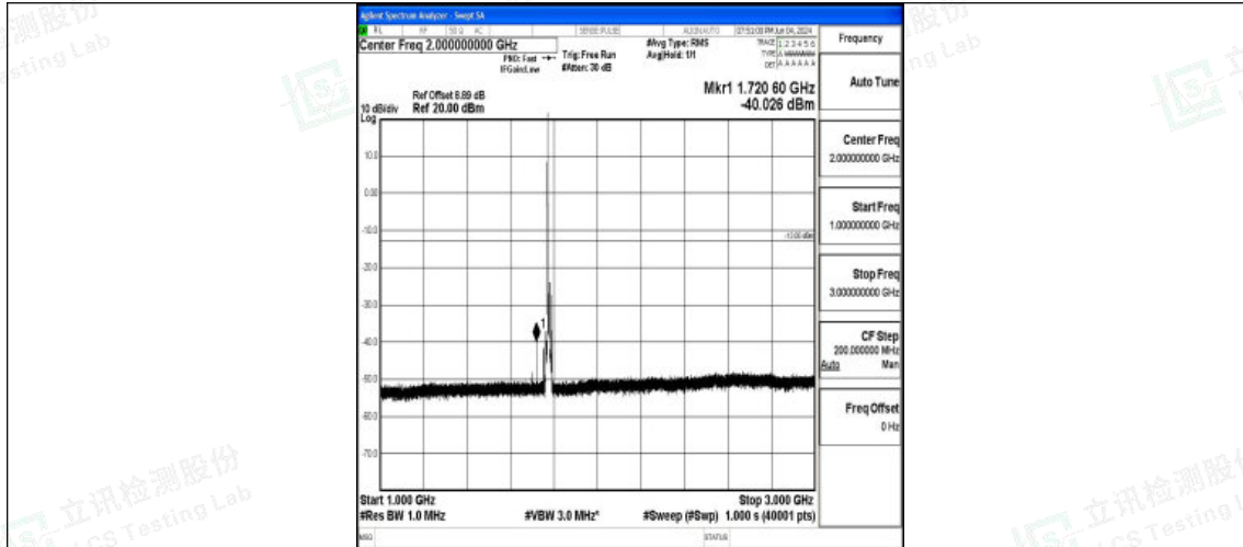
Band66_10MHz_16QAM_132622_1RB#0_1000~3000_1000~3000
