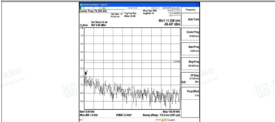
Band66_15MHz_QPSK_132597_1RB#0_0.009~0.15_0.009~0.15
