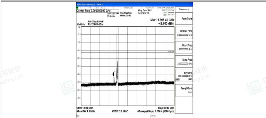
Band66_10MHz_QPSK_132622_1RB#0_1000~3000_1000~3000
