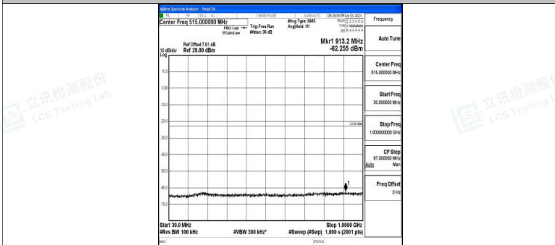
Band66_20MHz_16QAM_132572_1RB#0_30~1000_30~1000
