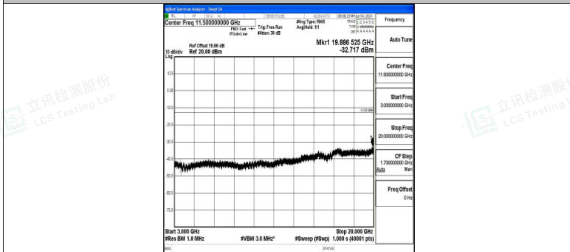
Band66_15MHz_QPSK_132597_1RB#0_3000~20000_3000~20000
