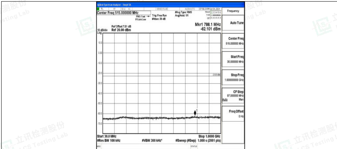
Band66_10MHz_QPSK_132622_1RB#0_30~1000_30~1000
