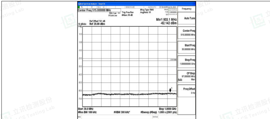
Band66_5MHz_QPSK_132647_1RB#0_30~1000_30~1000
