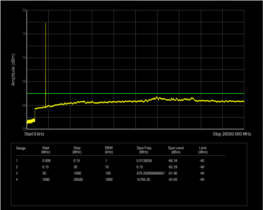
Band30 QPSK BW=10MHz Channel=27710 RB Size=1 Position=#0
