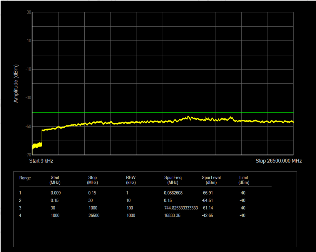
Band30 16QAM BW=10MHz Channel=27710 RB Size=1 Position=#0
