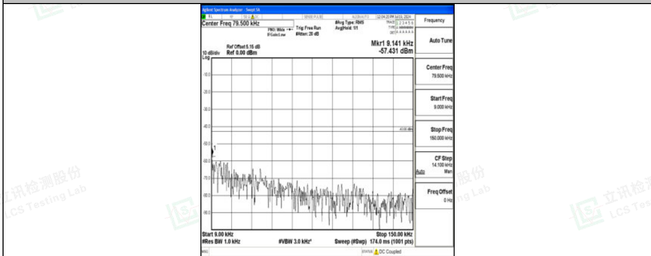
Band2_10MHz_QPSK_18650_1RB#0_0.009~0.15_0.009~0.15
