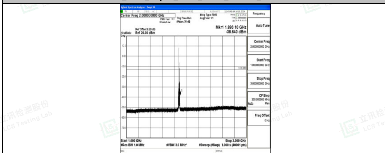
Band2_5MHz_16QAM_18900_1RB#0_1000~3000_1000~3000
