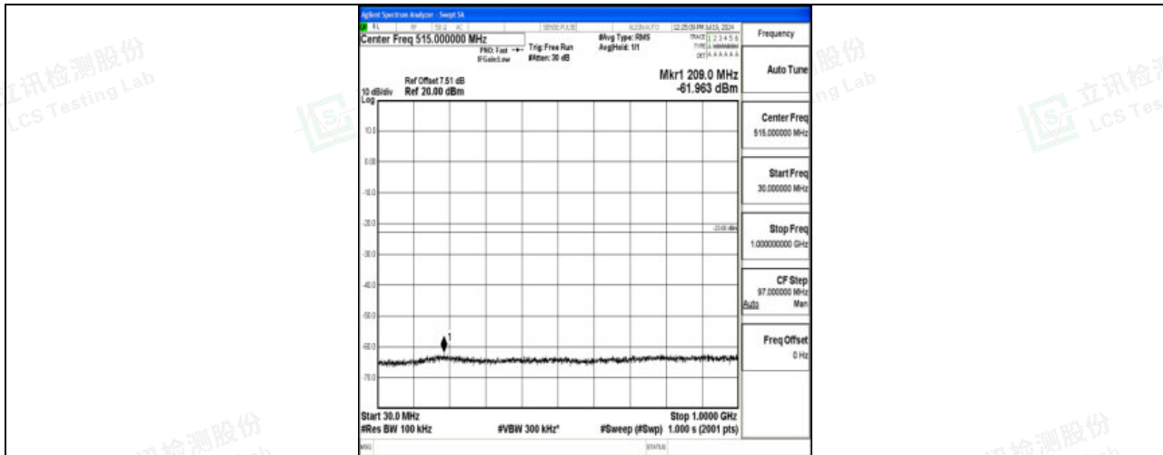
Band2_15MHz_QPSK_18675_1RB#0_30~1000_30~1000
