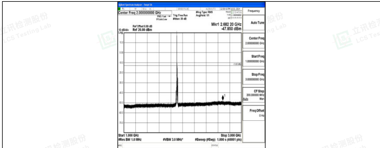
Band2_10MHz_QPSK_19150_1RB#0_1000~3000_1000~3000
