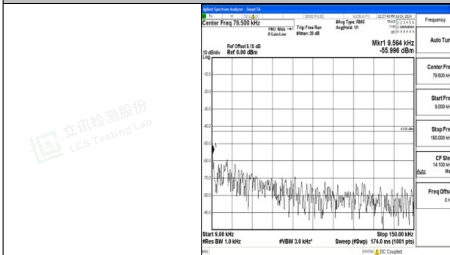
Band2_15MHz_16QAM_19125_1RB#0_0.009~0.15_0.009~0.15
