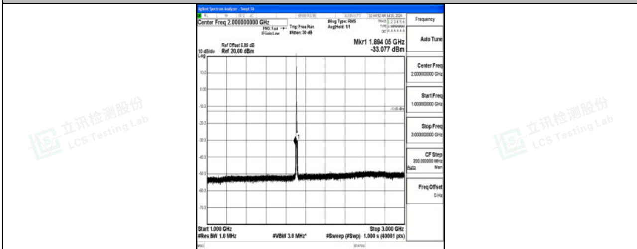
Band2_5MHz_16QAM_19175_1RB#0_1000~3000_1000~3000
