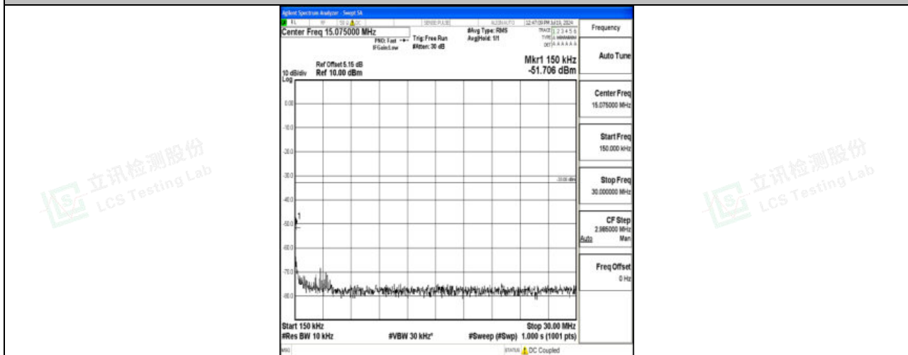
Band2_20MHz_16QAM_18900_1RB#0_0.15~30_0.15~30
