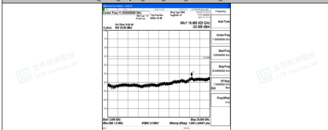
Band2_5MHz_16QAM_18900_1RB#0_3000~20000_3000~20000
