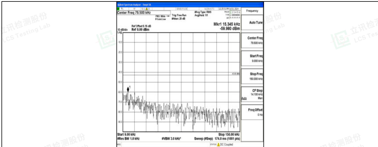
Band2_15MHz_16QAM_18675_1RB#0_0.009~0.15_0.009~0.15
