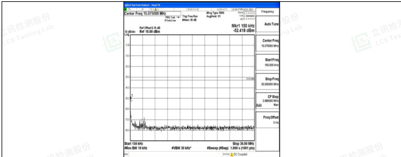
Band2_20MHz_QPSK_18900_1RB#0_0.15~30_0.15~30
