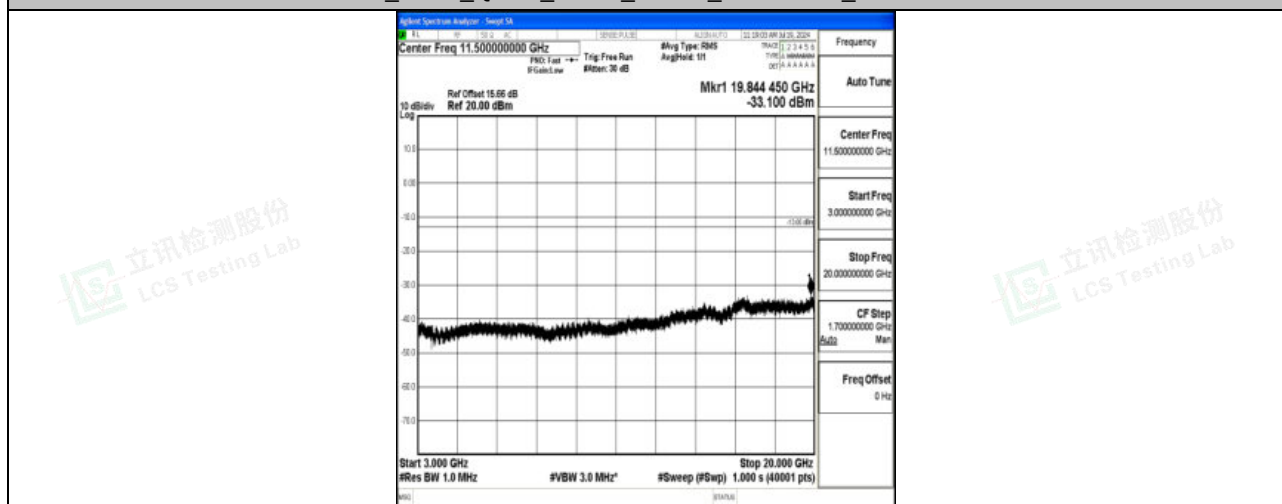
Band2_3MHz_QPSK_18615_1RB#0_3000~20000_3000~20000
