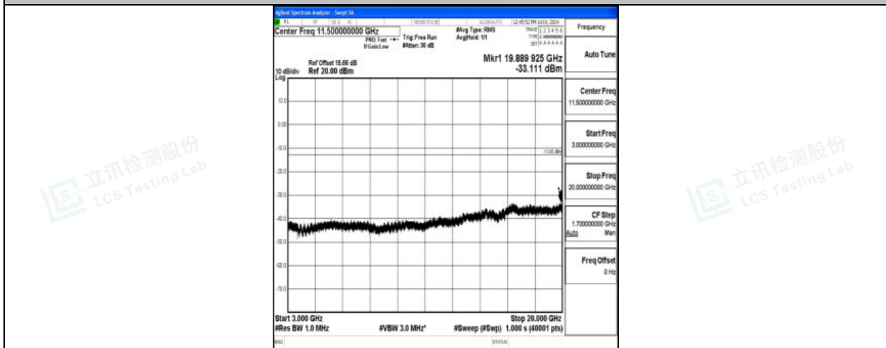
Band2_20MHz_QPSK_18700_1RB#0_3000~20000_3000~20000
