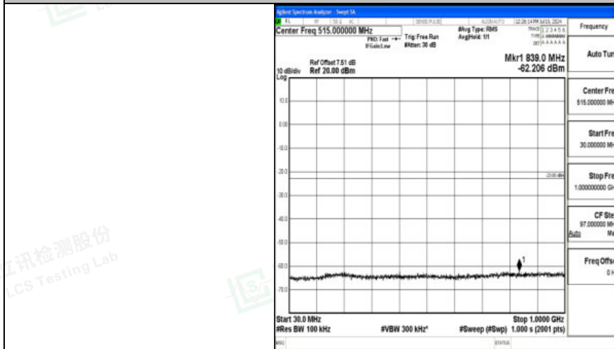
Band2_15MHz_QPSK_18900_1RB#0_30~1000_30~1000
