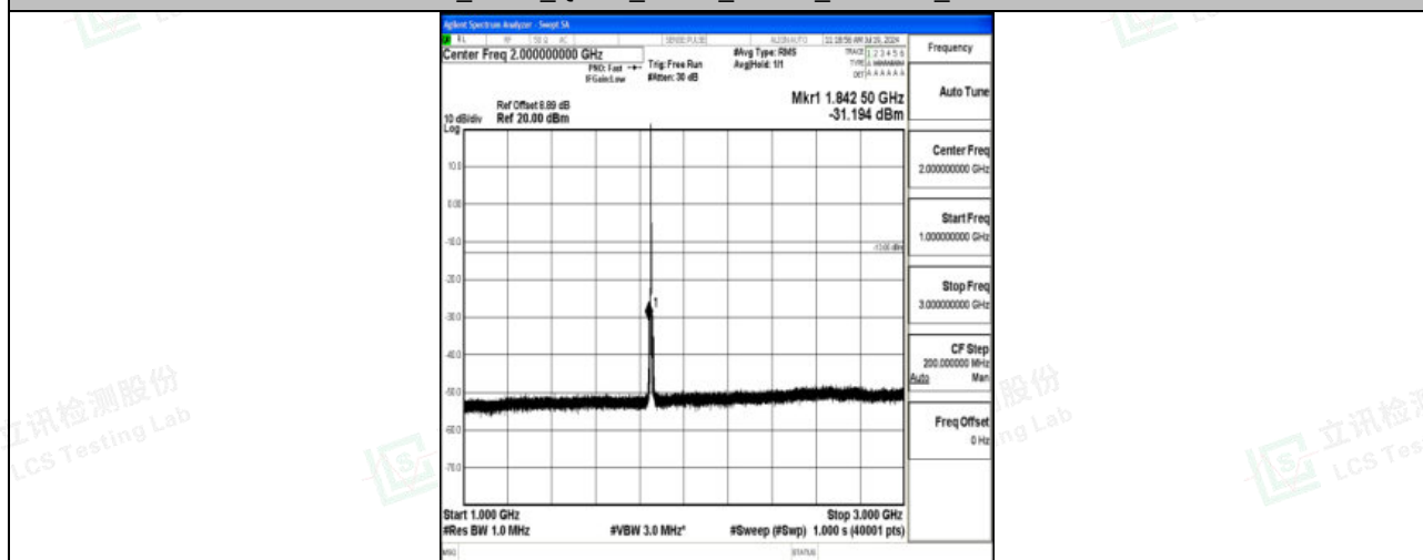
Band2_3MHz_QPSK_18615_1RB#0_1000~3000_1000~3000
