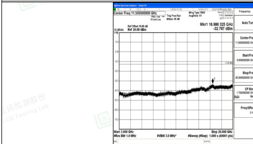
Band2_15MHz_QPSK_19125_1RB#0_3000~20000_3000~20000
