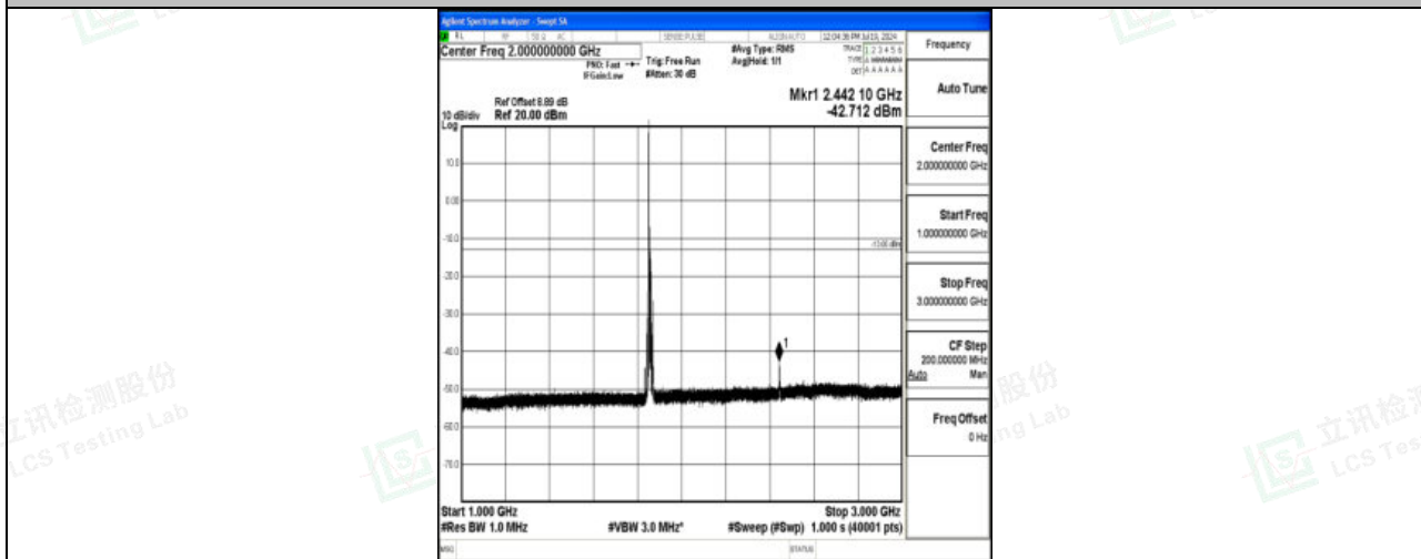
Band2_10MHz_QPSK_18650_1RB#0_1000~3000_1000~3000
