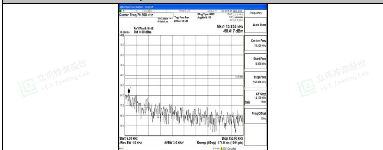
Band2_5MHz_16QAM_19175_1RB#0_0.009~0.15_0.009~0.15
