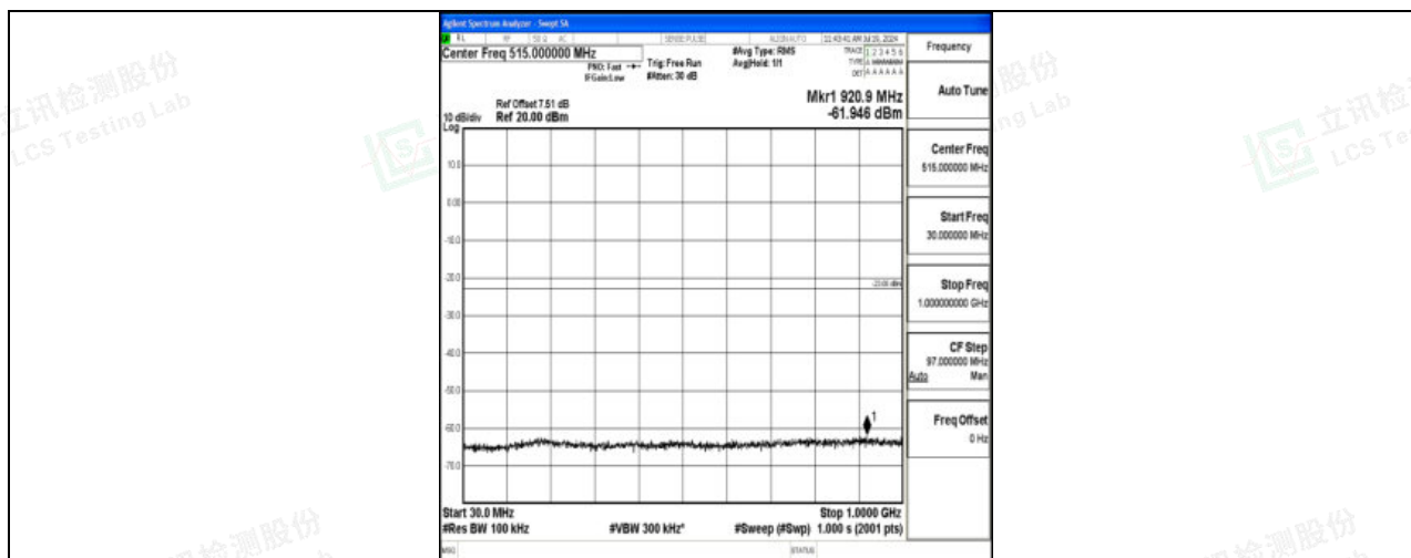
Band2_5MHz_16QAM_18900_1RB#0_30~1000_30~1000
