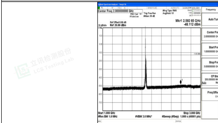
Band2_15MHz_QPSK_18900_1RB#0_1000~3000_1000~3000
