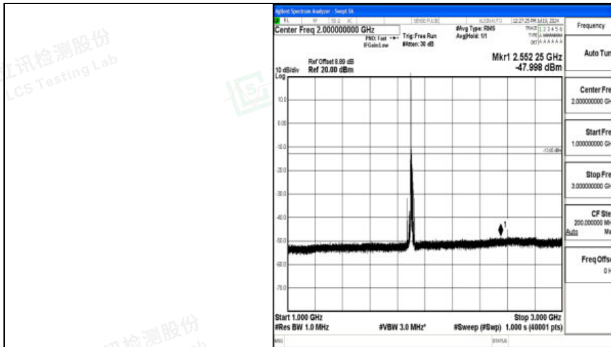
Band2_15MHz_QPSK_19125_1RB#0_1000~3000_1000~3000
