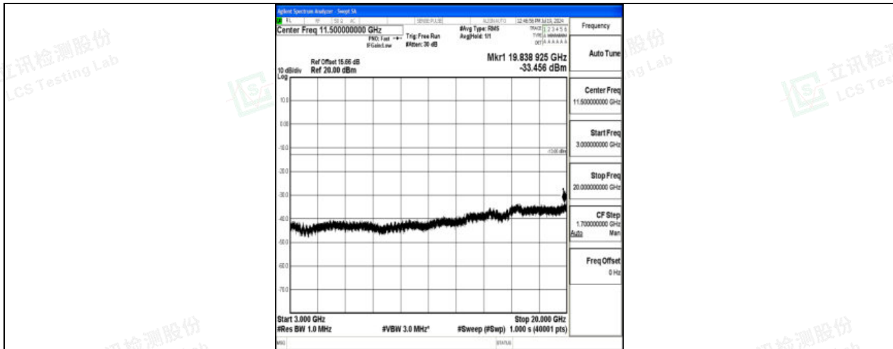
Band2_20MHz_QPSK_18900_1RB#0_3000~20000_3000~20000
