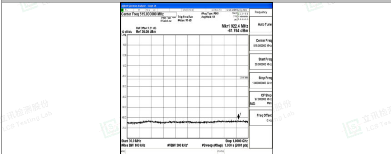
Band2_20MHz_QPSK_18900_1RB#0_30~1000_30~1000
