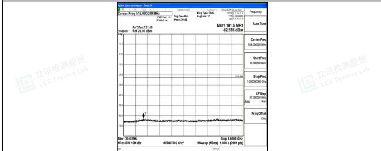
Band4_20MHz_QPSK_20175_1RB#0_30~1000_30~1000
