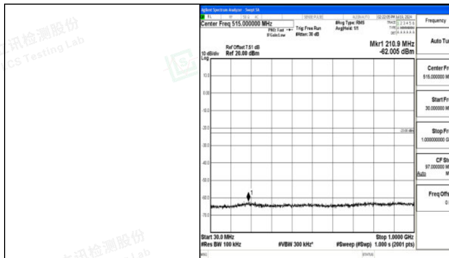
Band4_10MHz_QPSK_20350_1RB#0_30~1000_30~1000
