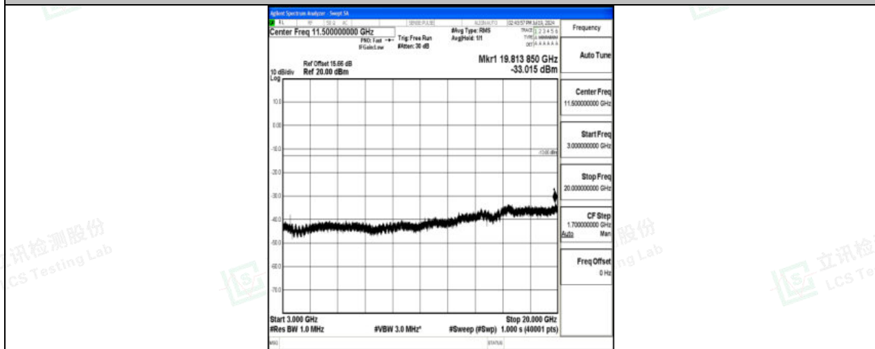
Band4_15MHz_16QAM_20325_1RB#0_3000~20000_3000~20000
