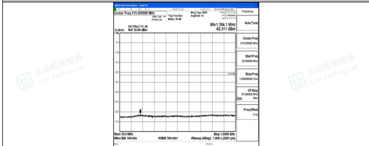
Band4_15MHz_16QAM_20325_1RB#0_30~1000_30~1000
