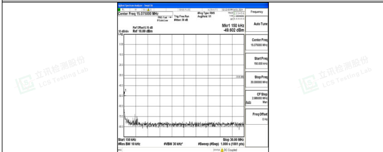
Band4_10MHz_QPSK_20350_1RB#0_0.15~30_0.15~30
