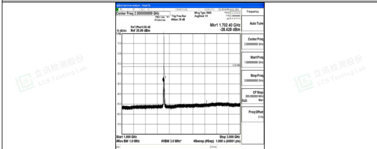
Band4_3MHz_QPSK_19965_1RB#0_1000~3000_1000~3000
