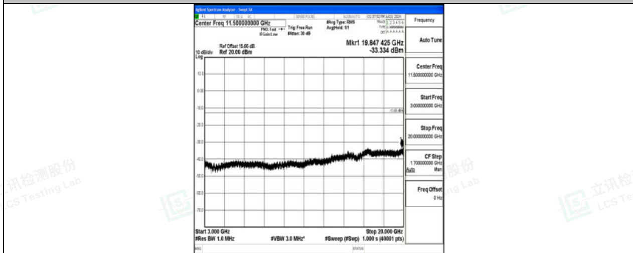
Band4_3MHz_16QAM_20385_1RB#0_3000~20000_3000~20000
