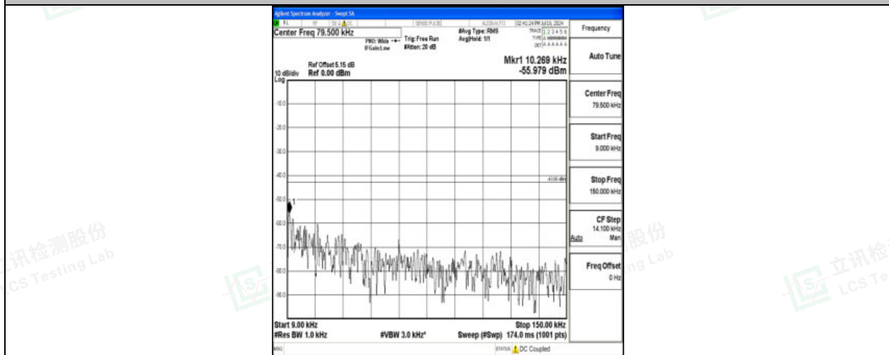
Band4_15MHz_16QAM_20025_1RB#0_0.009~0.15_0.009~0.15
