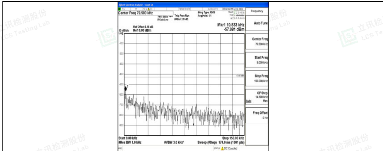
Band4_20MHz_QPSK_20175_1RB#0_0.009~0.15_0.009~0.15
