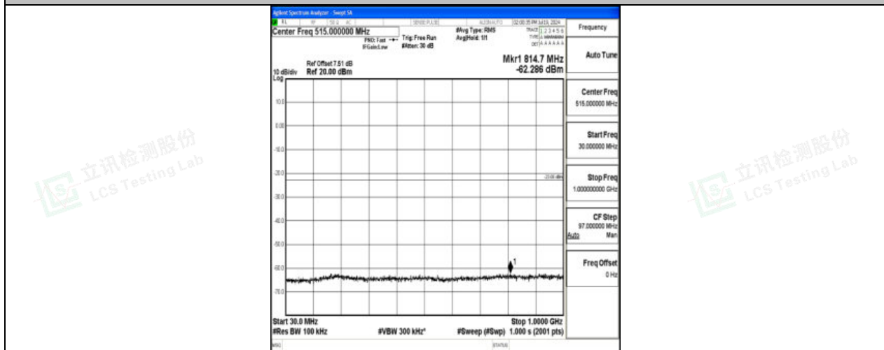
Band4_5MHz_16QAM_20375_1RB#0_30~1000_30~1000
