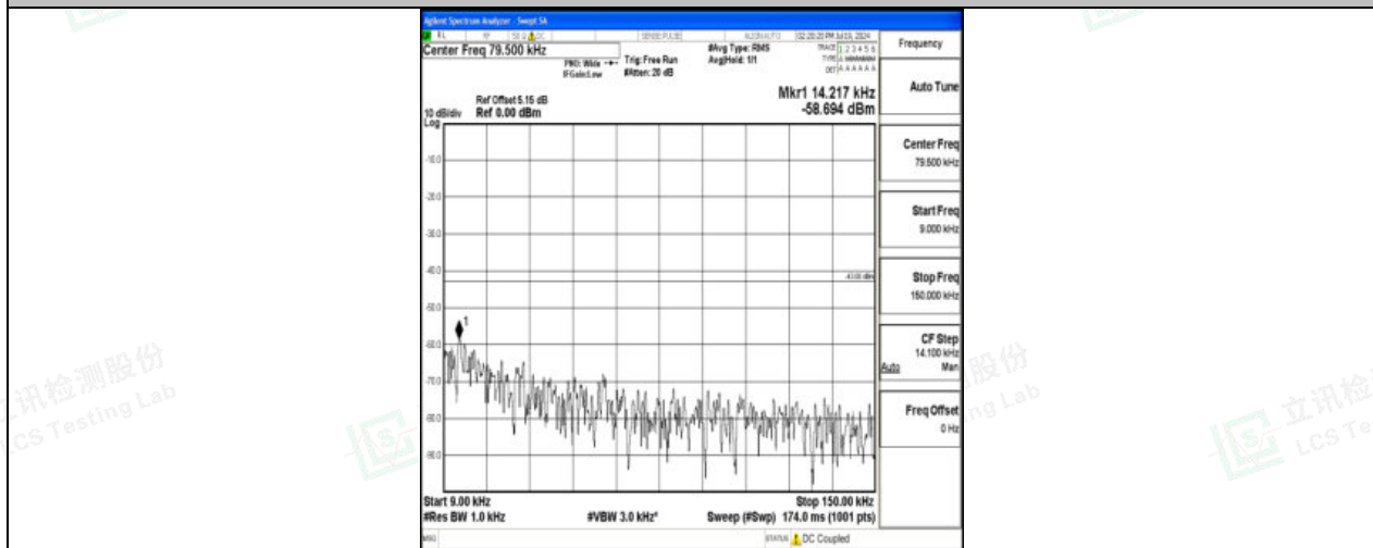
Band4_10MHz_16QAM_20000_1RB#0_0.009~0.15_0.009~0.15
