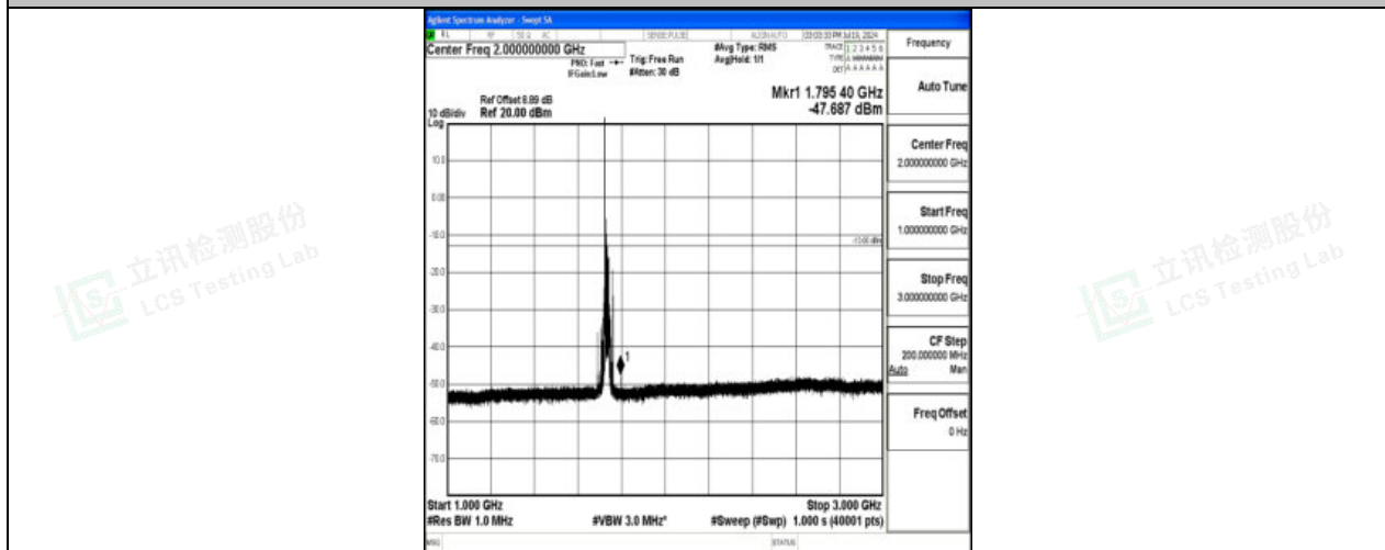
Band4_20MHz_16QAM_20175_1RB#0_1000~3000_1000~3000
