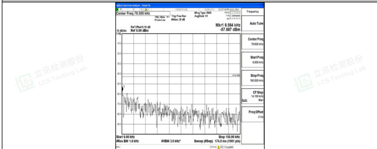
Band4_5MHz_QPSK_19975_1RB#0_0.009~0.15_0.009~0.15
