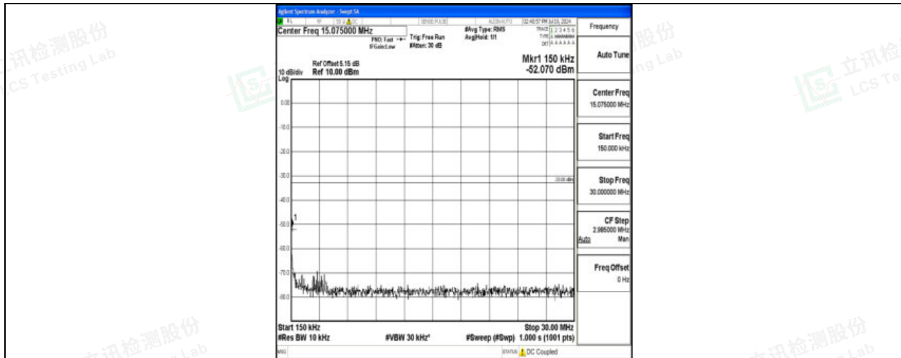
Band4_15MHz_QPSK_20025_1RB#0_0.15~30_0.15~30
