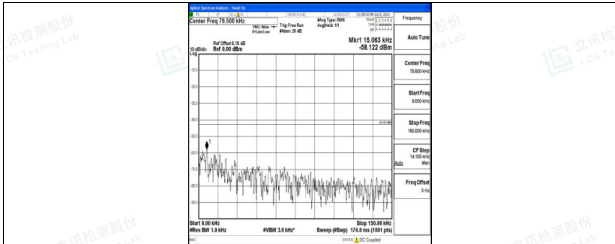
Band4_5MHz_QPSK_20175_1RB#0_0.009~0.15_0.009~0.15
