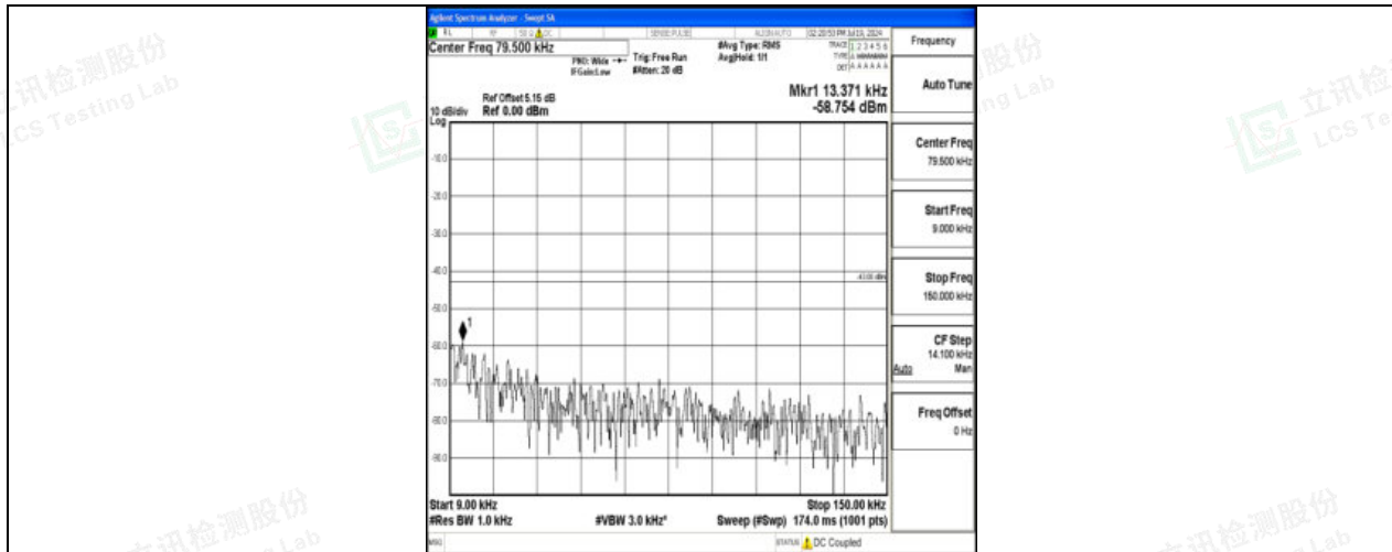
Band4_10MHz_QPSK_20175_1RB#0_0.009~0.15_0.009~0.15
