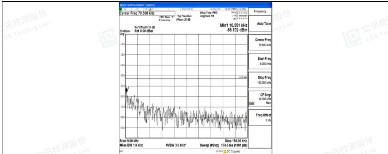
Band4_15MHz_QPSK_20175_1RB#0_0.009~0.15_0.009~0.15
