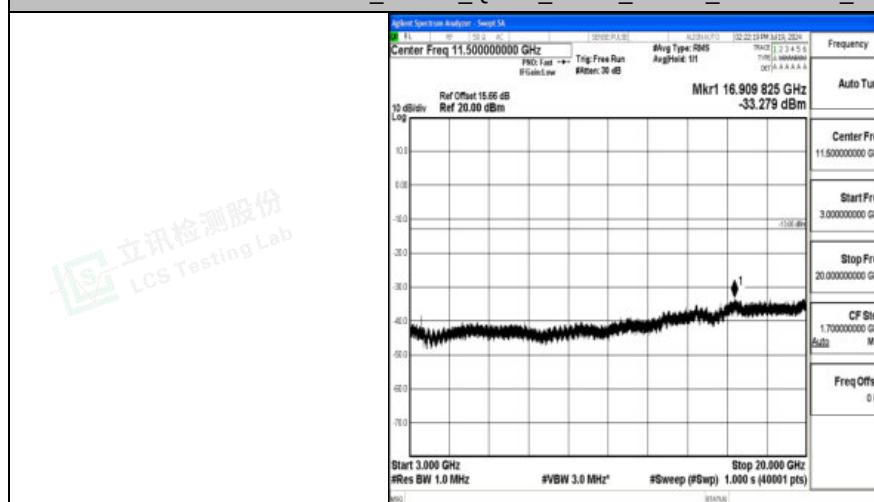
Band4_10MHz_QPSK_20350_1RB#0_3000~20000_3000~20000
