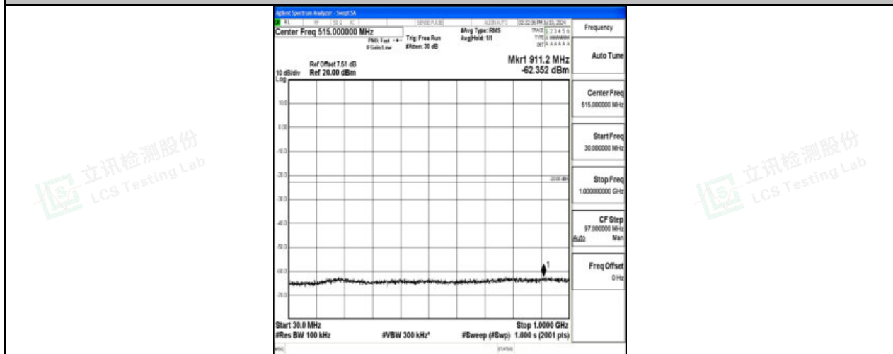
Band4_10MHz_16QAM_20350_1RB#0_30~1000_30~1000
