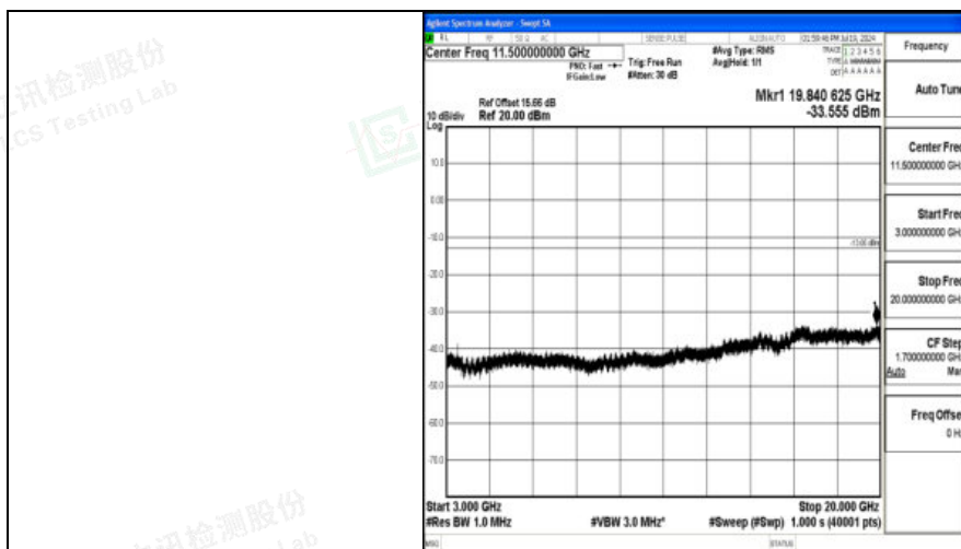
Band4 5MHz 16QAM 20175 1RB#0 3000~20000 3000~20000
