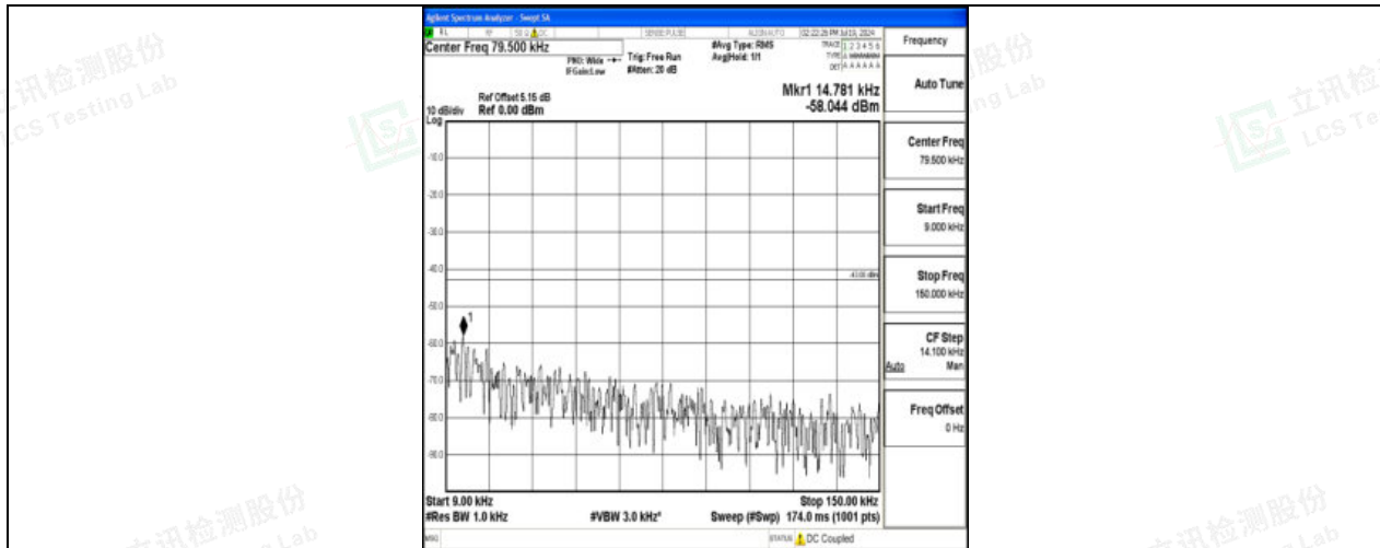
Band4_10MHz_16QAM_20350_1RB#0_0.009~0.15_0.009~0.15
