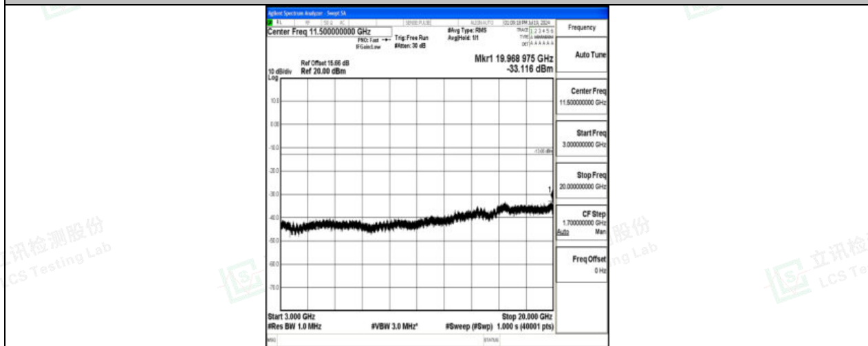
Band4_1.4MHz_16QAM_20393_1RB#0_3000~20000_3000~20000
