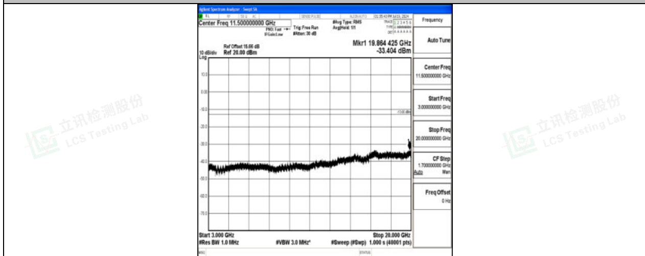
Band4_3MHz_16QAM_19965_1RB#0_3000~20000_3000~20000
