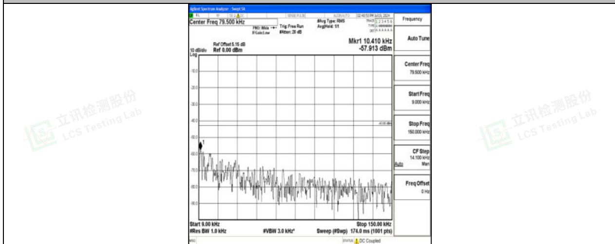
Band4_15MHz_QPSK_20025_1RB#0_0.009~0.15_0.009~0.15
