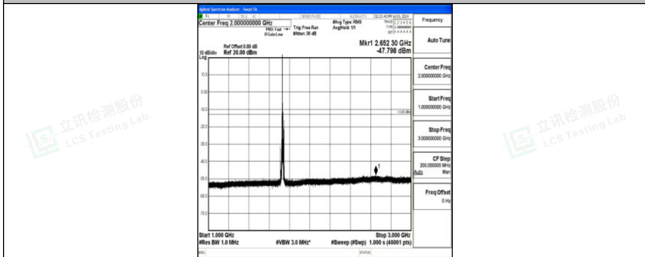
Band4_10MHz_16QAM_20175_1RB#0_1000~3000_1000~3000
