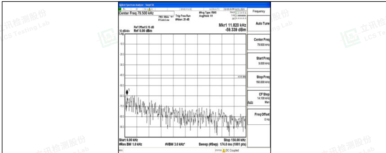
Band4_5MHz_16QAM_20375_1RB#0_0.009~0.15_0.009~0.15
