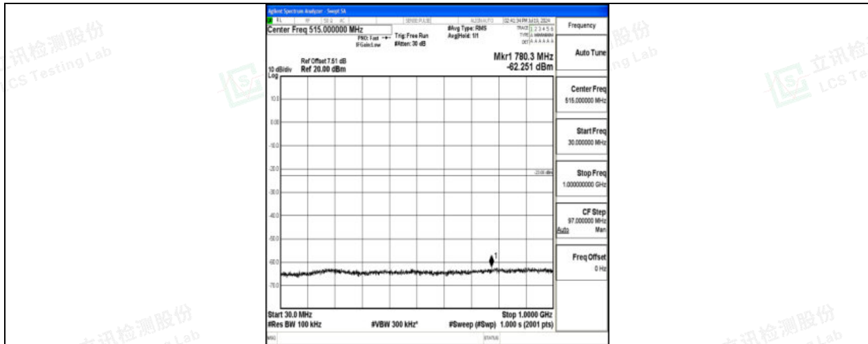
Band4_15MHz_16QAM_20025_1RB#0_30~1000_30~1000
