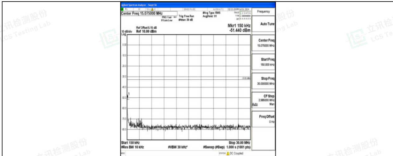
Band4_10MHz_16QAM_20175_1RB#0_0.15~30_0.15~30
