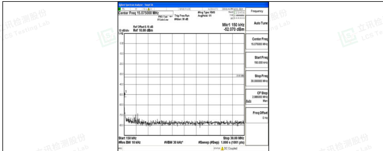
Band4_20MHz_QPSK_20050_1RB#0_0.15~30_0.15~30
