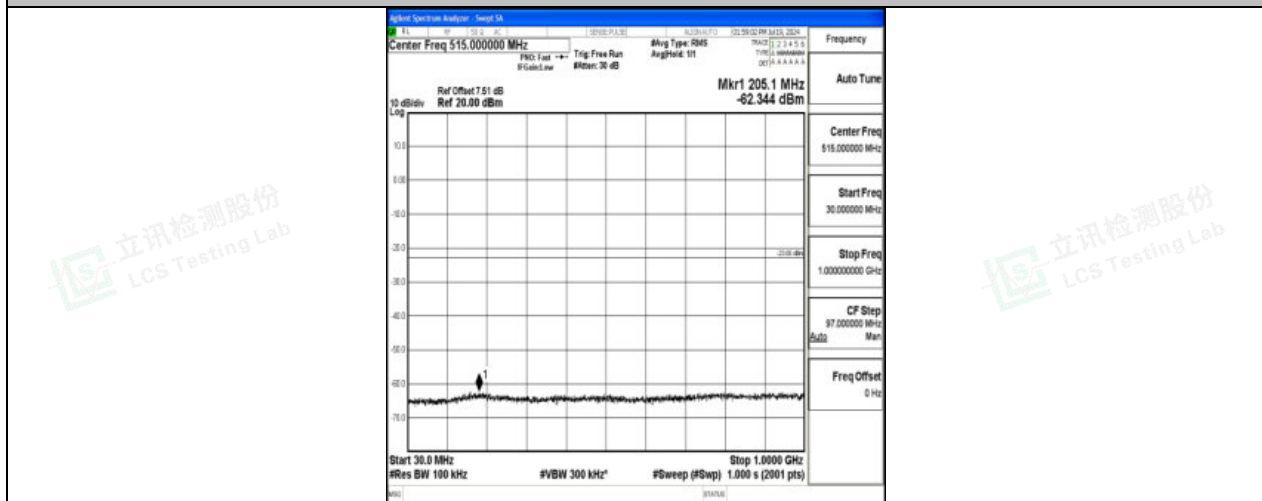
Band4_5MHz_QPSK_20175_1RB#0_30~1000_30~1000
