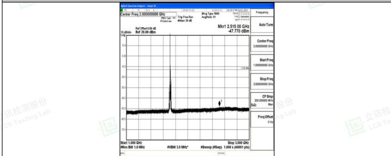
Band4_10MHz_16QAM_20000_1RB#0_1000~3000_1000~3000
