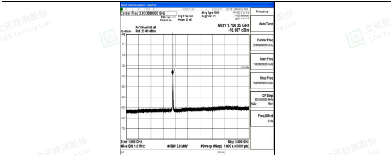
Band4_1.4MHz_16QAM_20393_1RB#0_1000~3000_1000~3000
