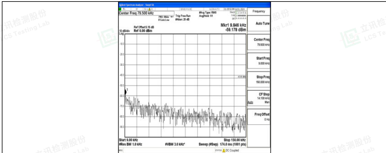
Band4_3MHz_QPSK_20175_1RB#0_0.009~0.15_0.009~0.15
