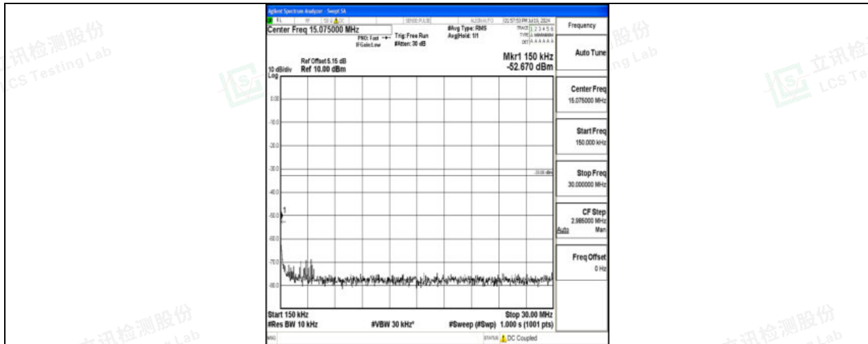
Band4_5MHz_QPSK_19975_1RB#0_0.15~30_0.15~30
