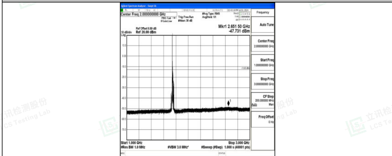
Band4_15MHz_QPSK_20325_1RB#0_1000~3000_1000~3000
