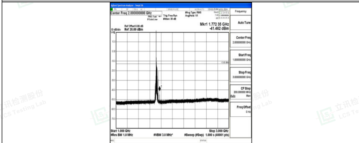
Band4_20MHz_16QAM_20050_1RB#0_1000~3000_1000~3000
