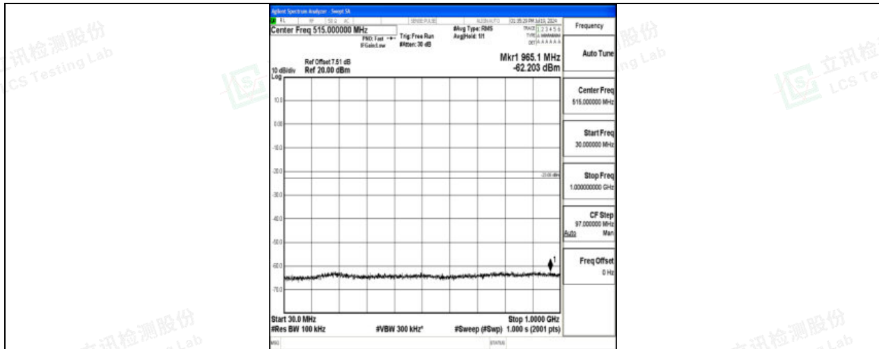
Band4_3MHz_16QAM_19965_1RB#0_30~1000_30~1000
