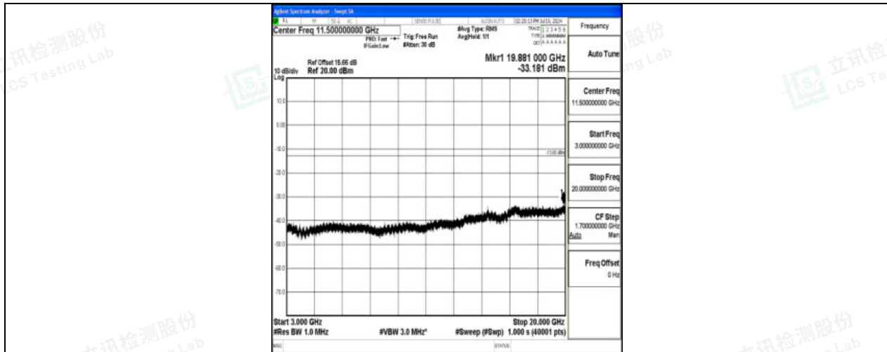
Band4_10MHz_QPSK_20000_1RB#0_3000~20000_3000~20000
