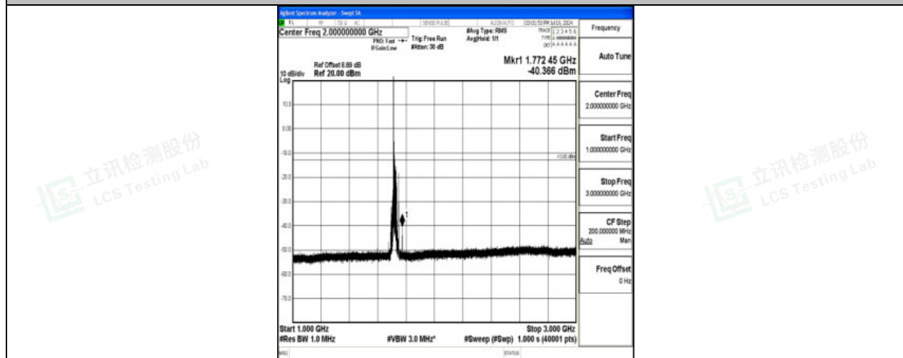
Band4_20MHz_QPSK_20050_1RB#0_1000~3000_1000~3000
