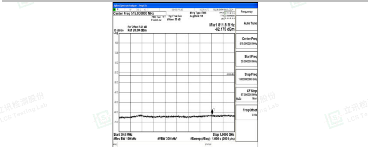
Band4_3MHz_16QAM_20175_1RB#0_30~1000_30~1000
