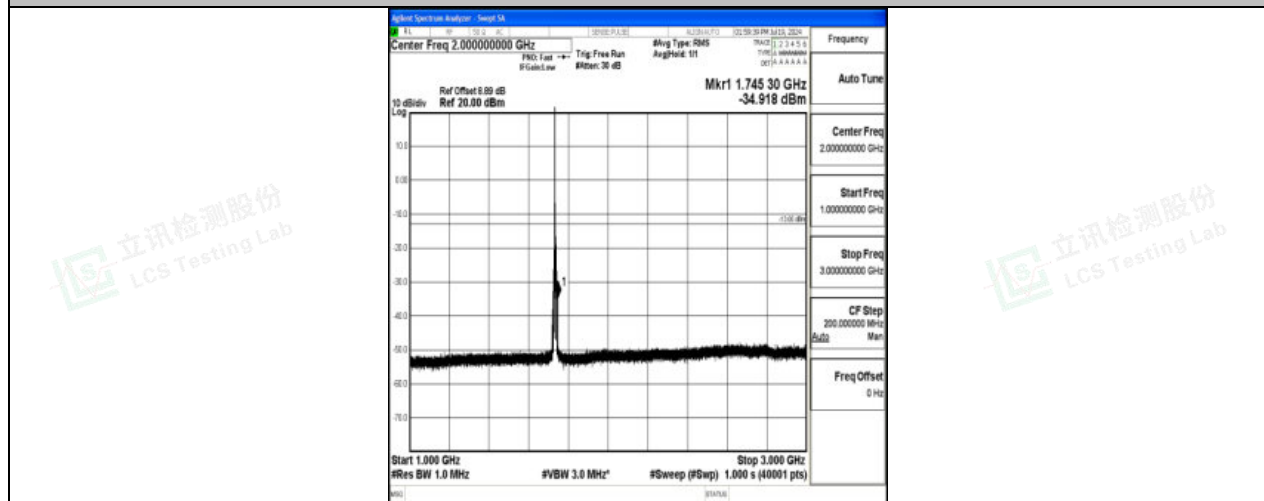
Band4_5MHz_16QAM_20175_1RB#0_1000~3000_1000~3000
