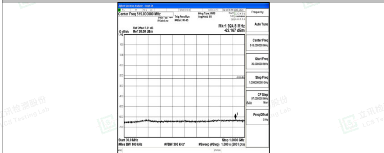
Band4_15MHz_16QAM_20175_1RB#0_30~1000_30~1000
