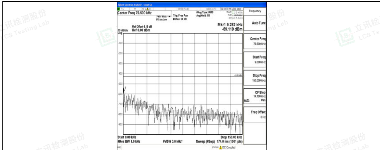
Band4_15MHz_16QAM_20325_1RB#0_0.009~0.15_0.009~0.15
