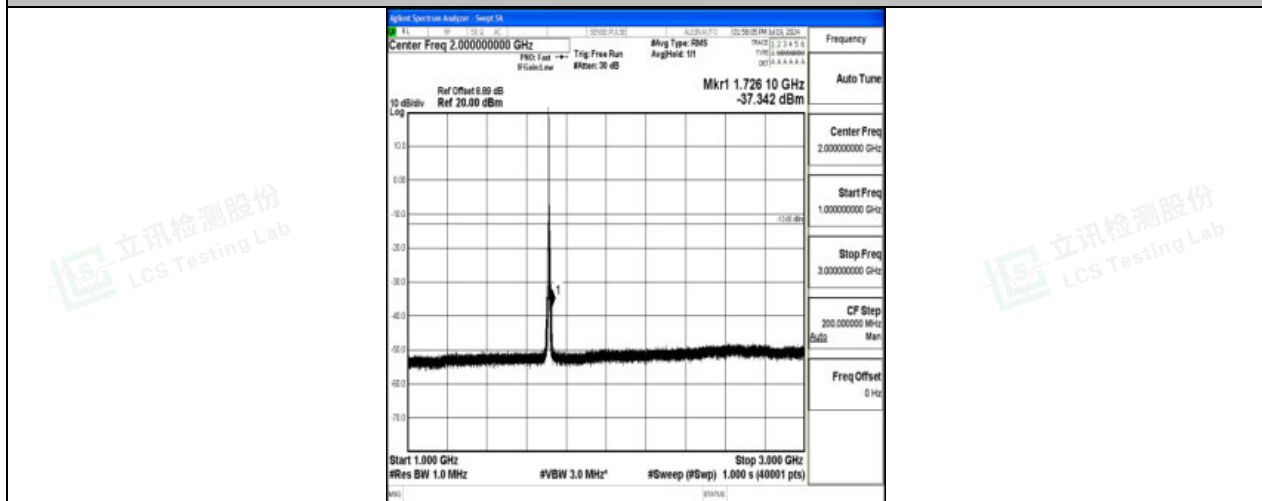
Band4_5MHz_QPSK_19975_1RB#0_1000~3000_1000~3000
