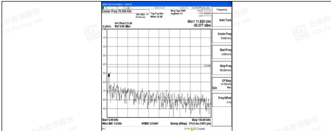
Band4_1.4MHz_16QAM_20393_1RB#0_0.009~0.15_0.009~0.15
