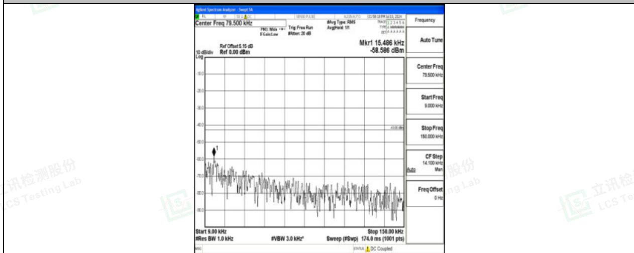
Band4_5MHz_16QAM_19975_1RB#0_0.009~0.15_0.009~0.15
