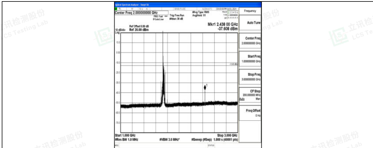
Band4_20MHz_QPSK_20175_1RB#0_1000~3000_1000~3000
