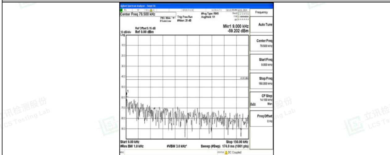
Band4_10MHz_QPSK_20350_1RB#0_0.009~0.15_0.009~0.15
