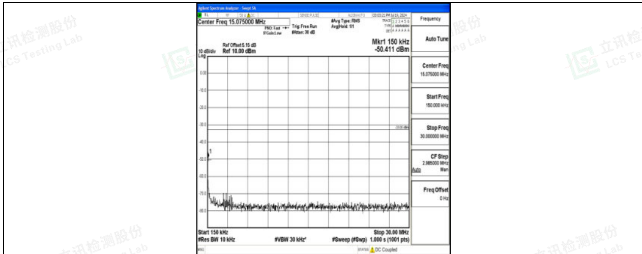
Band4_20MHz_16QAM_20175_1RB#0_0.15~30_0.15~30
