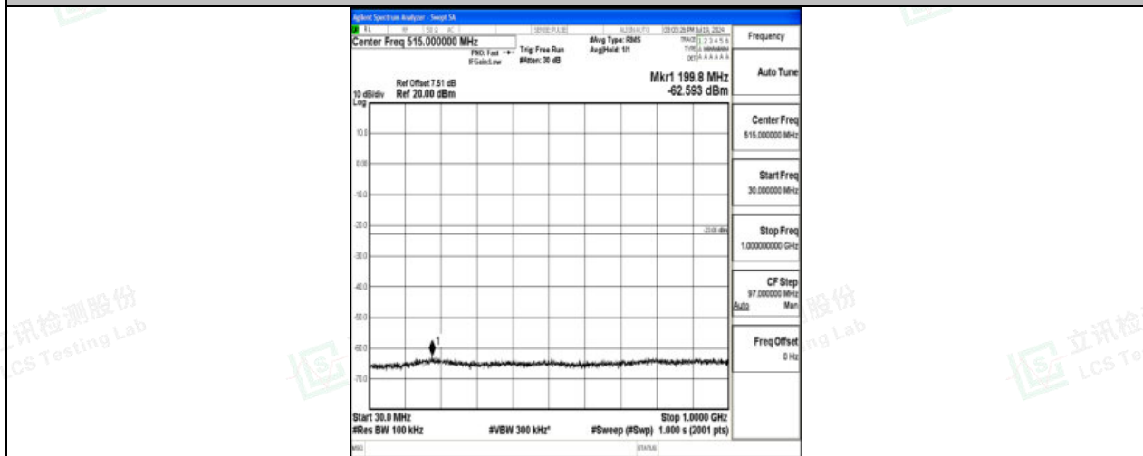
Band4_20MHz_16QAM_20175_1RB#0_30~1000_30~1000
