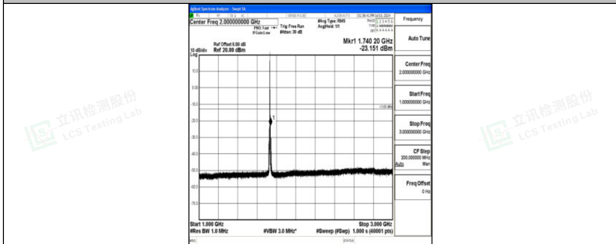
Band4_3MHz_16QAM_20175_1RB#0_1000~3000_1000~3000
