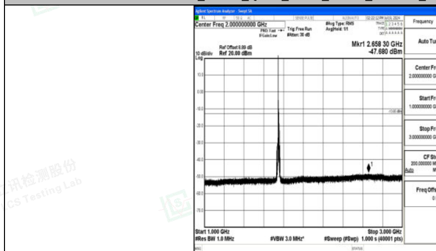
Band4_10MHz_QPSK_20350_1RB#0_1000~3000_1000~3000
