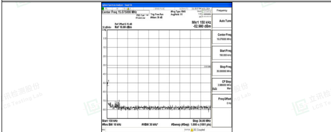
Band4_3MHz_QPSK_20175_1RB#0_0.15~30_0.15~30
