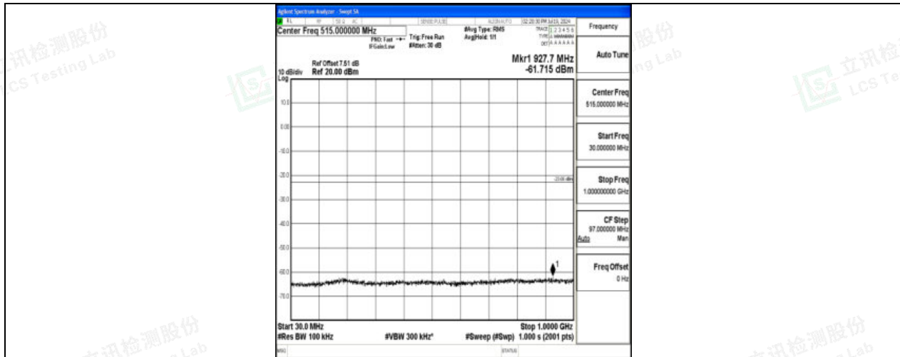
Band4_10MHz_16QAM_20000_1RB#0_30~1000_30~1000
