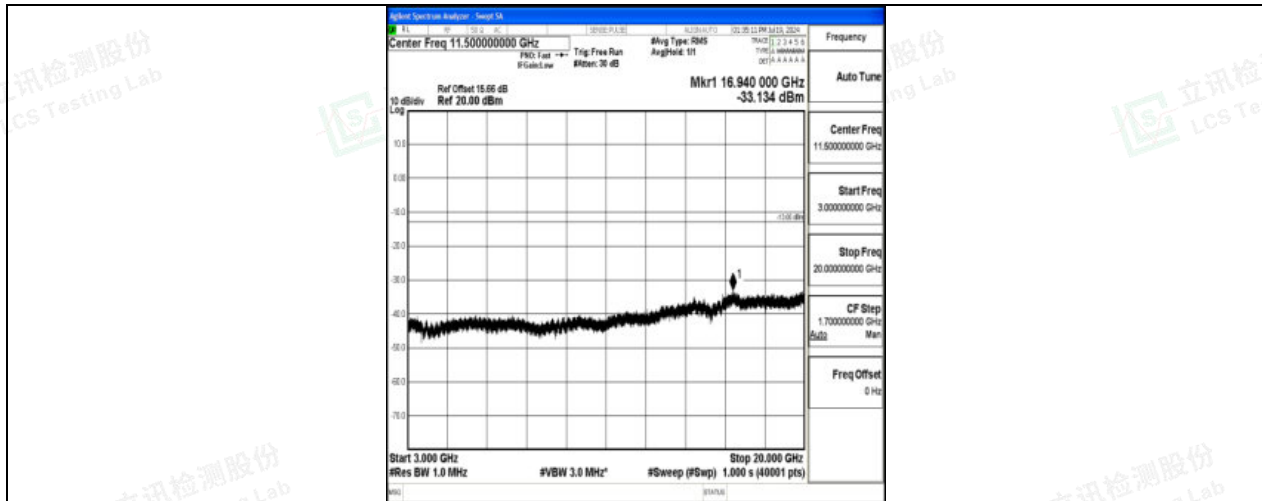
Band4_3MHz_QPSK_19965_1RB#0_3000~20000_3000~20000
