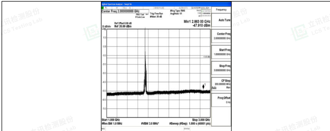
Band4_15MHz_16QAM_20325_1RB#0_1000~3000_1000~3000
