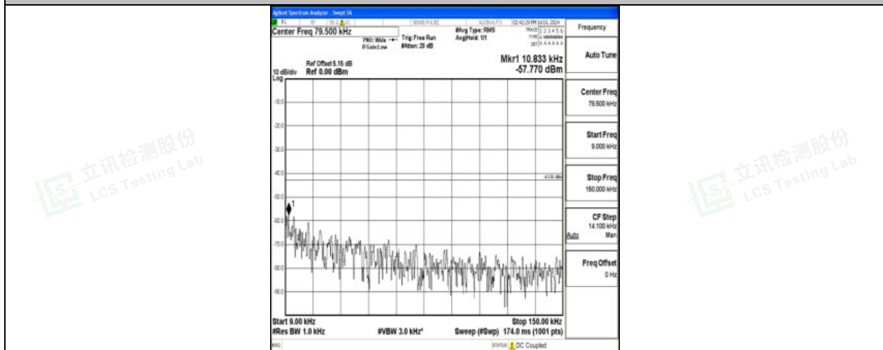
Band4_15MHz_16QAM_20175_1RB#0_0.009~0.15_0.009~0.15
