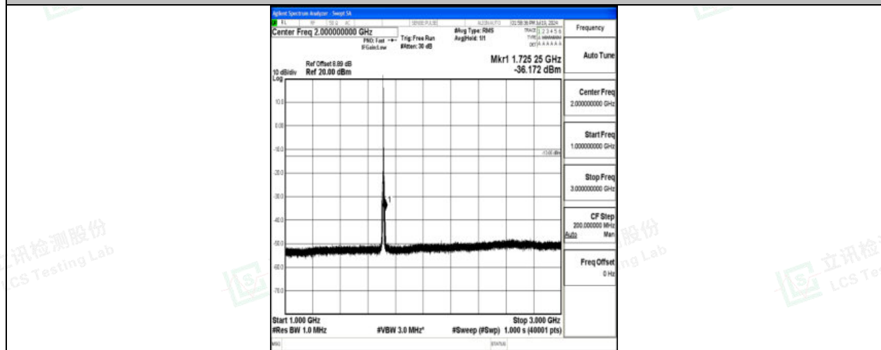
Band4_5MHz_16QAM_19975_1RB#0_1000~3000_1000~3000
