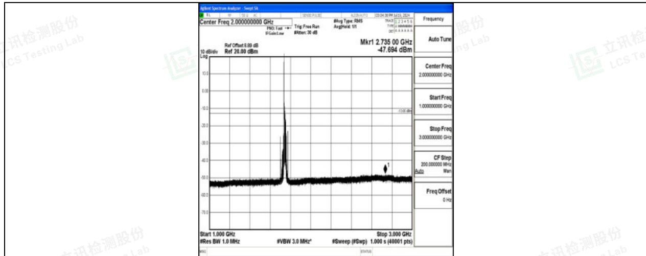
Band4_20MHz_16QAM_20300_1RB#0_1000~3000_1000~3000
