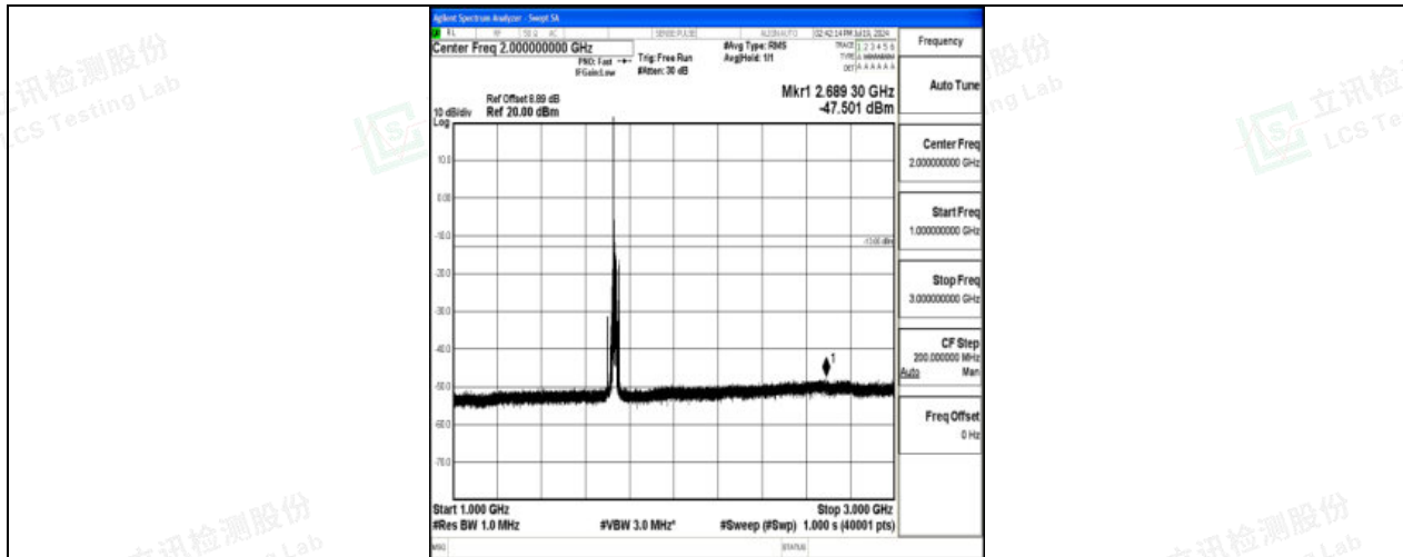
Band4_15MHz_QPSK_20175_1RB#0_1000~3000_1000~3000
