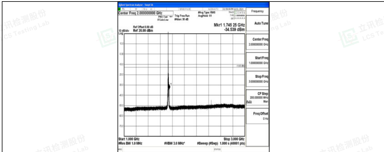
Band4_5MHz_QPSK_20175_1RB#0_1000~3000_1000~3000
