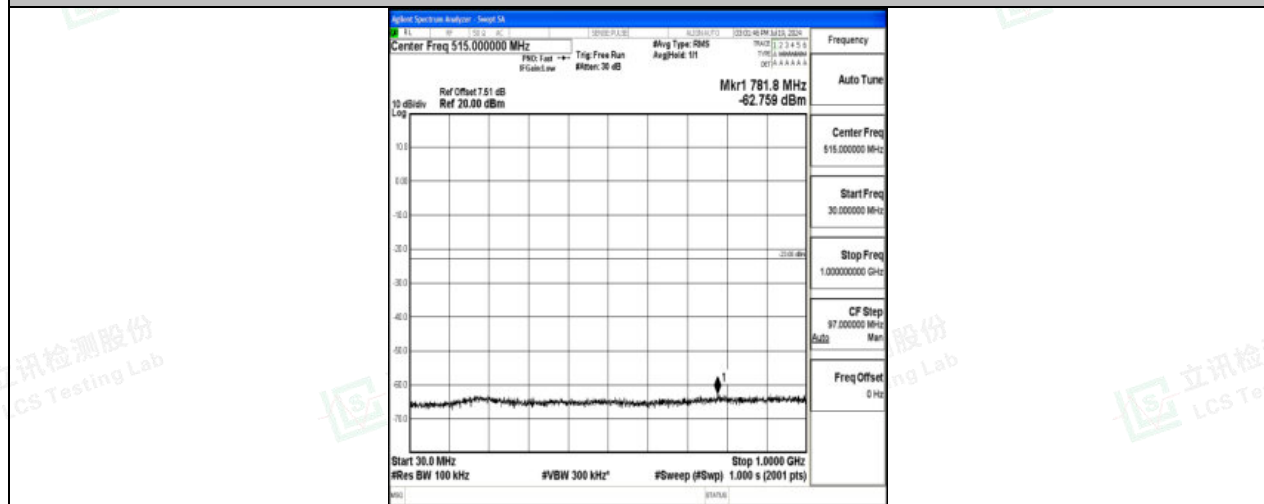
Band4_20MHz_QPSK_20050_1RB#0_30~1000_30~1000
