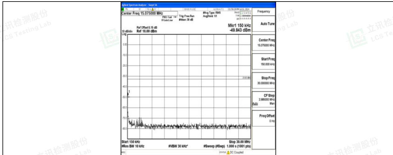
Band4_5MHz_16QAM_20175_1RB#0_0.15~30_0.15~30
