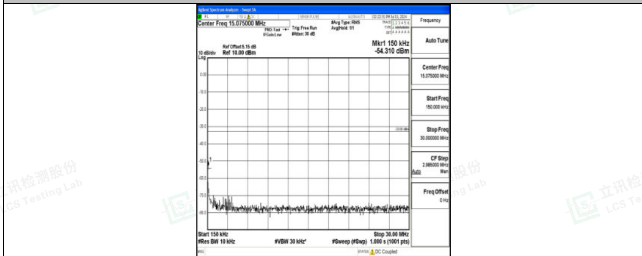
Band4_10MHz_16QAM_20350_1RB#0_0.15~30_0.15~30
