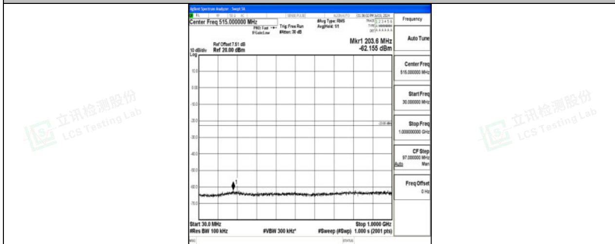
Band4_3MHz_QPSK_20175_1RB#0_30~1000_30~1000
