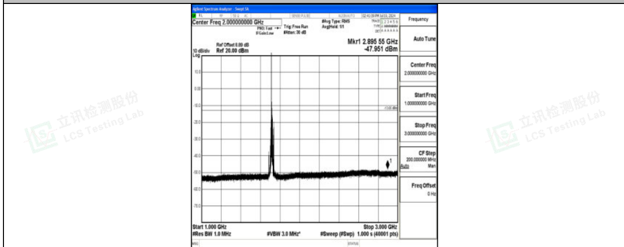
Band4_15MHz_QPSK_20025_1RB#0_1000~3000_1000~3000
