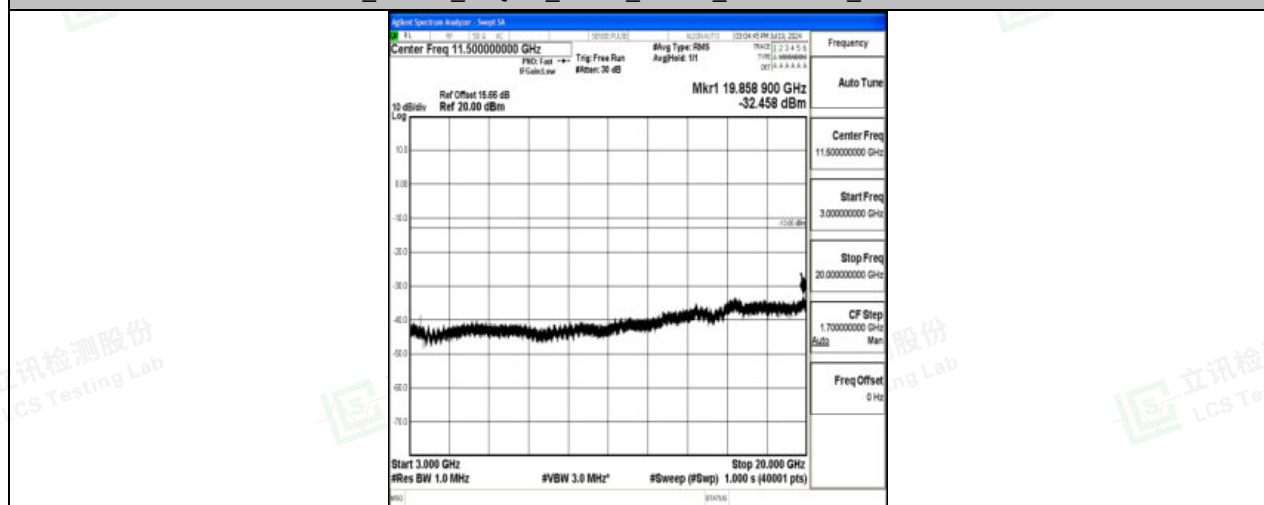
Band4_20MHz_16QAM_20300_1RB#0_3000~20000_3000~20000
