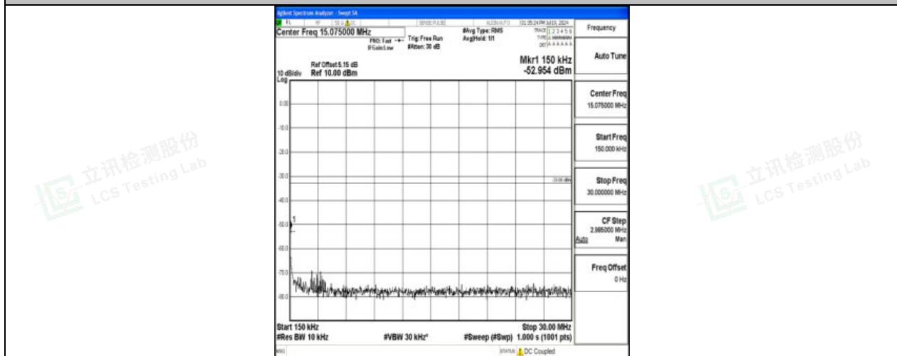
Band4_3MHz_16QAM_19965_1RB#0_0.15~30_0.15~30
