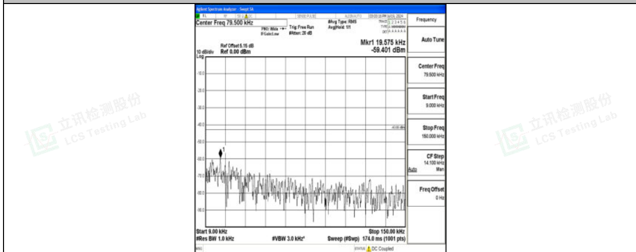
Band4_20MHz_16QAM_20175_1RB#0_0.009~0.15_0.009~0.15
