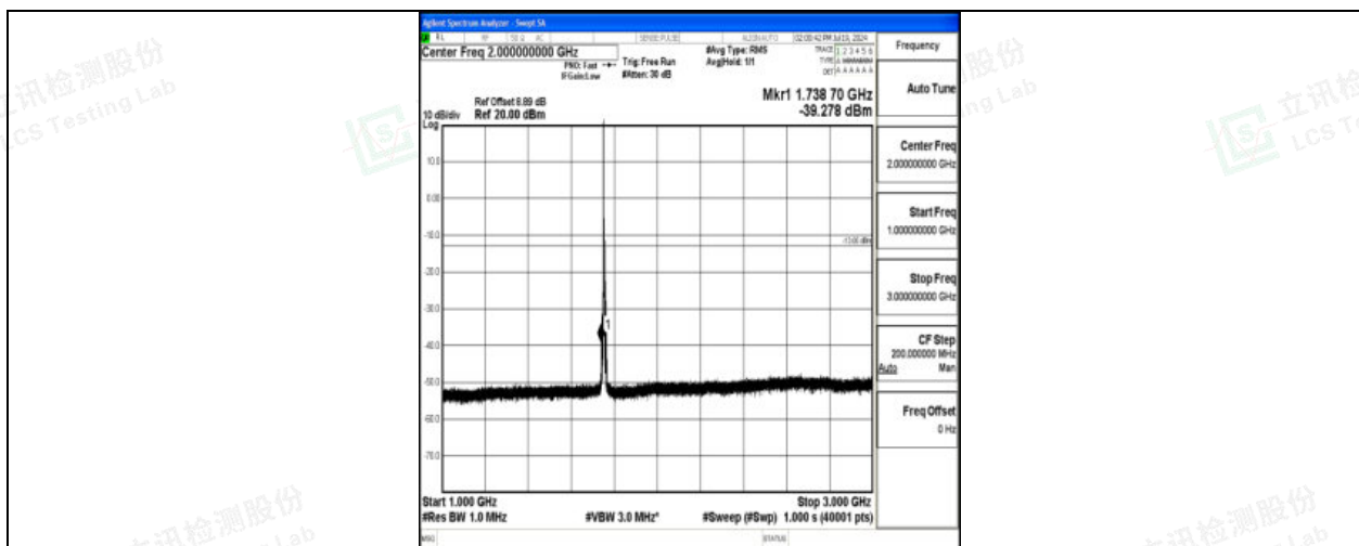
Band4_5MHz_16QAM_20375_1RB#0_1000~3000_1000~3000
