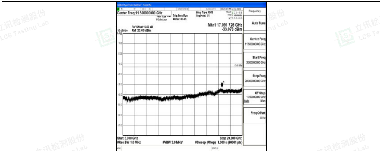
Band4_10MHz_16QAM_20175_1RB#0_3000~20000_3000~20000
