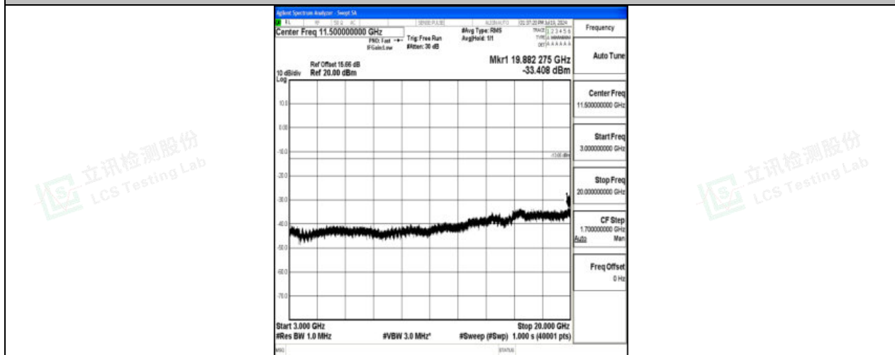
Band4_3MHz_QPSK_20385_1RB#0_3000~20000_3000~20000
