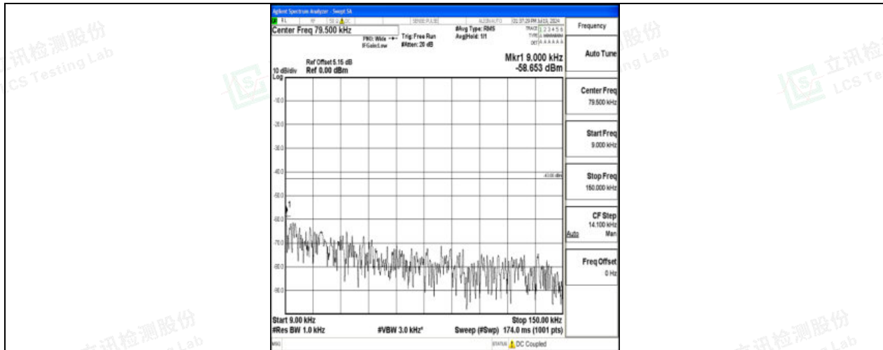
Band4_3MHz_16QAM_20385_1RB#0_0.009~0.15_0.009~0.15
