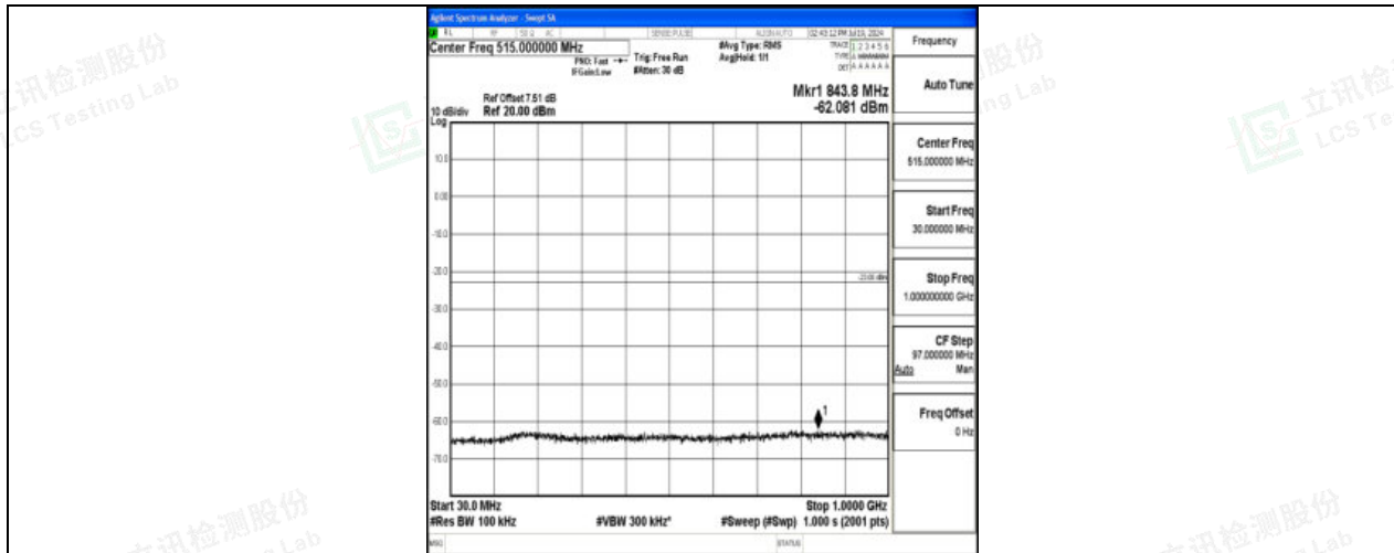
Band4_15MHz_QPSK_20325_1RB#0_30~1000_30~1000
