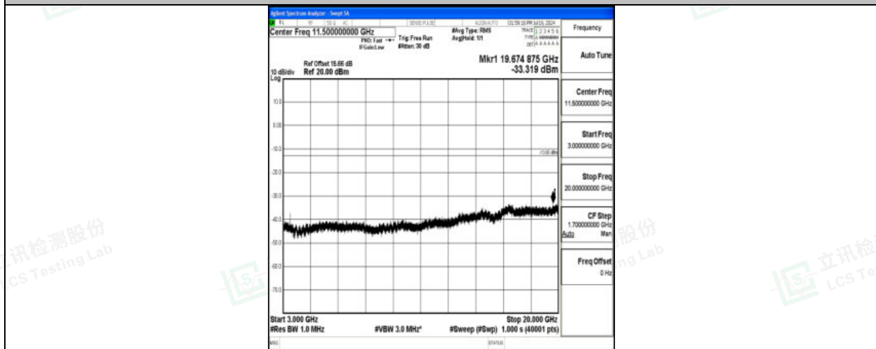
Band4_5MHz_QPSK_20175_1RB#0_3000~20000_3000~20000
