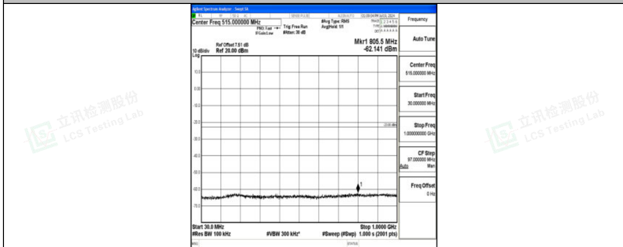
Band4_1.4MHz_16QAM_20393_1RB#0_30~1000_30~1000
