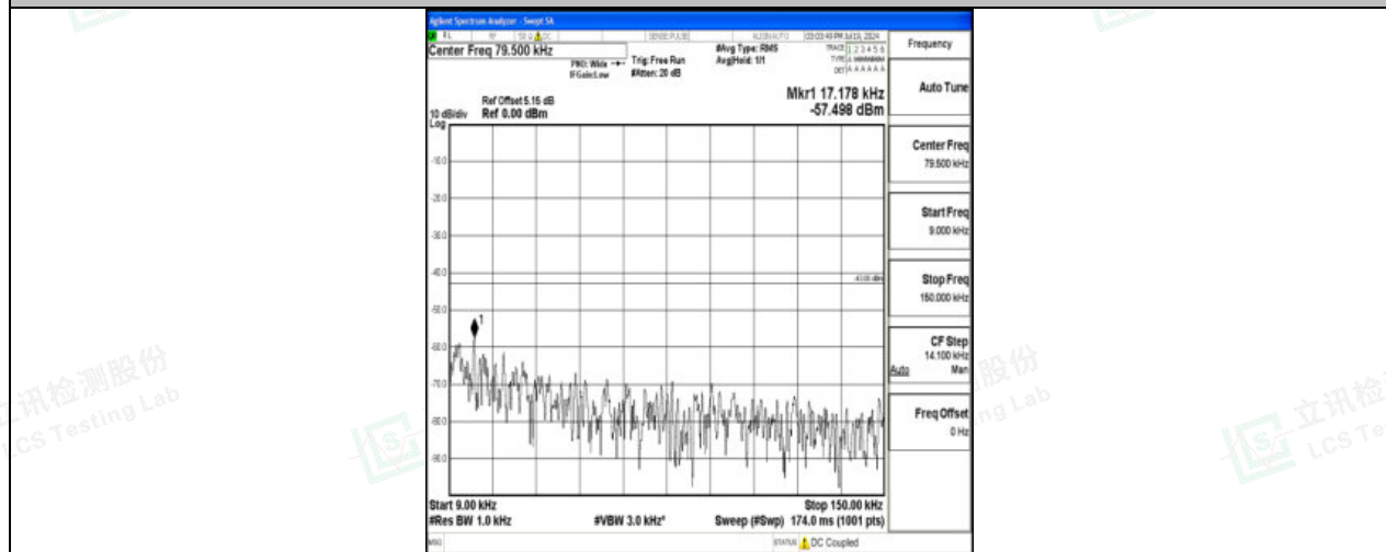
Band4_20MHz_QPSK_20300_1RB#0_0.009~0.15_0.009~0.15
