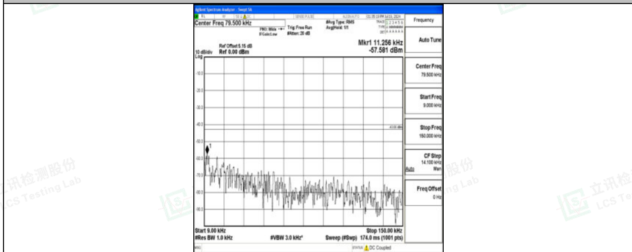
Band4_3MHz_16QAM_19965_1RB#0_0.009~0.15_0.009~0.15
