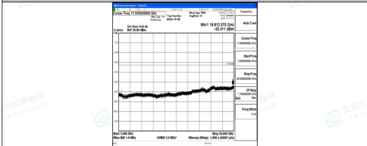
Band4_20MHz_QPSK_20175_1RB#0_3000~20000_3000~20000
