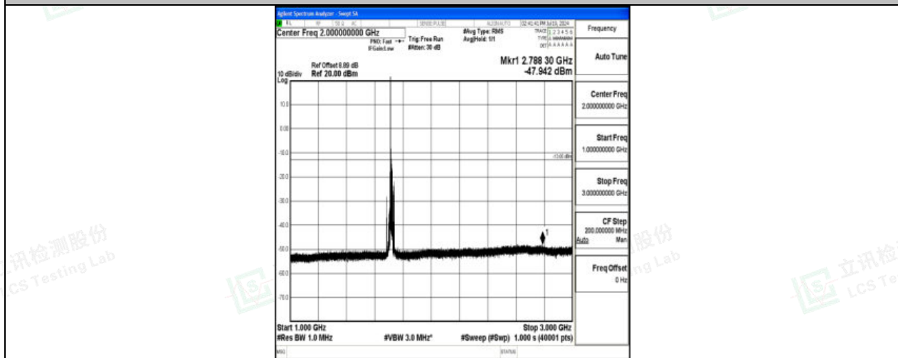
Band4_15MHz_16QAM_20025_1RB#0_1000~3000_1000~3000
