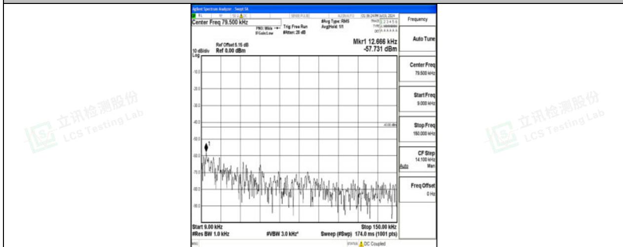
Band4_3MHz_16QAM_20175_1RB#0_0.009~0.15_0.009~0.15
