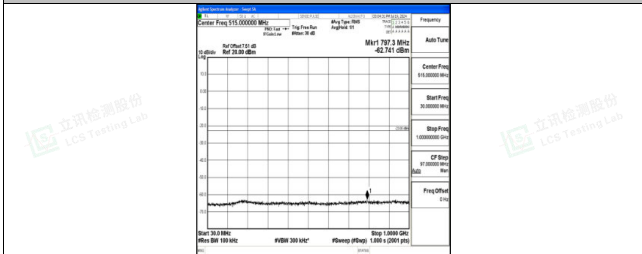
Band4_20MHz_16QAM_20300_1RB#0_30~1000_30~1000
