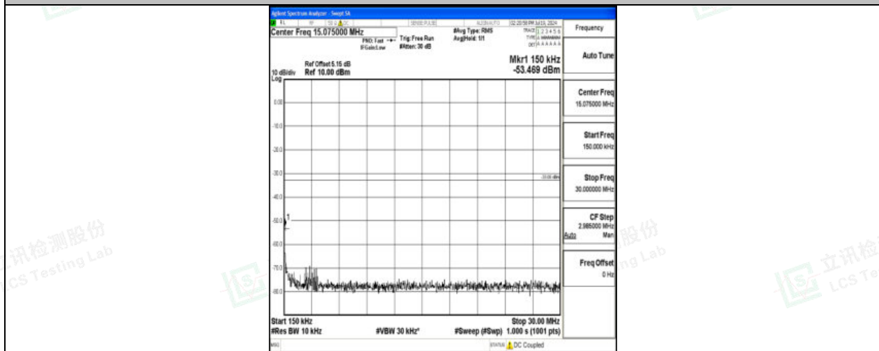
Band4_10MHz_QPSK_20175_1RB#0_0.15~30_0.15~30
