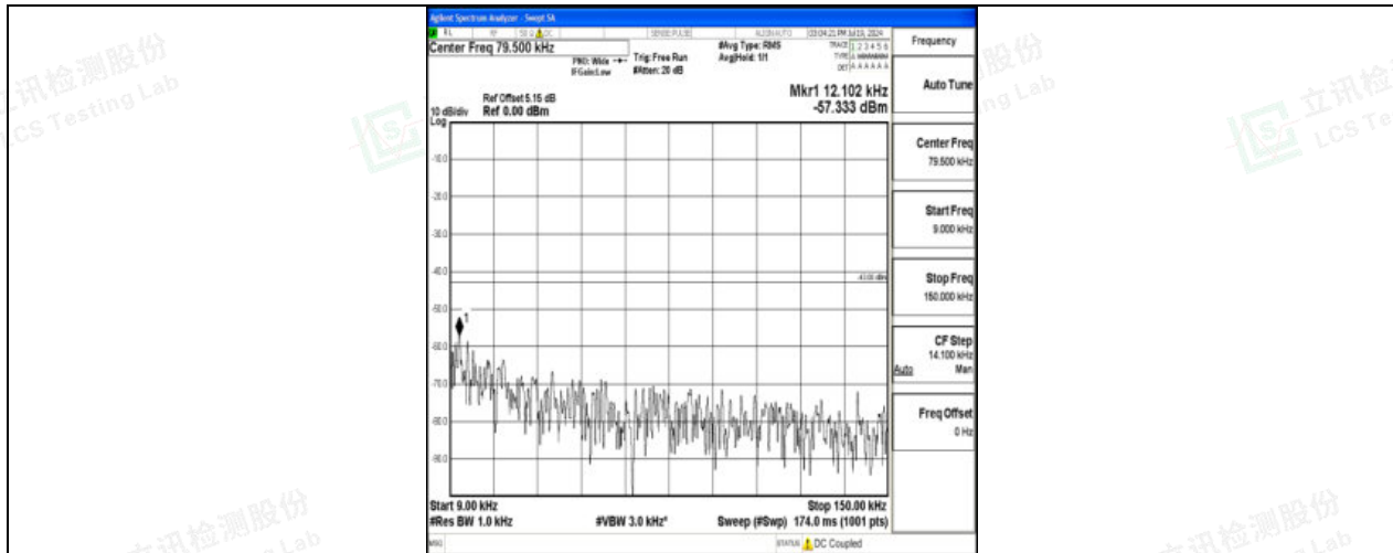
Band4_20MHz_16QAM_20300_1RB#0_0.009~0.15_0.009~0.15
