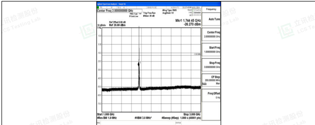
Band4_3MHz_16QAM_20385_1RB#0_1000~3000_1000~3000
