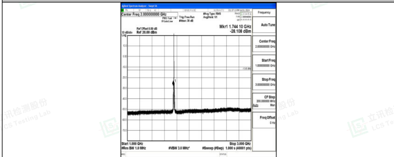
Band4_3MHz_QPSK_20385_1RB#0_1000~3000_1000~3000
