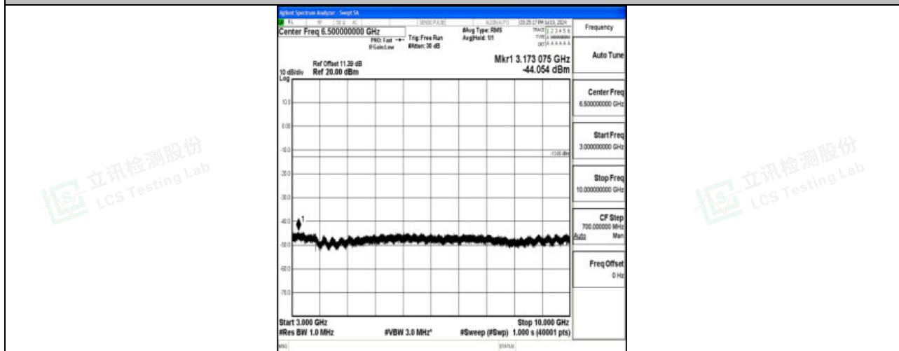
Band5_1.4MHz_16QAM_20643_1RB#0_3000~10000_3000~10000
