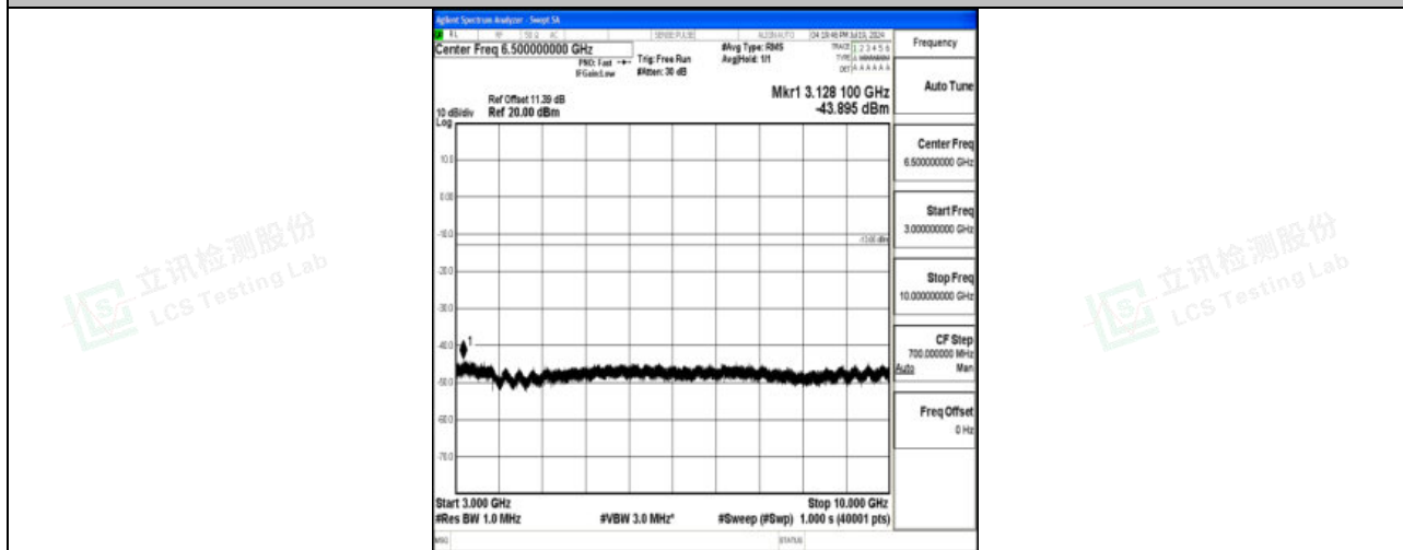
Band5_5MHz_16QAM_20625_1RB#0_3000~10000_3000~10000
