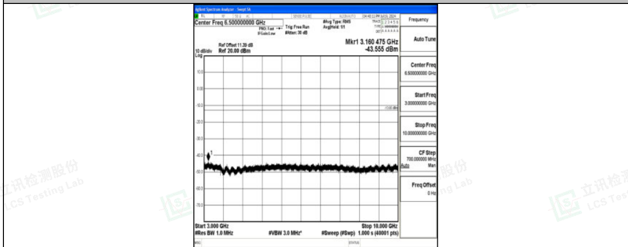
Band5_10MHz_QPSK_20450_1RB#0_3000~10000_3000~10000
