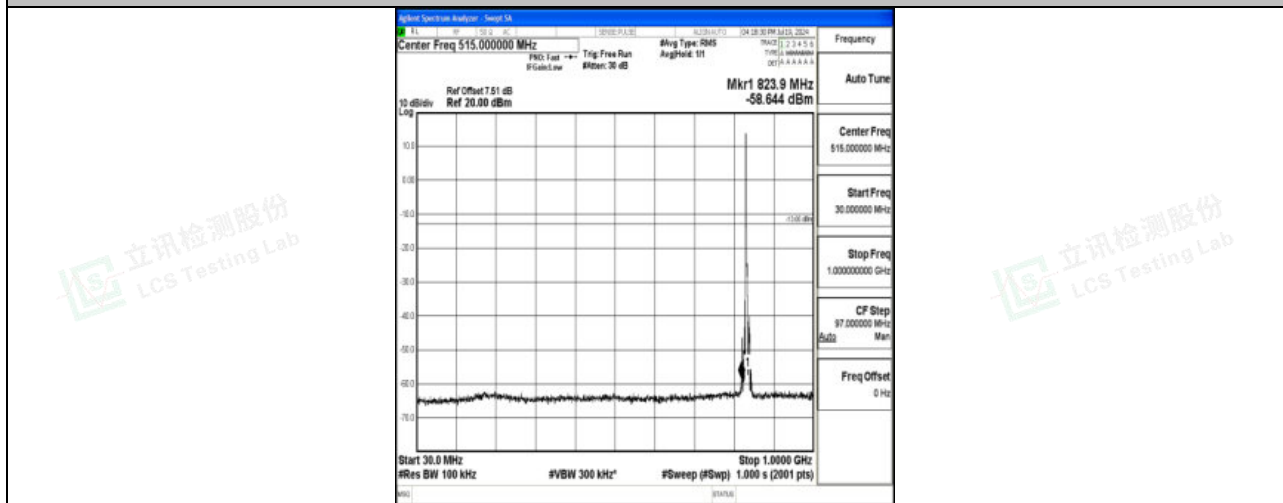
Band5_5MHz_16QAM_20525_1RB#0_30~1000_30~1000
