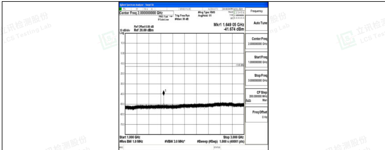
Band5_10MHz_QPSK_20450_1RB#0_1000~3000_1000~3000
