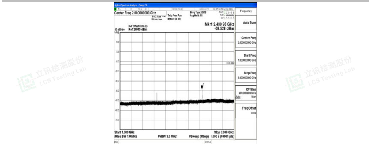
Band5_5MHz_16QAM_20425_1RB#0_1000~3000_1000~3000
