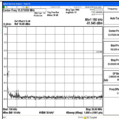
Band12_5MHz_QPSK_23155_1RB#0_0.15~30_0.15~30
