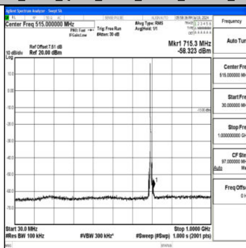
Band12 5MHz QPSK 23035 1RB#0 30~1000 30~1000
