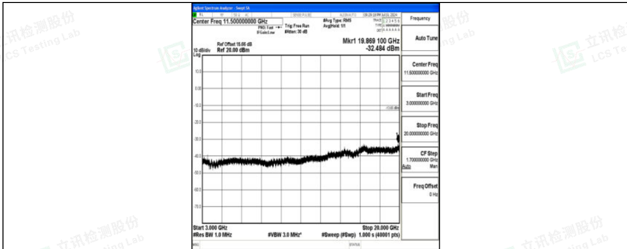
Band66_10MHz_16QAM_132322_1RB#0_3000~20000_3000~20000
