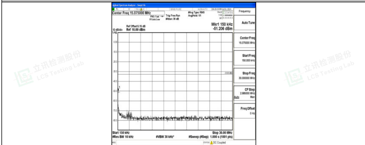
Band66_10MHz_QPSK_132622_1RB#0_0.15~30_0.15~30
