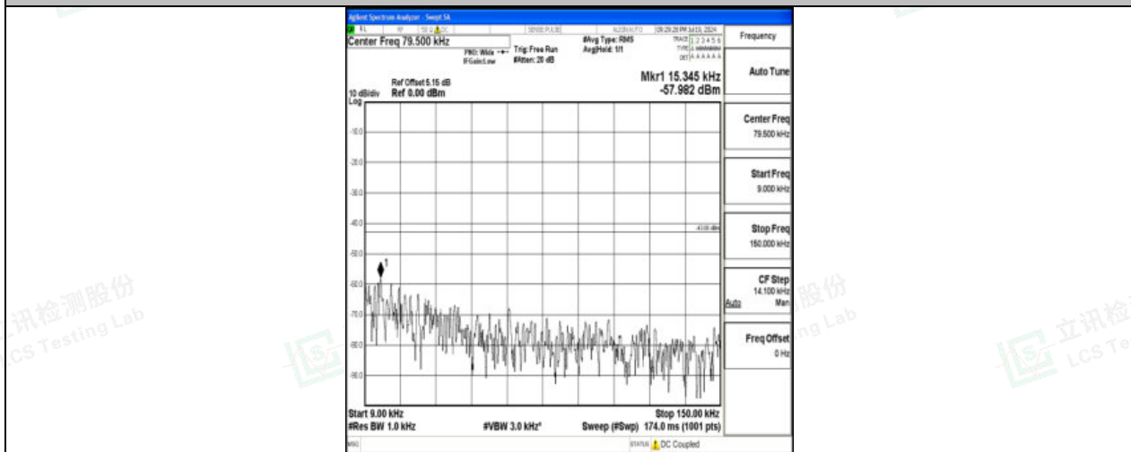
Band66_10MHz_QPSK_132622_1RB#0_0.009~0.15_0.009~0.15
